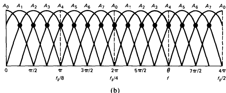
Fig. 10—Operation of the FTLS for M=8 , N=4 : (a) first stage, and (b) second stage.
