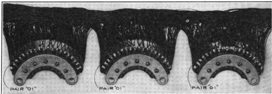
FIG. 48.—Wiring of connector-switch banks.
