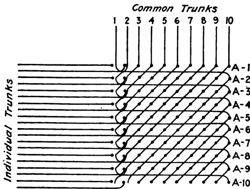
FIG. 17.—Individual trunks with slipped common trunks.
