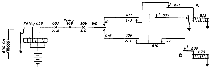
FIG. 220.—Principle of register selection.
