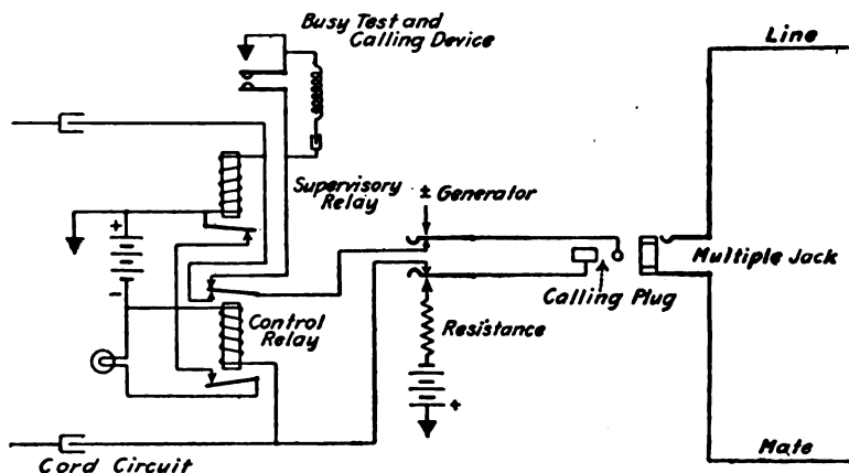
FIG. 169.—Outgoing trunk to district station.
