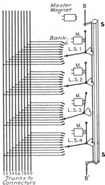
FIG. 35.—Scheme of master switch control of Keith line switches.
