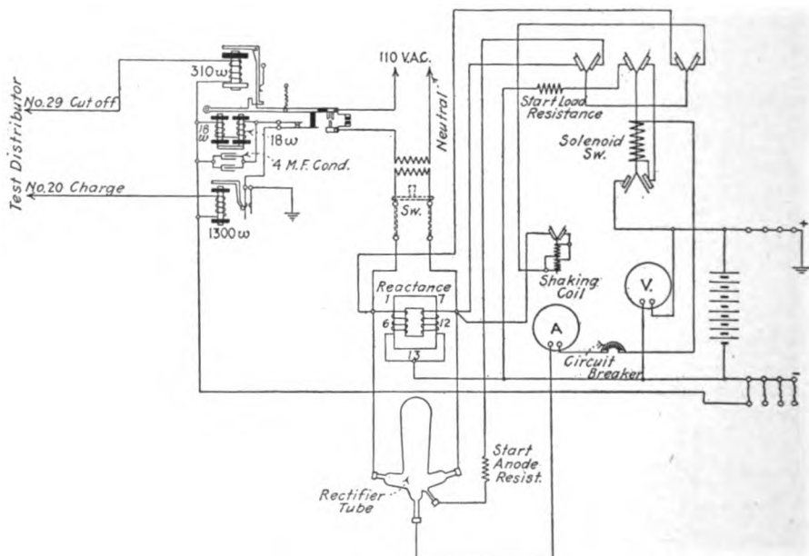
FIG. 244.—Circuits of a Mercury arc rectifier charging outfit for a district station.
