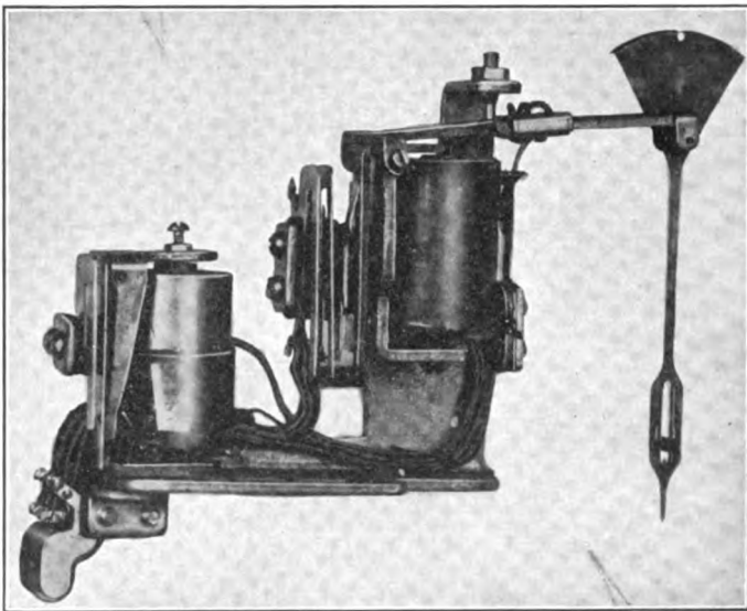
FIG. 52.—Two-spool Keith line switch.
