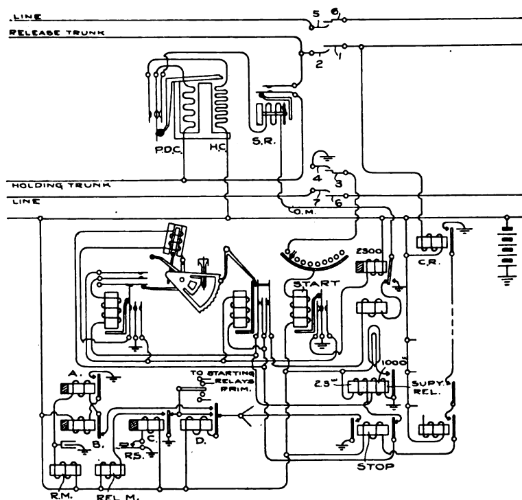
FIG. 61.—Circuit of chain relays and an associated master switch.
