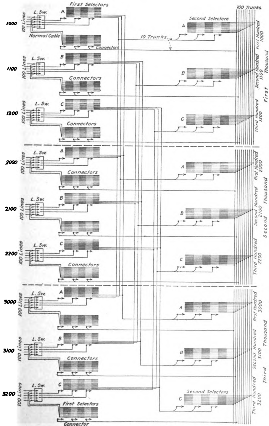
FIG. 23.—Ten-thousand-line exchange with line switches.
