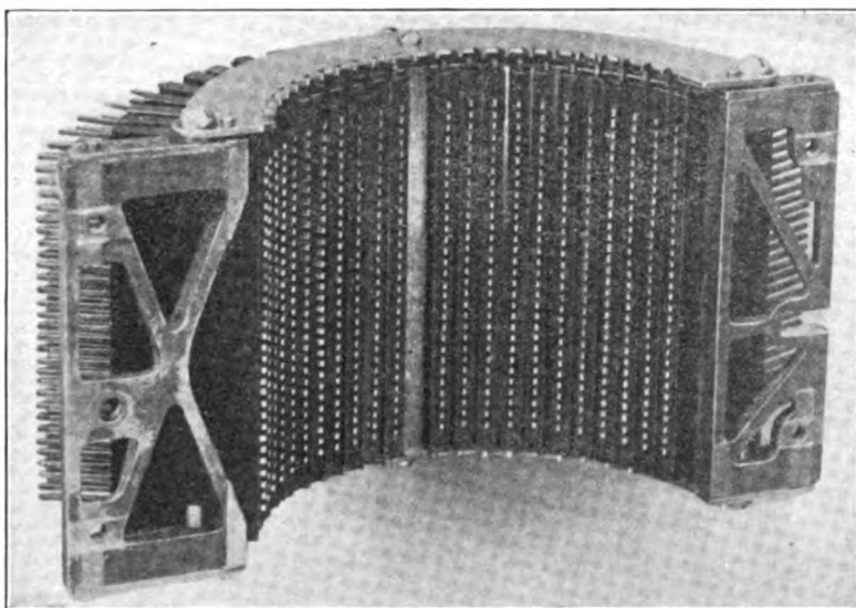
FIG. 202.—Switch bank.
