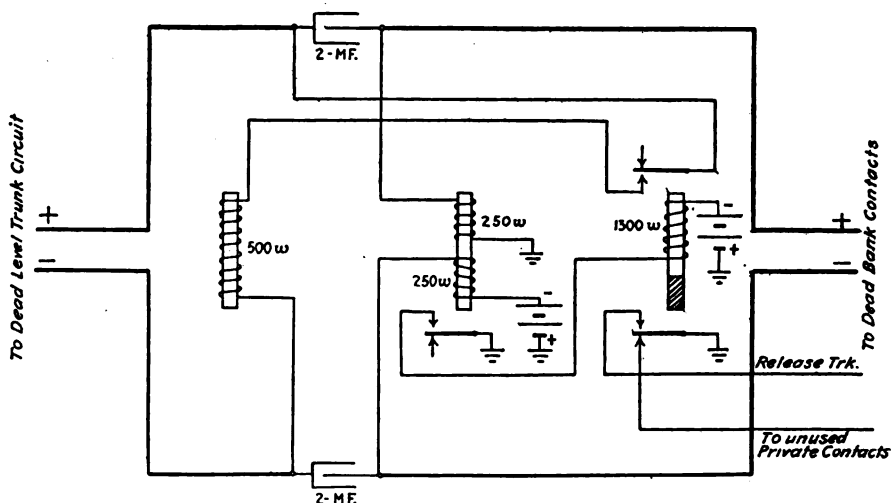
FIG. 257.—Repeater for use on a trunk circuit for connecting dead selector bank levels or pairs of contacts in a district station to an operator's position in the district station's main office.
