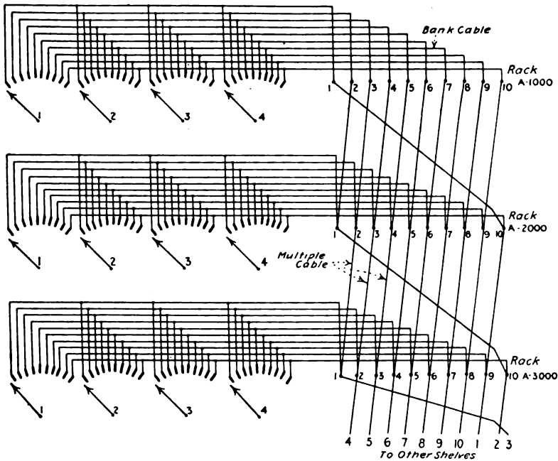
FIG. 14.—Bank slip in multiple cable.
