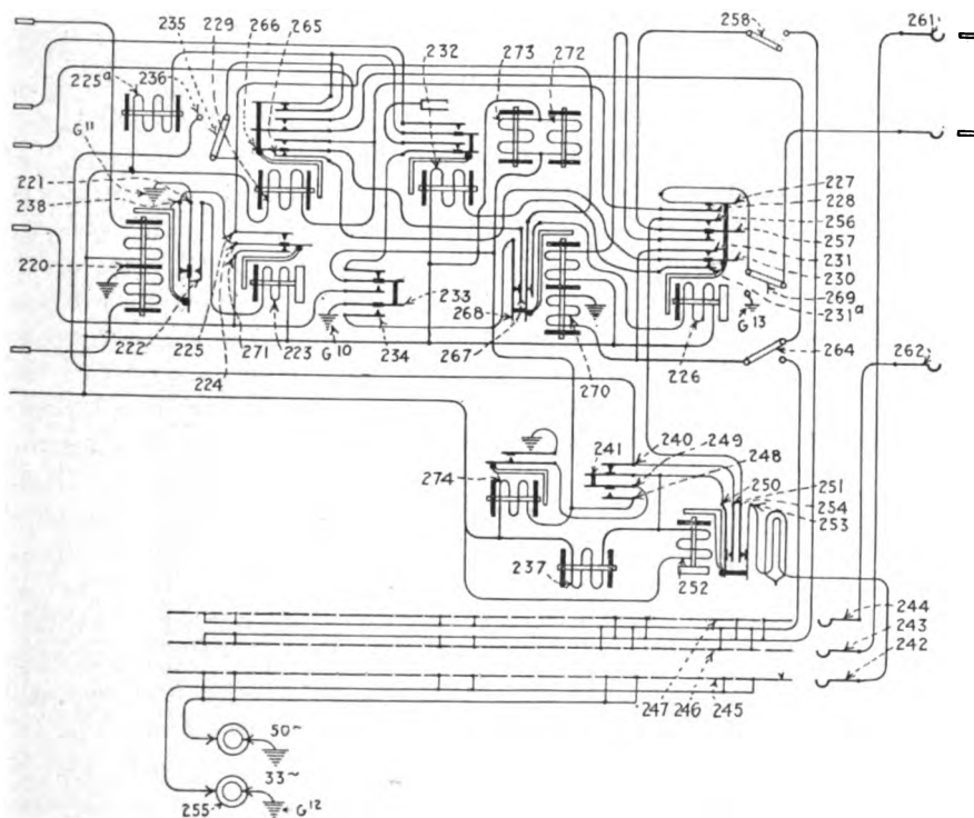
FIG. 96.—Party line connector and frequency selector circuit.
