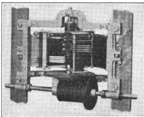
FIG. 198.—Finder switch.
