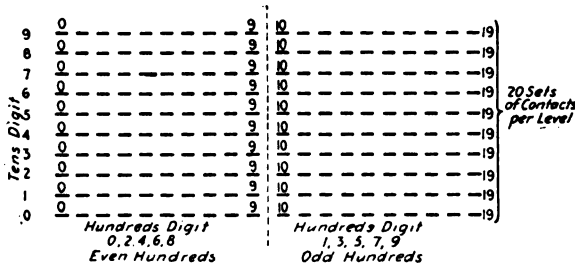
FIG. 207.—Numbering of switch bank.
