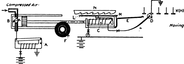
FIG. 155.—Christensen pneumatic selector moving.
