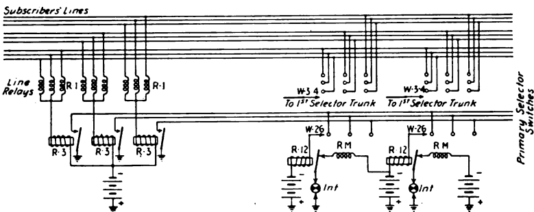
FIG. 180.—Identifying the calling line.
