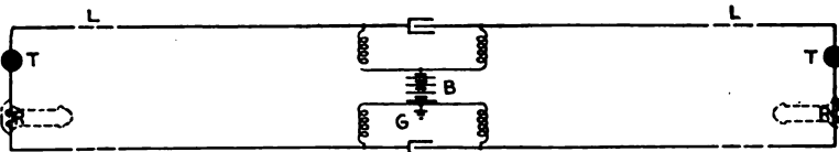
FIG. 51.—Talking circuit of single office connection.
