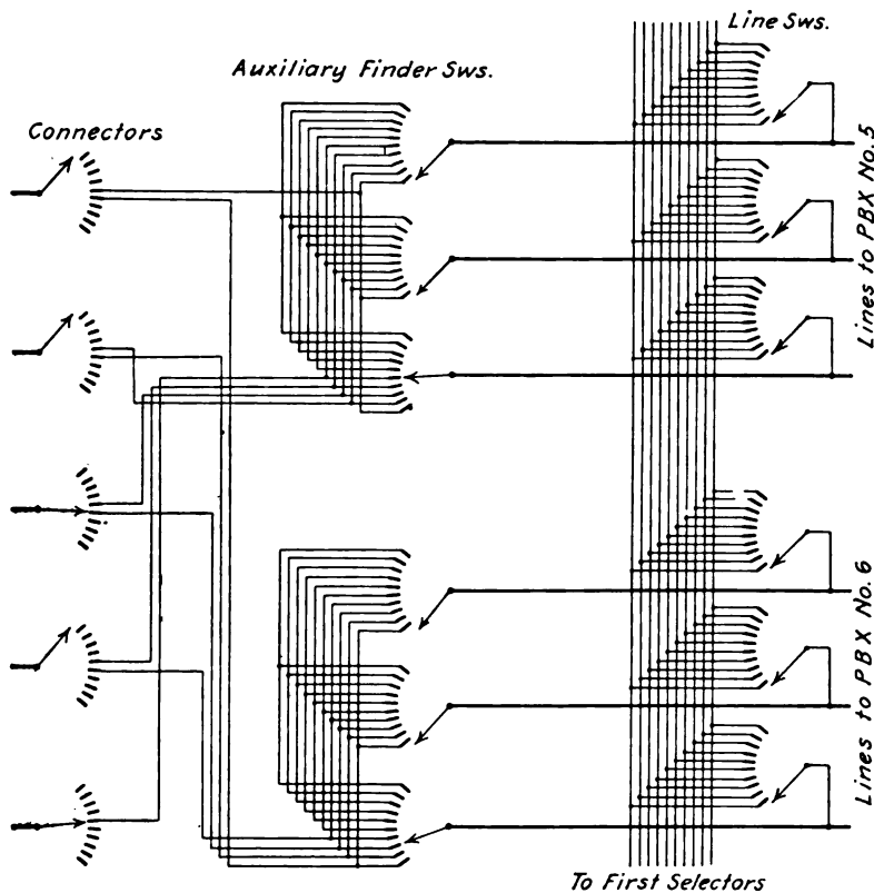
FIG. 115.—Trunking through auxiliary finders to private branch exchanges.
