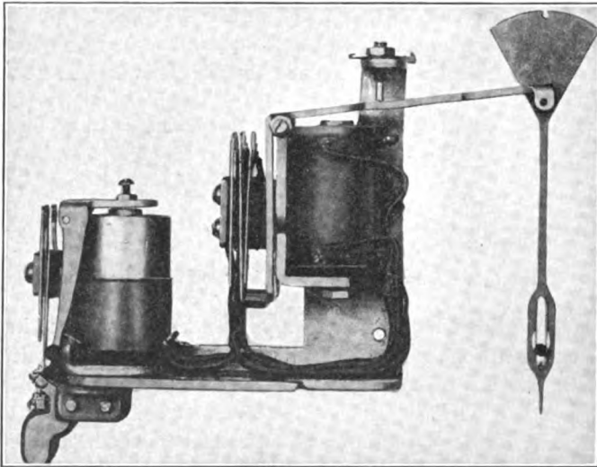
FIG. 57.—Secondary line switch.
