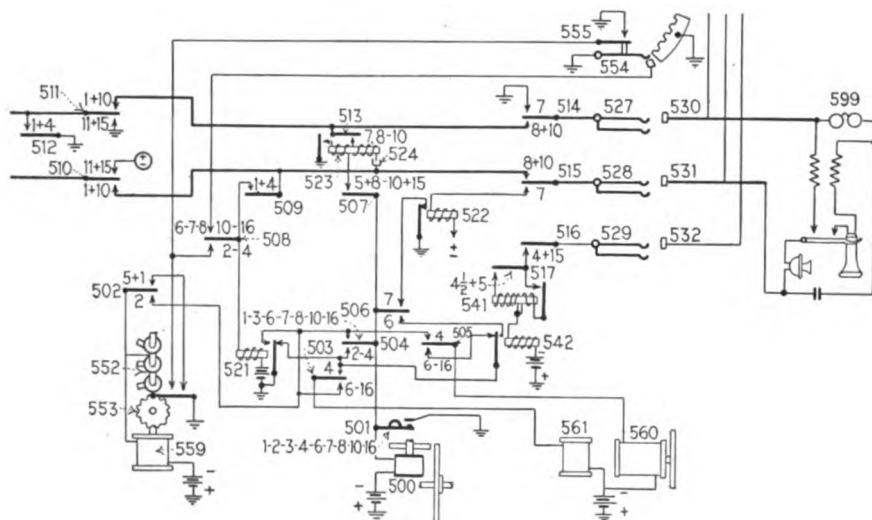
FIG. 214.—Connector circuit.
