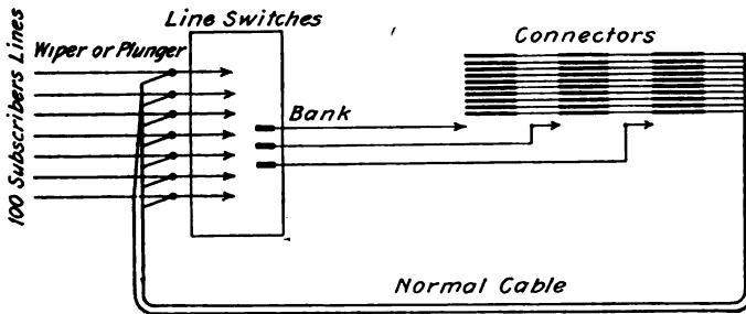
FIG. 21.—One-hundred-line system with line switches.
