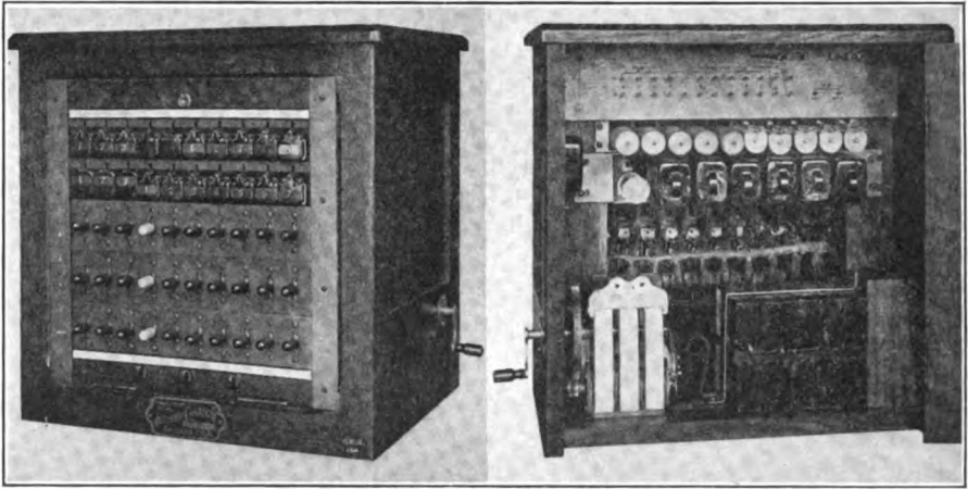
FIG. 70.—Cordless private branch switchboard.
