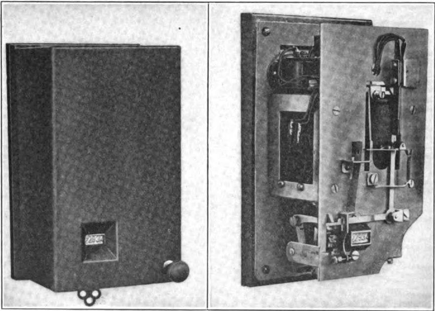
FIG. 82.—A subscriber's station meter.
