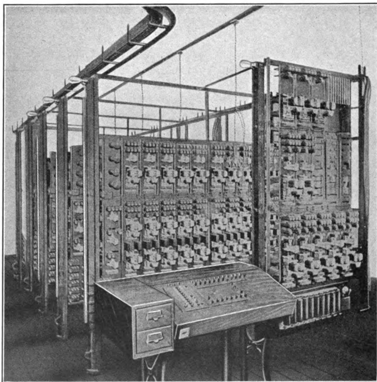
FIG. 188.—500-line installation.
