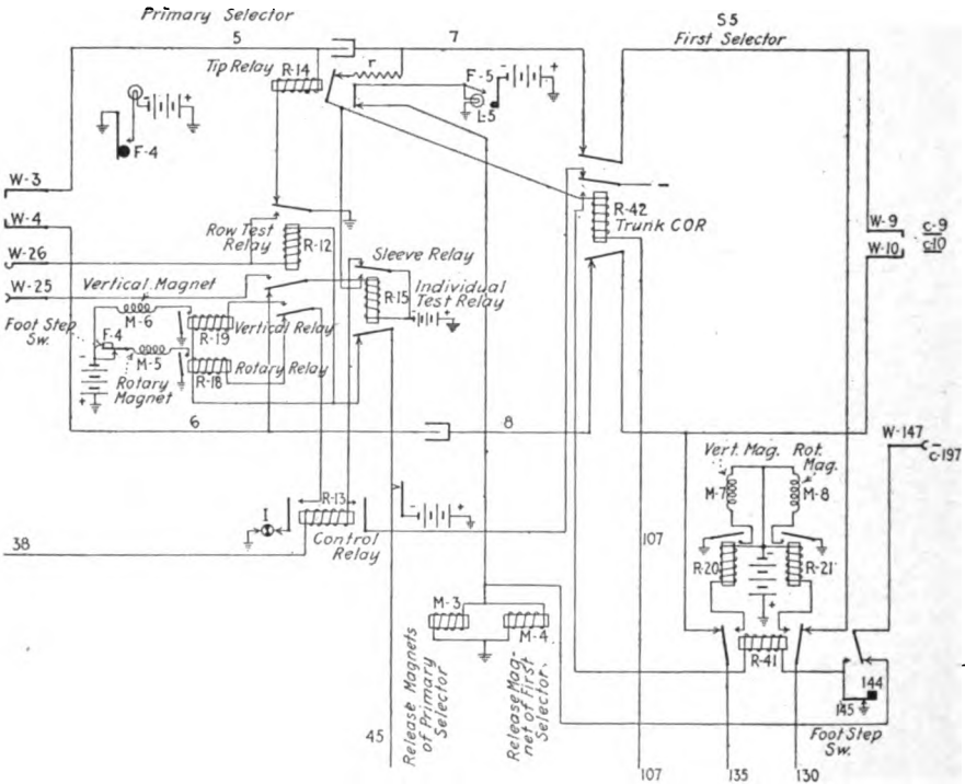
FIG. 178.—Primary and first selector circuits.
