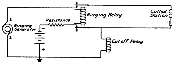
FIG. 184.—Ringing conditions.
