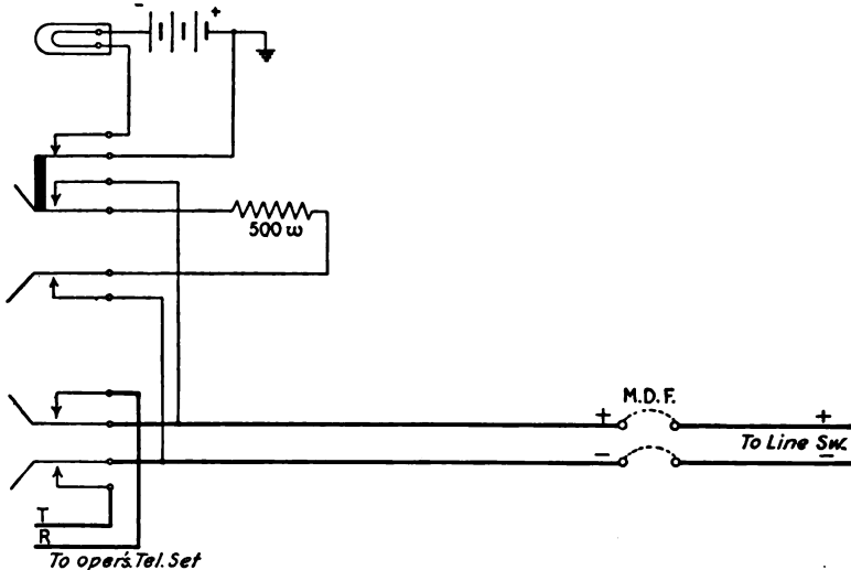
FIG. 259.—Outgoing trunk circuit from an information or complaint operator's position to an automatic switchboard.
