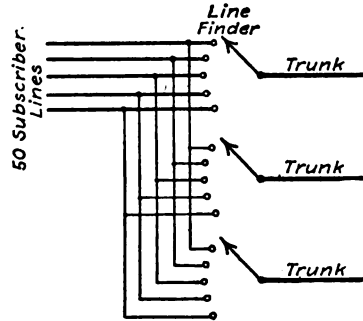
FIG. 25.—Principle of line finder.
