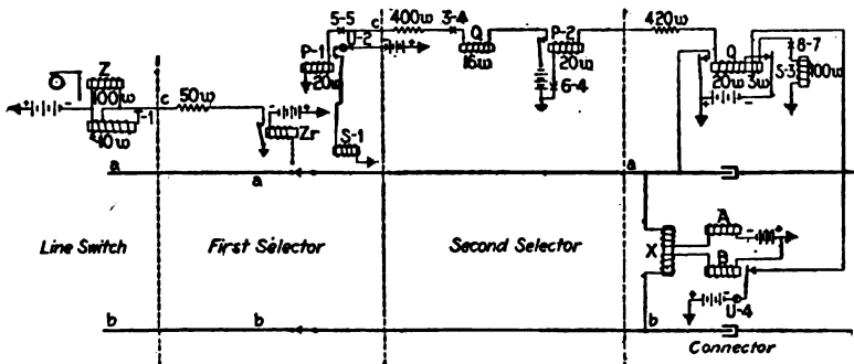
FIG. 112.—Operation of service meter.
