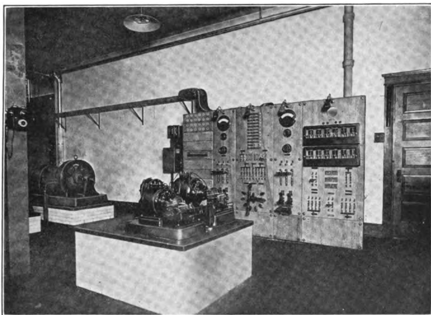
FIG. 240.—View of power plant.
