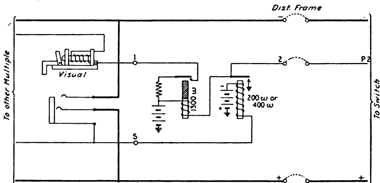
FIG. 233.—Toll-board end of a service trunk to a local automatic switchboard.
