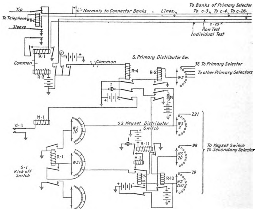
FIG. 176.—Subscriber's line and distributor circuits.
