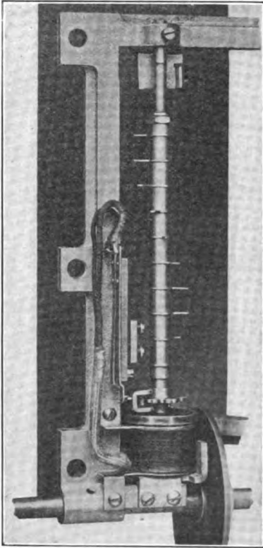
FIG. 205.—Tripping spindle.
