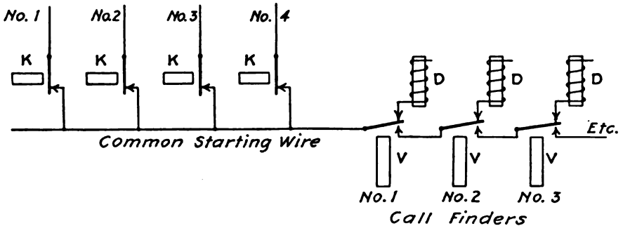
FIG. 124.—Method of seizing an idle call finder.
