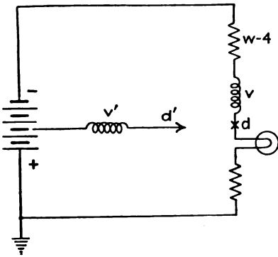
FIG. 121.—Conditions of busy test for finding a free operator.
