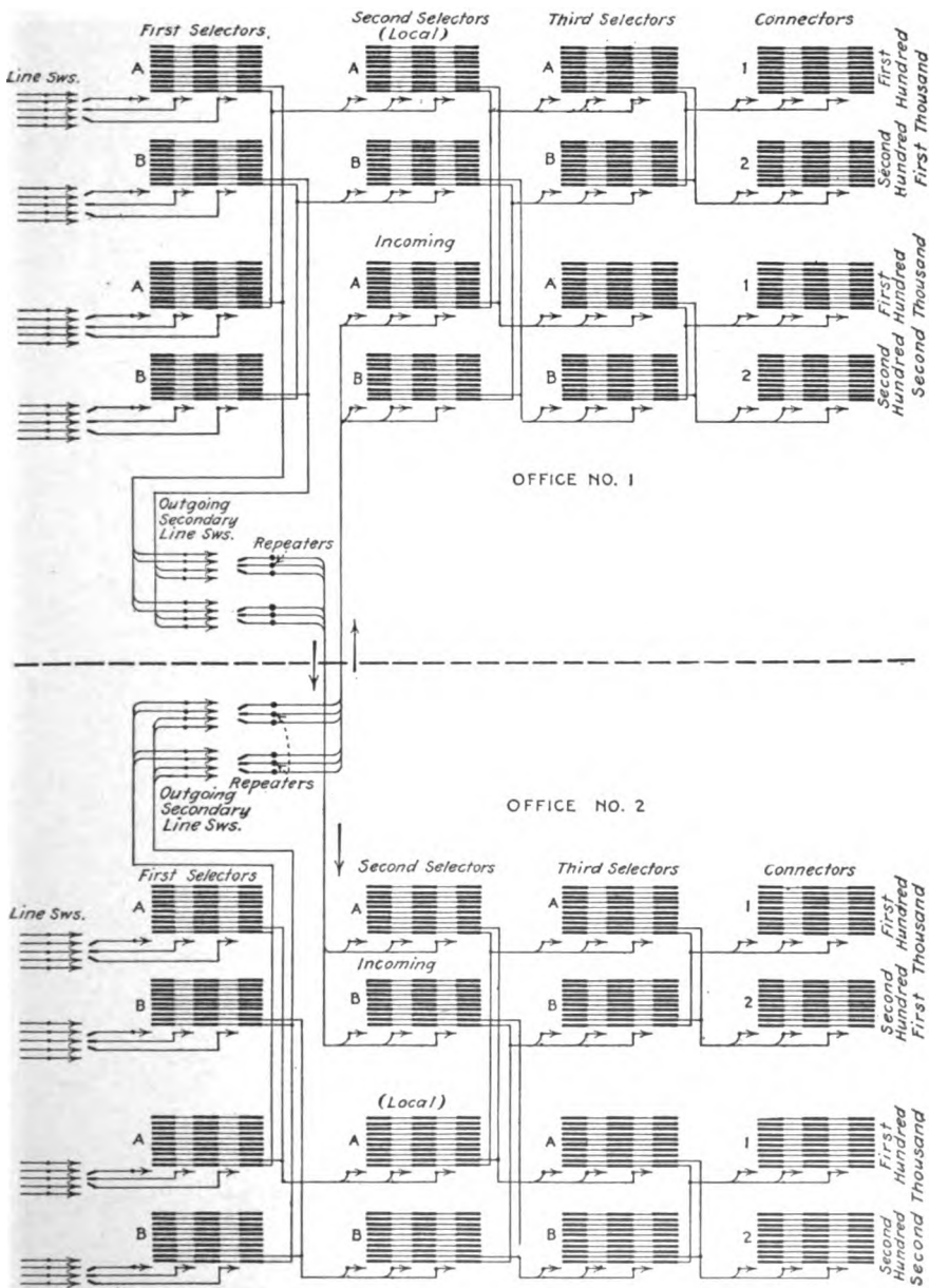
FIG. 27.—Inter-office trunking (100,000-line system).
