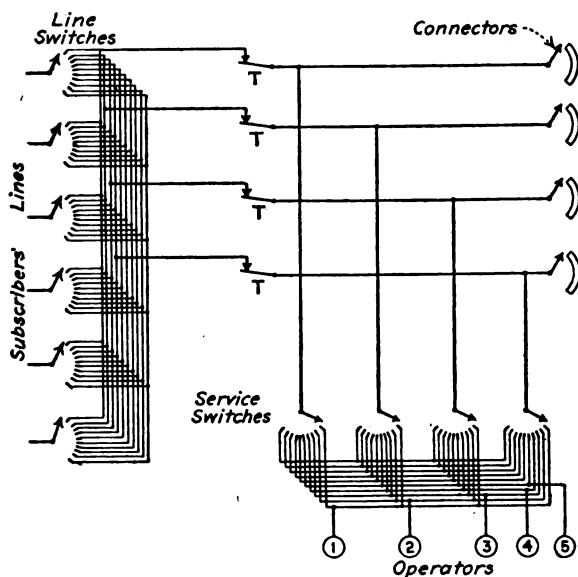
FIG. 119.—Trunking in semi-automatic system with service switches.
