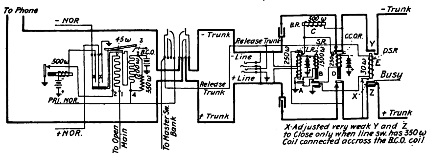
FIG. 74.—Discriminating outgoing trunk circuit.
