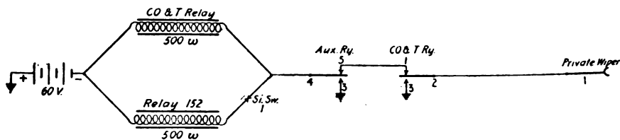
FIG. 171.—Testing circuit.
