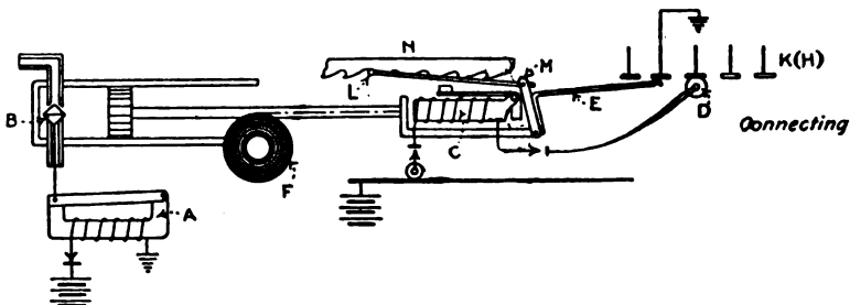
FIG. 157.—Christensen pneumatic selector "connecting."
