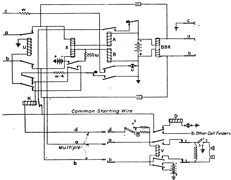
FIG. 123.—Call-finder circuit.
