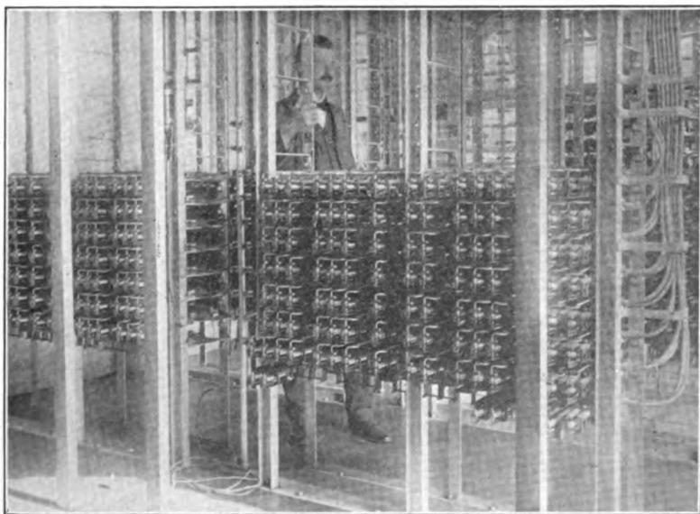
FIG. 154.—Racks with Christensen pneumatic selectors mounted upon them.
