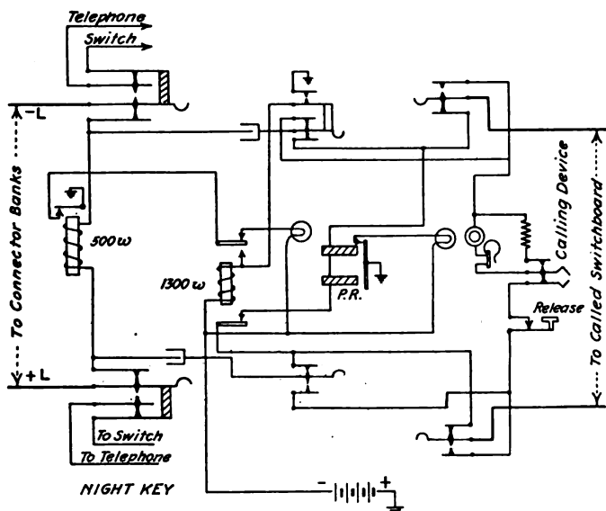
FIG. 76.—Circuit through an automatic P.B.X. attendant's cabinet (secret).
