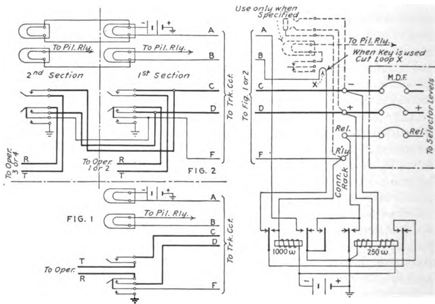
FIG. 252.—Trunk incoming to an information operator's position from selector switch banks.
