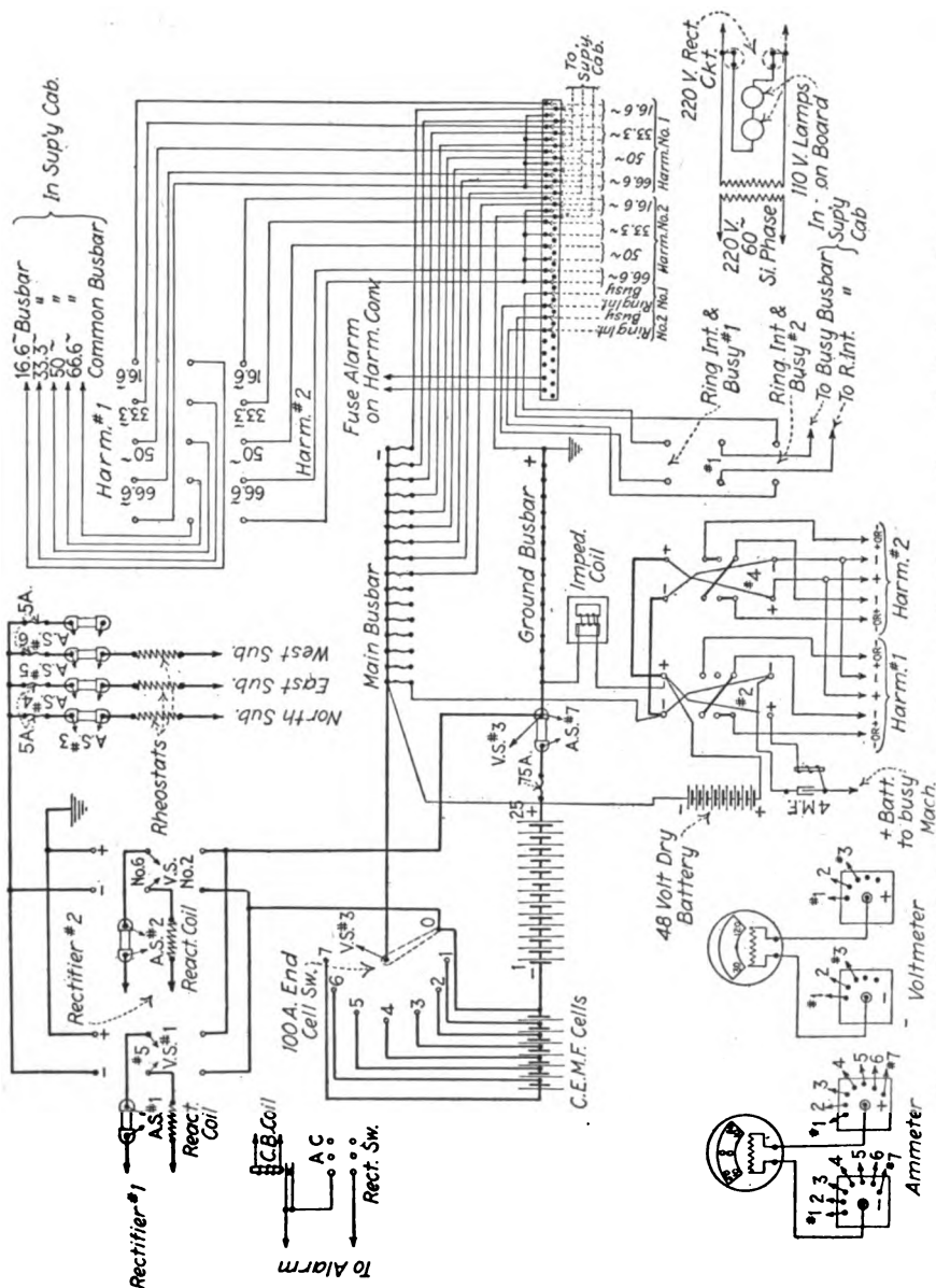
FIG. 243.—Typical circuit diagram of power plant for an office with district stations.
