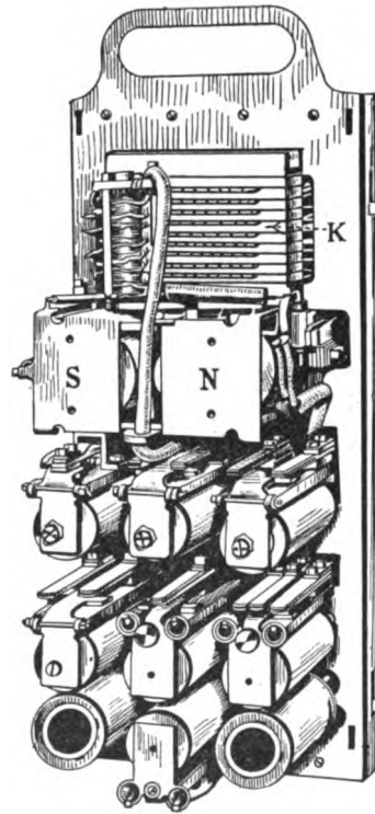
FIG. 104.—Relay assembly.
