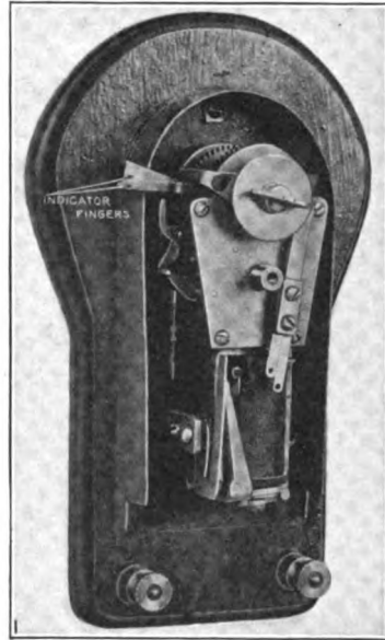
FIG. 248.—Calling device speed indicator.
