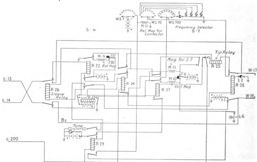
FIG. 183.—Connector circuit.
