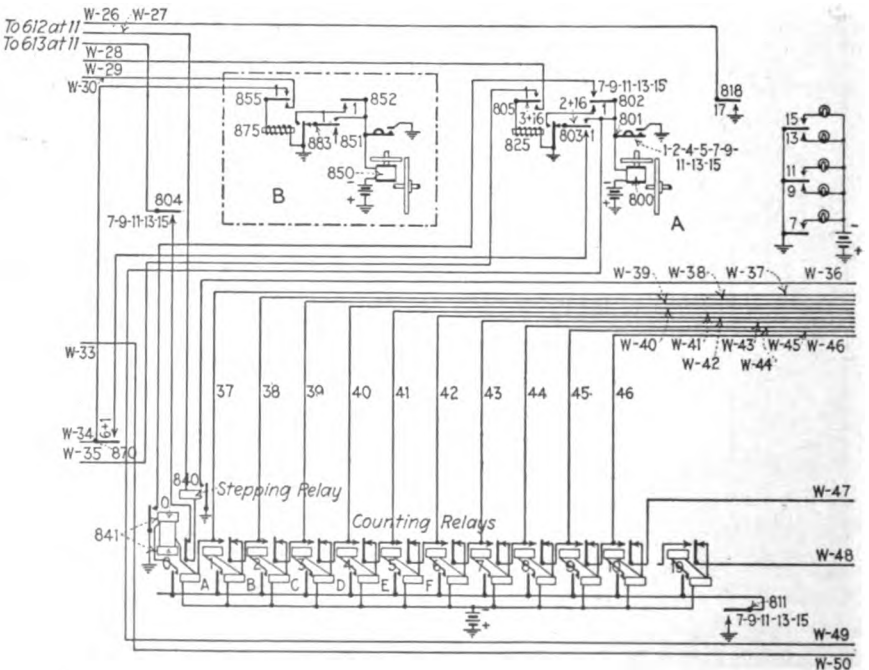
FIG. 217.—Counting relay circuit.
