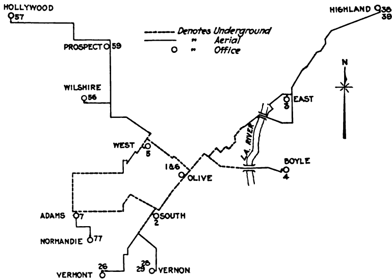
FIG. 265.—Skeleton diagram of the automatic telephone system of Los Angeles, Cal.
