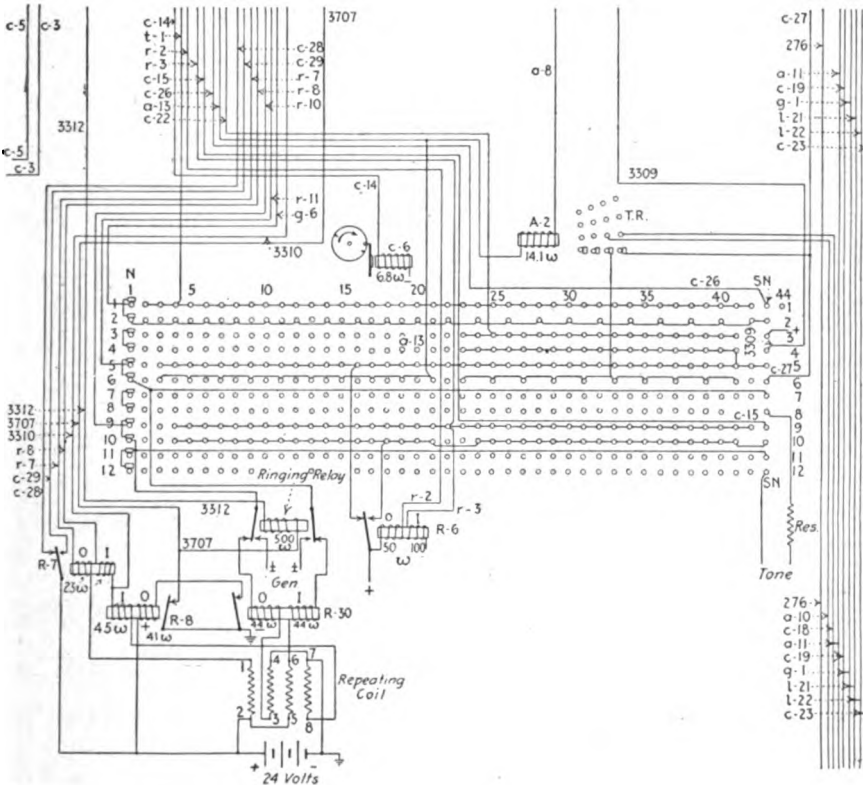
FIG. 144.—Signal transmitter controller circuit.
