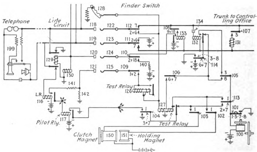
FIG. 210.—Line and primary finder circuit.
