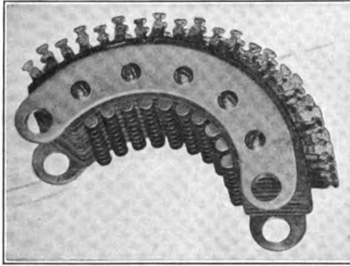
FIG. 46.—Connector-switch bank, unwired.
