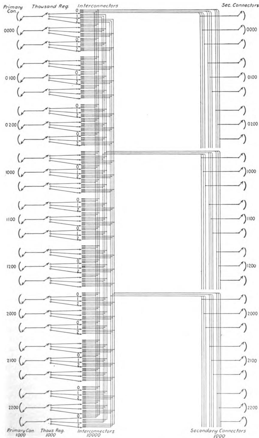
FIG. 135.—10,000-line trunking system.
