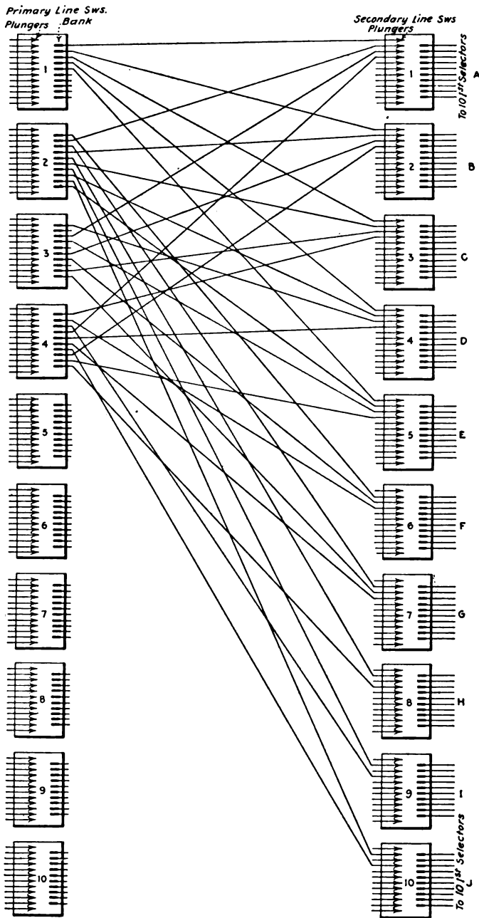
FIG. 24.—Primary and secondary trunking (distributive.)
