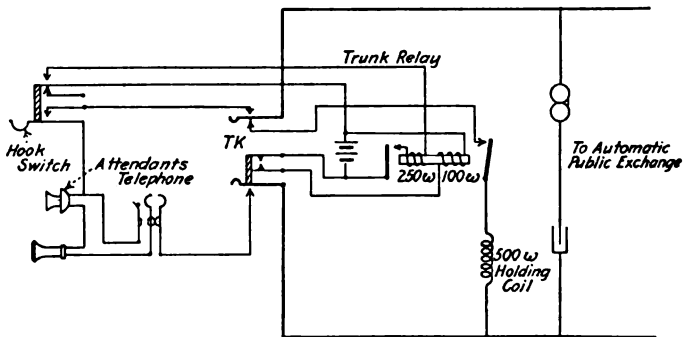
FIG. 69.—Trunk circuit to attendant's station of a push key inter-communicating system.
