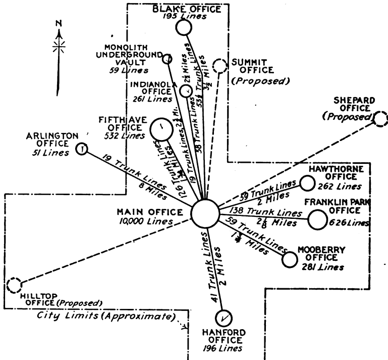
FIG. 266.—Skeleton diagram of automatic telephone system of one main central office surrounded by district stations in Columbus, O.
