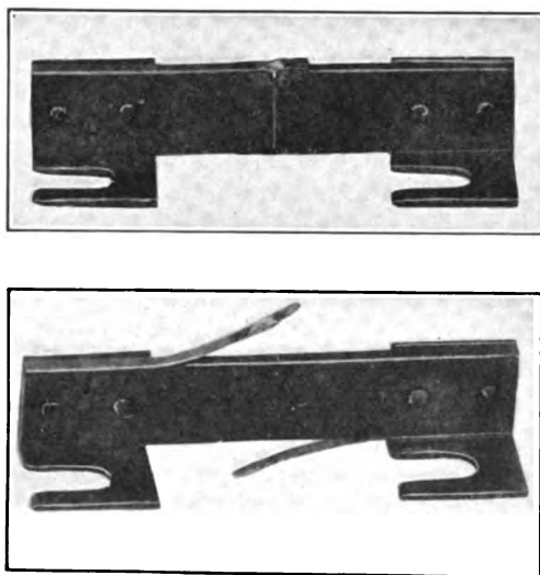
FIG. 247.—Above, tell-tale fuse set. Below, tell-tale fuse operated.
