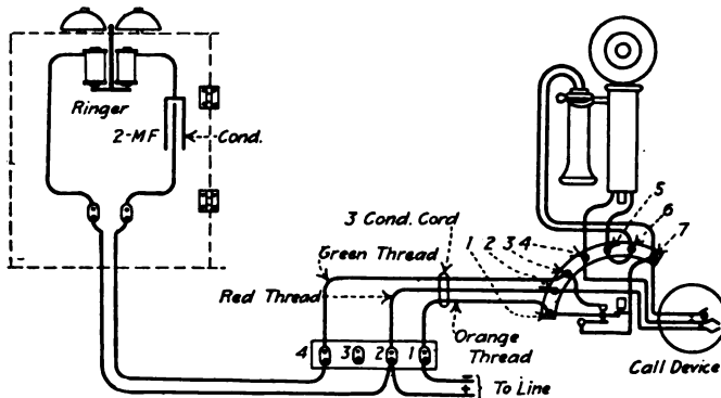
FIG. 65.—Desk telephone wiring diagram.
