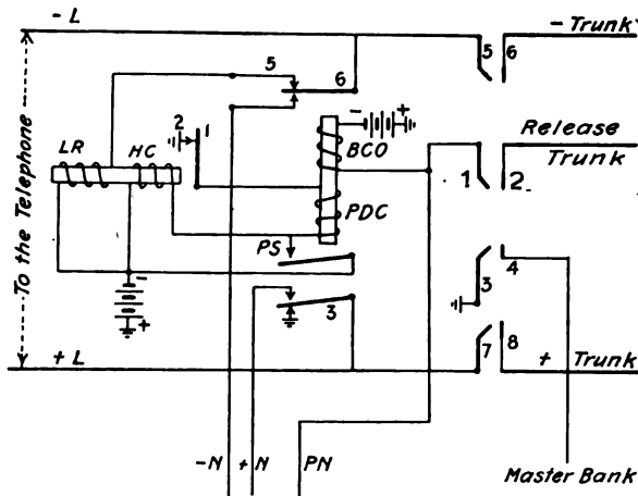
FIG. 39.—Circuit of two-spool Keith line switch.
