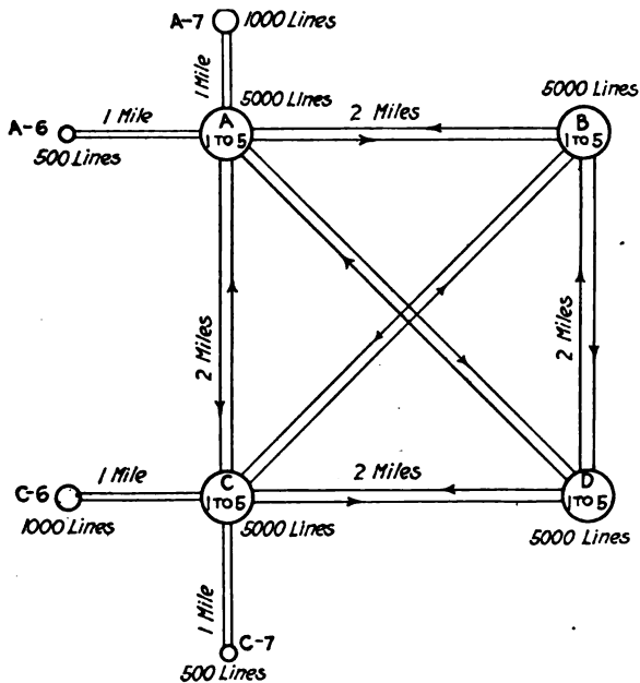
FIG. 270.—Diagram representing hypothetical system of 4 main offices A, B, C, and D and 4 subsidiary offices, A-6, A-7, C-6, and C-7.
