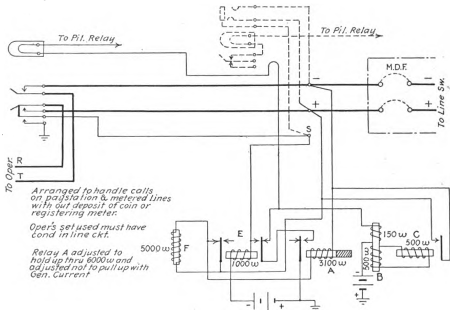
FIG. 254.—Dead number trunk circuit for use in an exchange having metered lines or sub-station coin collectors actuated by "reversing battery" connector switches.
