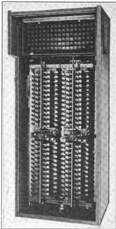
FIG. 78.—Line switch unit with meters at top.
