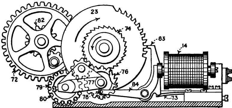
FIG. 134.—Clutch and magnet.
