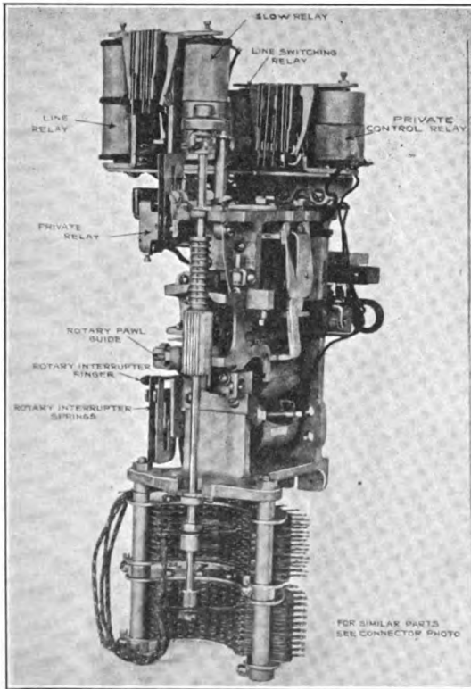
FIG. 54.—Two-wire selector switch.
