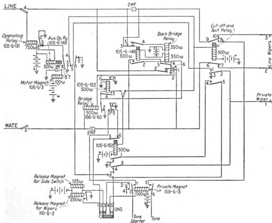
FIG. 170.—Connector circuit at district station.
