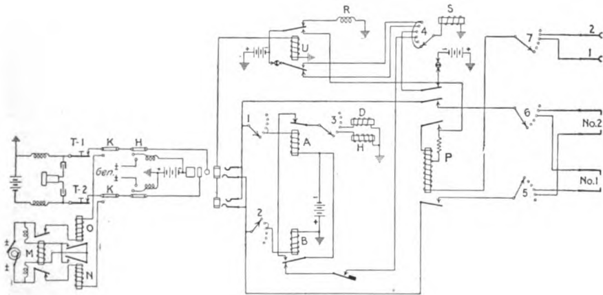
FIG. 113.—Toll selector circuit.
