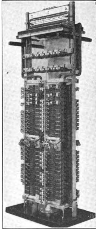
FIG. 58.—Secondary line-switch unit.
