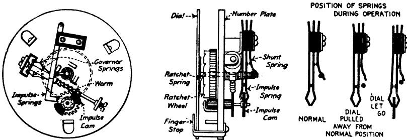
FIG. 32.—Details of calling device.
