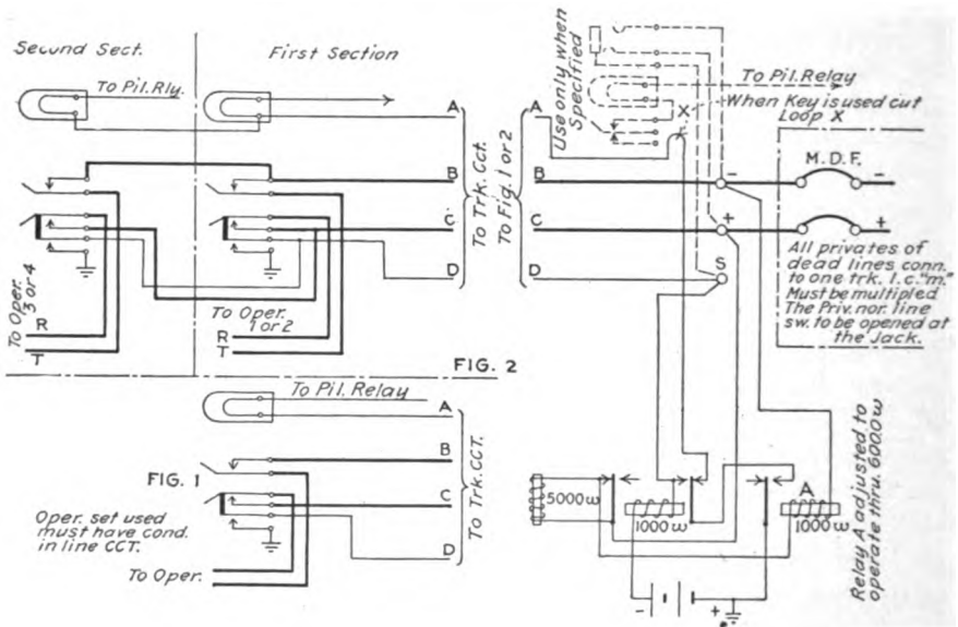
FIG. 253.—Trunk for connecting dead lines or numbers to an information operator's position.
