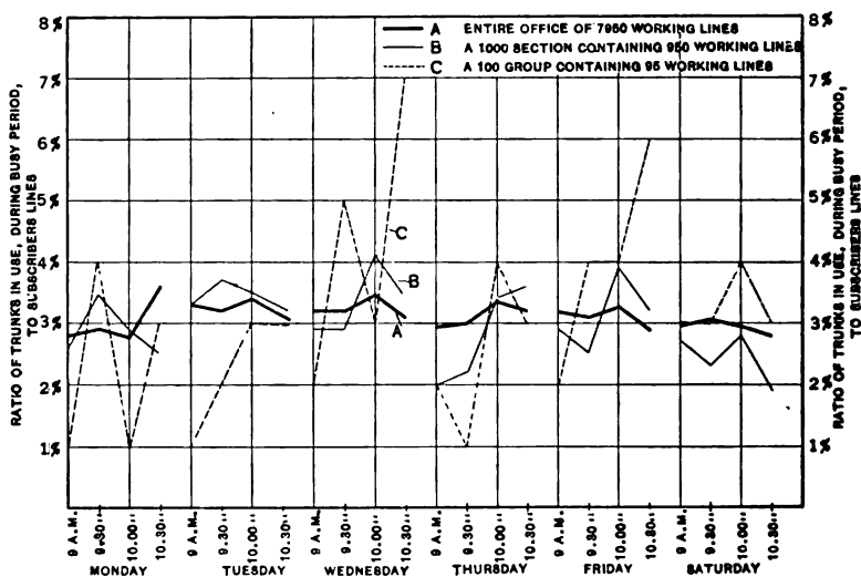
FIG. 261.—Curves showing ratios of trunks in use to subscribers' lines during the busy hour of each day of a week.
