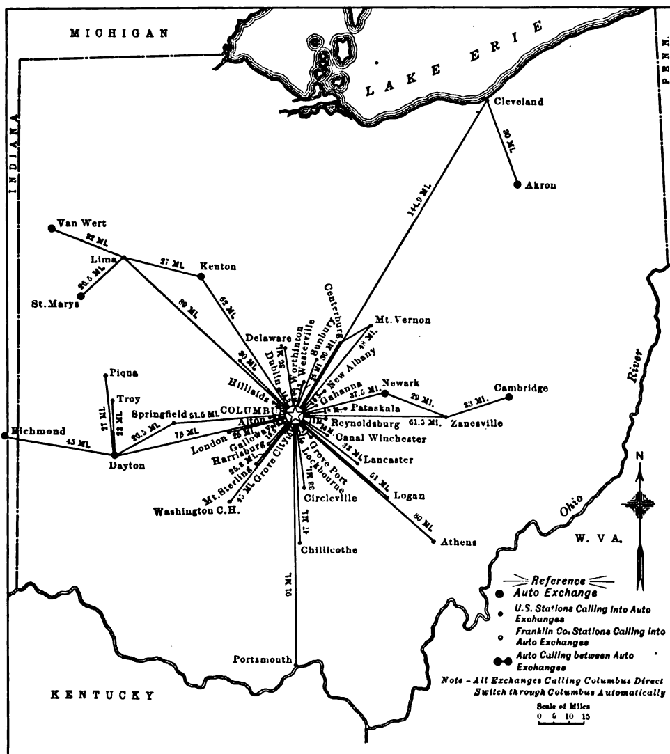
FIG. 237.—Map showing long distance automatic lines centering at Columbus, Ohio.
