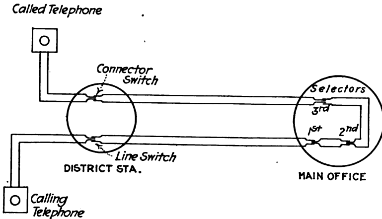
FIG. 268.—Showing switches and inter-office trunks used for a reverting district-station call.
