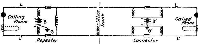
FIG. 56.—Talking circuit of an inter-office connection.
