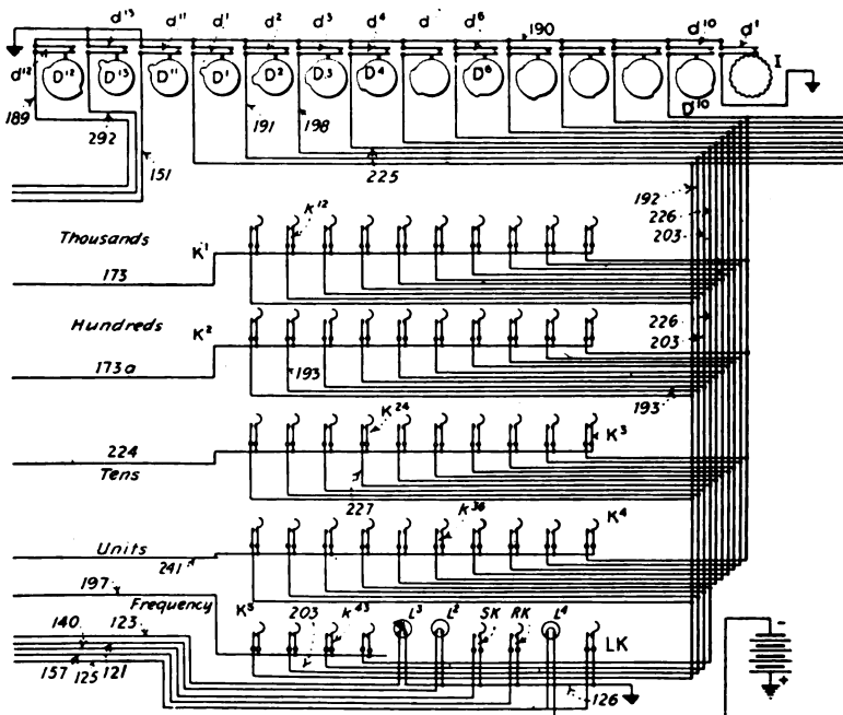
FIG. 181.—Sending machine and keyset circuit.
