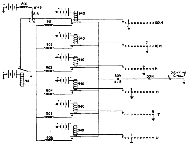
FIG. 222.—Principle of setting registers from keyboard.
