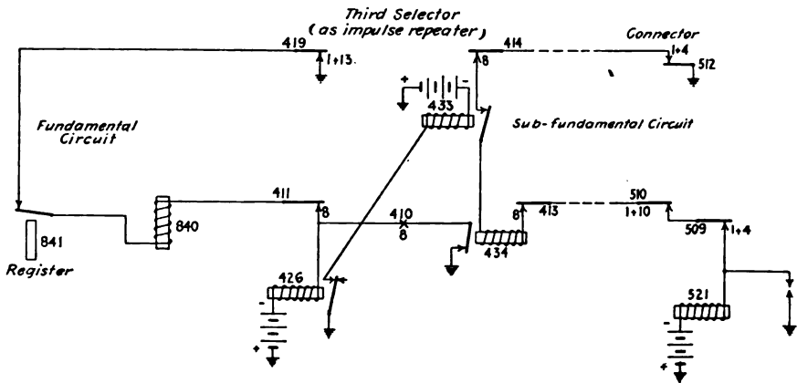
FIG. 227.—Principle of impulse repeater.
