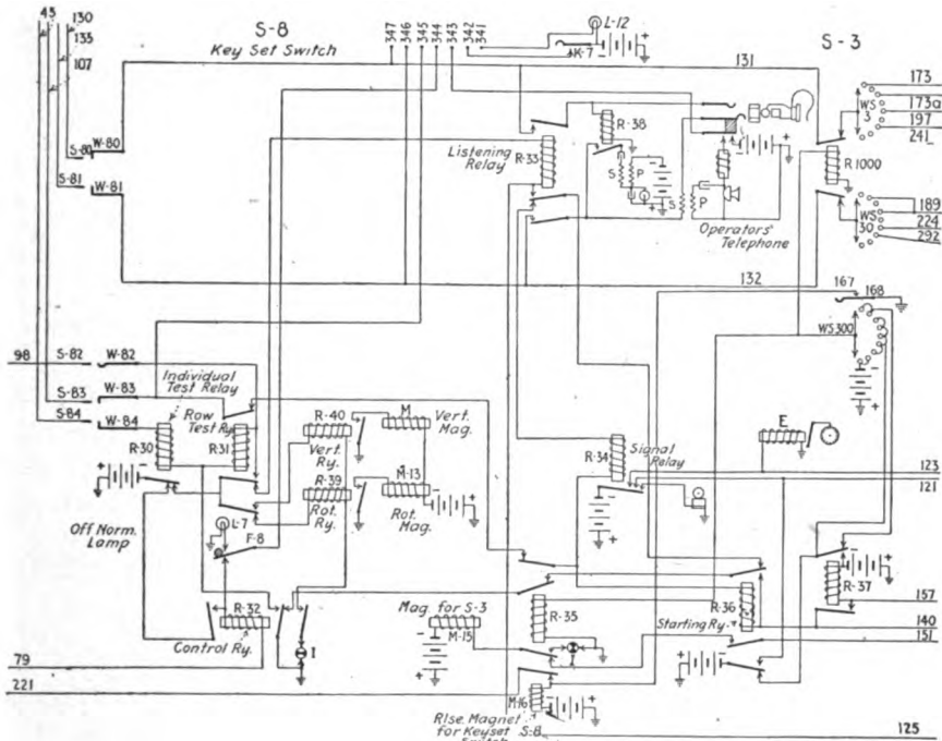
FIG. 179.—Operator's keyset switch circuit.
