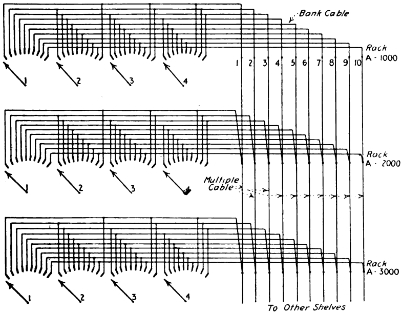
FIG. 13.—Bank slip in bank cable.
