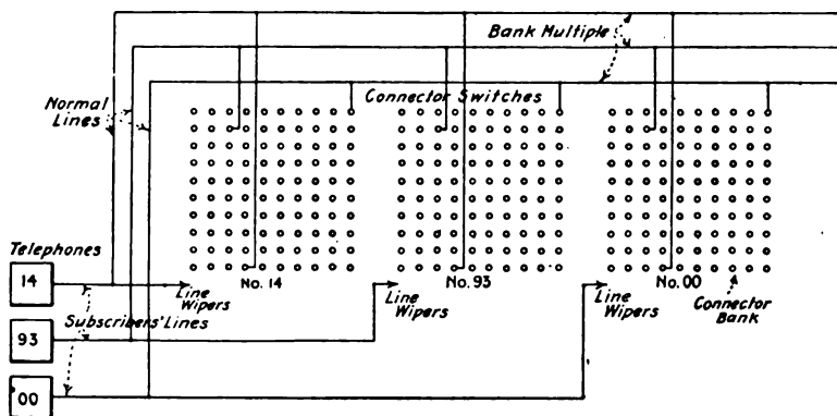
FIG. 5.—Theory of 100-line exchange.
