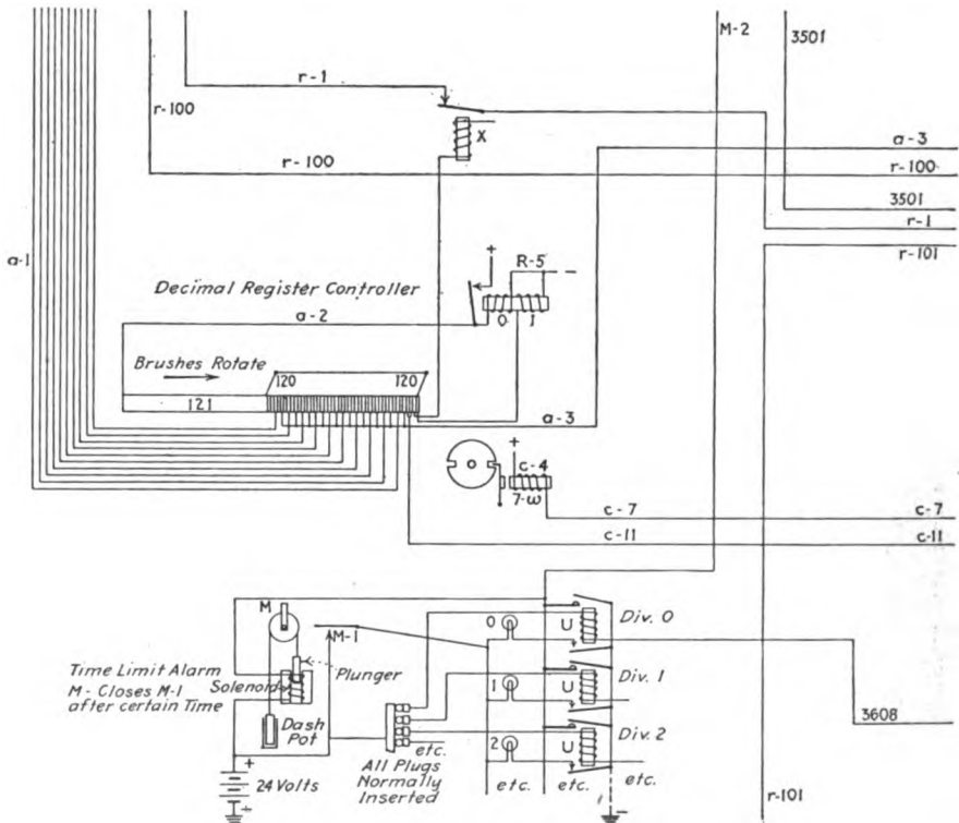
FIG. 140.—Decimal register controller circuit.
