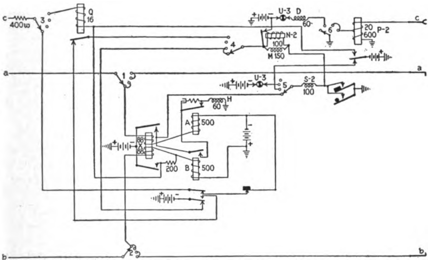
FIG. 110.—Second selector circuit.
