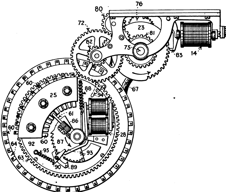
FIG. 133.—Driving gear for cylinder switch.
