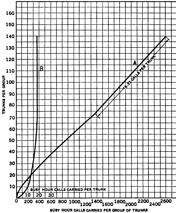
FIG. 262.—Curve A shows call-carrying capacities of trunk groups of various sizes, manual central offices; average trunk holding time of 120 seconds. Curve B shows call-carrying capacity of each trunk in groups of various sizes.
