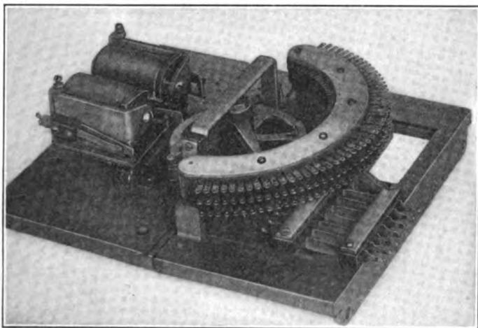
FIG. 90.—Switch bank and wipers.
