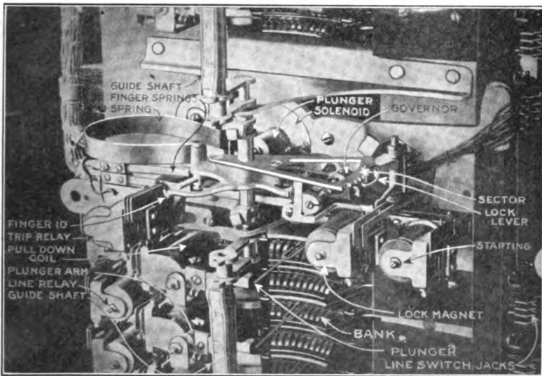
FIG. 38.—Master switch mounted on shelf of Keith line-switch unit.
