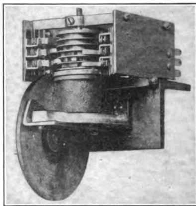
FIG. 197.—Number register (full automatic).
