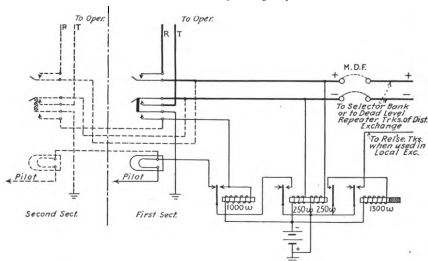
FIG. 256.—Trunk for connecting dead levels or pairs of selector bank contacts to an operator's position.
