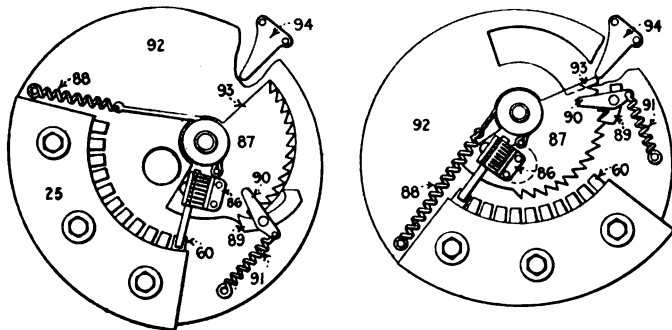
FIG. 131.—Register switch.
