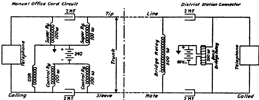
FIG. 173.—Talking circuit between subscribers. (Manual office to district station.)
