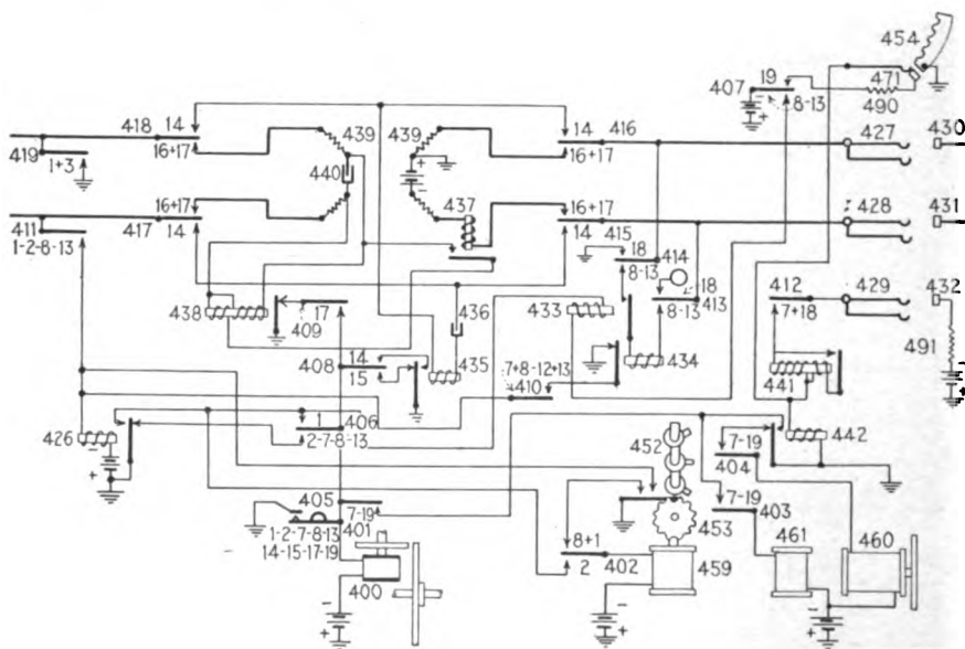
FIG. 213.—Third selector circuit.
