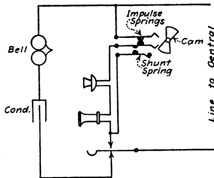
FIG. 33.—Automatic telephone circuit.
