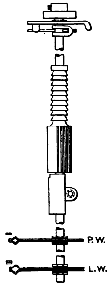
FIG. 43.—Switch shaft and wipers.
