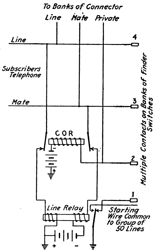
FIG. 166.—Subscriber's line circuit.
