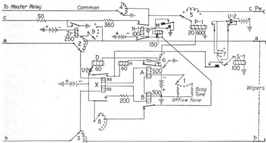
FIG. 109.—First selector circuit.
