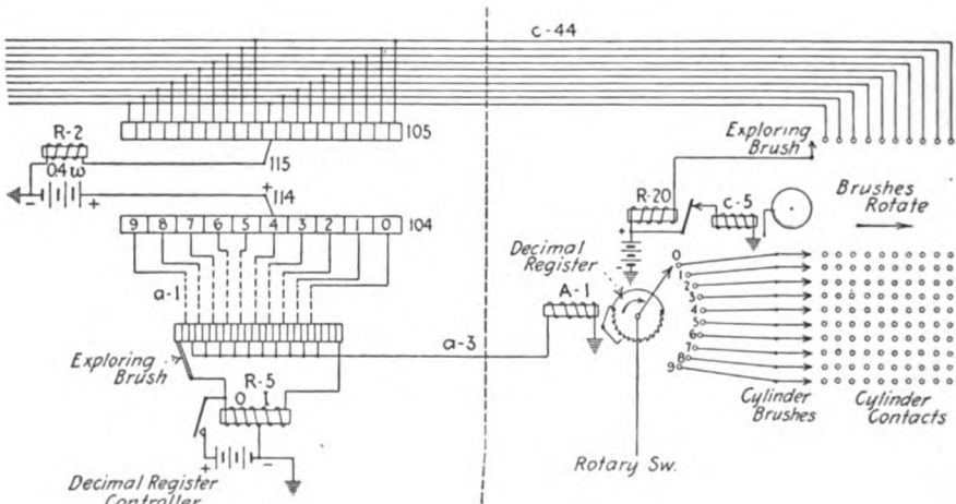
FIG. 147.—Finding the calling line.
