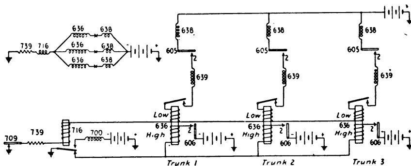
FIG. 221.—Elimination of simultaneous calls.
