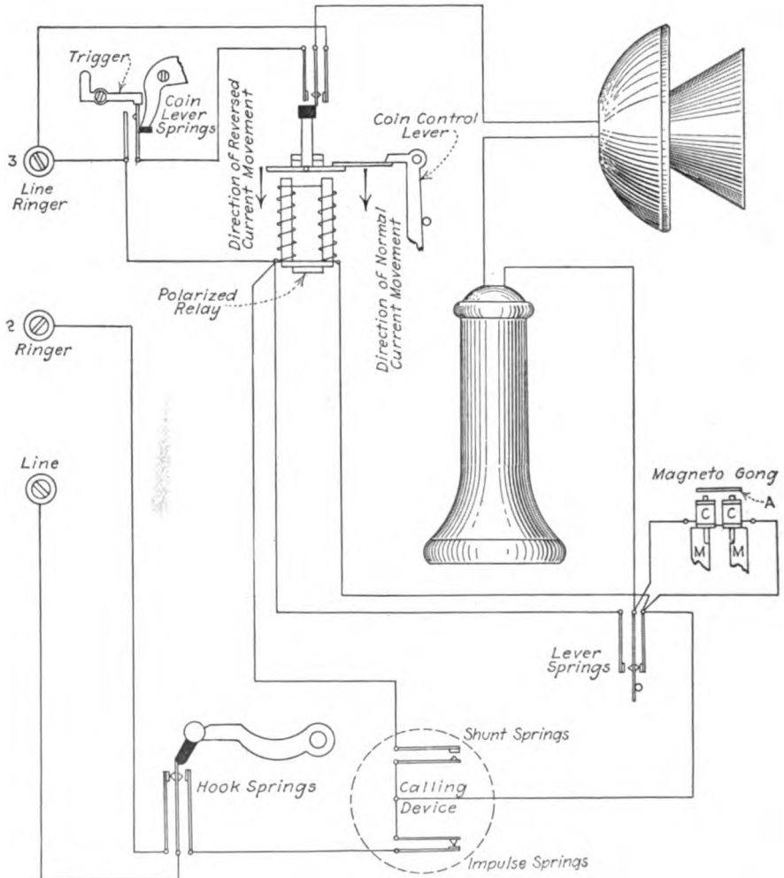
FIG. 84.—Circuit of combination telephone and collector shown in Fig. 83.
