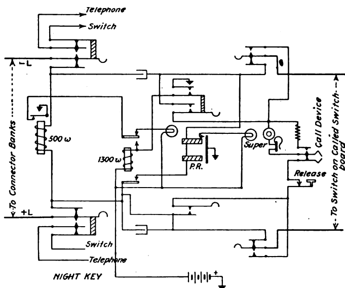
FIG. 75.—Circuit through an automatic P.B.X. attendant's cabinet (non-secret).
