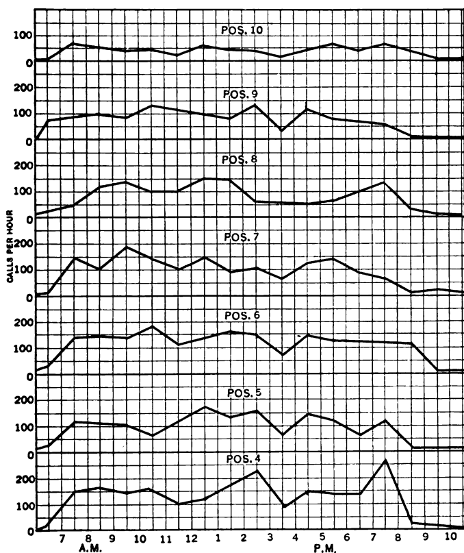
FIG. 151.—Simultaneous load curves of manual switchboard operators' positions.
