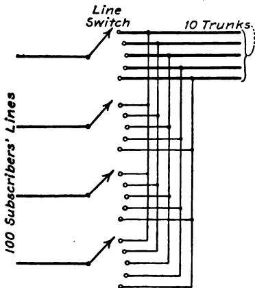
FIG. 18.—Principle of rotary line switch.
