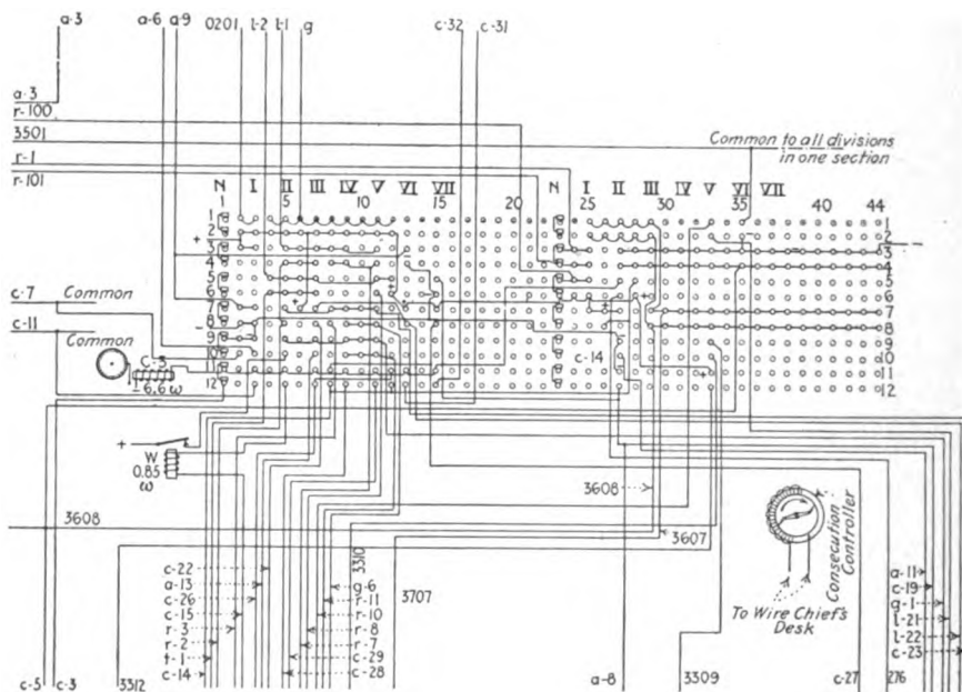
FIG. 143.—Rotary switch circuit.
