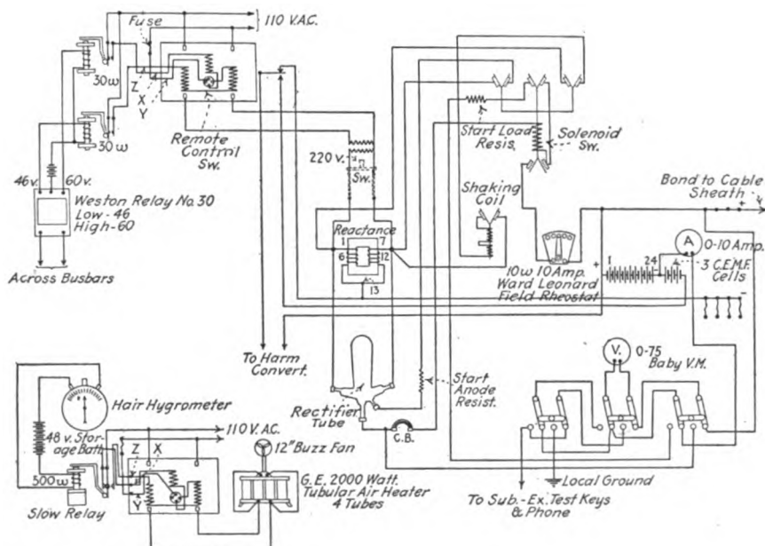
FIG. 245.—Circuit of district station power plant arranged for remote control of charging apparatus and automatic control of heating apparatus.
