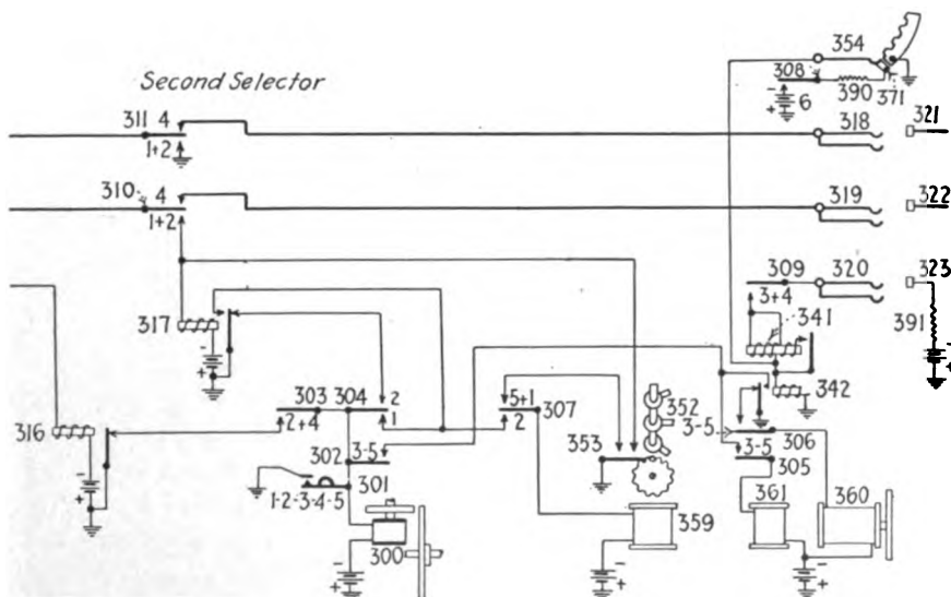
FIG. 212.—Second selector circuit.
