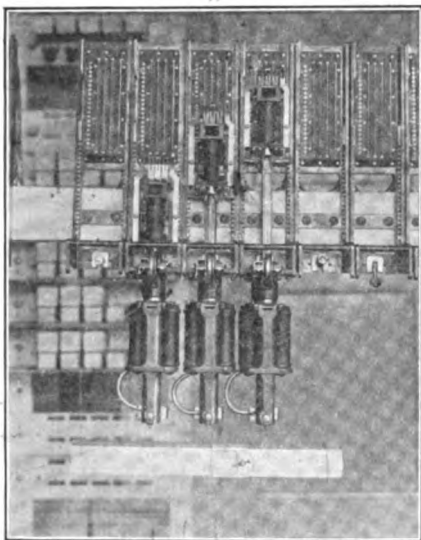
FIG. 152.—View from below of three Christensen pneumatic selectors.
