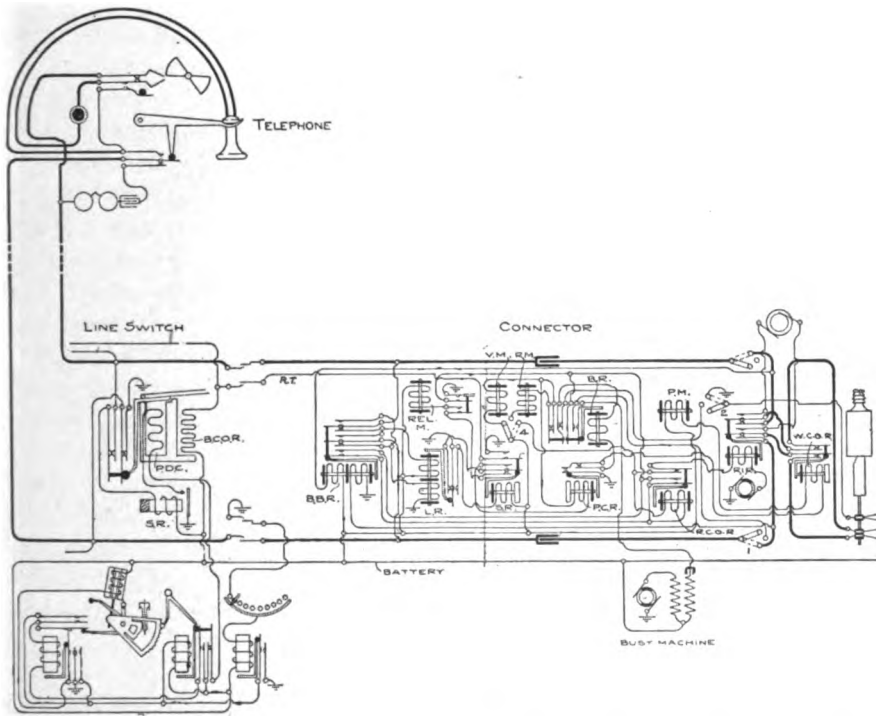
FIG. 53.—Circuits of a two-spool Keith line switch and a corresponding connector switch.
