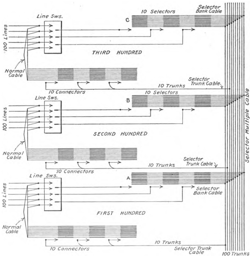
FIG. 22.—One-thousand-line system with line switches.
