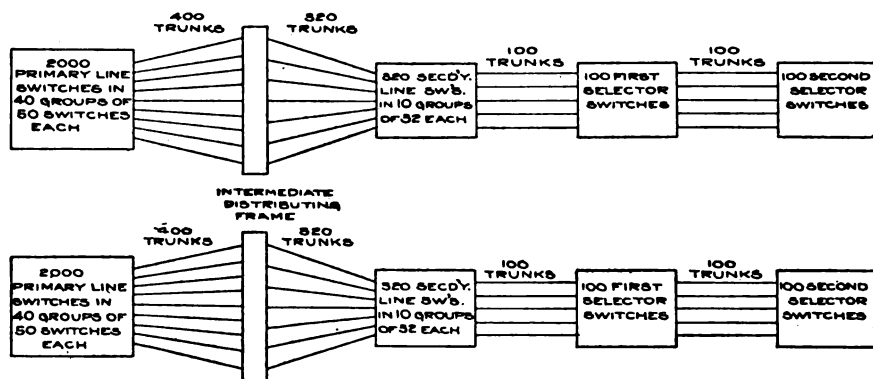
FIG. 59.—Diagram illustrating scheme of using secondary line switches to reduce first and second selectors.
