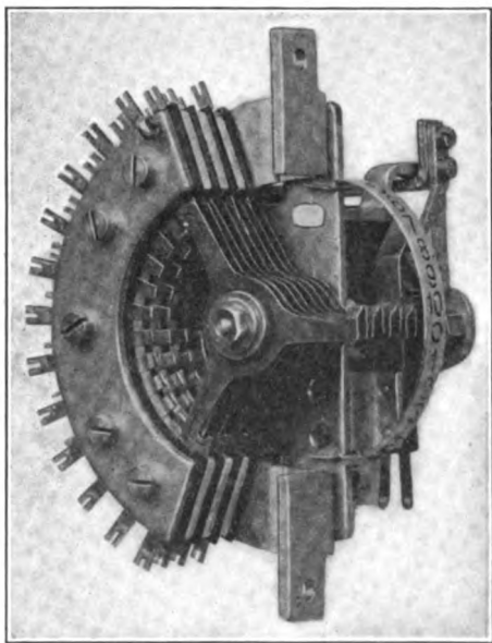
FIG. 102.—Rotary line switch.
