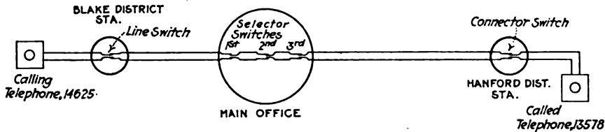
FIG. 267.—Diagram illustrating steps in setting up a connection from a subscriber connected to Blake to one connected to Hanford district station.
