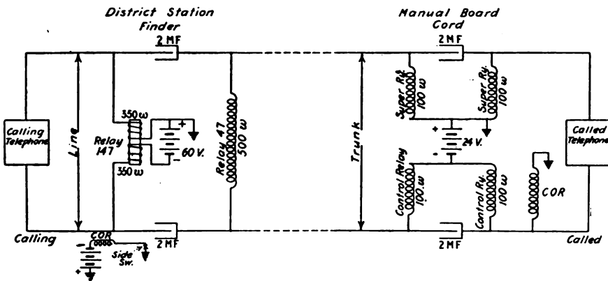
FIG. 168.—Talking circuit between telephones (district station to manual office).
