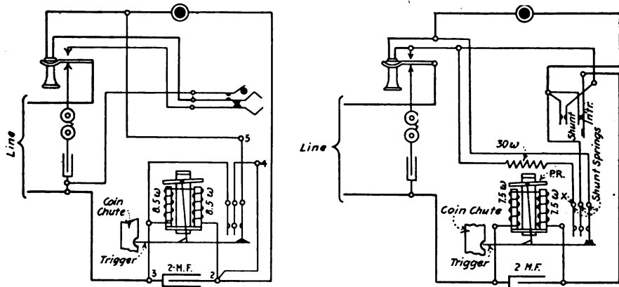
FIG. 81.—Two different circuits of a telephone with a coin collector.
