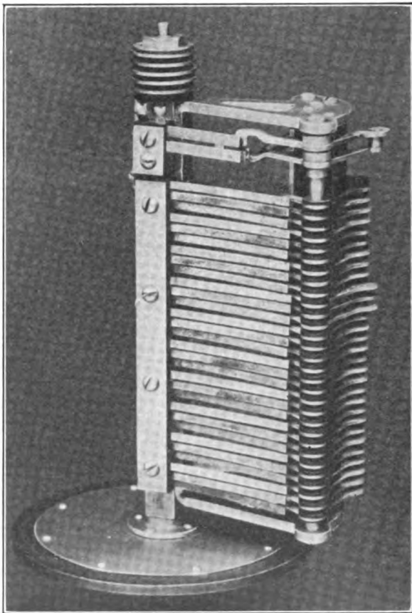
FIG. 204.—Selector brush carriage.
