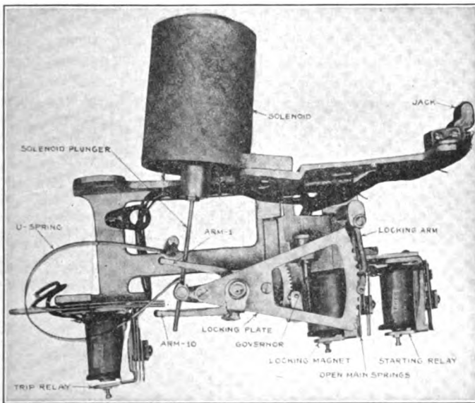
FIG. 40.—Unmounted master switch.
