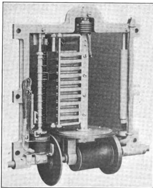
FIG. 203.—Selector brushes and mechanism.
