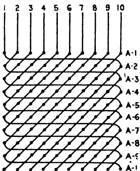
FIG. 15.—Symbol for bank slip.
