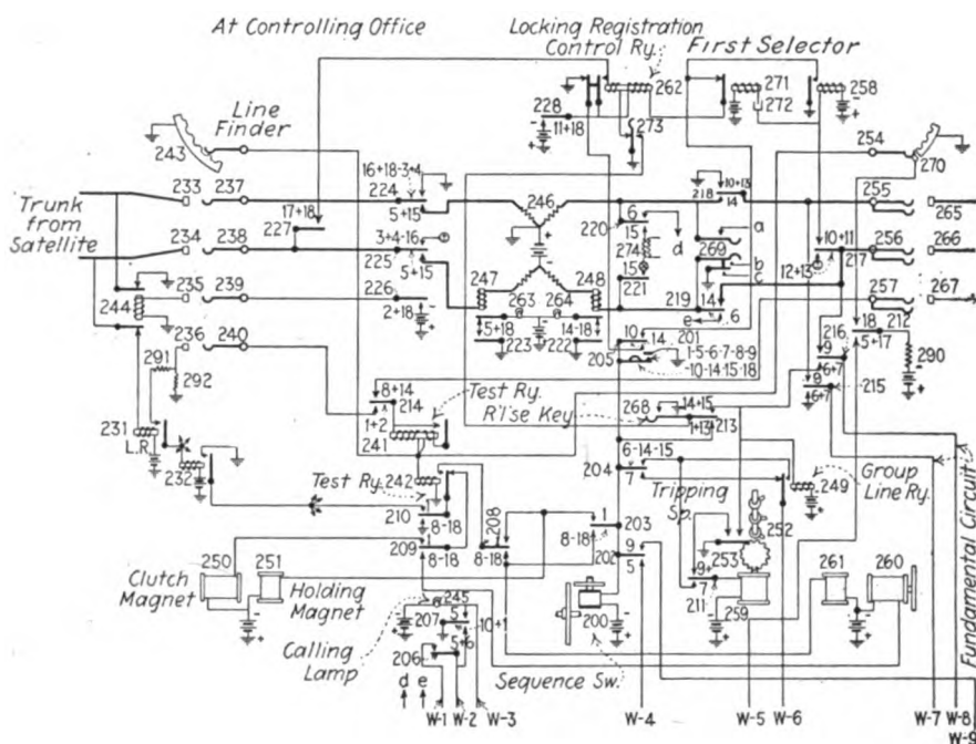
FIG. 211.—Secondary finder and first selector circuit.
