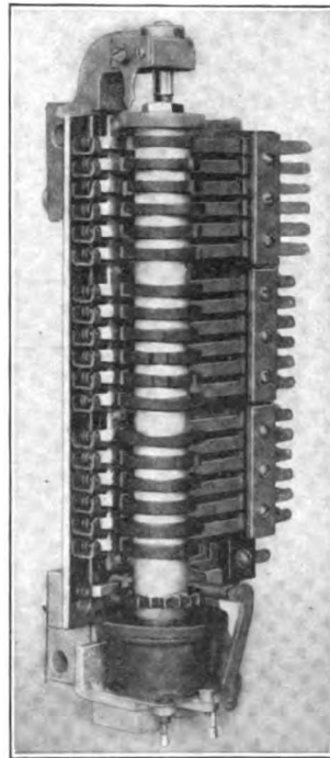
FIG. 206.—Sequence switch.
