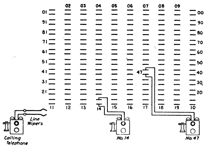
FIG. 4.—Essential principle of connector switch.
