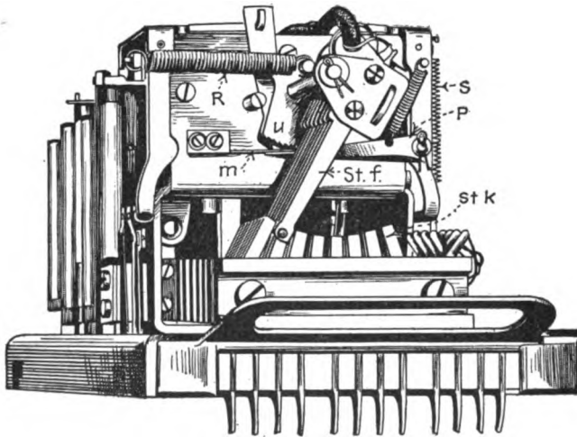
FIG. 105.—Side switch (top view).
