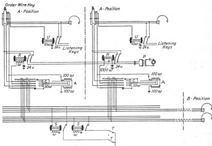
FIG. 159.—Circuit of automatic order wire system.
