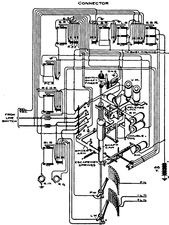
FIG. 50.—Connector-switch circuit.
