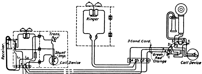
FIG. 66.—Wiring diagram for a wall telephone with an extension.
