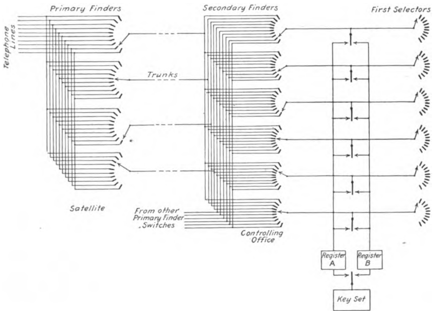
FIG. 209.—Arrangement of finders.
