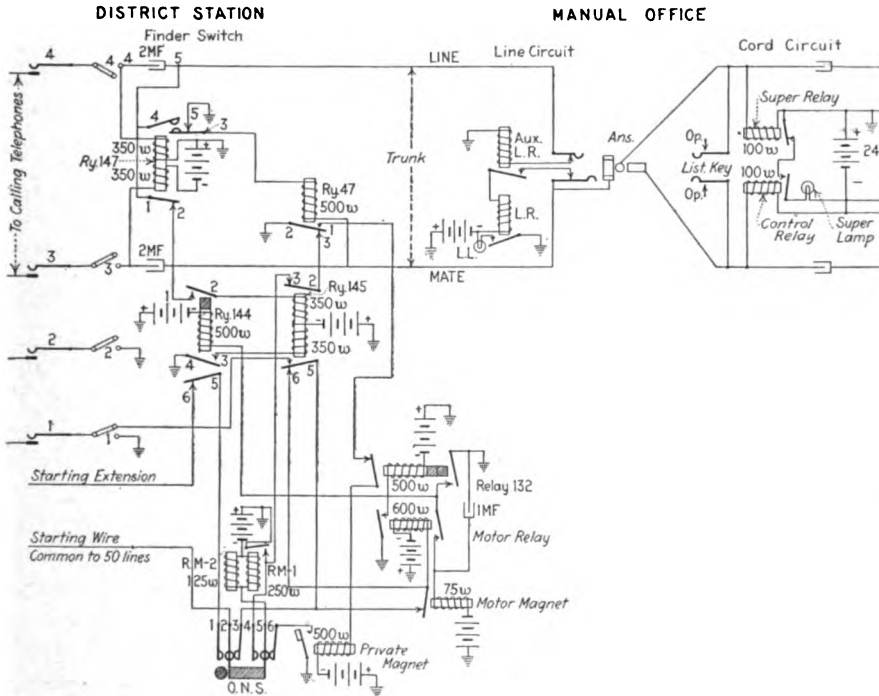
FIG. 167.—Finder circuit.
