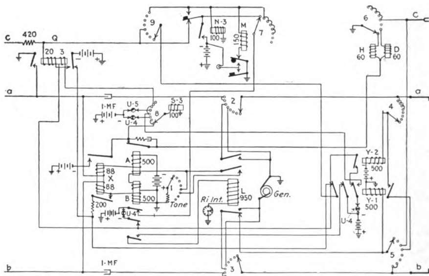
FIG. 111.—Connector circuit.
