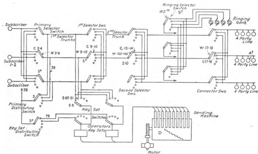
FIG. 175.—Trunking System.
