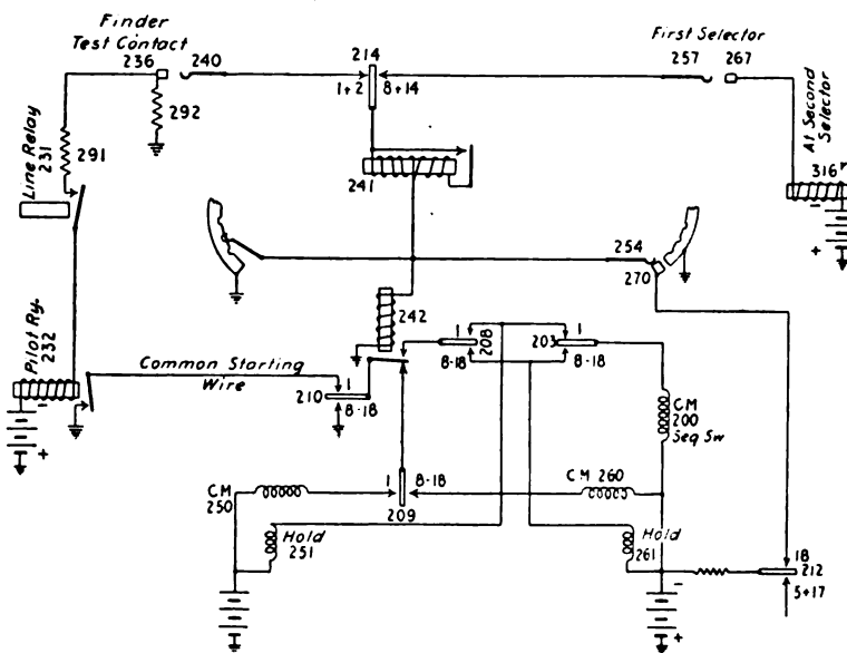
FIG. 225.—Testing circuit of secondary finder and first selector.
