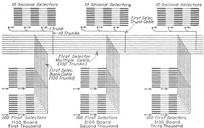
FIG. 9.—Trunking of first selectors by levels.
