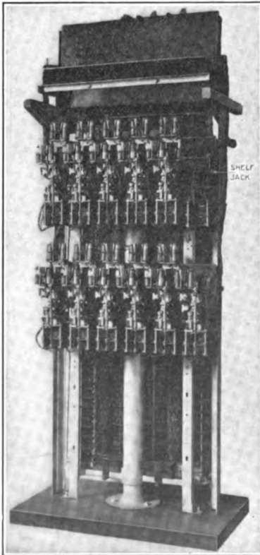
FIG. 45.—Reverse view of line-switch unit showing connector switches mounted.
