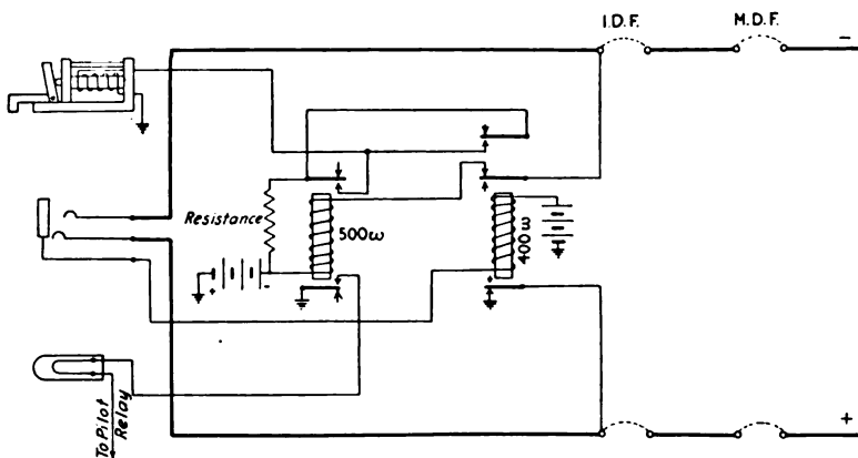
FIG. 232.—A pay-station line equipment at its toll-board end.
