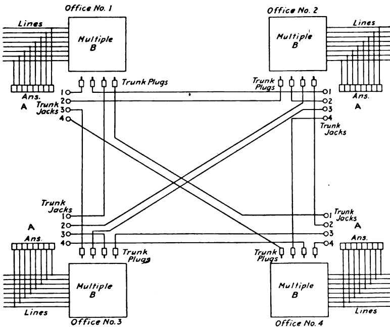
FIG. 3.—Manual inter-office trunking without " A " multiple.
