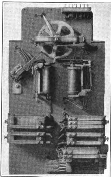
FIG. 92.—Selector switch, magnets and relays.
