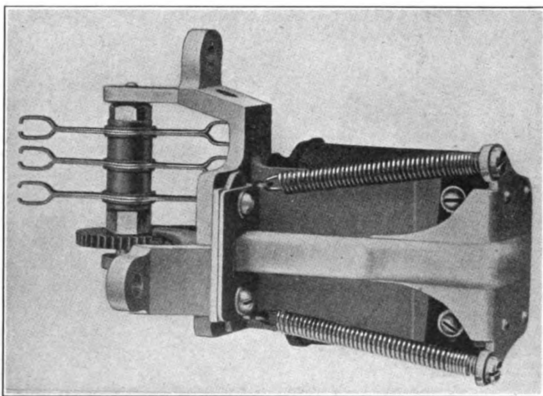
FIG. 189.—Wipers and magnet of rotary switch.
