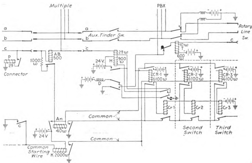
FIG. 117.—Auxiliary finder circuit.
