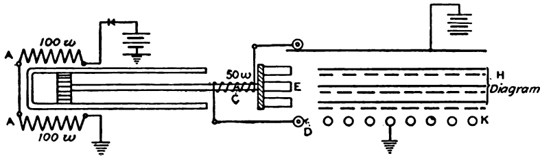
FIG. 158.—Diagram of circuit of Christensen pneumatic selector.
