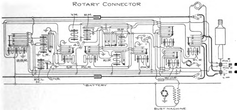
FIG. 63.—Circuit of a rotary or trunk selecting connector switch.
