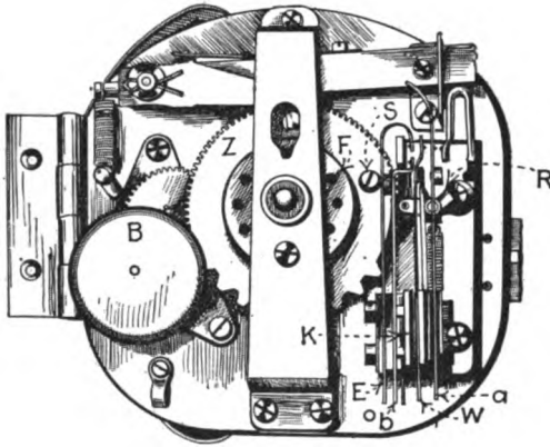
FIG. 100.—Rear of calling device.
