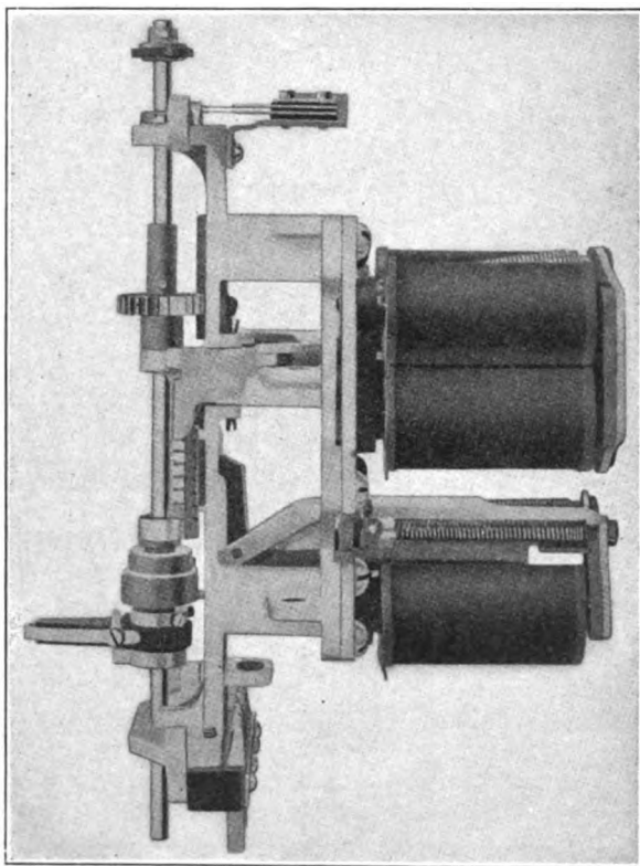
FIG. 192.—Wipers and magnets of switch unit.
