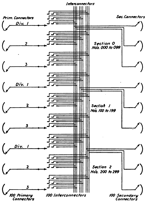
FIG. 126.—1000-line trunking system.
