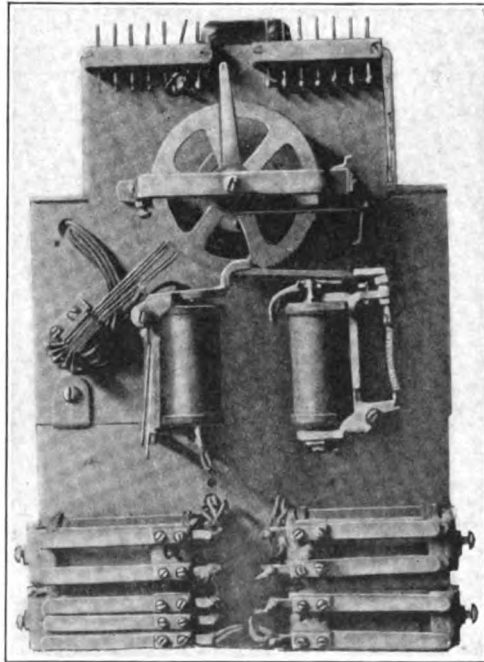
FIG. 91.—Finder switch with magnets and relays.
