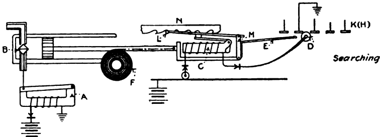
FIG. 156.—Christensen pneumatic selector "searching."
