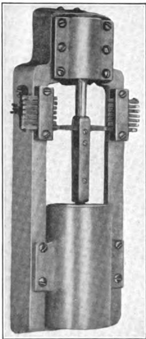
FIG. 241.—Solenoid ringing current interrupter.
