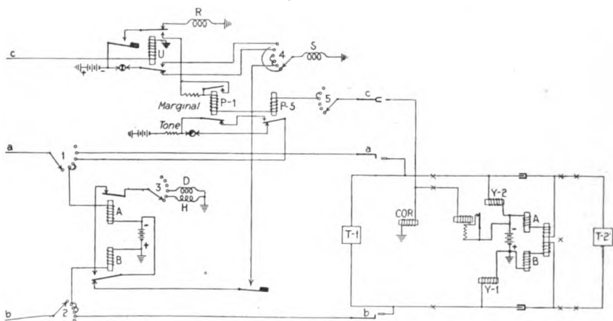
FIG. 114.—Toll connector circuit.
