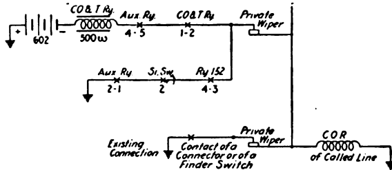
FIG. 174.—Testing a busy line.
