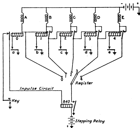
FIG. 223.—Principle of counting relays.
