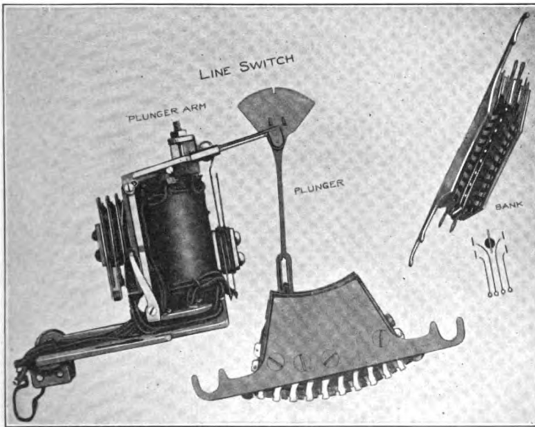
FIG. 36.—Single-spool Keith line switch with an unwired bank.
