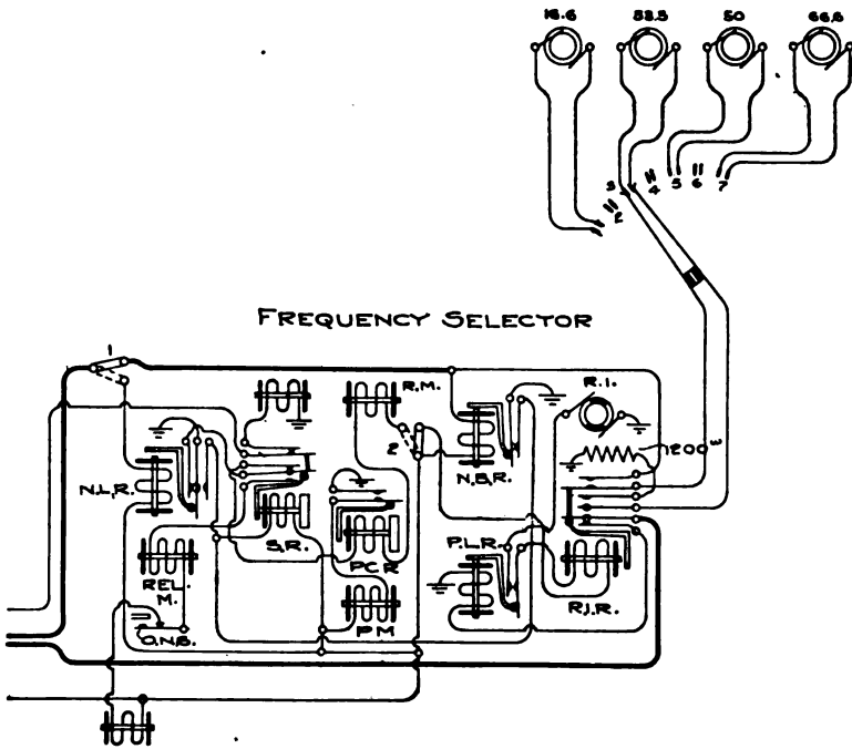
FIG. 62.—Circuit of a frequency selector.
