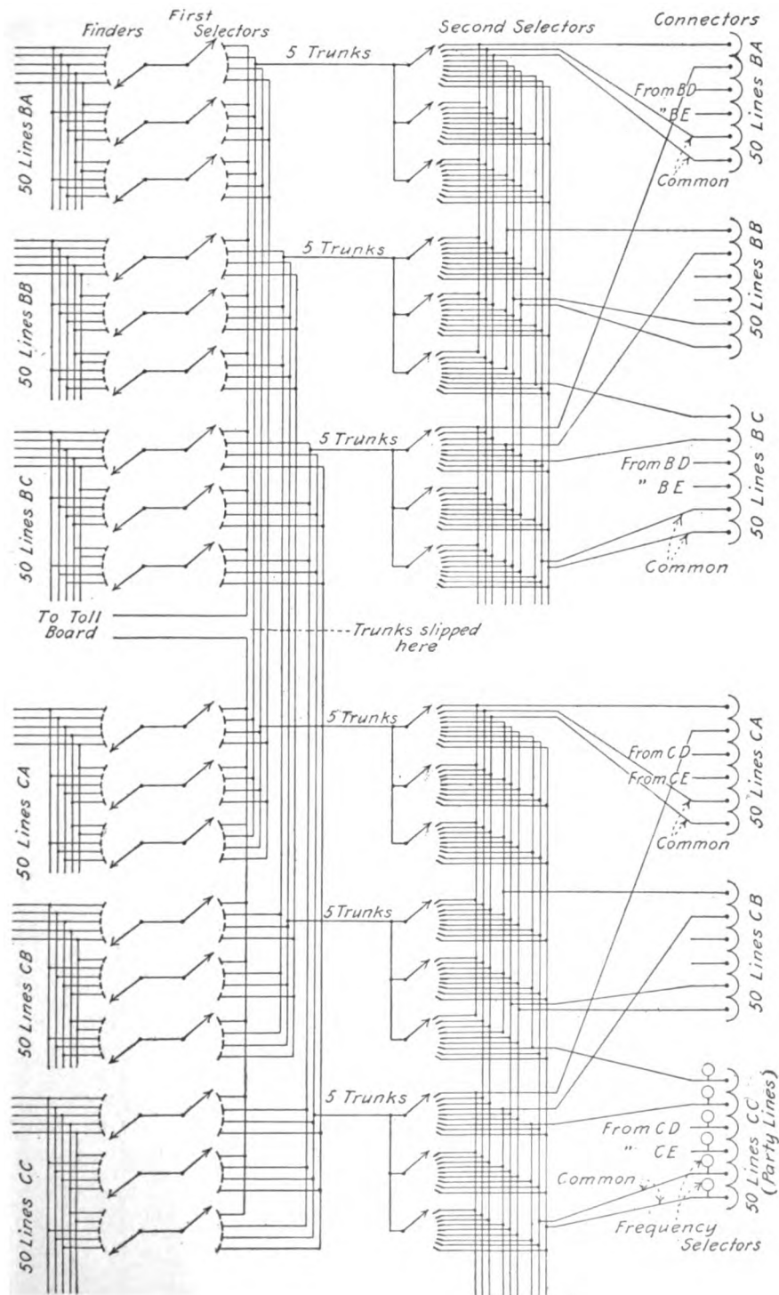
FIG. 94.—Trunking system.
