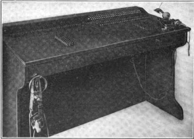
FIG. 195.—Operator's Desk.
