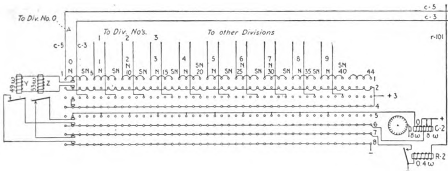
FIG. 141.—Division starter circuit.
