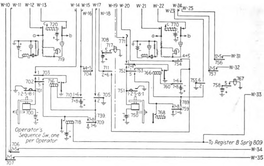
FIG. 216.—Operators' circuit.
