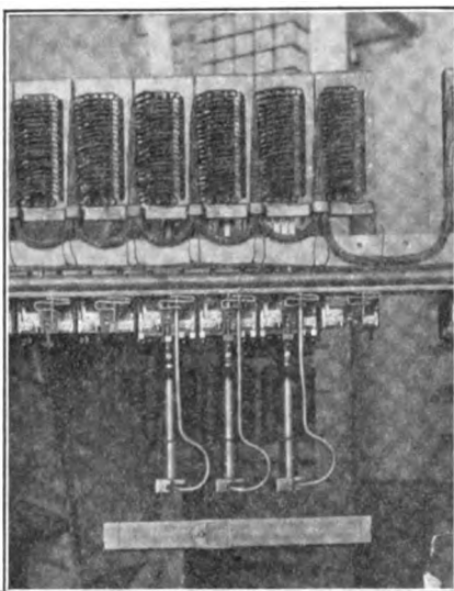
FIG. 153.—View from above of Christensen pneumatic selectors.
