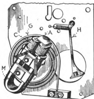
FIG. 85.—Magneto gong of collector in Fig. 83.
