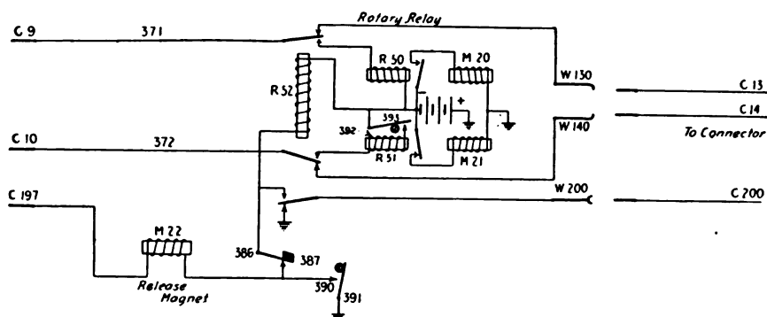
FIG. 182.—Second selector circuit.
