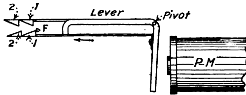
FIG. 44.—Private magnet and spider arm escapement.
