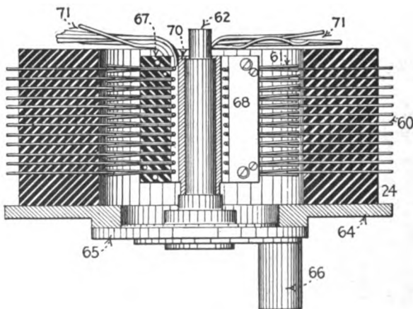
FIG. 128.—Vertical cross-section of cylinder switch.
