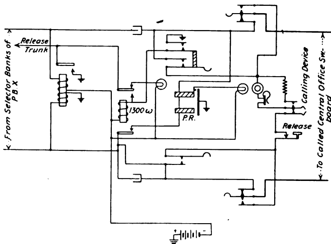
FIG. 77.—Outgoing trunk circuit through attendant's cabinet.
