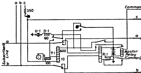
FIG. 106.—Rotary line-switch circuit.
