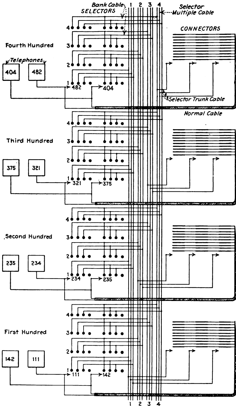
FIG. 6.—Principle of 1000-line exchange.
