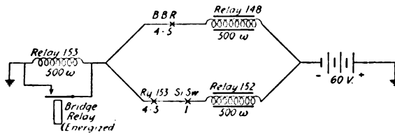
FIG. 172.—Holding circuit in connector.
