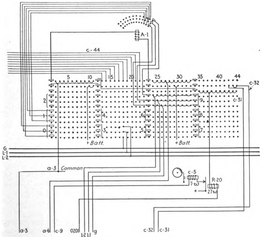
FIG. 142.—Primary connector circuit.
