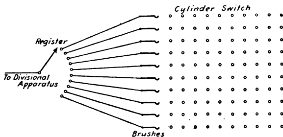
FIG. 132.—Relation of register to cylinder switch.
