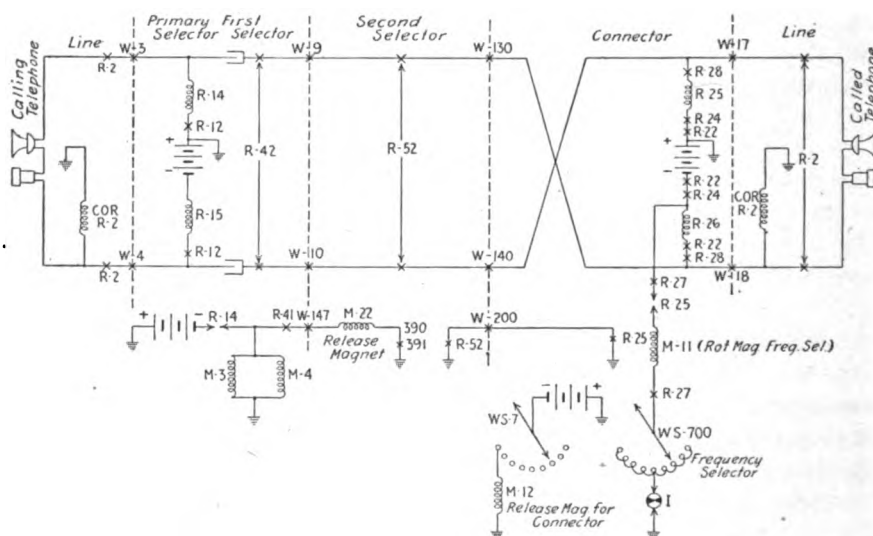
FIG. 185.—Talking connection between stations.
