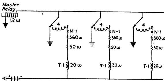
FIG. 107.—Master relay circuit.
