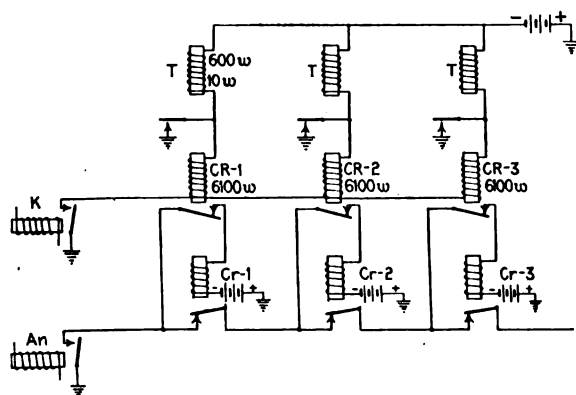
FIG. 118.—Removal of starting relays from circuit.
