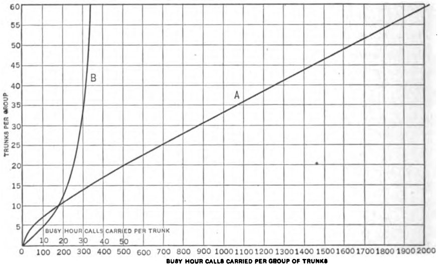
FIG. 263.—Curve A shows call-carrying capacities of trunk groups of various sizes between automatic central offices; average trunk holding time of 83 seconds. Curve B shows call-carrying capacity of each trunk in groups of various sizes.
