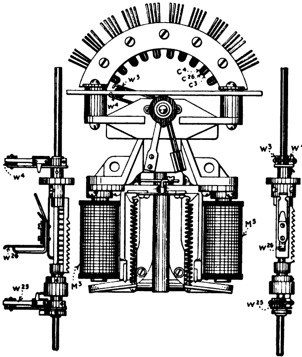
FIG. 194.—Plan-view of 2-motion switch.
