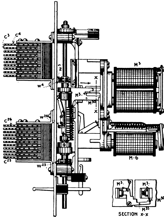
FIG. 193.—Side view of 2-motion switch.
