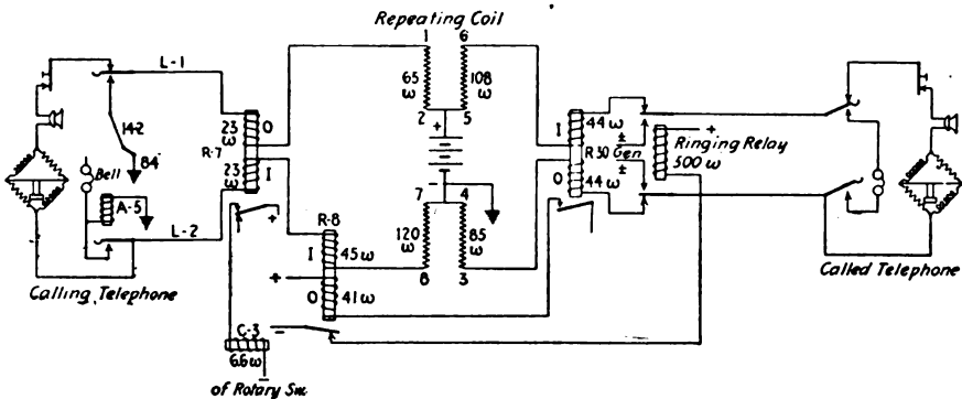
FIG. 149.—Talking circuit between subscribers.
