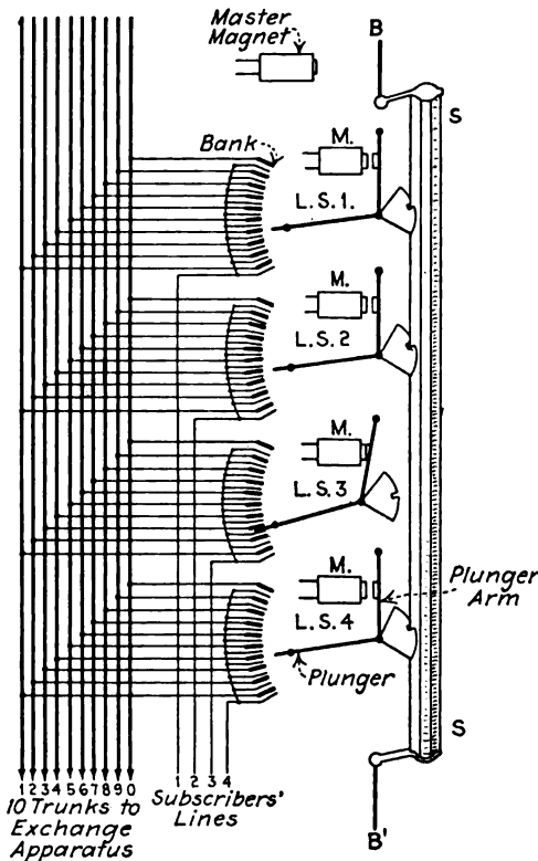
FIG. 20.—Principle of Keith type line switch.
