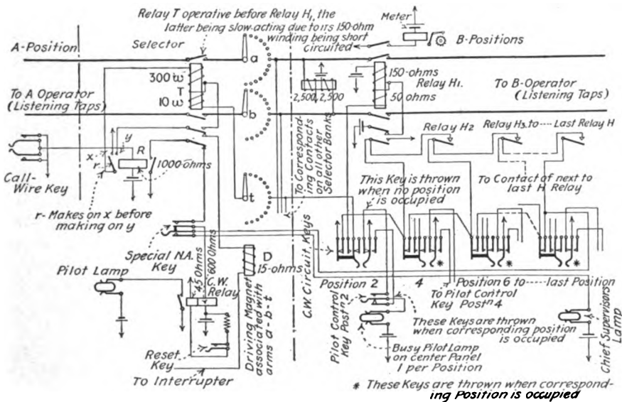
FIG. 163.—Circuit of Siemens-Halske call wire selector installed at the Central exchange in London.
