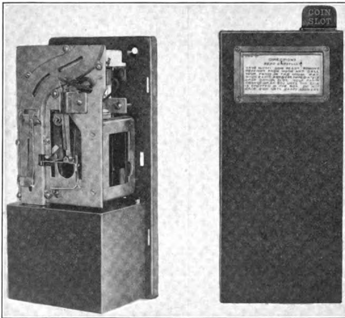
FIG. 80.—Interior and exterior views of automatic coin collector.
