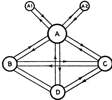
FIG. 2.—Indirect inter-office trunking.
