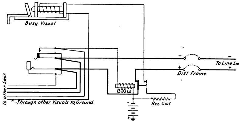
FIG. 231.—An overflow trunk from a toll switchboard to an automatic switchboard.
