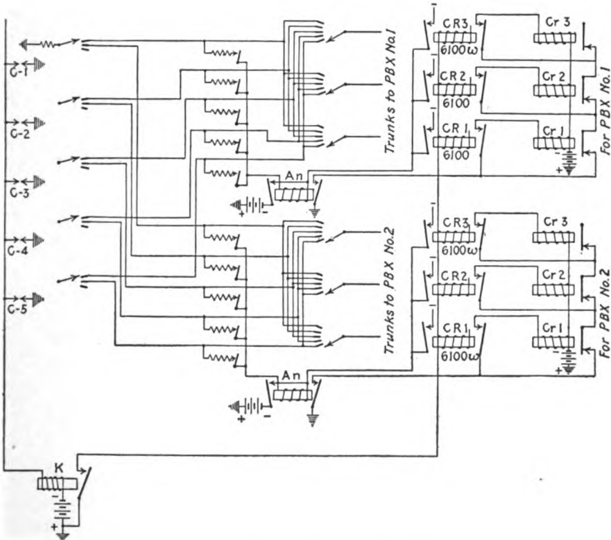
FIG. 116.—Selection of idle trunk to PBX.
