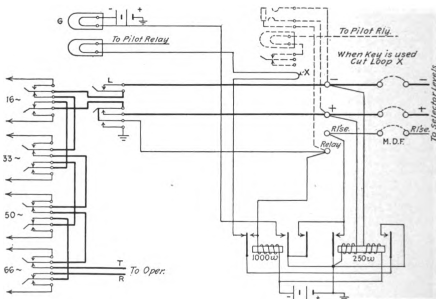
FIG. 255.—Trunk circuit for handling reverting calls on 4-party lines.
