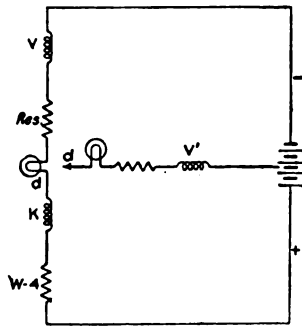
FIG. 125.—Protection of call finder from other finders.
