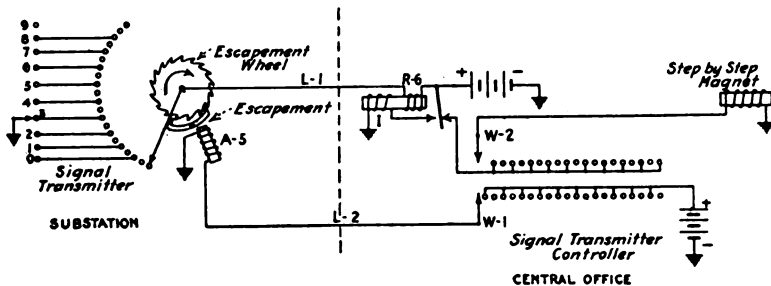
FIG. 138.—Line circuit (telephone to switches).
