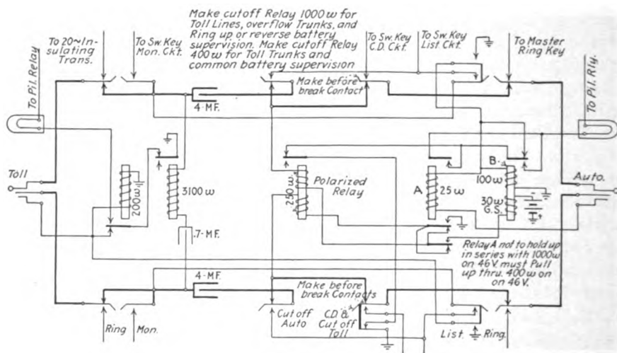
FIG. 230.—A typical cord circuit for connecting toll lines to local automatic switchboard lines.
