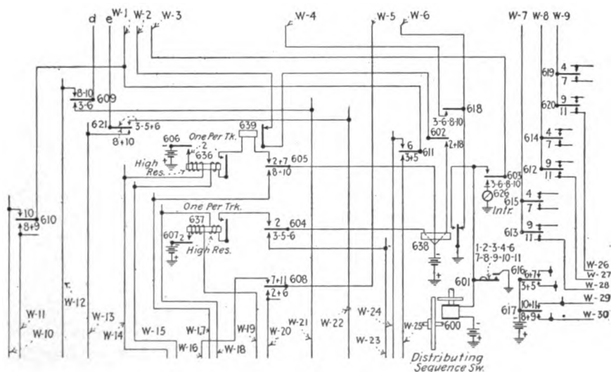
FIG. 215.—Distributing sequence switch circuit.
