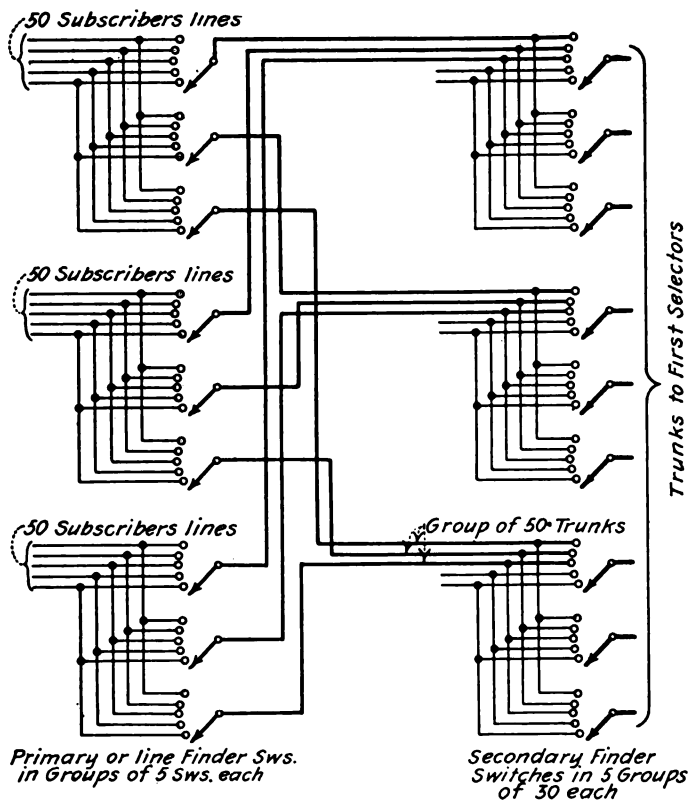
FIG. 26.—Primary and secondary line finders.
