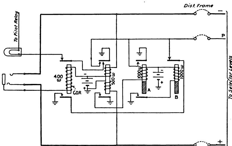
FIG. 235.—Circuit of trunk incoming to a rural-line switchboard from an automatic switchboard.
