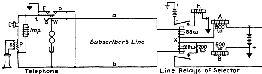
FIG. 108.—Line circuit (telephone to selector).
