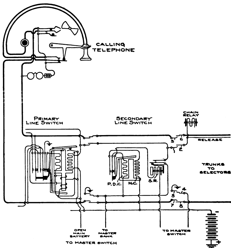
FIG. 60.—Circuit of secondary line switch.
