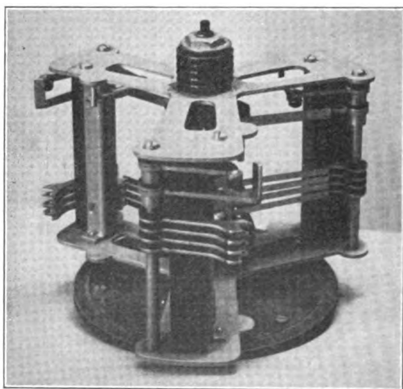
FIG. 199.—Finder brush carriage.
