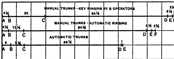
FIG. 264.—Graphical analysis of trunk holding times: A , is instant at which a trunk is assigned by a " B " operator or taken by an automatic selector switch; B , connection completed and ringing started; C , subscriber answers; D , Conversation completed—disconnect signals given to " A " operator; E , " A " operator or automatic selector disconnects from the trunk; F , " B " operator releases the trunk.
