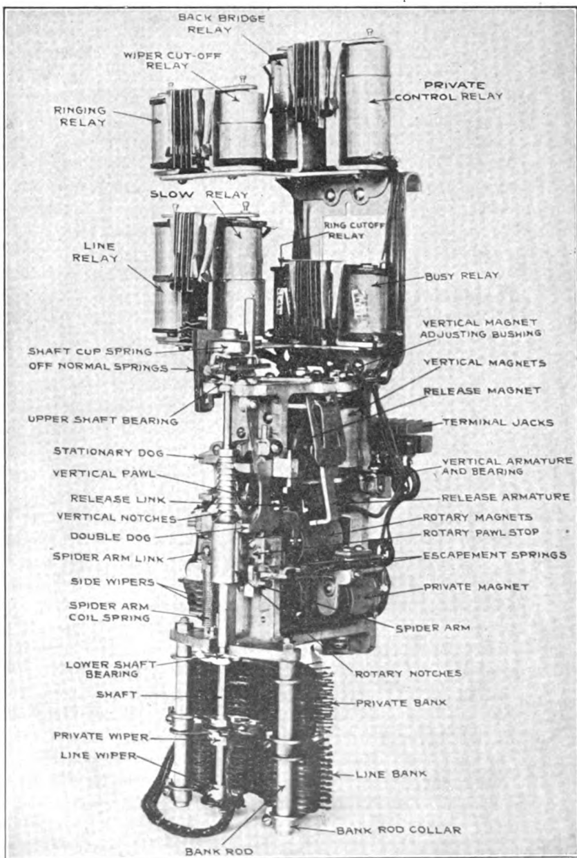
FIG. 42.—Two-wire connector switch.
