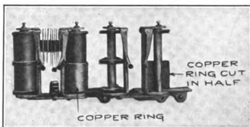
FIG. 49.—Details of slow-acting relays.
