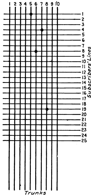
FIG. 19.—Relation of subscribers' lines to trunks in Keith line switch.
