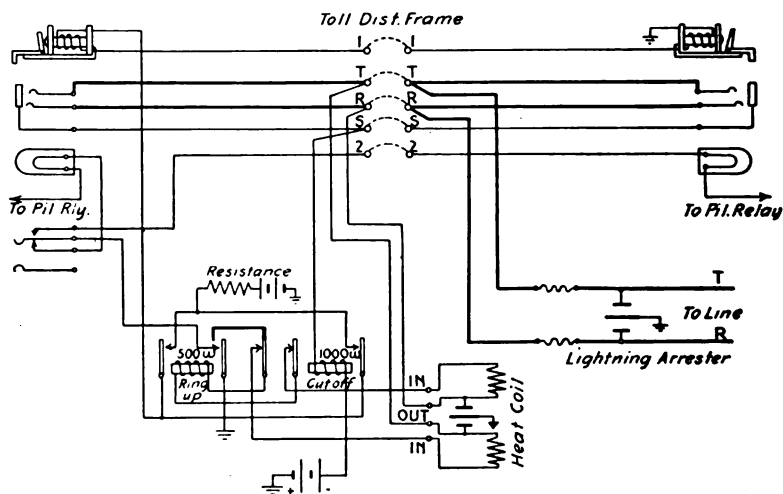
FIG. 229.—A typical toll or rural-line circuit.
