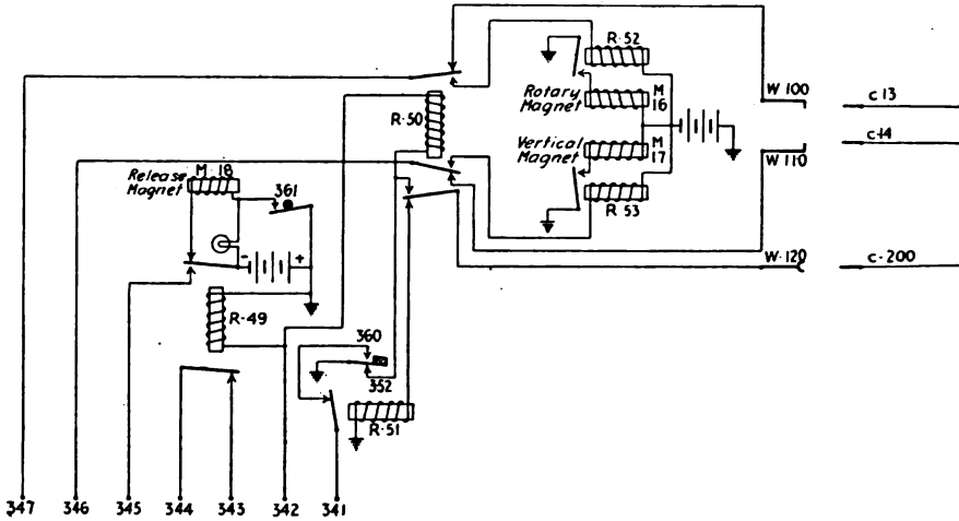
FIG. 186.—Selector for reverting calls.
