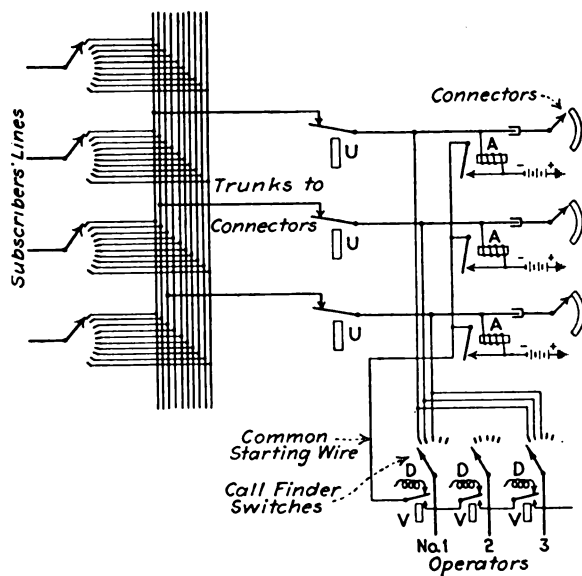
FIG. 122.—Trunking in semi-automatic system with call finders.
