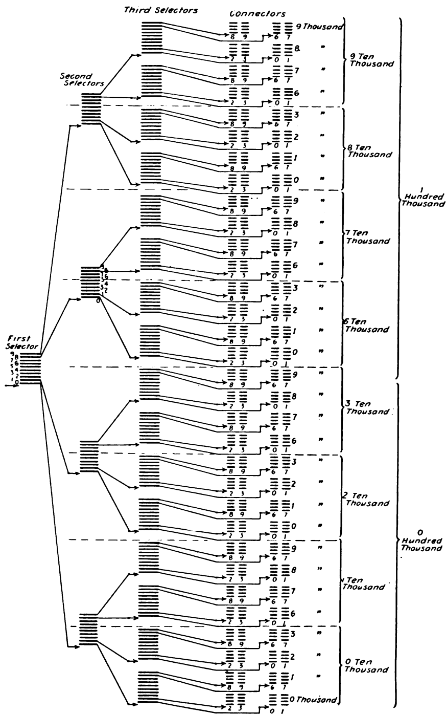
FIG. 208.—Trunking scheme.
