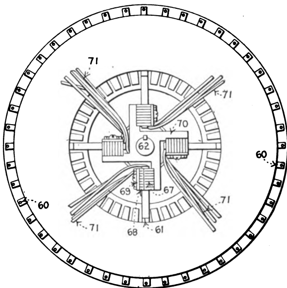
FIG. 127.—Top view of cylinder switch.
