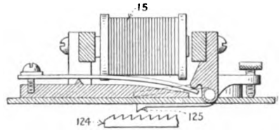
FIG. 136.—Stop magnet of decimal indicator.
