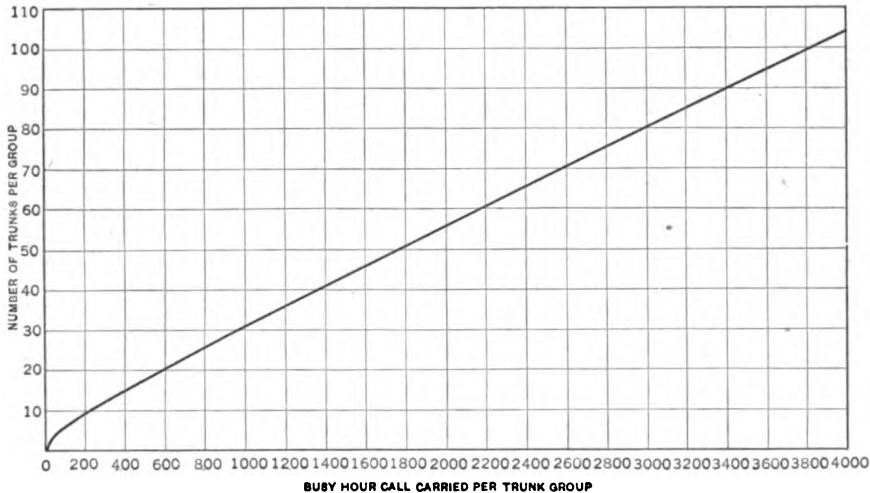
FIG. 271.—Curve showing carrying capacities of trunk groups of hypothetical system in Fig. 270.
