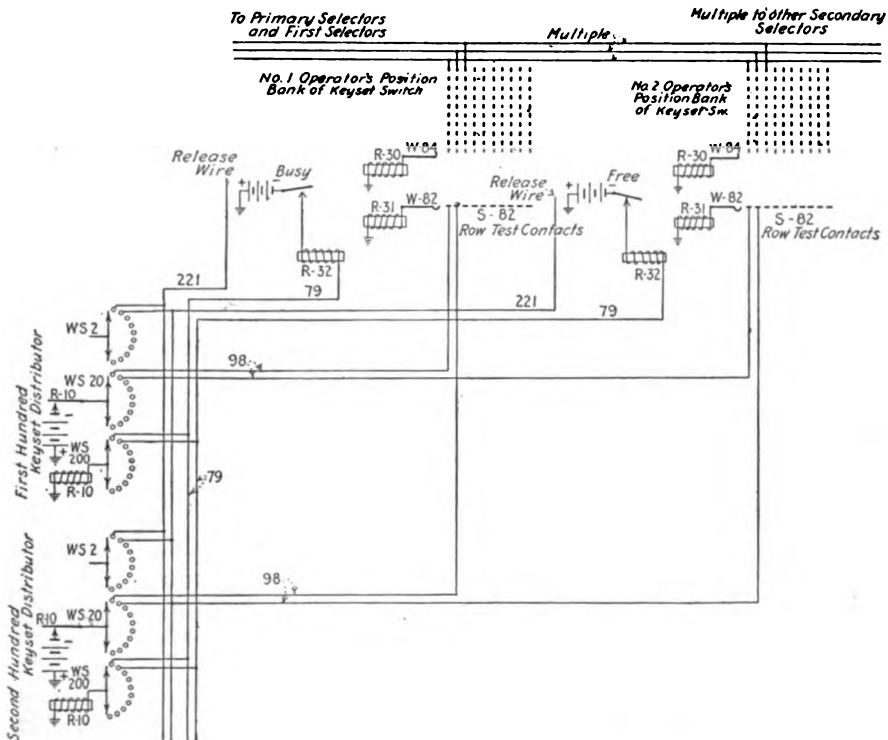
FIG. 177.—Relation between distributors and keyset switches.
