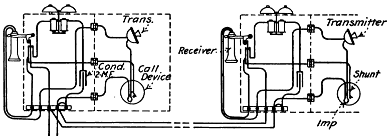
FIG. 67.—Wiring diagram of a wall telephone with an extension.
