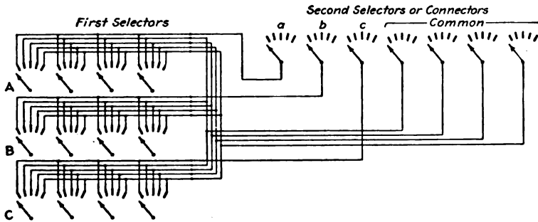
FIG. 16.—Individual trunks with common group.
