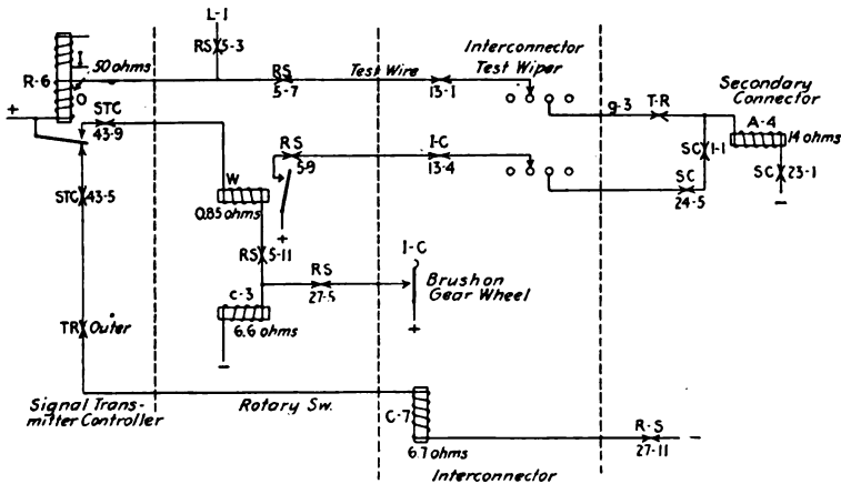
FIG. 148.—Selecting an idle trunk.
