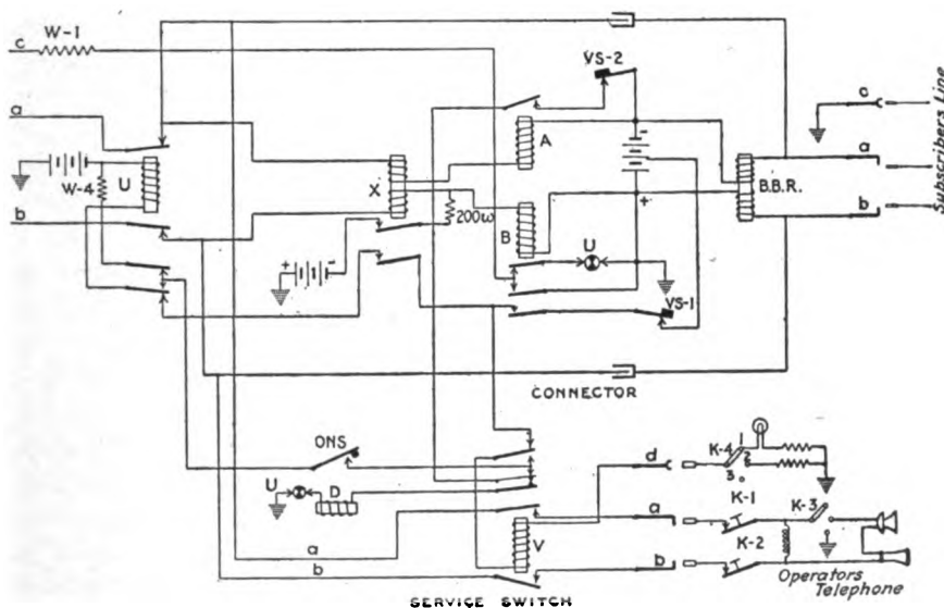
FIG. 120.—Circuit of service switch.
