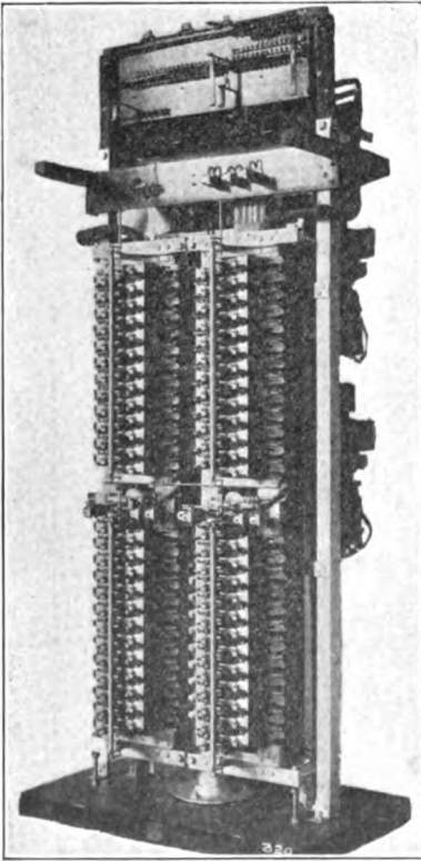
FIG. 37.—Keith line switch unit carrying 100-line switches.
