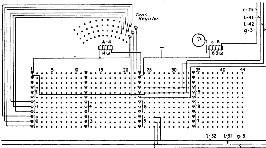
FIG. 146.—Secondary connector circuit.
