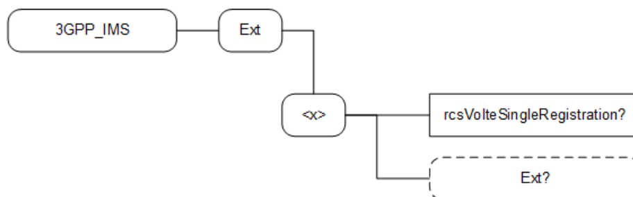
Figure 32: Additions to the IMS MO sub tree
