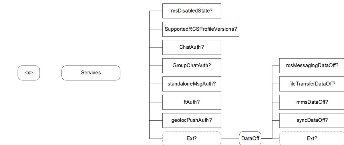
Figure 28: RCS additions, Services sub tree
