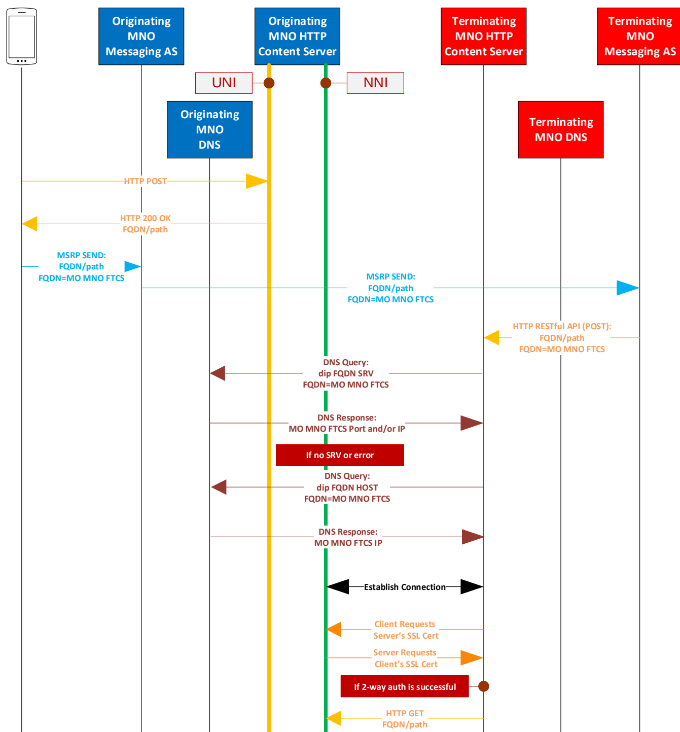
Figure 20: Mutual Authentication for HTTP File Transfer Localization Option 1 (SRV based)
