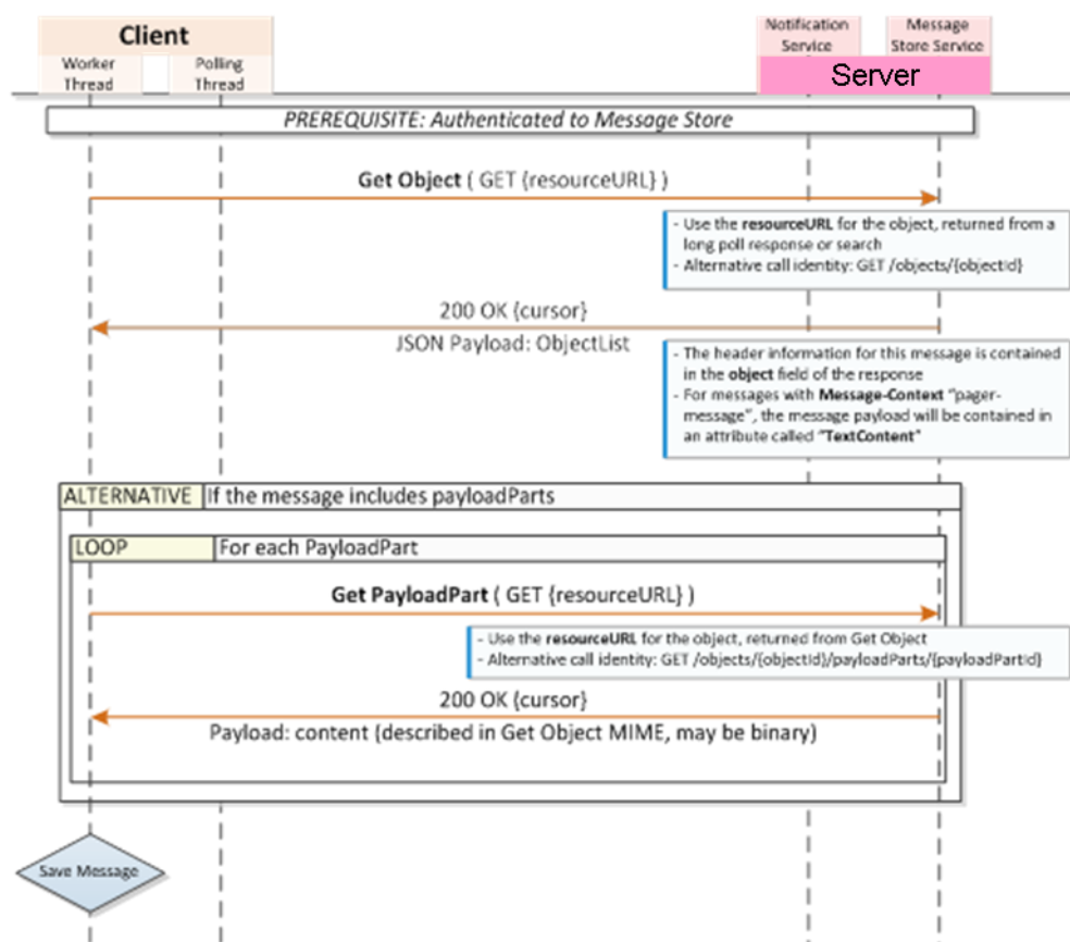
Figure 45: Message Store – Example Object Download
