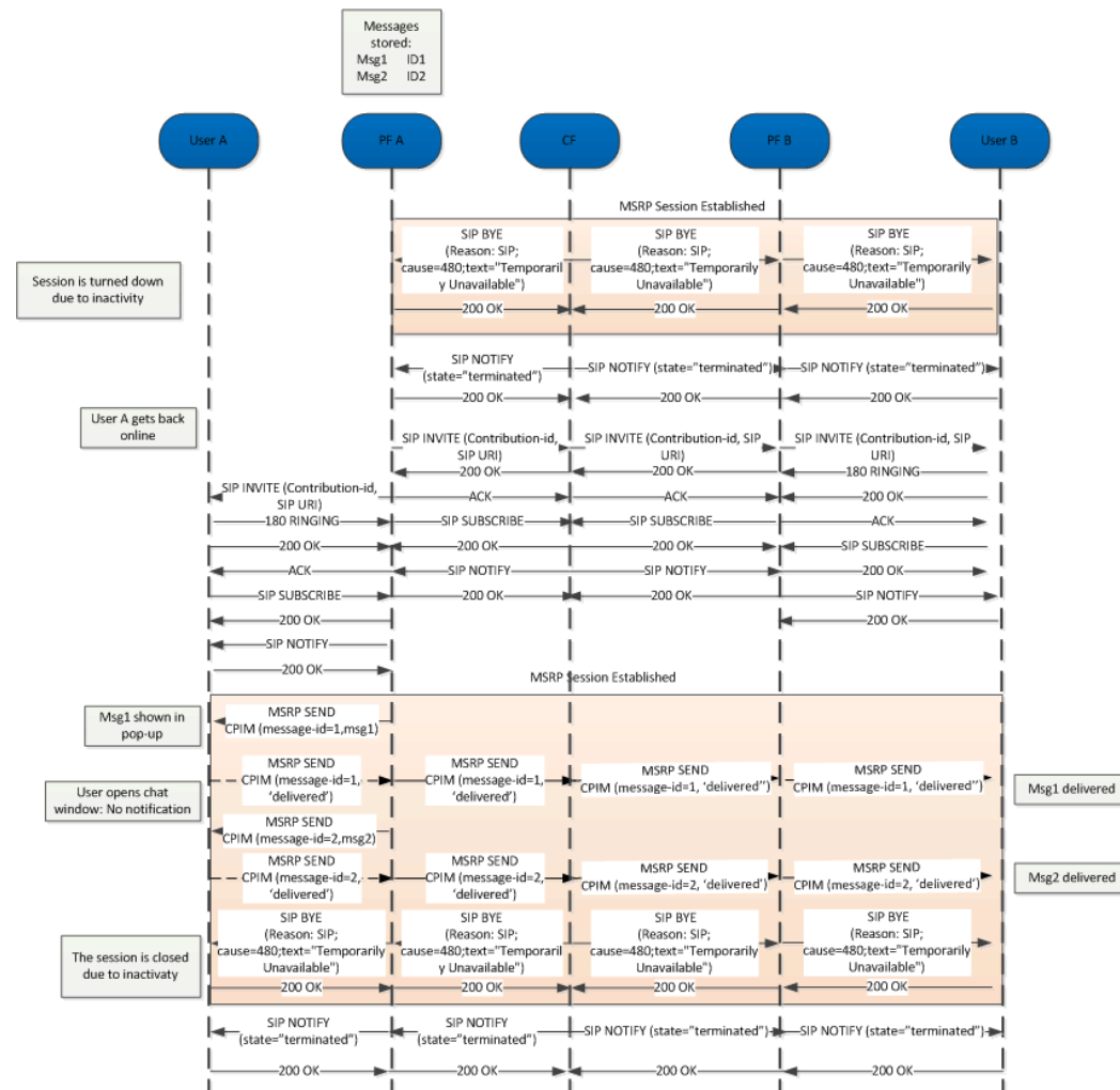
Figure 41: Deliver Group Chat Messages while Chat is idle*
