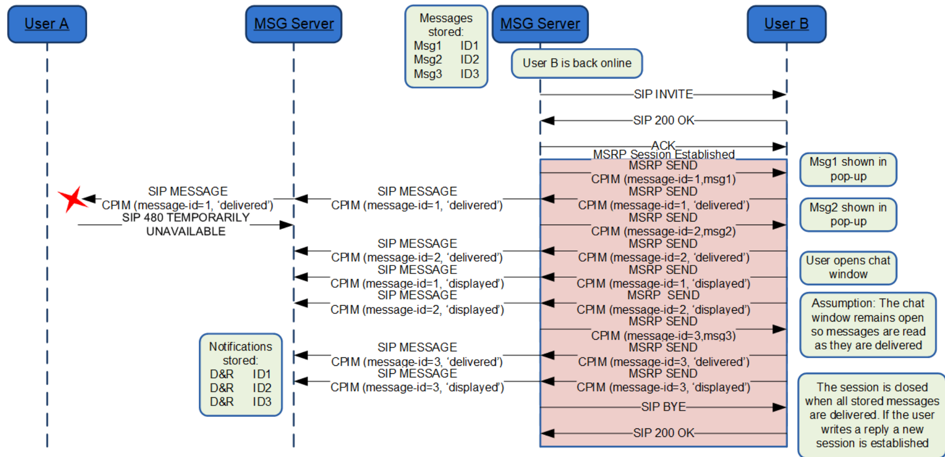
Figure 36: Store and forward: Message(s) deferred delivery with a sender offline (delivery notifications) *
