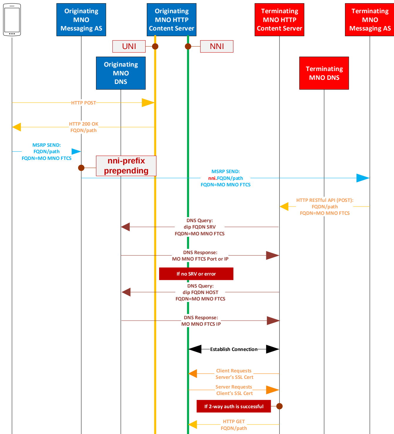
Figure 21: Mutual Authentication for HTTP File Transfer Localization Option 2 with Originating MNO performing “nni-prefix prepending”
