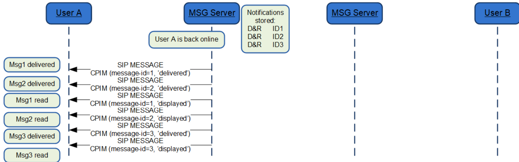
Figure 37: Store and forward: Notification(s) deferred delivery*
