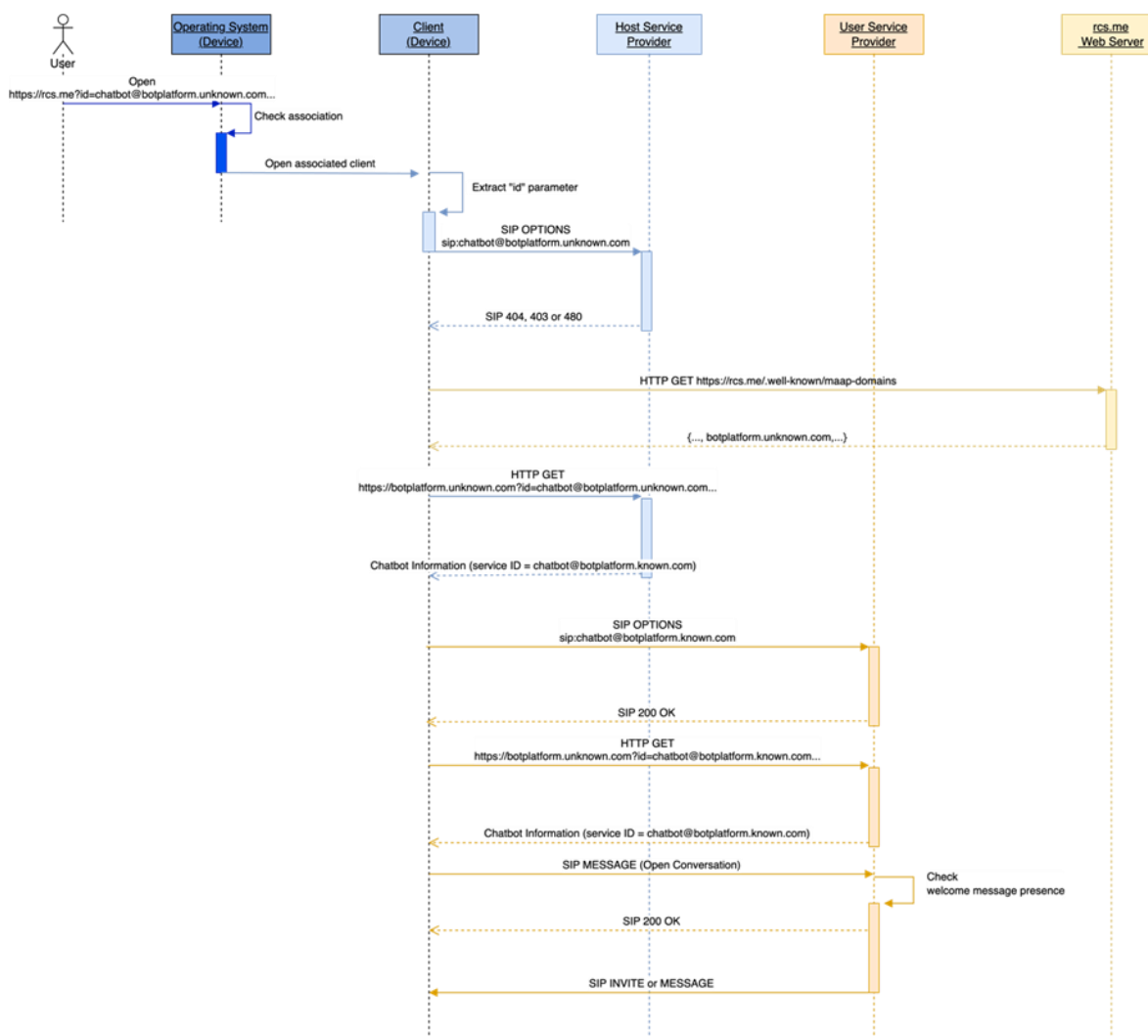
Figure 13: rcs.me fallback via alternative Chatbot service identifier
