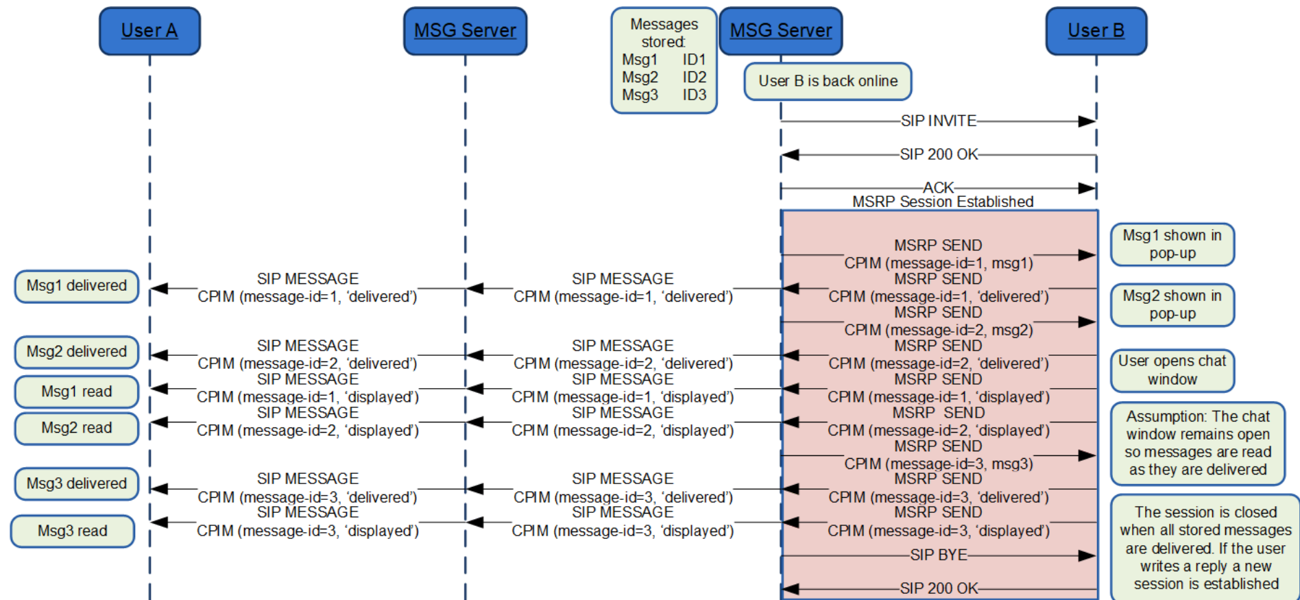
Figure 35: Store and forward: Message deferred delivery with sender online *
