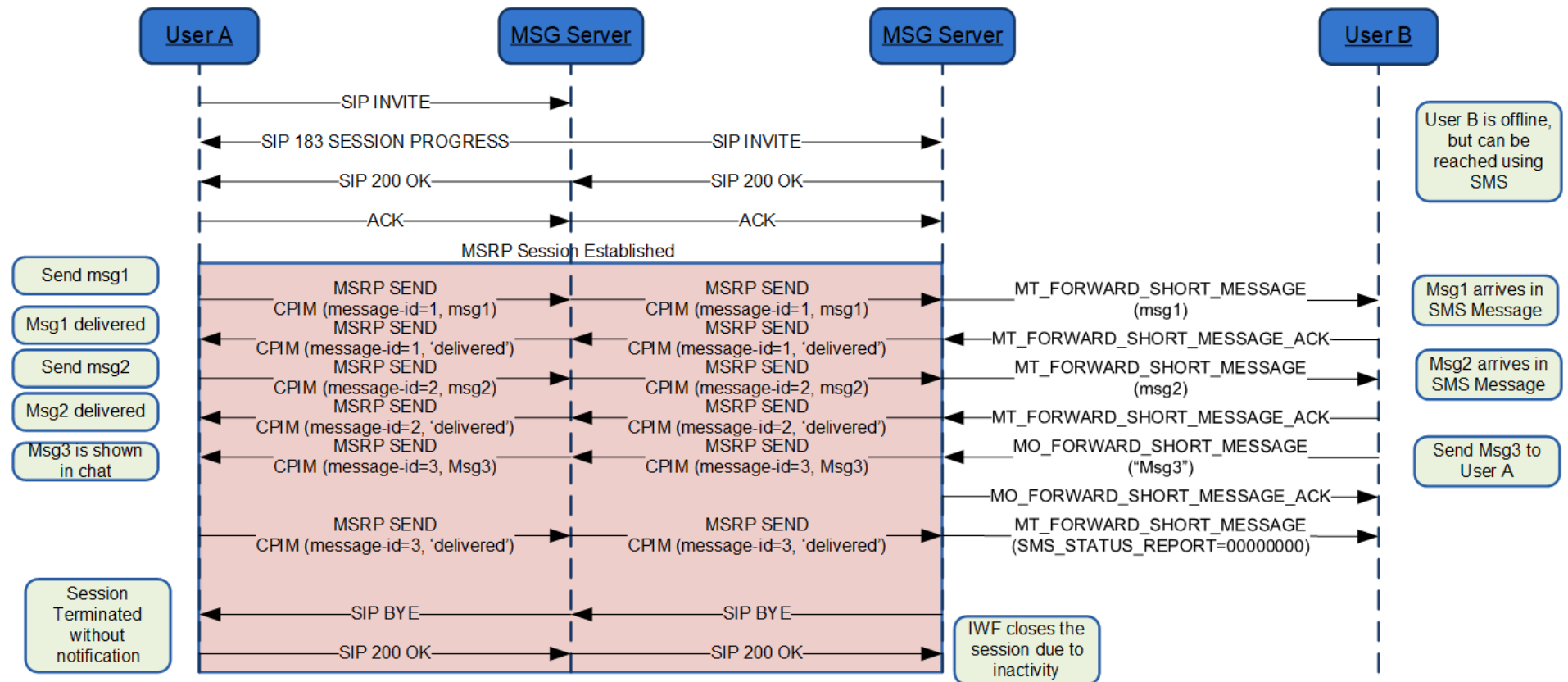
Figure 38: Interworking: Automatic acceptance on behalf of the SMS/MMS user*
