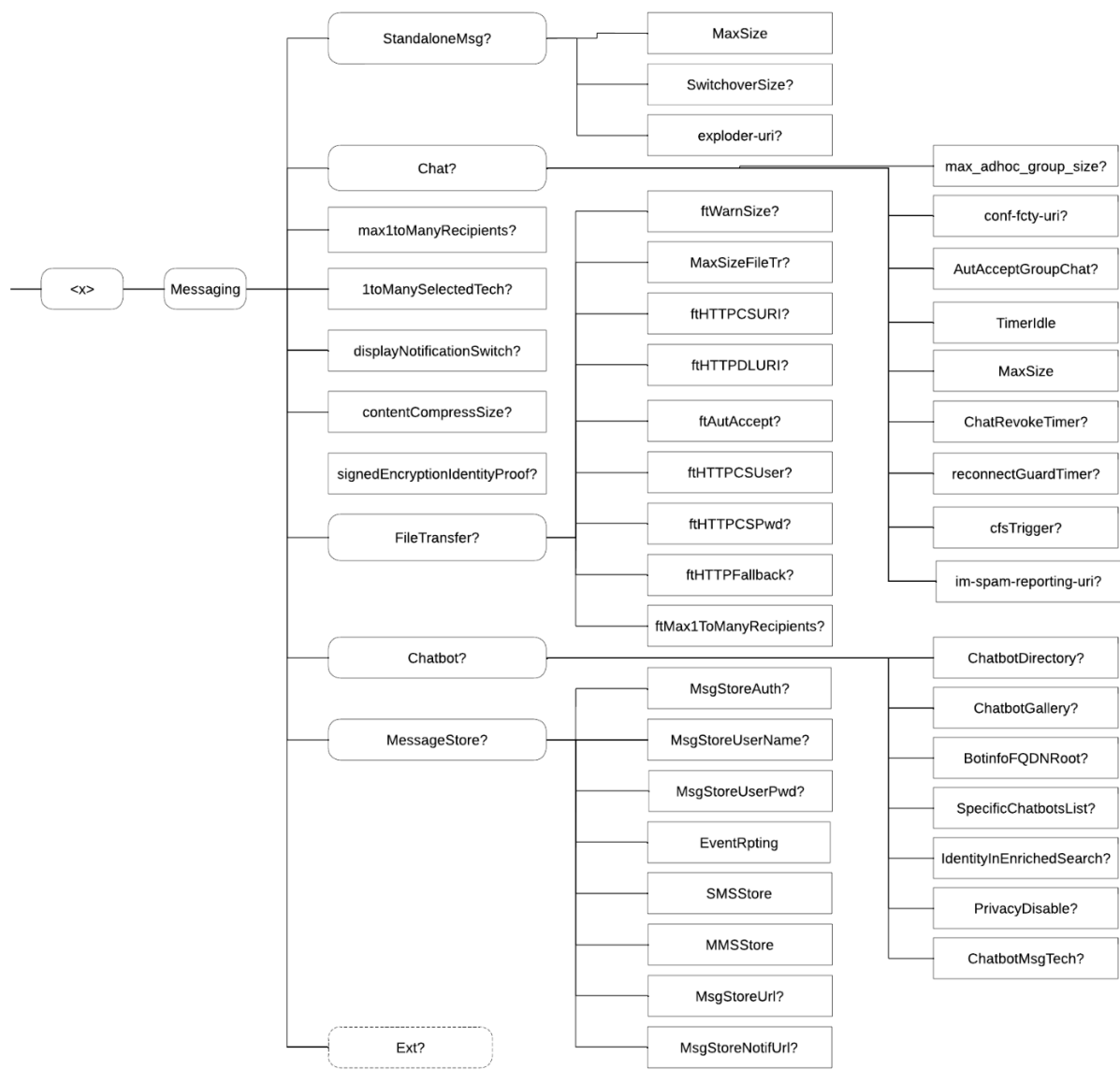
Figure 29: RCS additions to the IM MO sub tree
