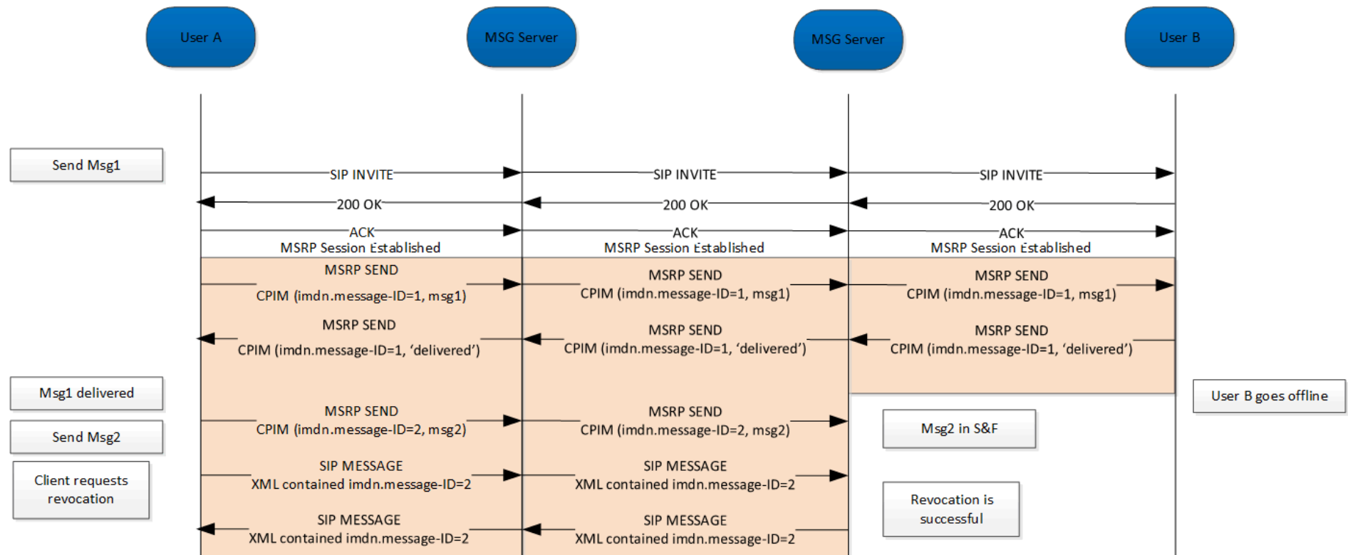
Figure 39: Message Revoke, Successful request*
