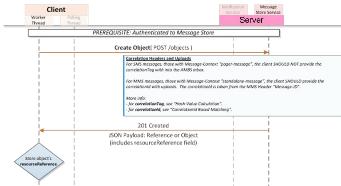
Figure 44: Message Store – Object Upload
