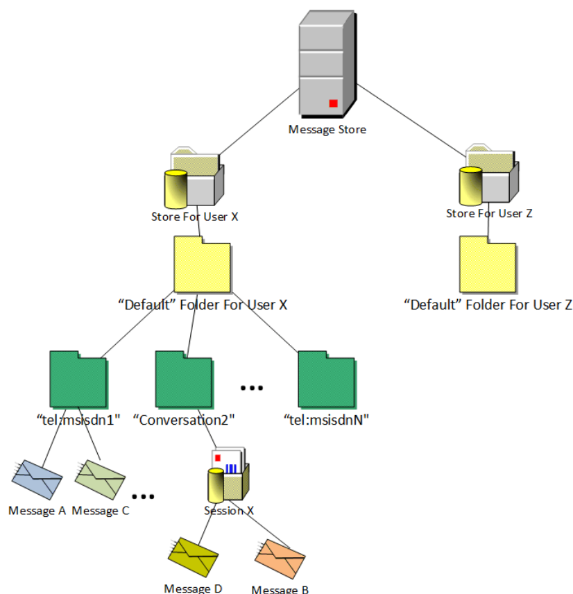
Figure 18: Example Folder Structure
