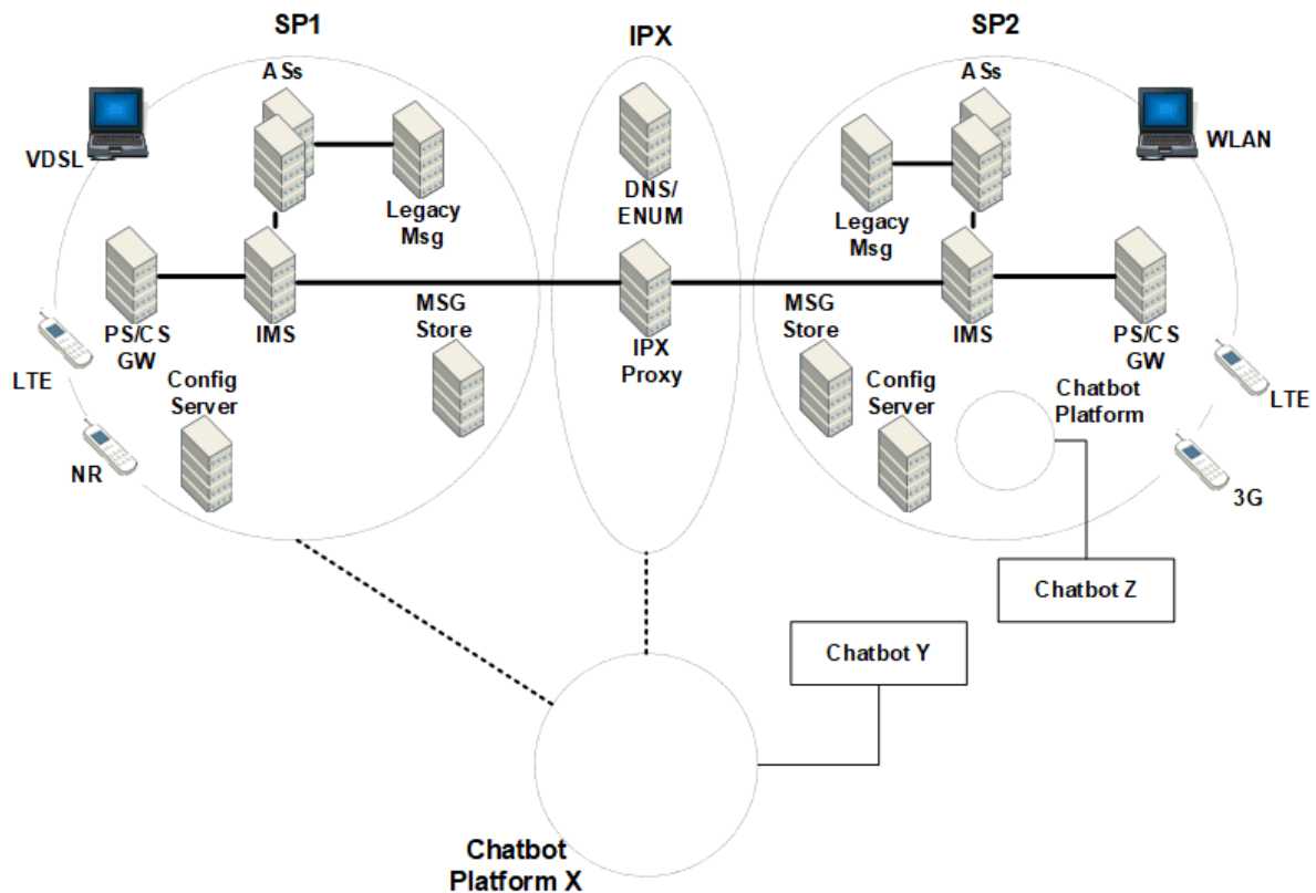
Figure 1: Simplified Example of RCS Architecture
