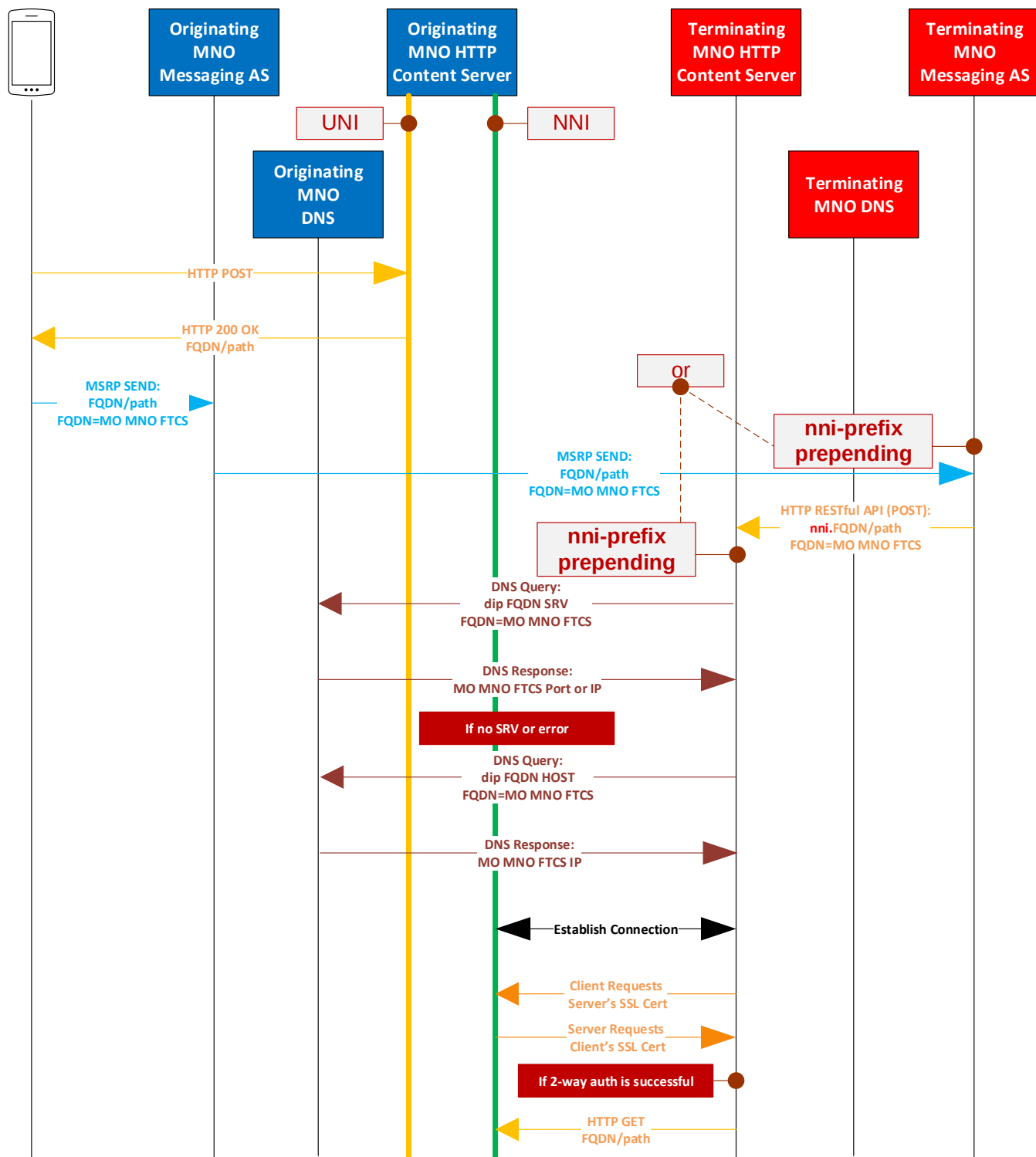
Figure 22: Mutual Authentication for HTTP File Transfer Localization Option 2 with Terminating MNO performing “nni-prefix prepending”
