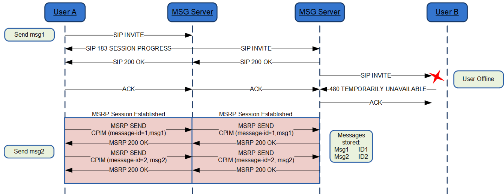
Figure 33: Store and forward: Receiver offline*
