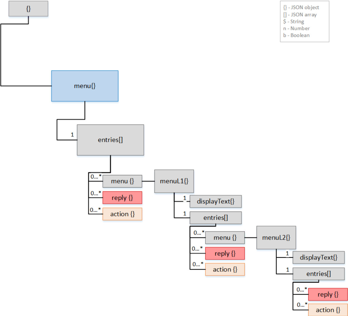
Figure 17: JSON Chatbot Menu data structure overview
