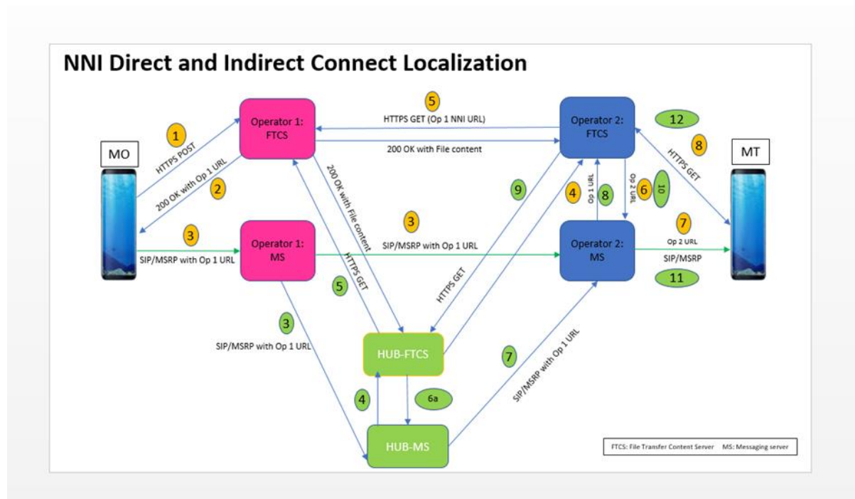
Figure 23: NNI Localisation with direct and indirect connections
