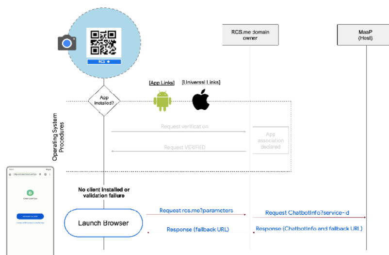
Figure 12: rcs.me validation failure
