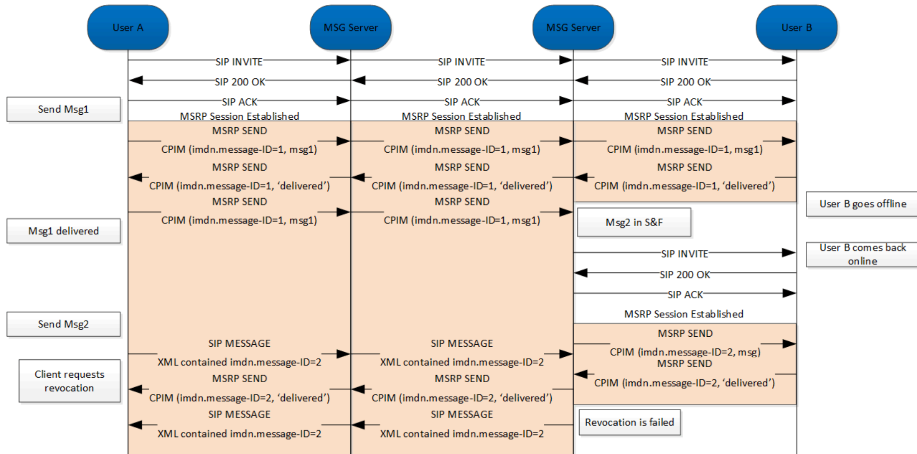
Figure 40: Message Revoke, Failed request*
