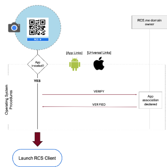
Figure 11: rcs.me link validation
