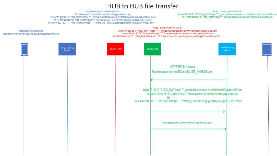
Figure 25: Mutual Authentication for HTTP File Transfer Localization Hub to Hub transfer (Part 2)
