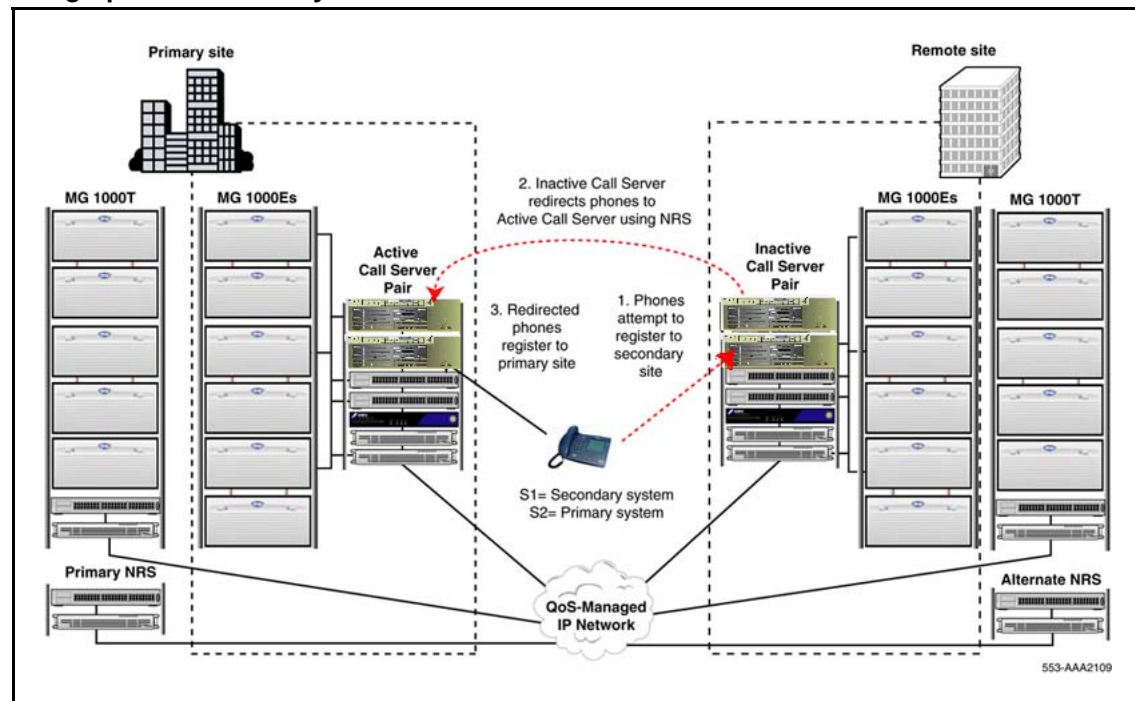
Figure 17 Geographic Redundancy
