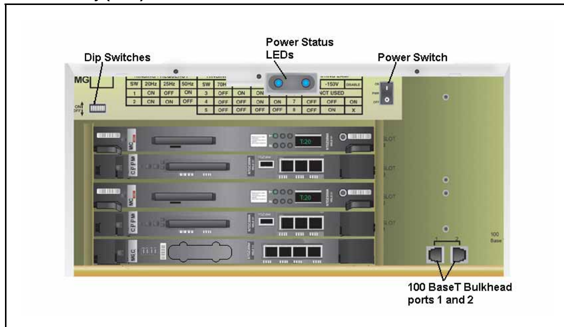
Figure 4 Media Gateway (front)
