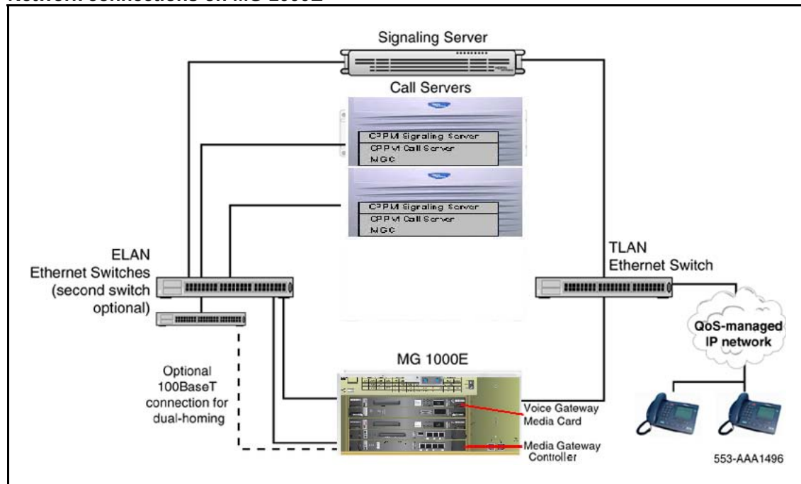
Figure 10 Network connections on MG 1000E
