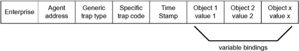
Figure 15: SNMPv1 trap PDU fields
