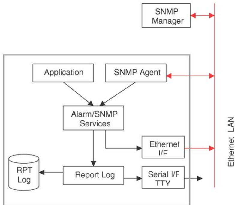
Figure 5: Event architecture on the Voice Gateway Media Card and Gateway Controller
