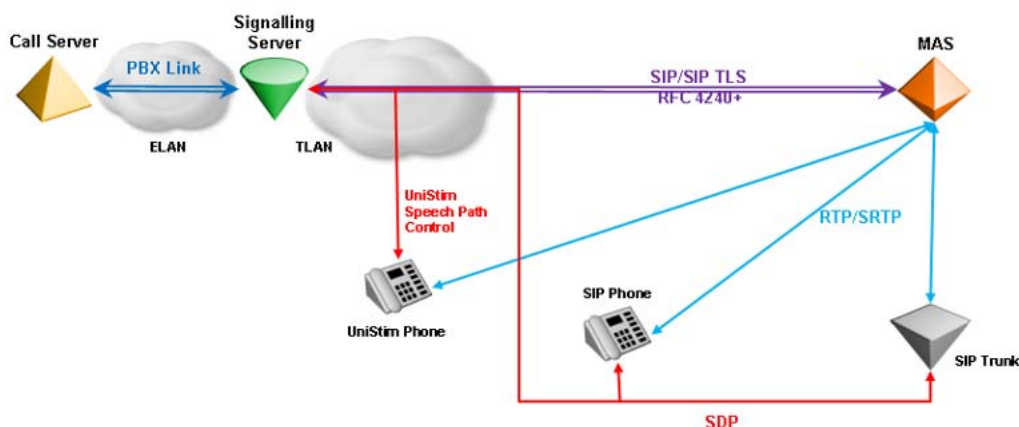
Figure 7: IP Media Services system architecture
