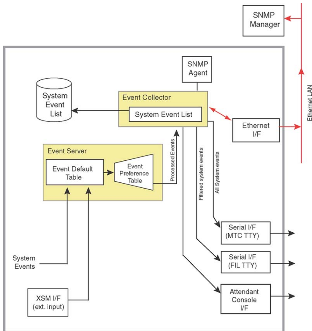
Figure 4: Event architecture on the Call Server
