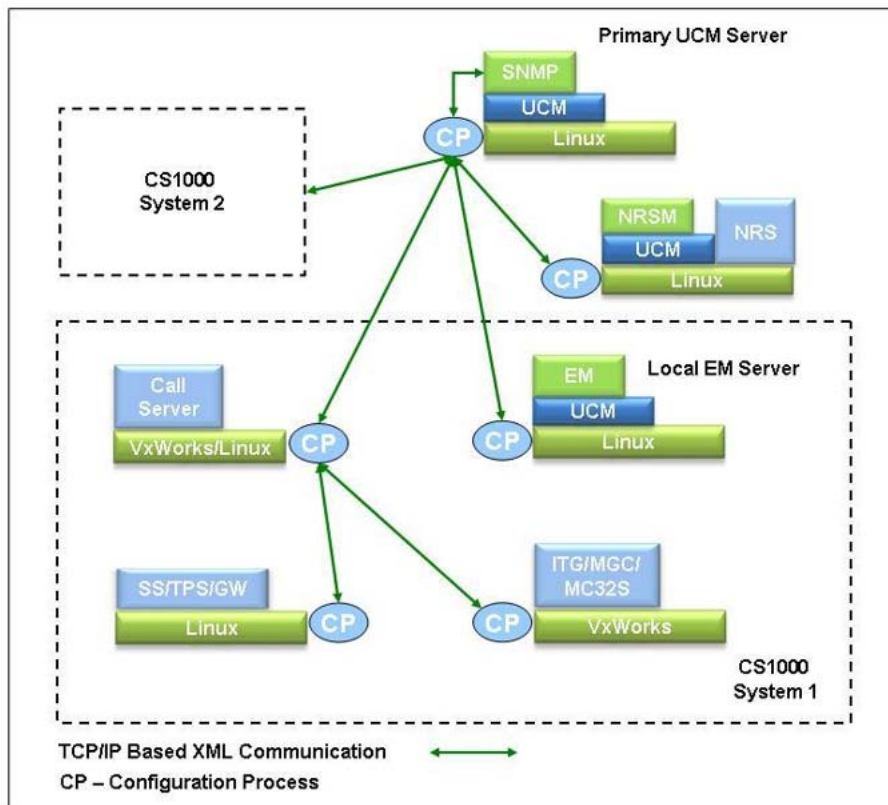
Figure 3: System propagation of SNMP parameters
