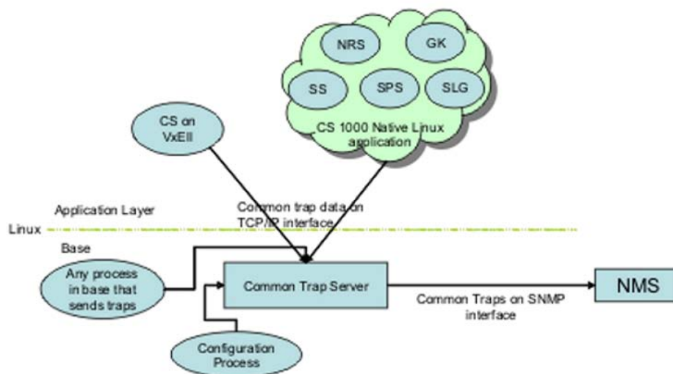
Figure 6: Common Trap Server in Linux
