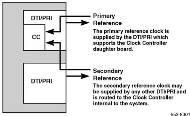
Figure 25: Clock controller primary and secondary tracking
