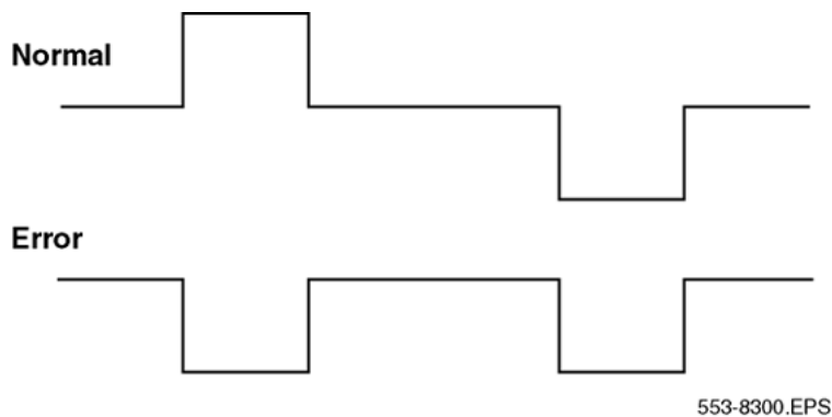
Figure 29: Bipolar violations
