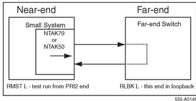
Figure 33: 2.0 Mb PRI link diagnostic (far-end loopback) test
