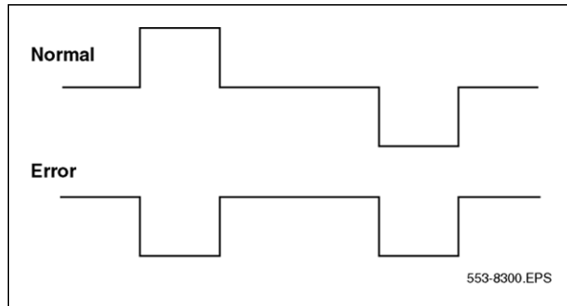
Figure 19 Bipolar violations
