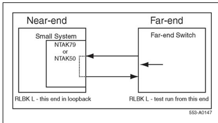
Figure 34 2.0 Mb PRI remote loopback test
