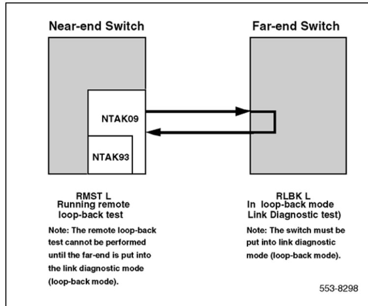
Figure 18 DTI/PRI link diagnostic and remote loopback tests
