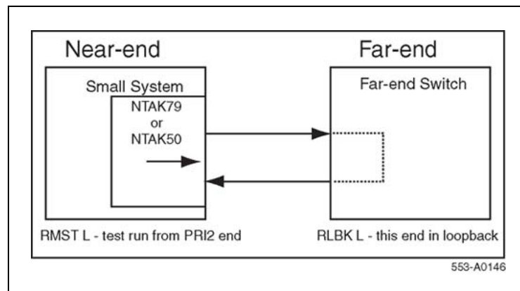
2.0 Mb PRI link diagnostic (far-end loopback) test
