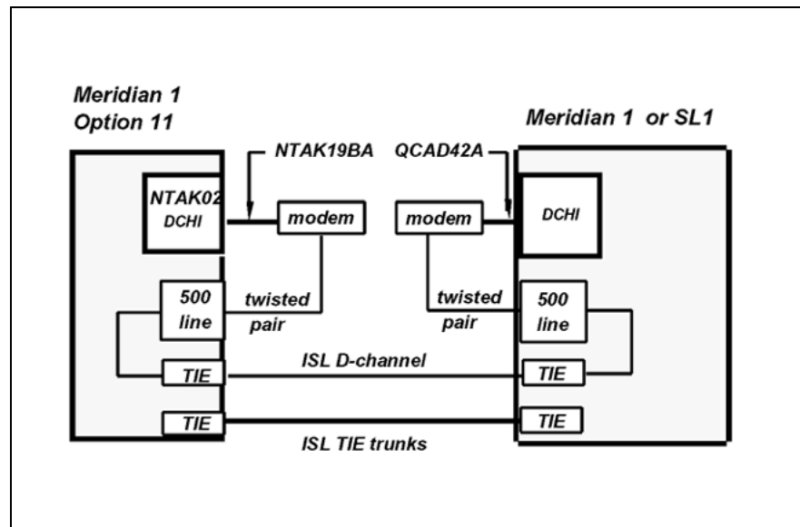
Figure 37 ISL in dedicated mode using dial-up modem
