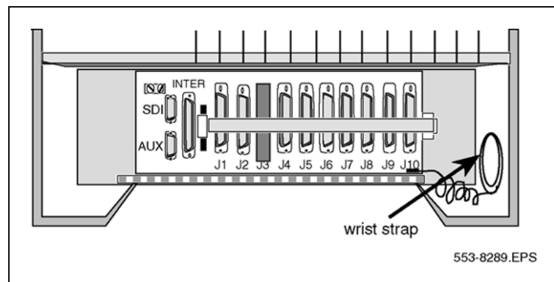
Figure 28 Wrist strap connection to the Small System
