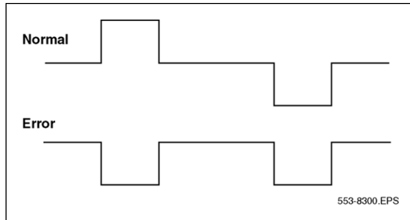
Figure 29 Bipolar violations
