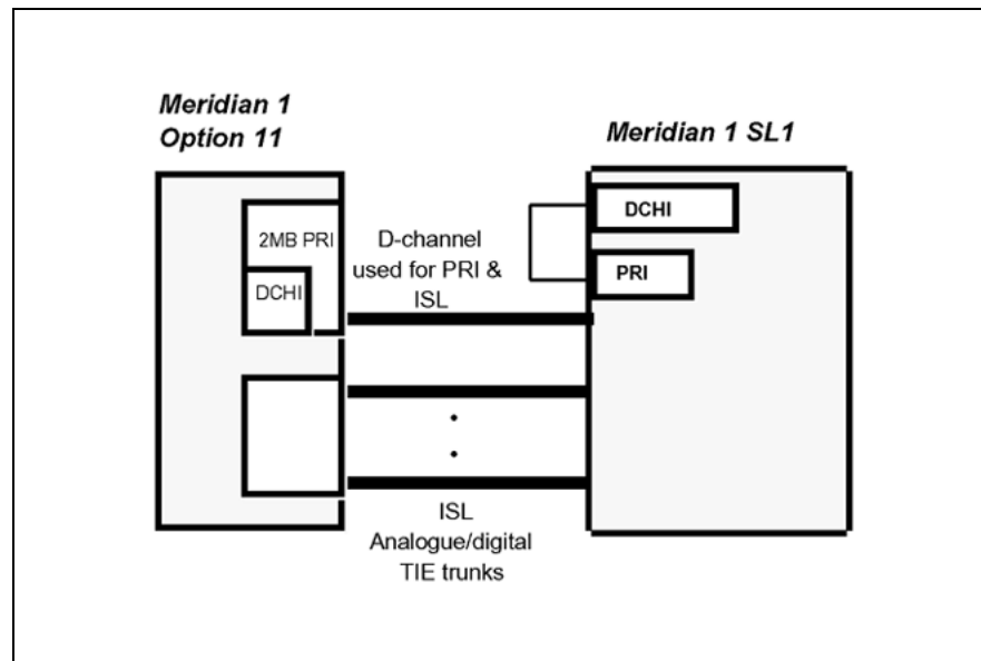
Figure 35 ISL in shared mode
