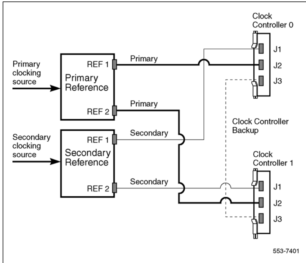
Figure 14 Clock controller primary and secondary tracking
