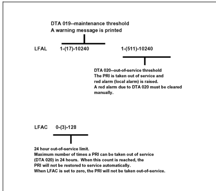
Figure 23 Frame alignment thresholds
