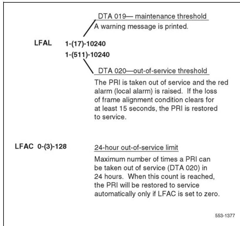
Figure 7 Frame alignment
