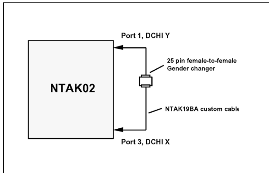
Figure 38 ISL back-to-back connection
