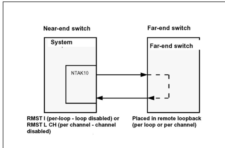
Figure 30 Near-end trunk loopback
