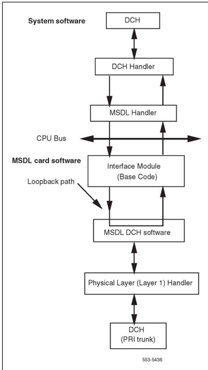
Figure 12 Local loopback test (NT6D80)
