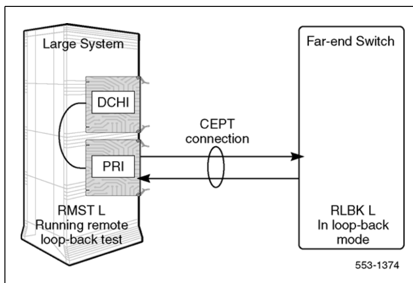
Figure 2 PRI link-diagnostic and remote loopback tests
