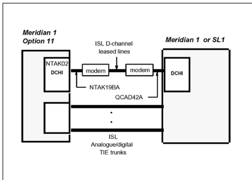
Figure 36 ISL in dedicated mode using leased line
