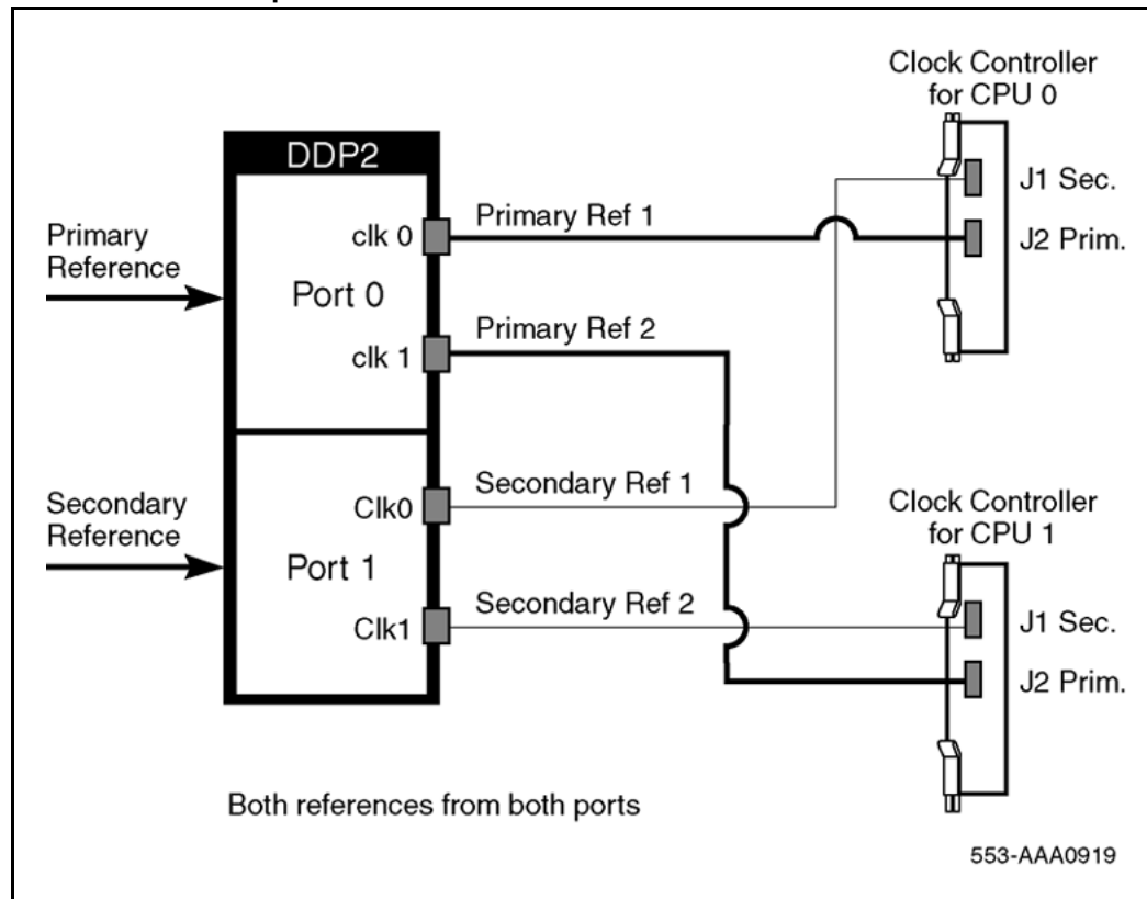
Figure 59 Clock Controller Option 4
