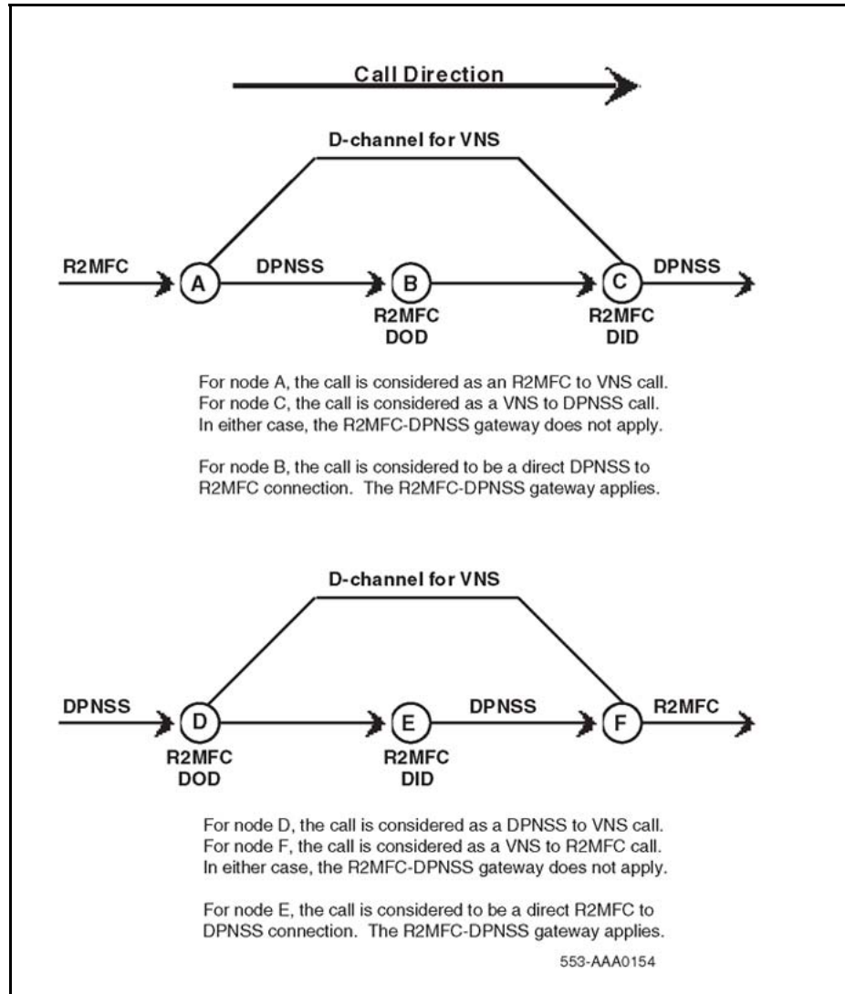
Figure 12 Applicability of R2MFC-DPNSS1 Gateway to VNS Calls
