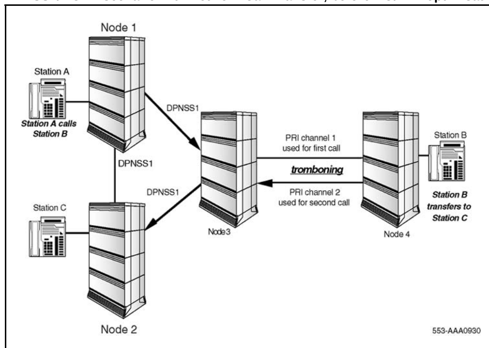
Figure 16 DPNSS1/MCDN scenario with Network Call Transfer, before RO/TAT optimisation
