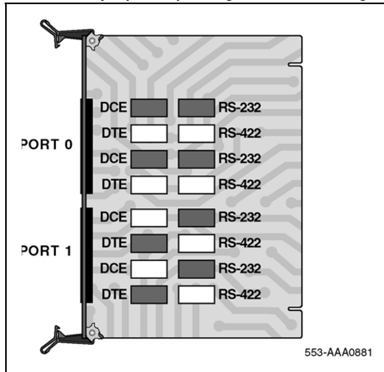
Figure 40 NT6D11AE/AF jumper strap settings for DPNSS1 configuration
