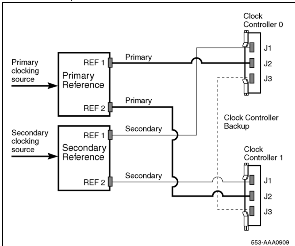
Figure 56 Clock Controller Option 1
