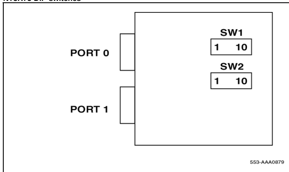
Figure 36 NT5K75 DIP switches
