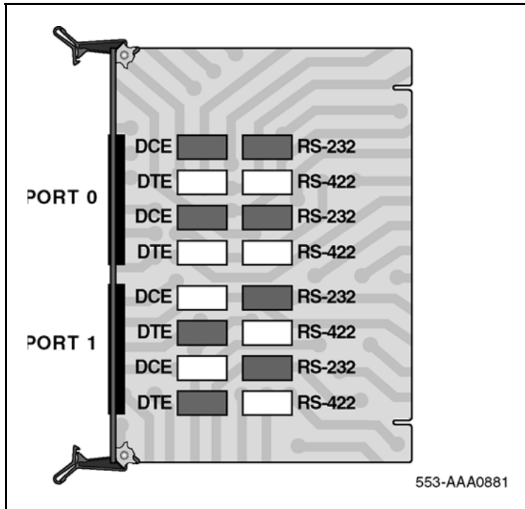
Figure 38 NT5K75 jumper straps for APNSS1 configuration
