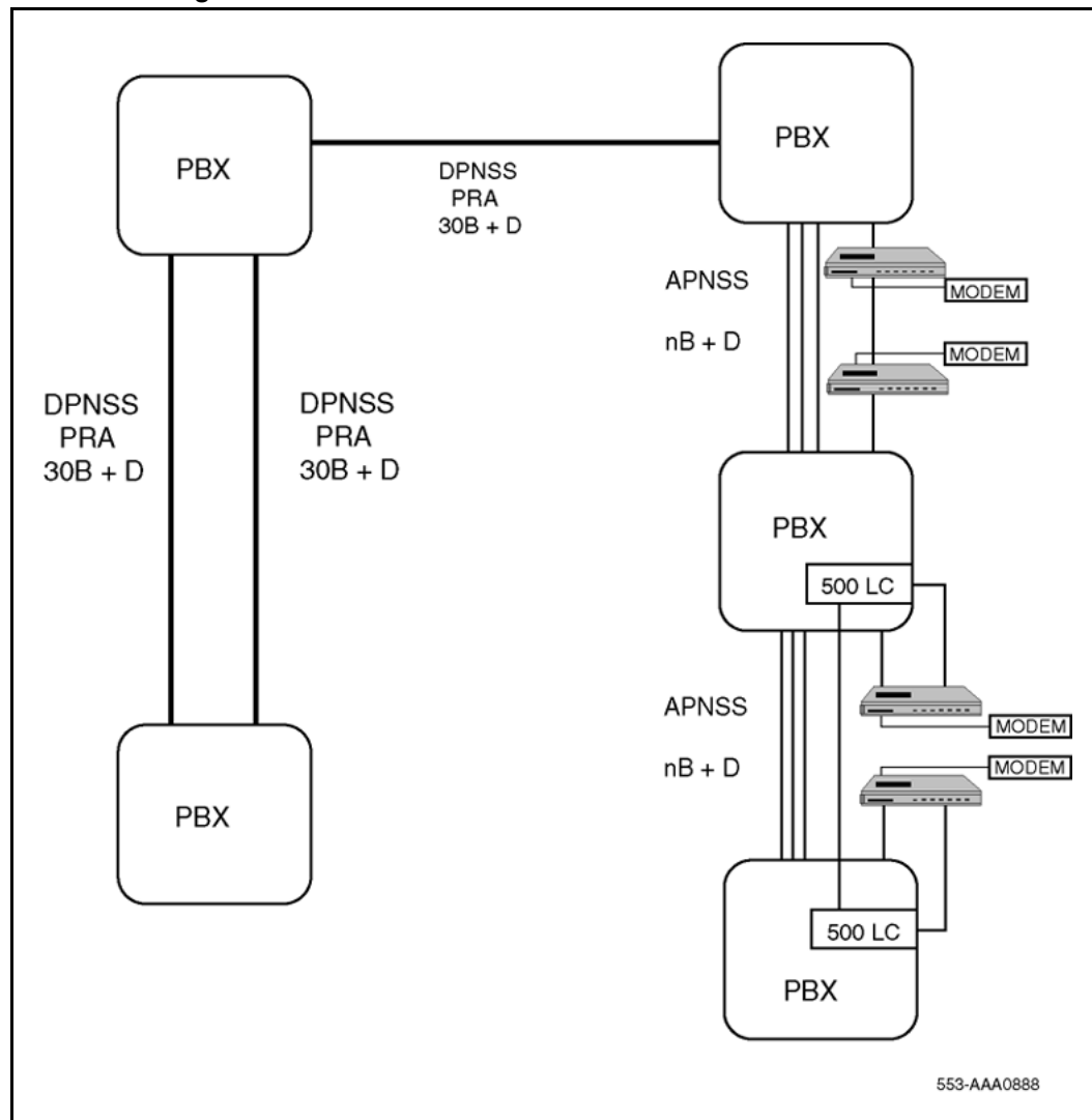
Figure 6 Channel configurations for DPNSS1 and APNSS
