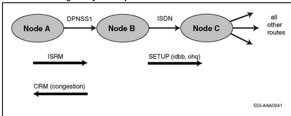
Figure 27 DPNSS1-to-ISDN gateway node operation
