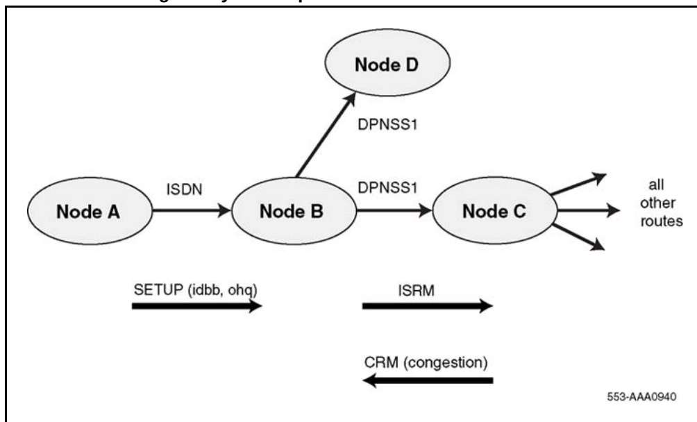
Figure 26 ISDN-to-DPNSS1 gateway node operation
