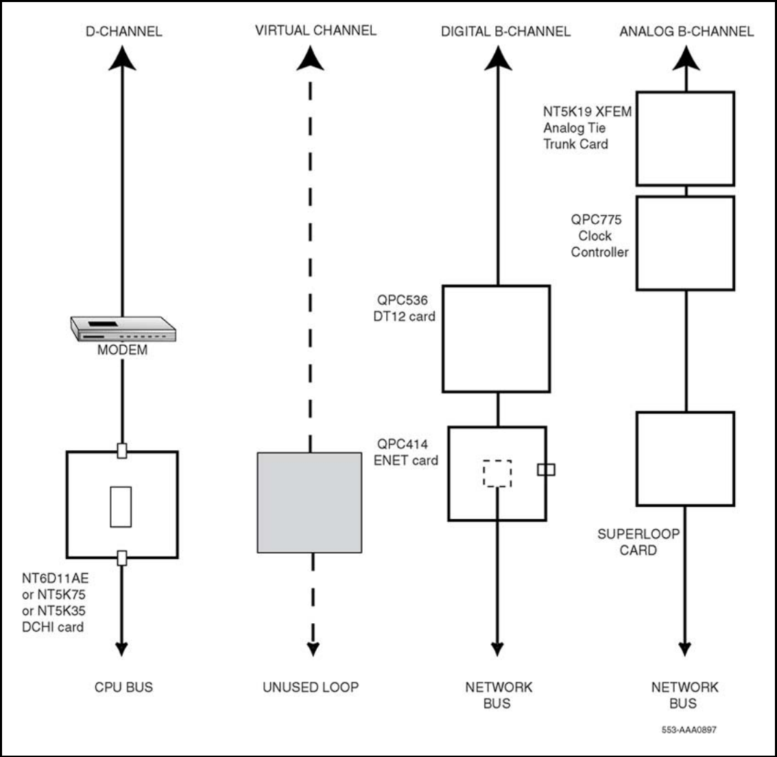
Figure 43 A typical APNSS hardware configuration
