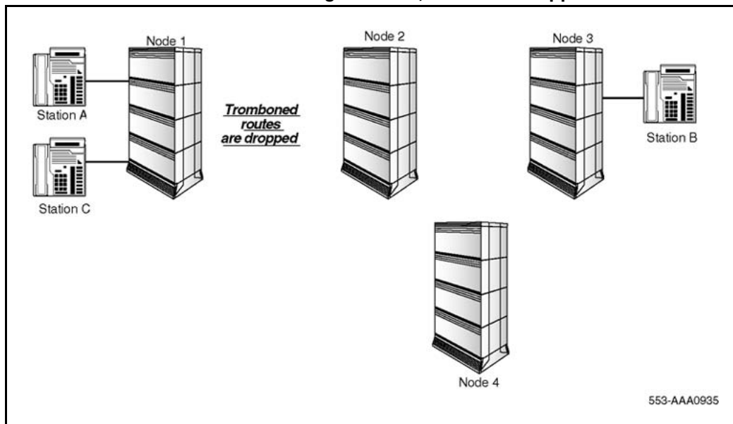
Figure 21 MCDN/DPNSS1 RO/TAT Interworking scenario, after TAT is applied
