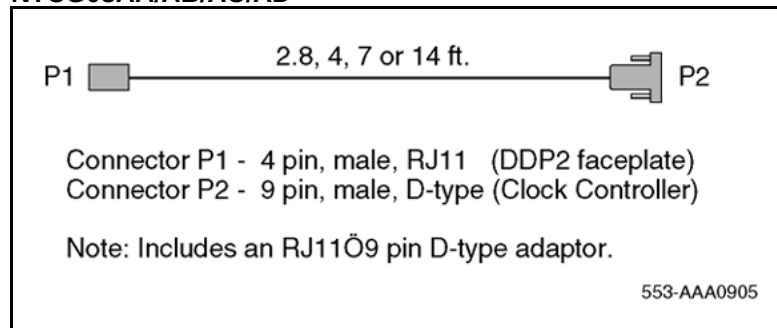
Figure 51 NTCG03AA/AB/AC/AD
