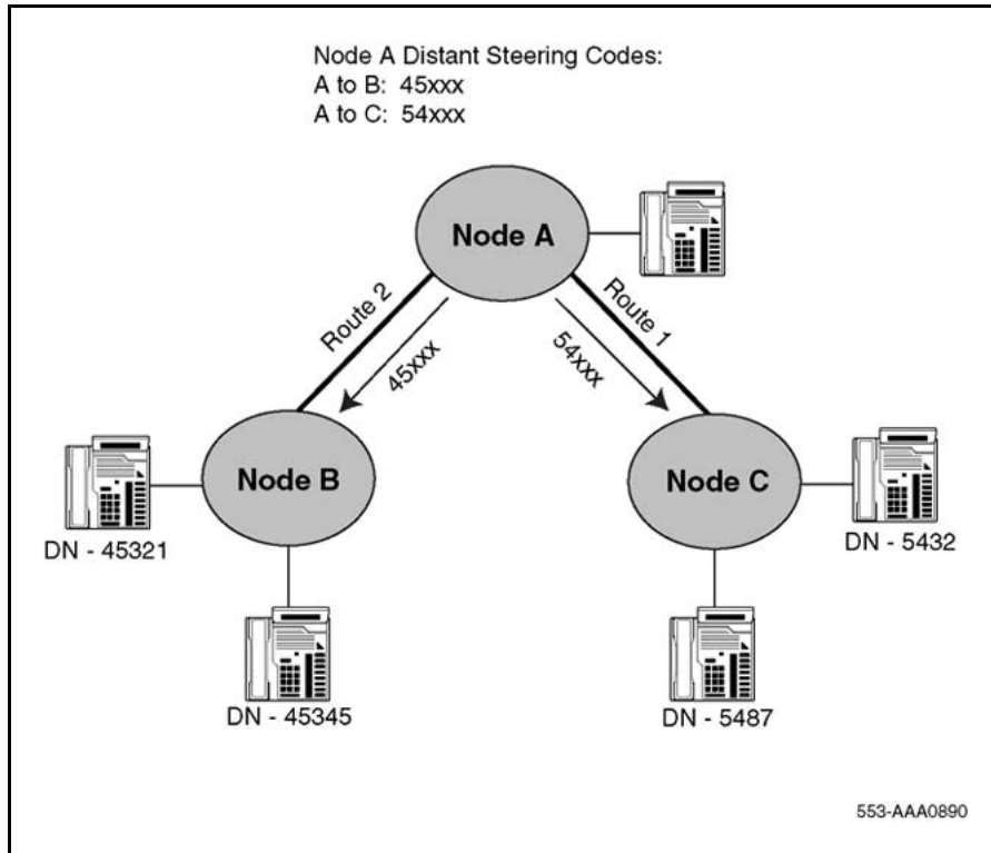
Figure 8 Distant Steering Code
