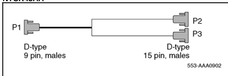
Figure 47 NTCK45AA
