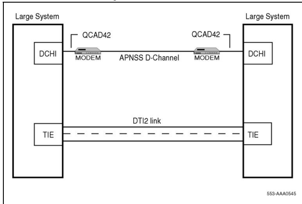
Figure 32 APNSS dedicated mode, using leased line
