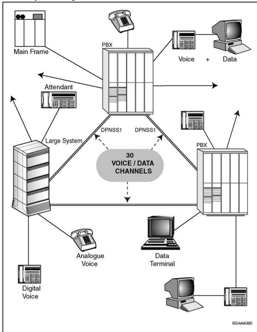
Figure 3 DPNSS1 system configuration
