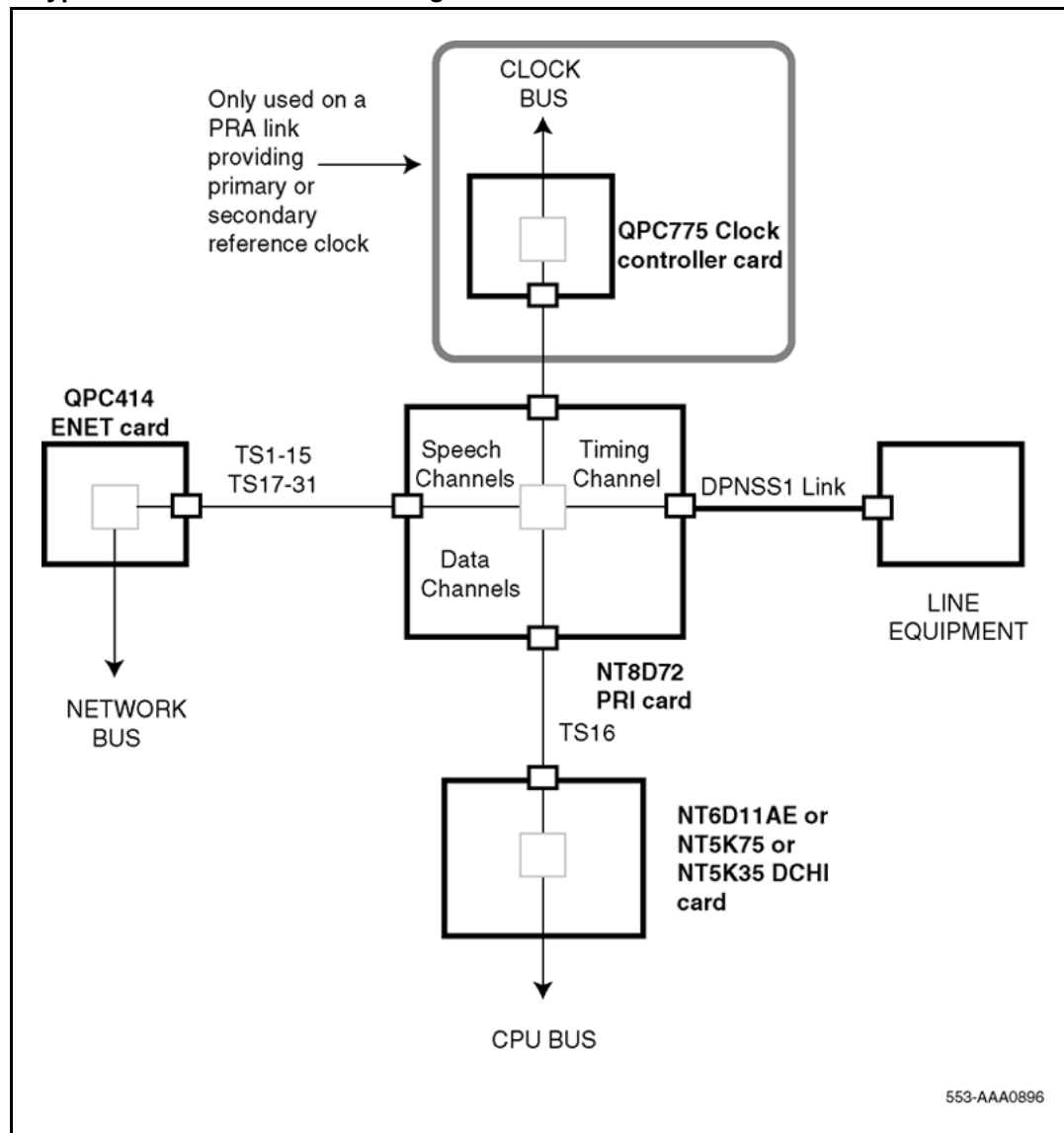
Figure 42 A typical DPNSS1 hardware configuration
