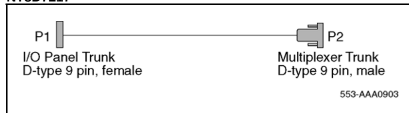
Figure 48 NT8D7217
