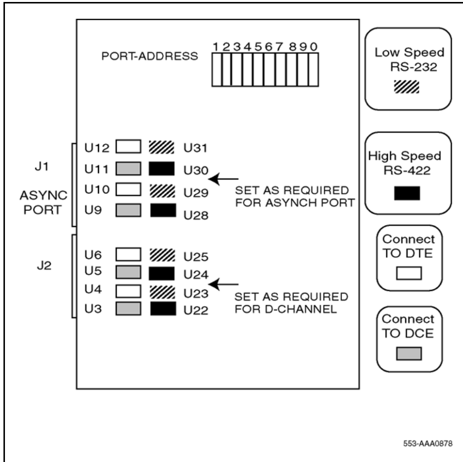
Figure 35 NT5K35 jumper strap settings
