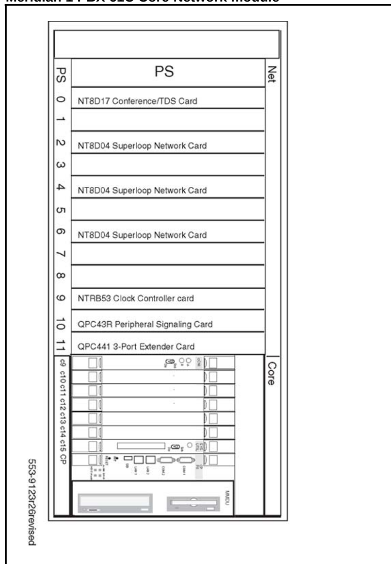
Figure 61 Meridian 1 PBX 61C Core Network module
