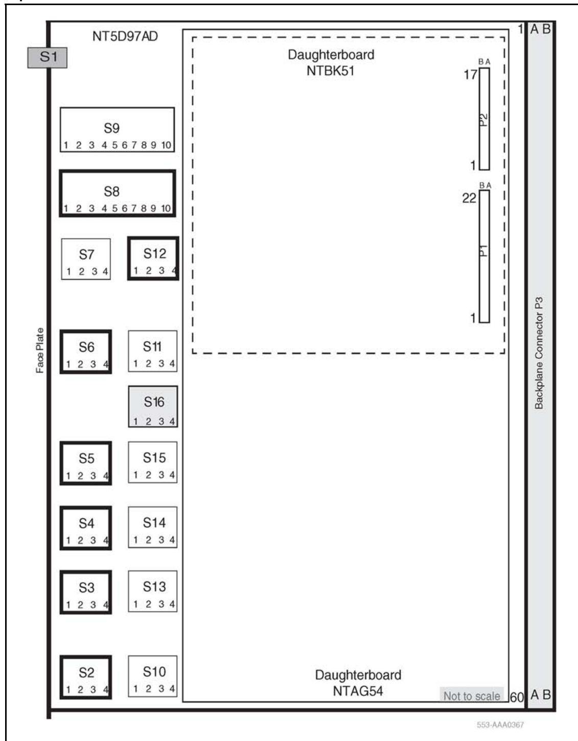
Figure 66 Dip switches locations
