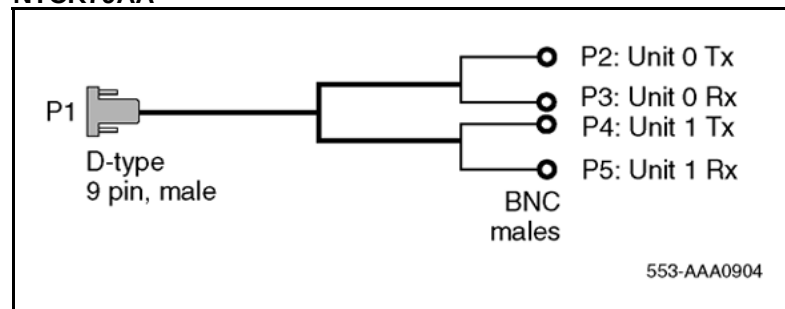
Figure 50 NTCK79AA
