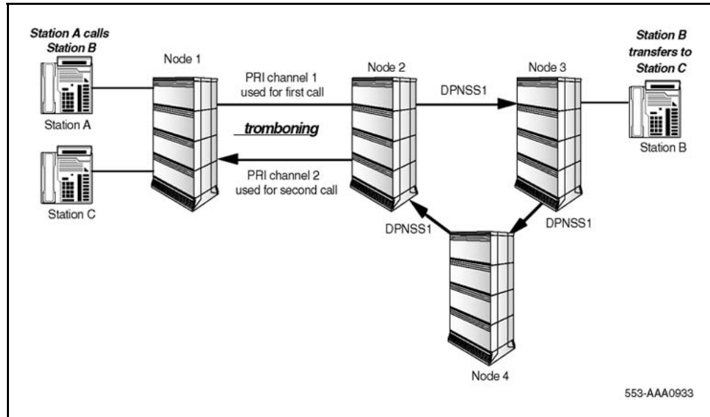
Figure 19 MCDN/DPNSS1 RO/TAT Interworking scenario, before RO has been applied
