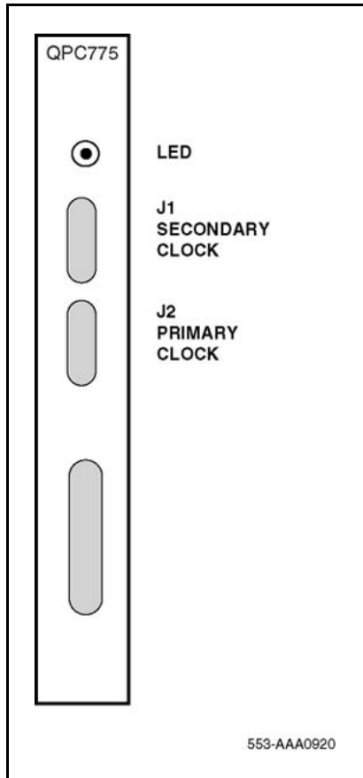
Figure 60 QPC775 Clock Controller faceplate layout
