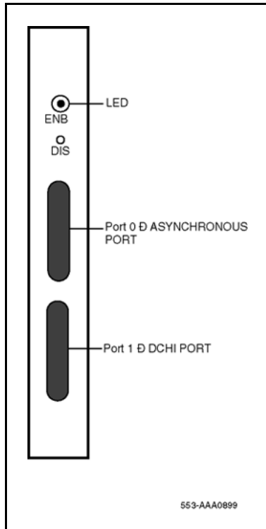
Figure 44 NT5K35, NT5K75, NT6D11AE/AF DCHI faceplate layout
