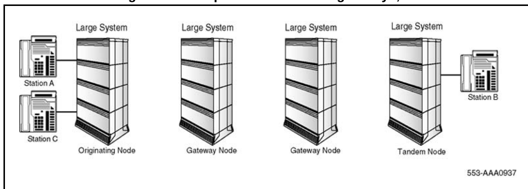
Figure 23 RO/TAT Interworking within multiple DPNSS1/MCDN gateways, after RO/TAT
