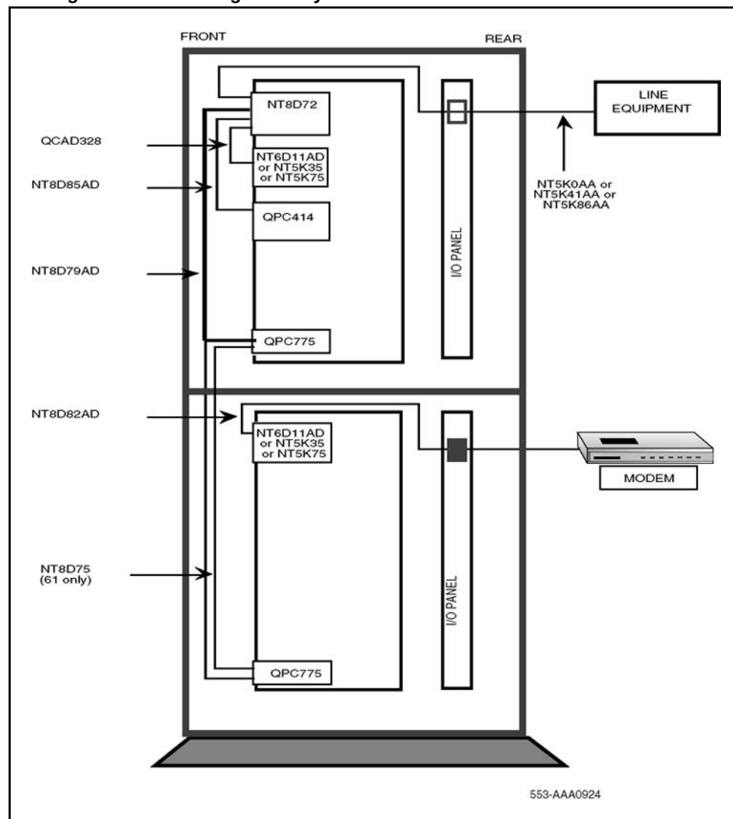
Figure 64 Cabling schematic for a generic system
