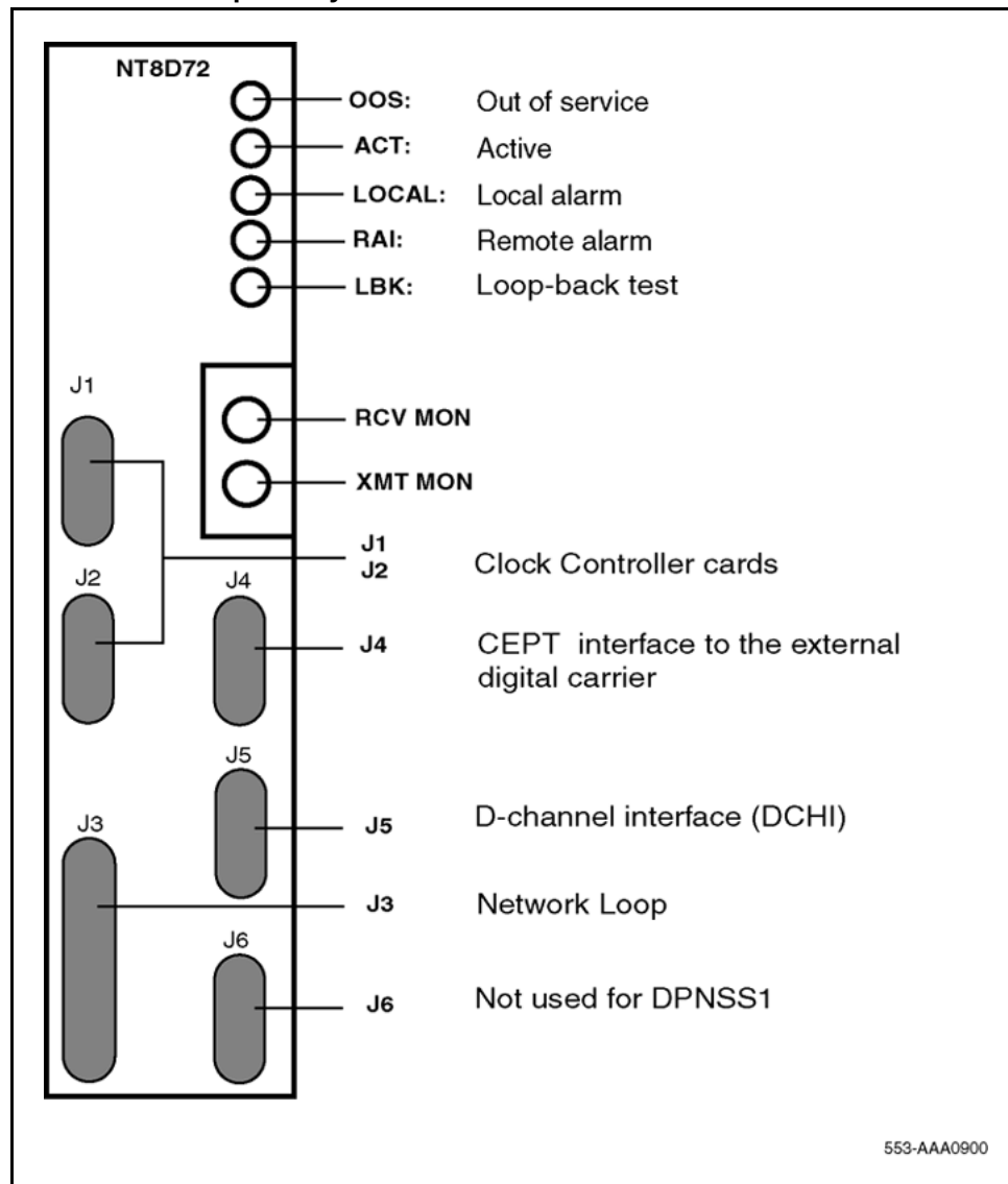
Figure 45 NT8D72 PRI faceplate layout
