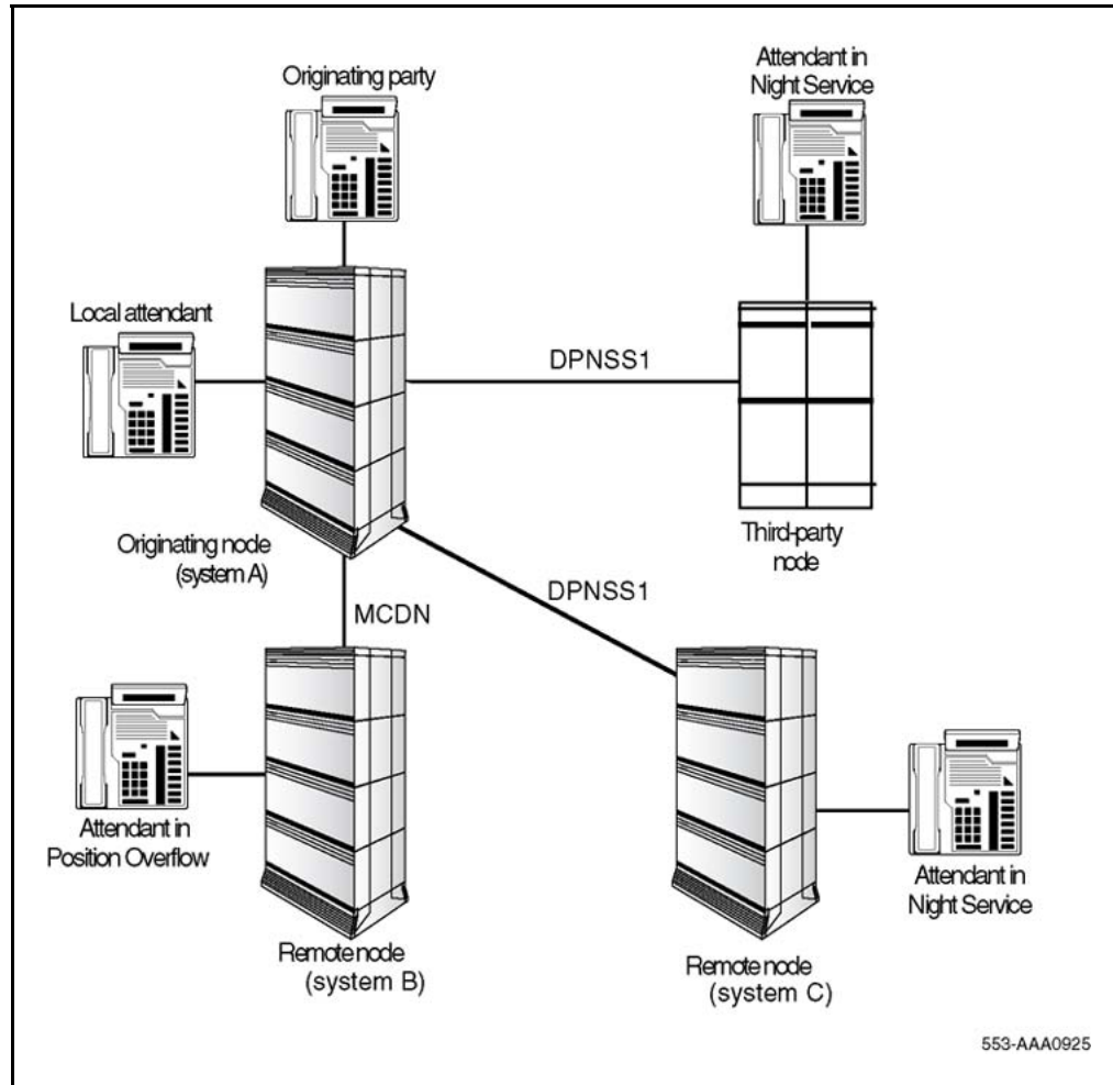
Figure 15 Example of DPNSS1 Night Service Diversion
