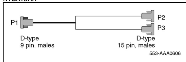
Figure 49 NTCK78AA
