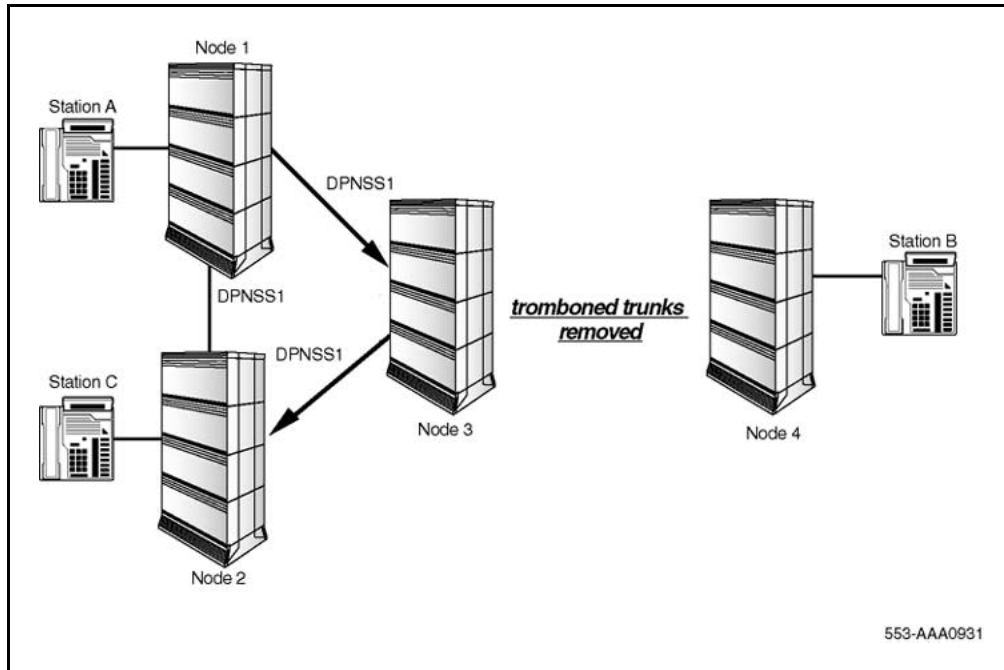
Figure 17 DPNSS1/MCDN RO/TAT Interworking scenario, after TAT has been applied
