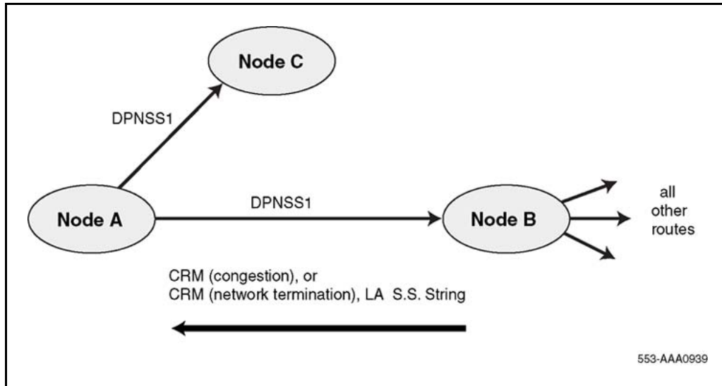
Figure 25 Originating node operation
