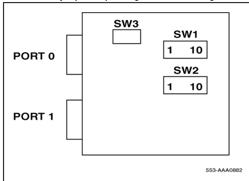
Figure 41 NT6D11AE/AF jumper strap settings for APNSS configuration
