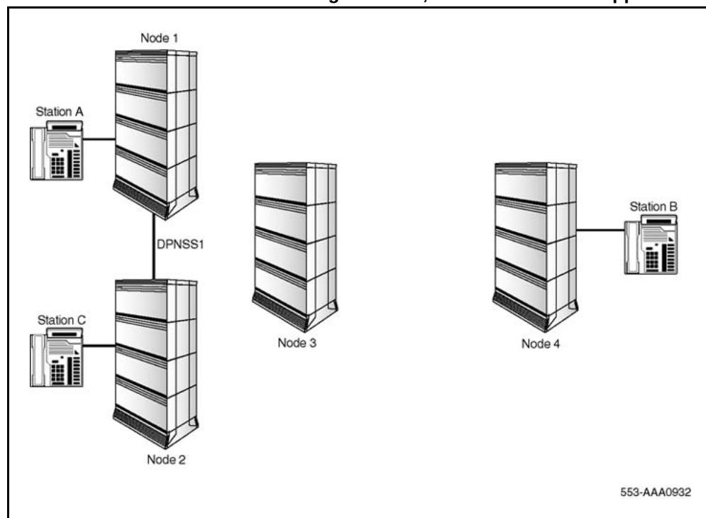
Figure 18 DPNSS1/MCDN RO/TAT Interworking scenario, after RO has been applied
