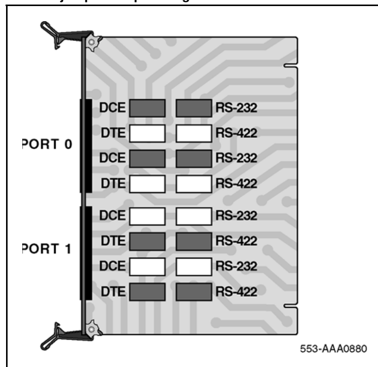
Figure 37 NT5K75 jumper strap settings for DPNSS1
