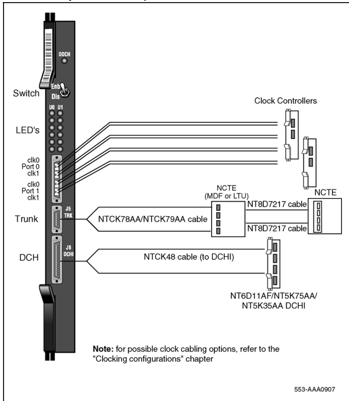
Figure 53 DDP2 cable for systems with an I/O panel
