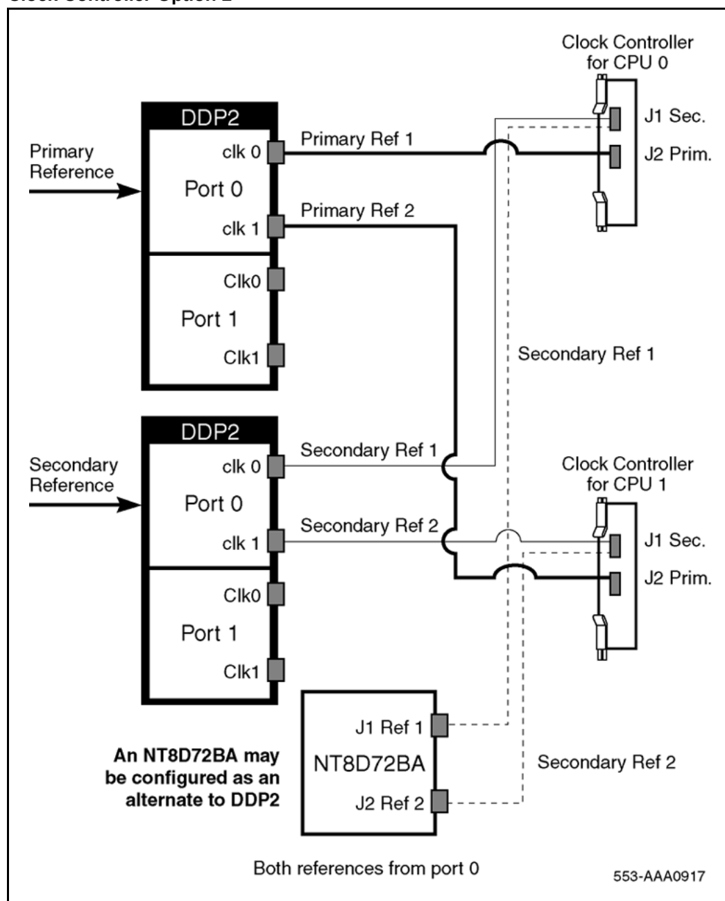
Figure 57 Clock Controller Option 2
