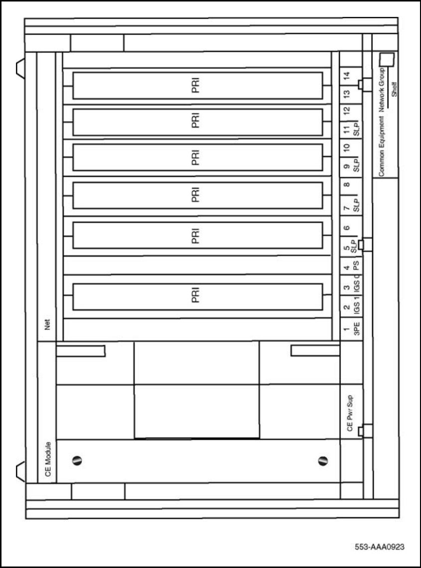
Figure 63 Network Expansion module with six PRI cards
