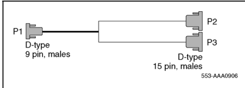
Figure 52 NTCK46AA/AB/AC/AD
