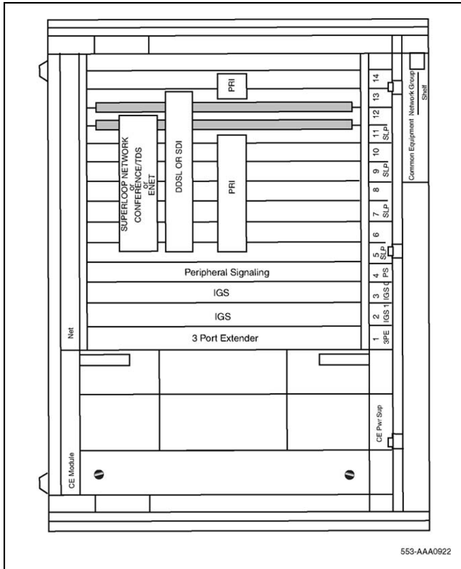
Figure 62 CS 1000M MG and Meridian 1 PBX 81C Network module
