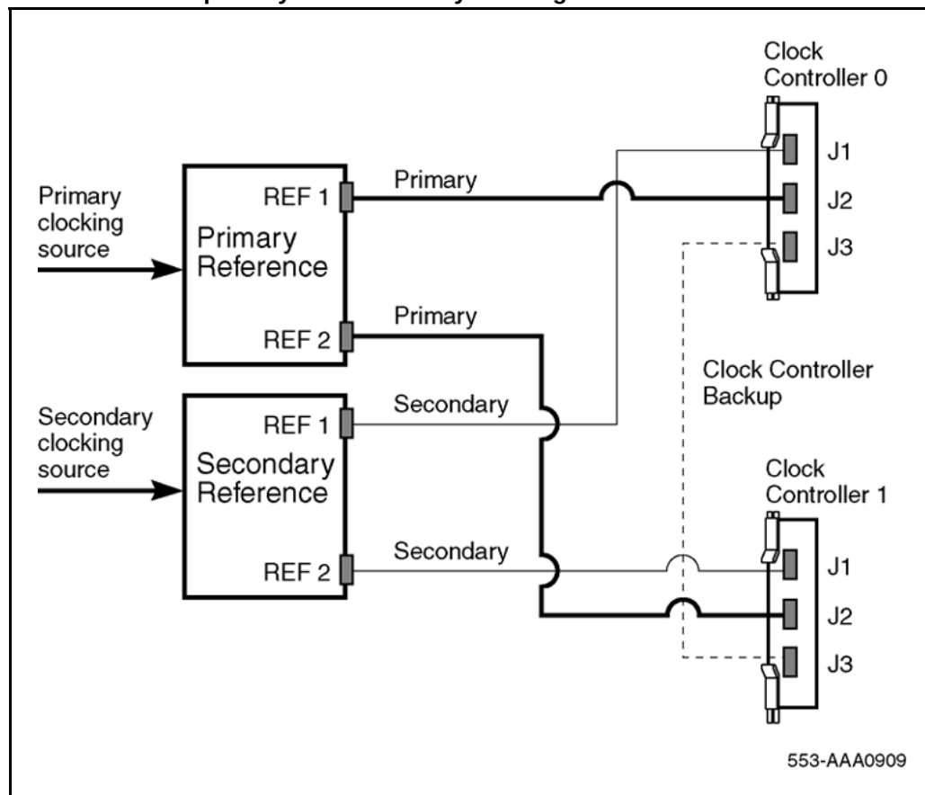
Figure 55 Clock Controller primary and secondary tracking
