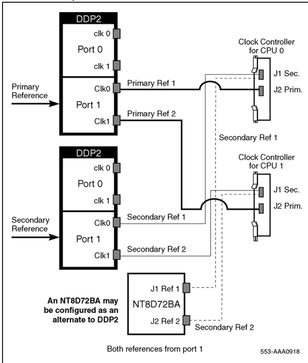
Figure 58 Clock Controller Option 3
