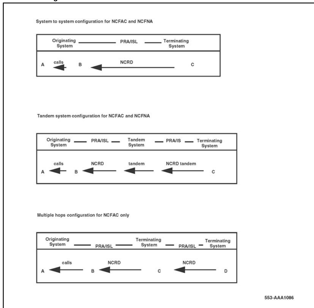
Figure 18 Network configurations for NCFAC and NCFNA
