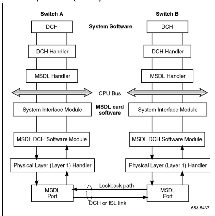
Figure 133 Remote loopback tests (NT6D80)
