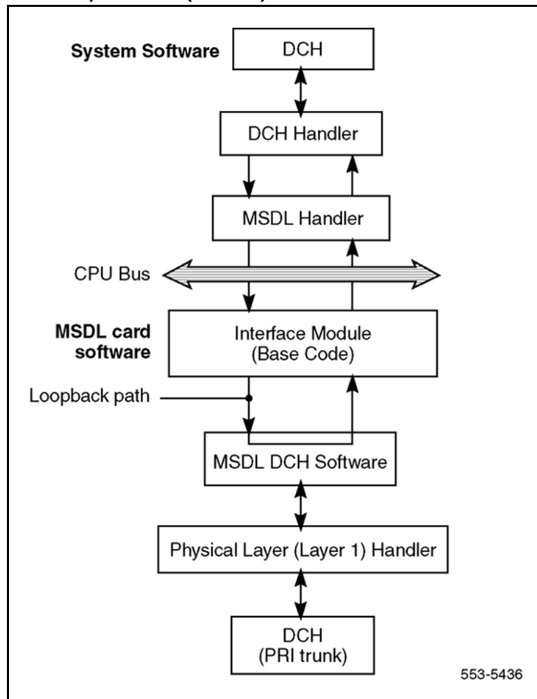
Figure 132 Local loopback test (NT6D80)
