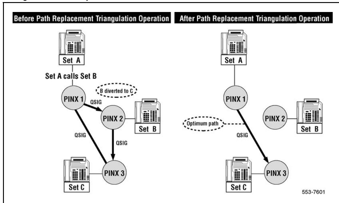
Figure 32 Triangulation Path Replacement
