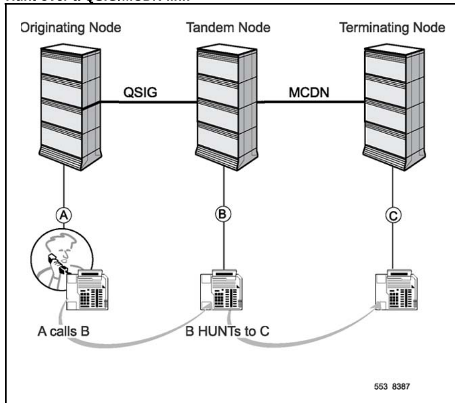
Figure 26 Hunt over a QSIG/MCDN link
