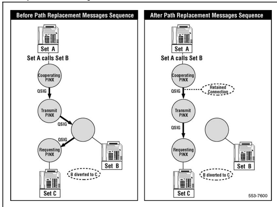
Figure 34 Path Replacement Retaining Part of Old Connection
