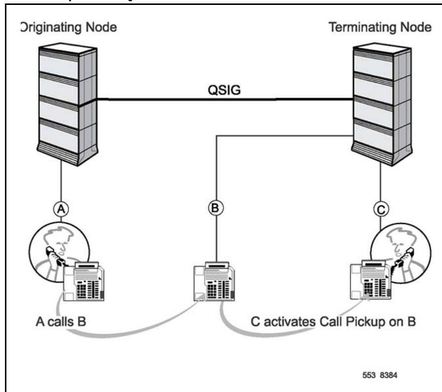
Figure 19 Call Pickup over a QSIG link
