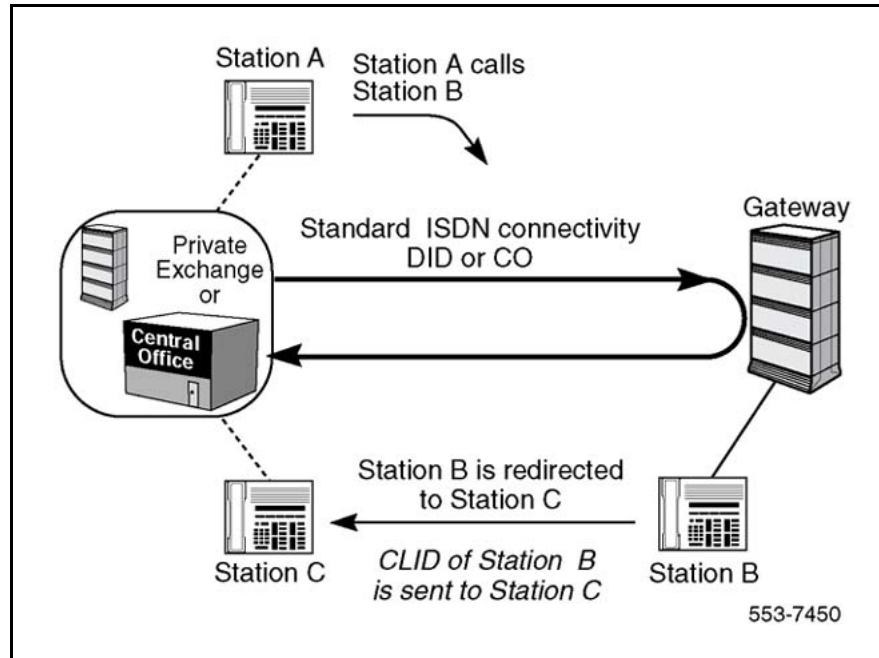
Figure 4 Incoming EuroISDN call redirected back to the Public Network/PBX
