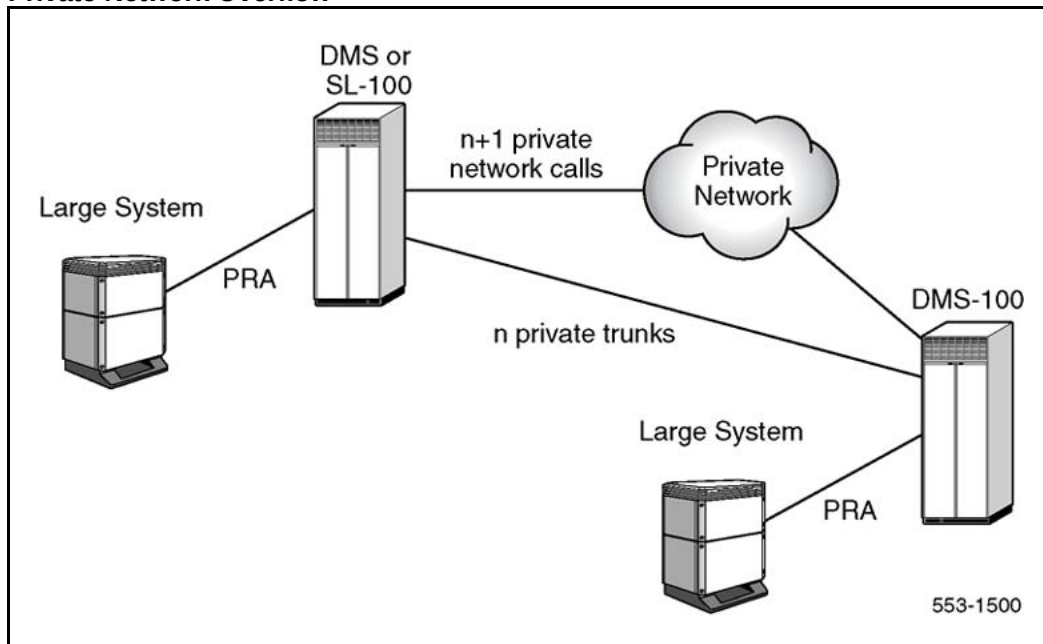
Figure 3 Private Network Overflow
