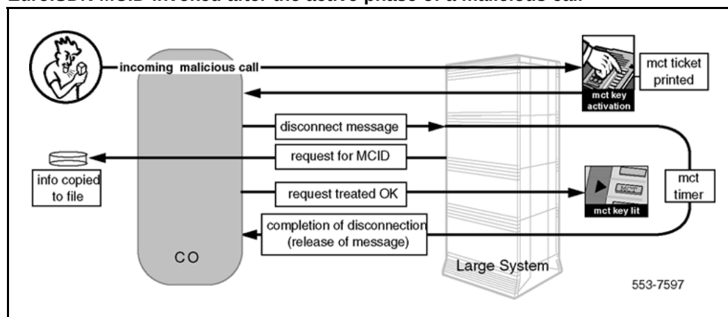
Figure 11 EuroISDN MCID invoked after the active phase of a malicious call
