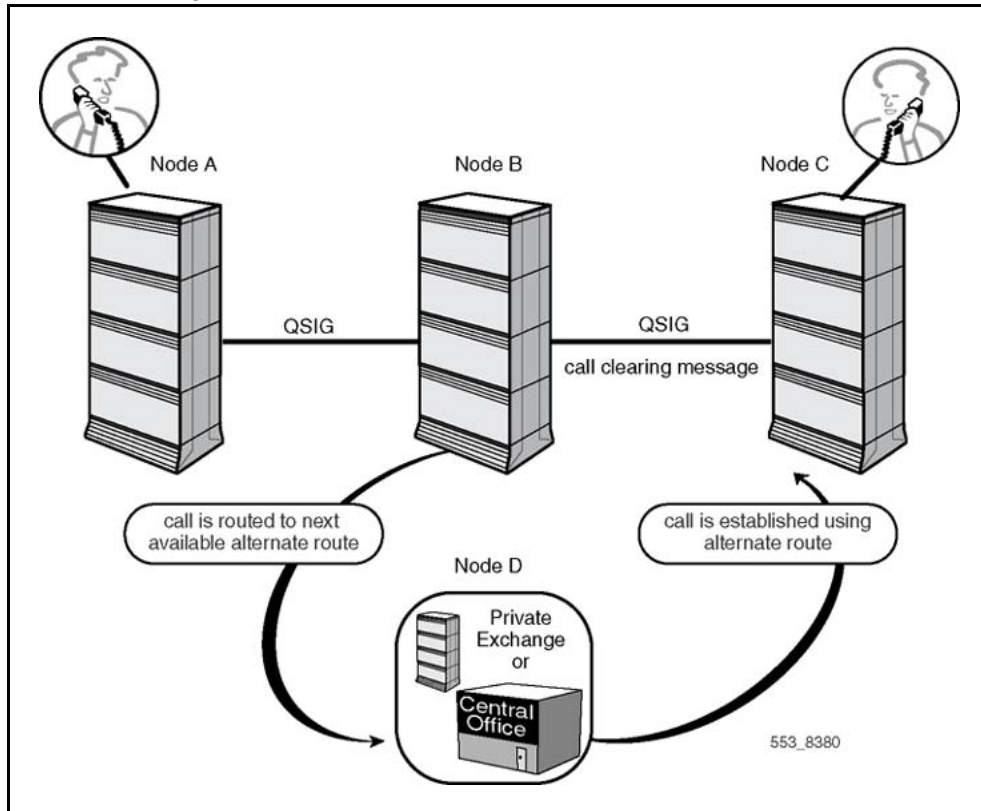
Figure 14 Transit node operation
