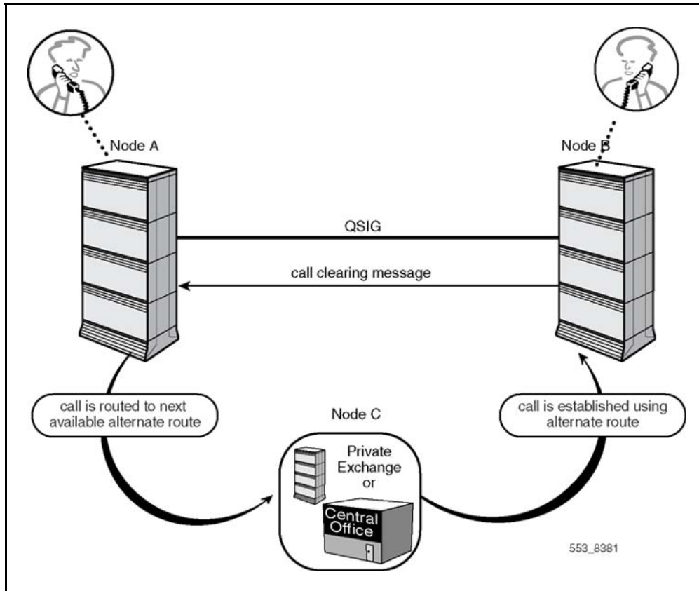
Figure 15 Originating node operation
