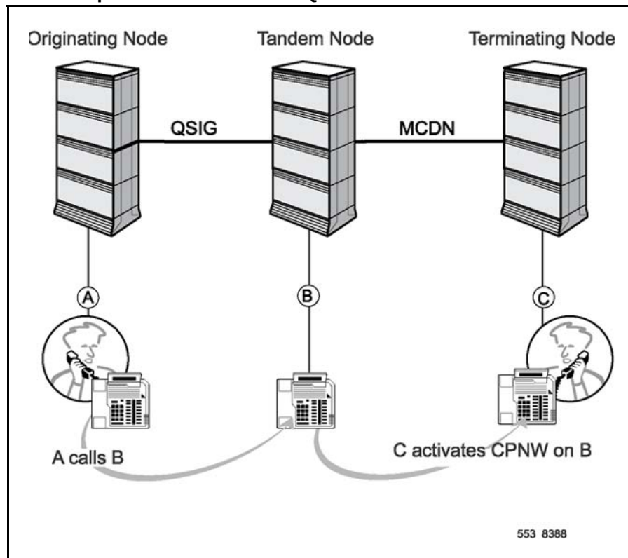
Figure 27 Call Pickup Network Wide over a QSIG/MCDN link
