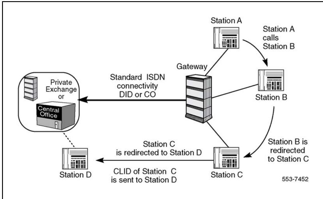
Figure 6 Internal call (stand-alone case) redirected to the Public Network/PBX
