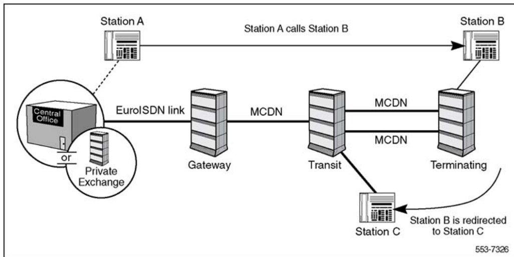
Figure 8 EuroISDN calling scenario before Trunk Optimization is applied
