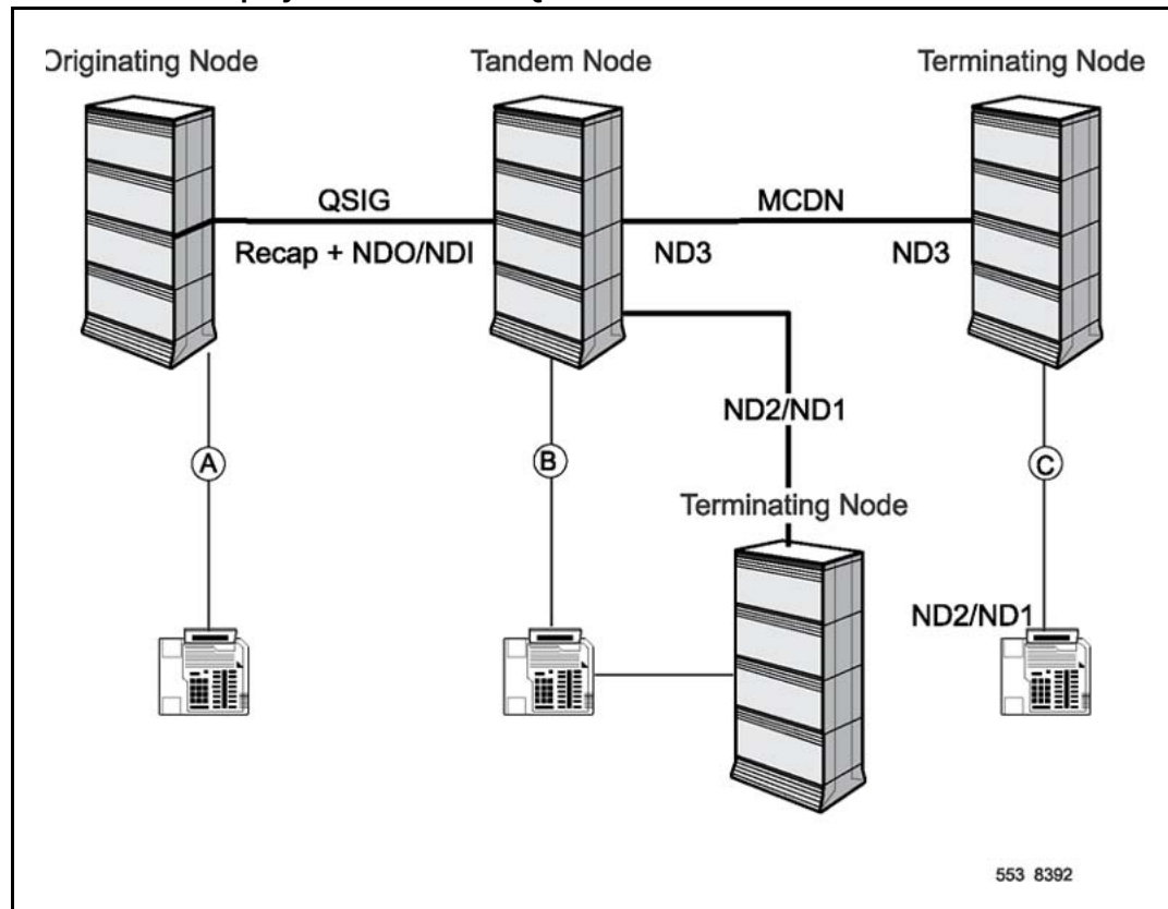
Figure 31 MCDN Name Display features over a QSIG/MCDN link
