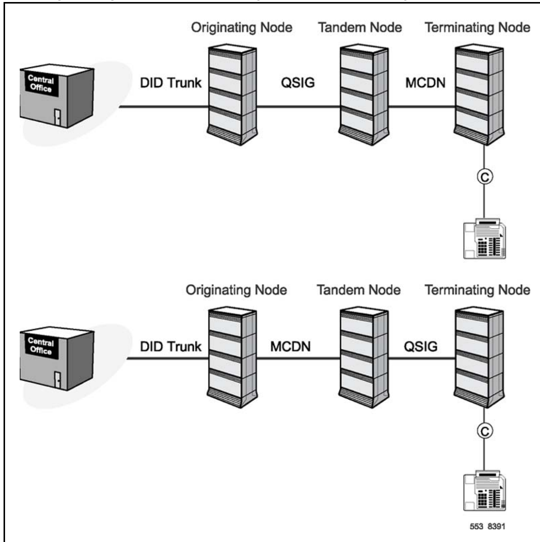
Figure 30 Incoming DID Digit Conversion over a QSIG/MCDN, or MCDN/QSIG link
