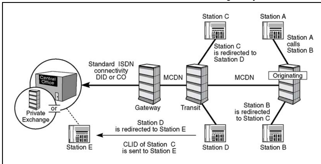
Figure 7 MCDN call redirected to the Public Network/PBX from a non-gateway node
