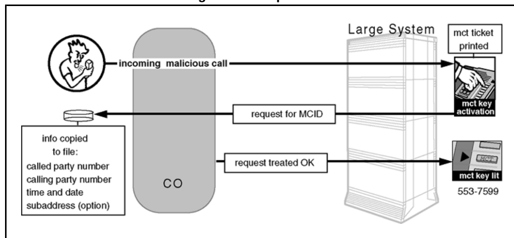
Figure 10 EuroISDN MCID invoked during the active phase of a malicious call
