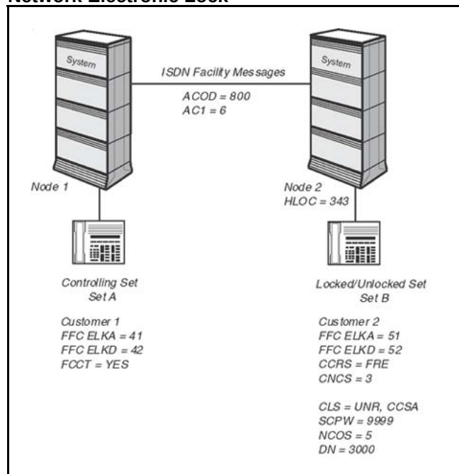
Figure 1 Network Electronic Lock
