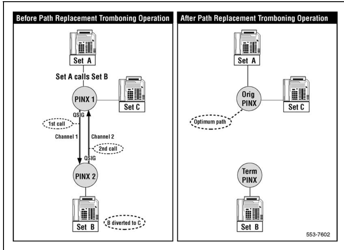
Figure 33 Tromboning Path Replacement
