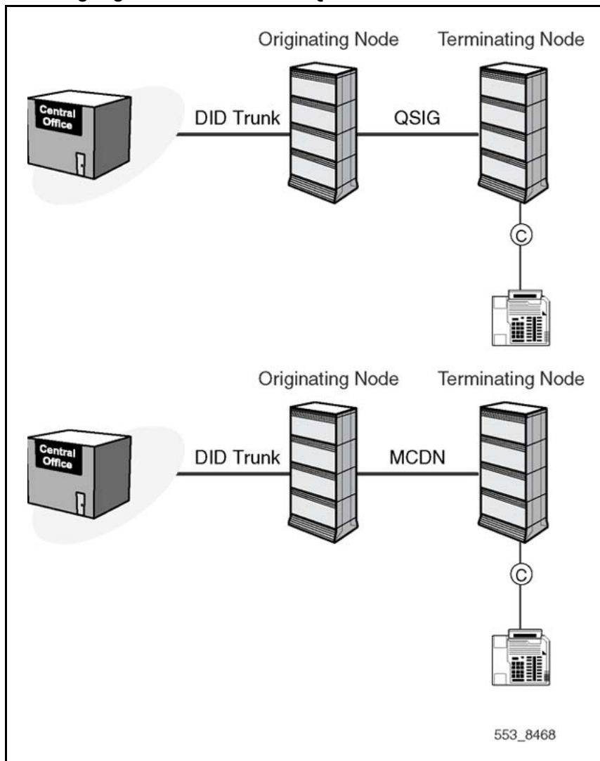
Figure 24 Incoming Digit Conversion over a QSIG link
