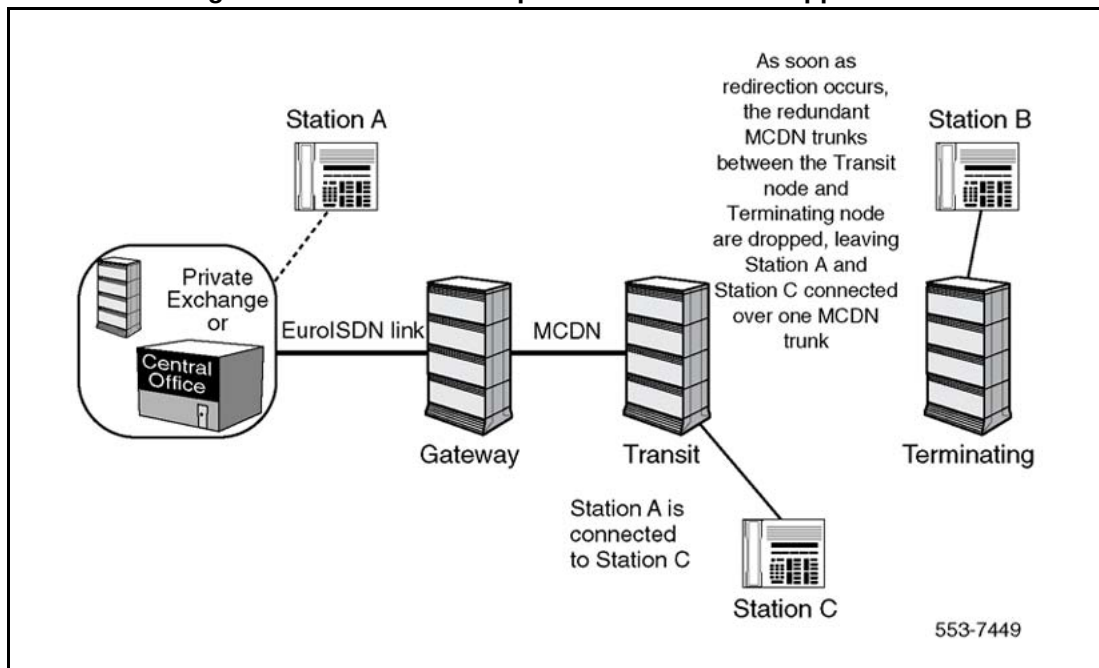
Figure 9 EuroISDN calling scenario after Trunk Optimization has been applied
