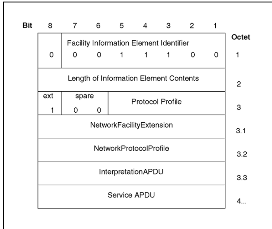
Figure 16 Facility IE layout
