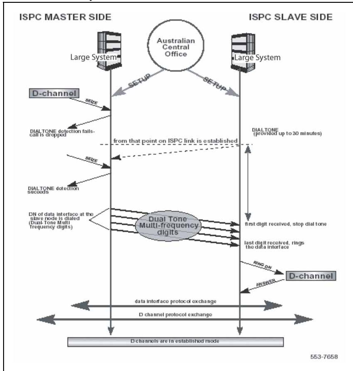
Figure 35 Mechanism Used to Synchronize Data Interfaces
