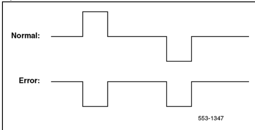
Figure 1 Bipolar violations
