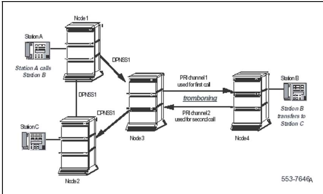
Figure 66 DPNSS1/MCDN scenario with Network Call Transfer, before RO/TAT optimisation
