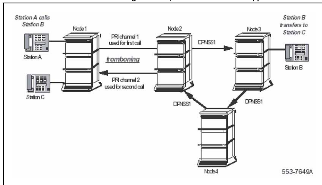
Figure 69 MCDN/DPNSS1 RO/TAT Interworking scenario, before RO has been applied
