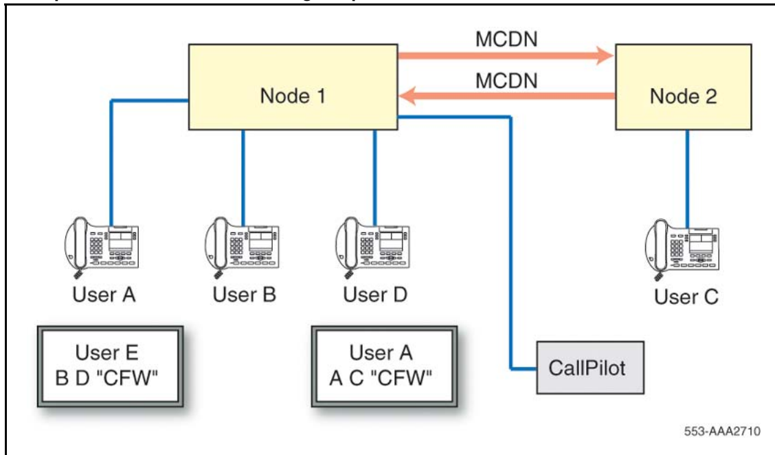
Figure 60 Example of Trunk Anti-Tromboning in operation and ARDN = YES
