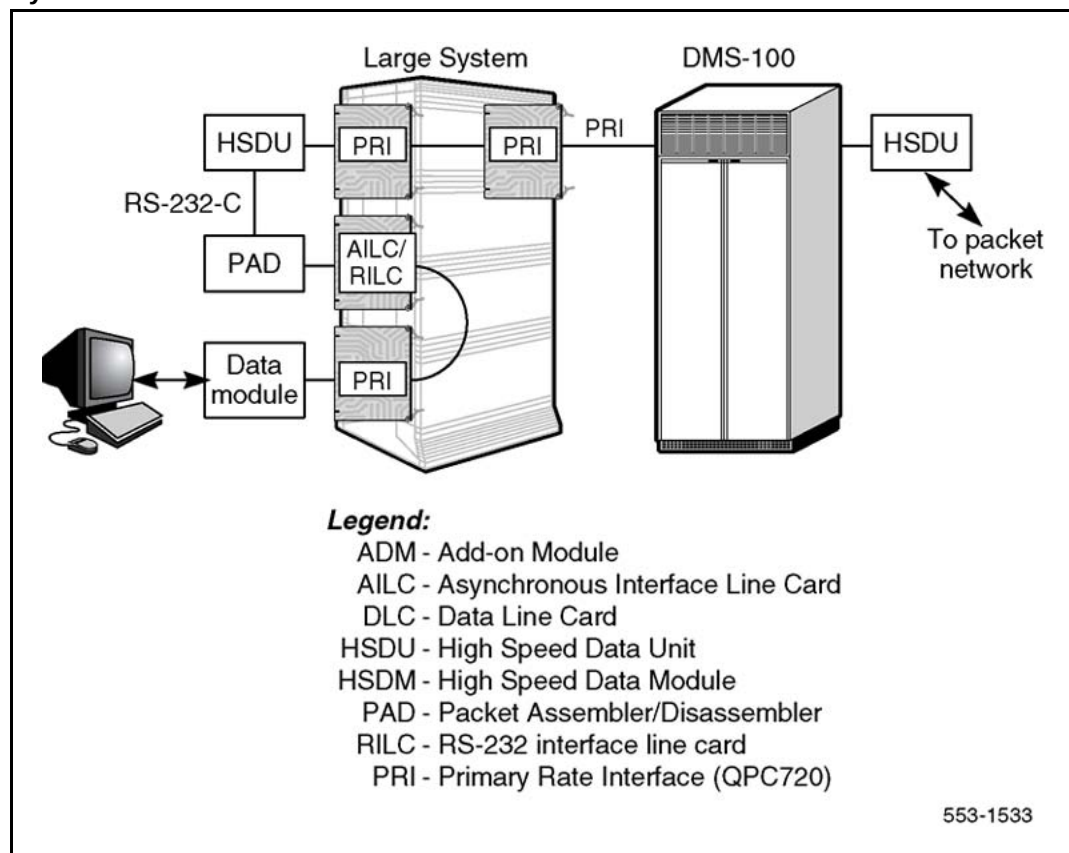
Figure 63 System PRI to DMS-100 Data Packet Network
