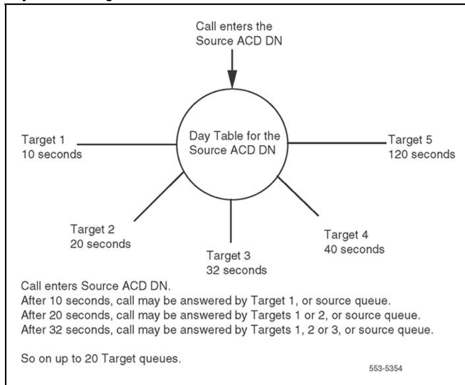
Figure 12 Day table routing
