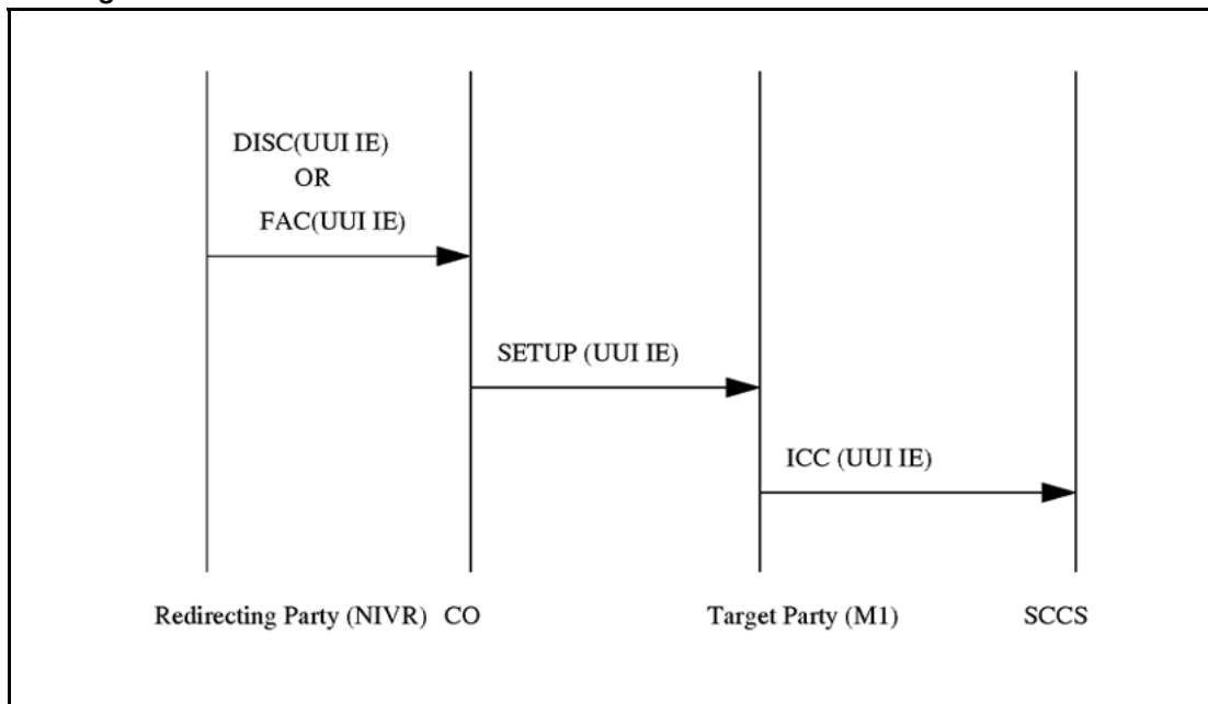
Figure 6 Message flow for UUS call scenario
