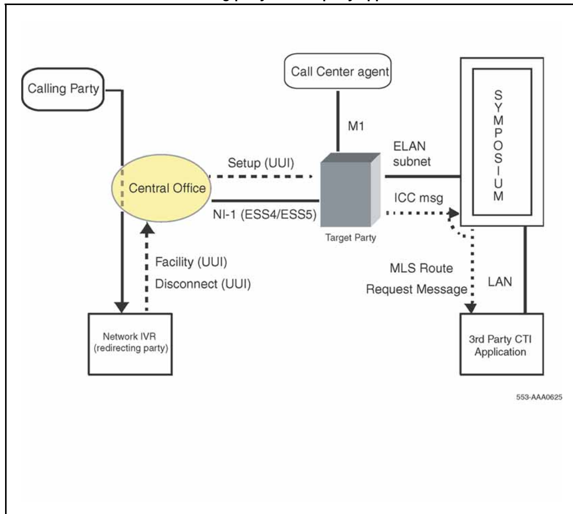
Figure 5 User-to-User data flow from calling party to third-party application
