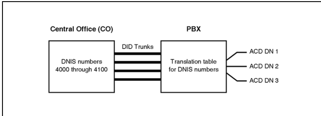
Figure 9 Incoming Digit Conversion
