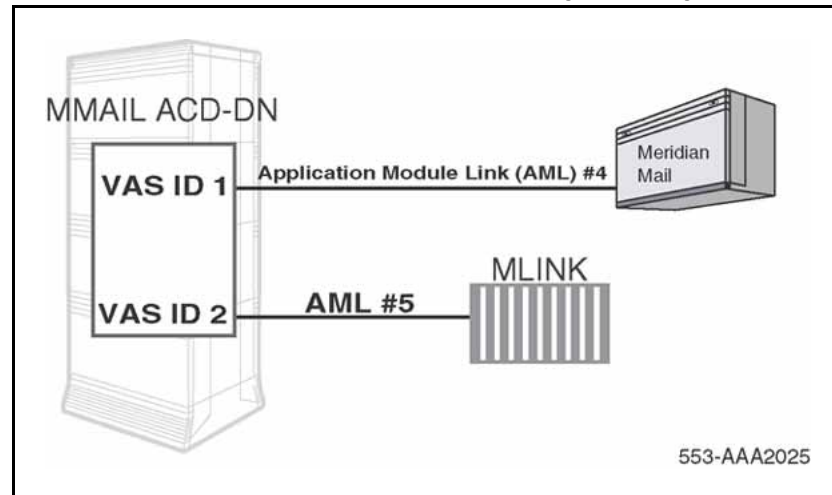
Figure 10 Meridian Mail and Meridian Link connectivity to the system
