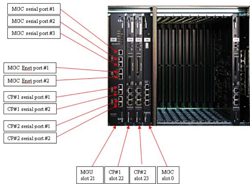
Figure 198: NTC314AAE6 utility card
