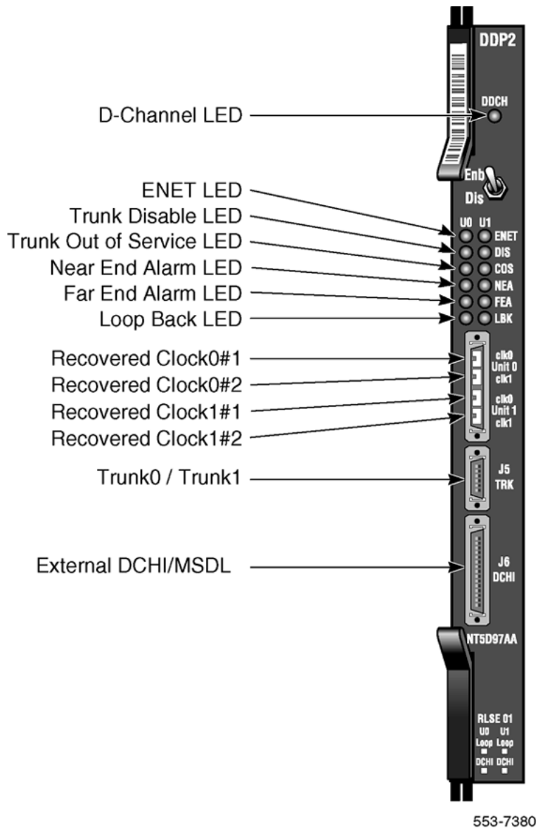
Figure 73: NT5D97 faceplate
