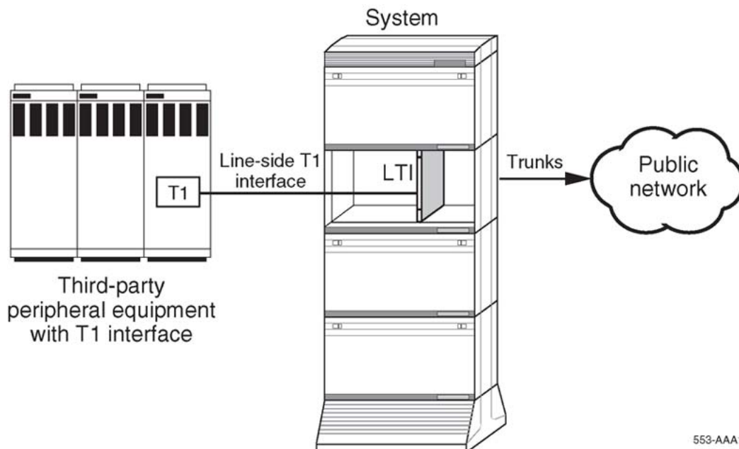
Figure 41: Lineside T1 interface connection to IPE
