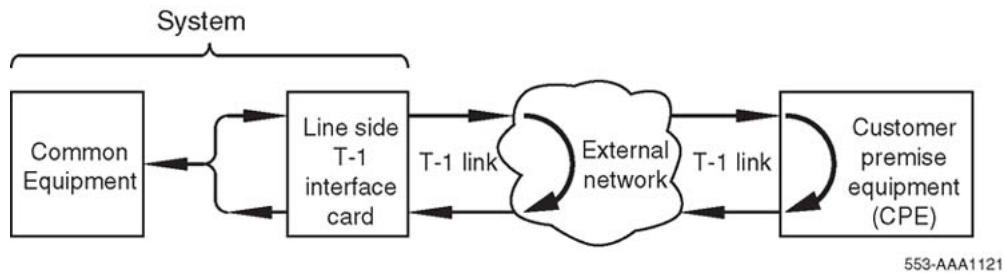
Figure 39: MMI external loopback test
