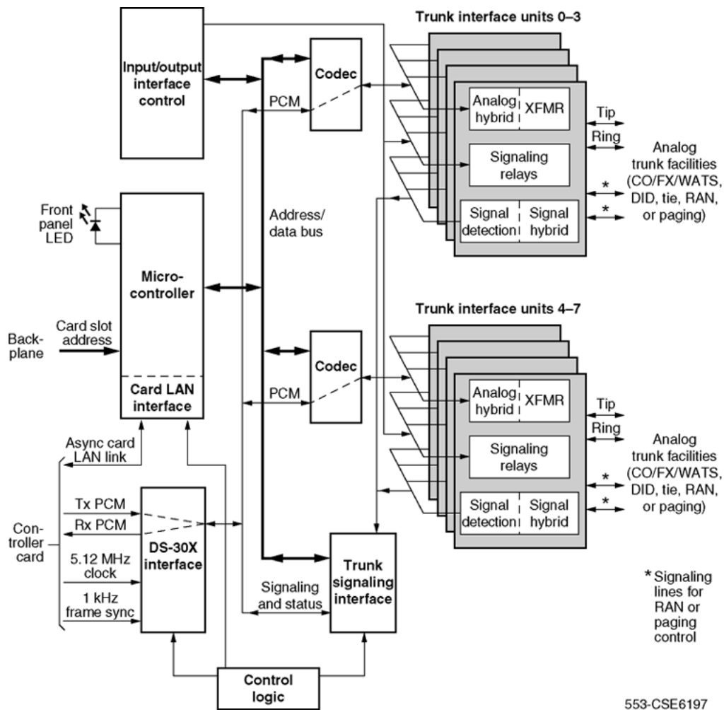
Figure 110: NT8D14 Universal trunk card - block diagram
