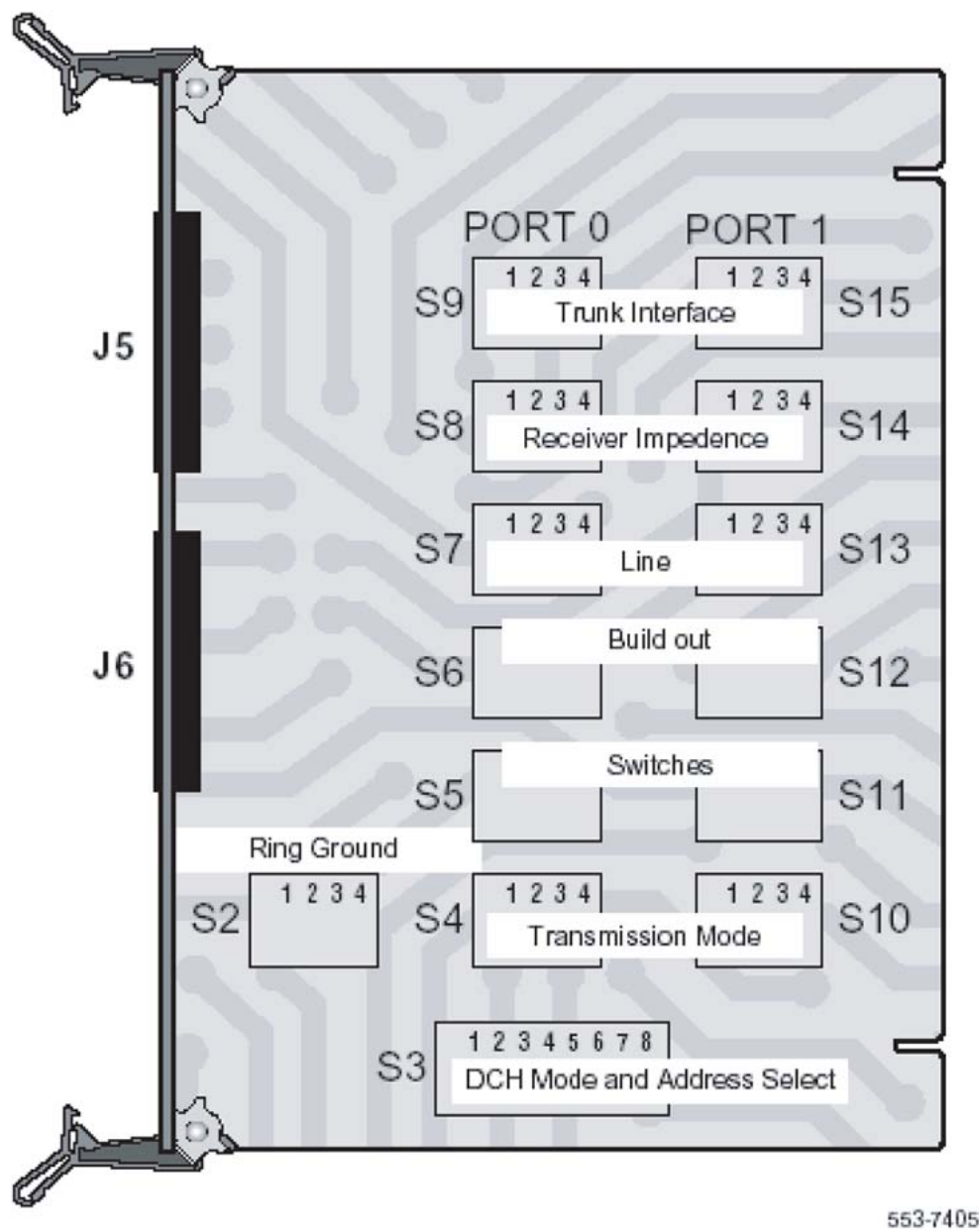
Figure 83: Dip switches for NT5D97AA/AB
