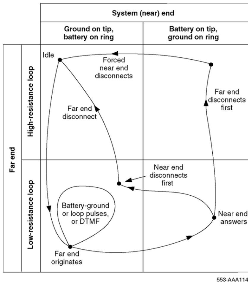
Figure 129: Two-way, loop OAID, TIE trunk call states - incoming call from far-end PBX
