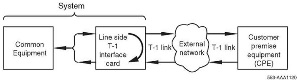
Figure 38: MMI local loopback test
