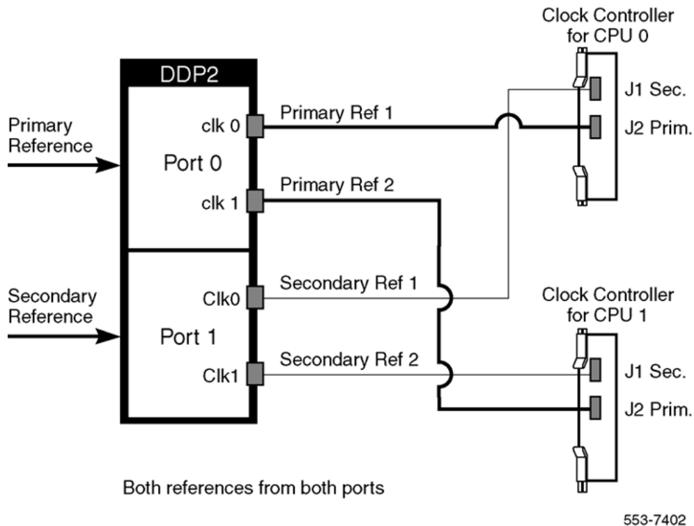
Figure 89: Clock Controller - Option 4
