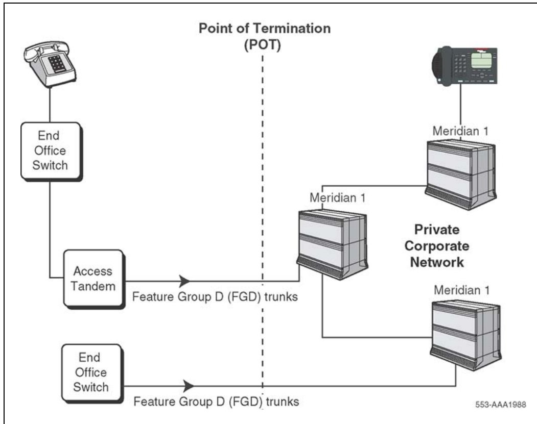
Figure 8 Configuration example
