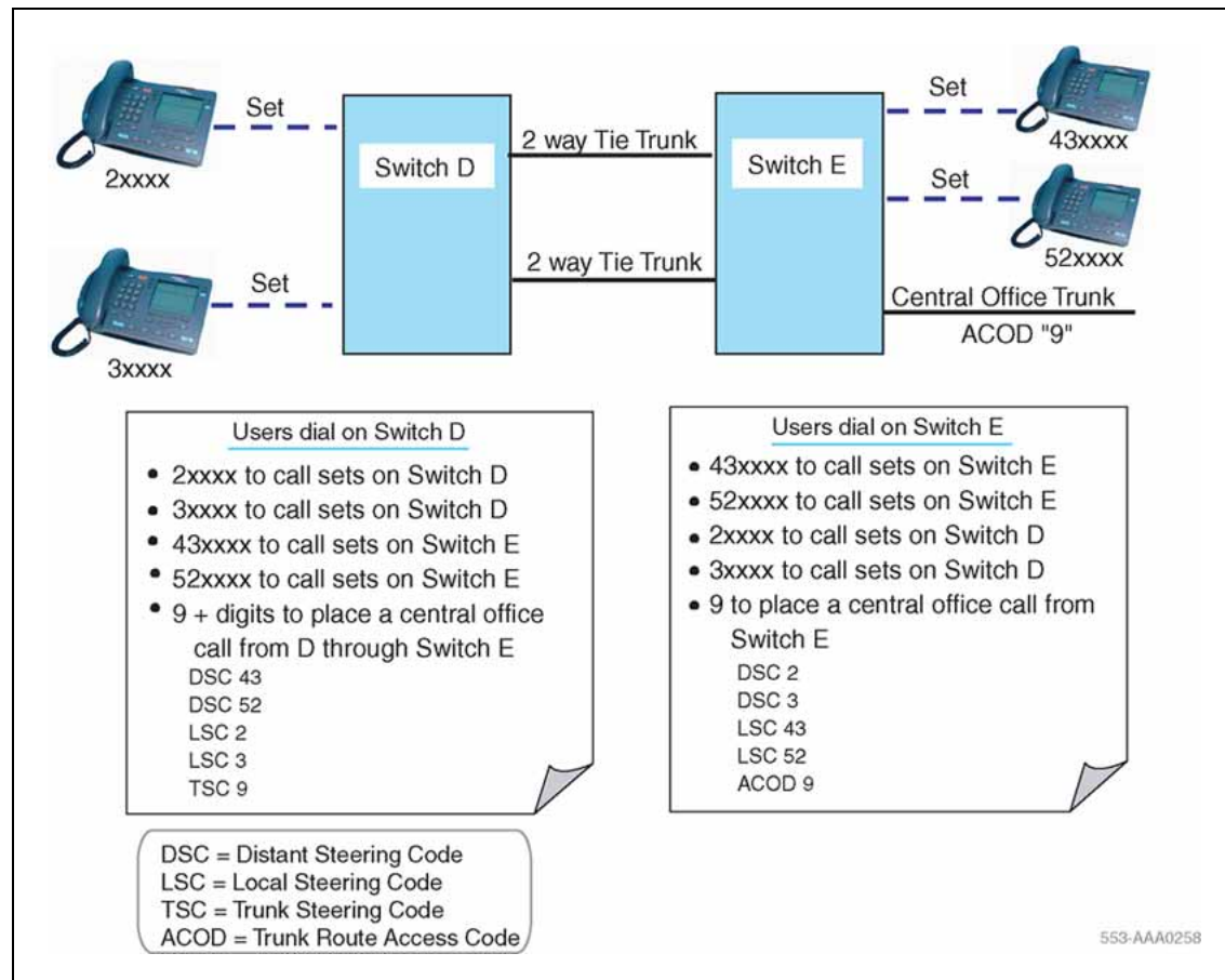
Figure 1 Example of a Coordinated Dialing Plan
