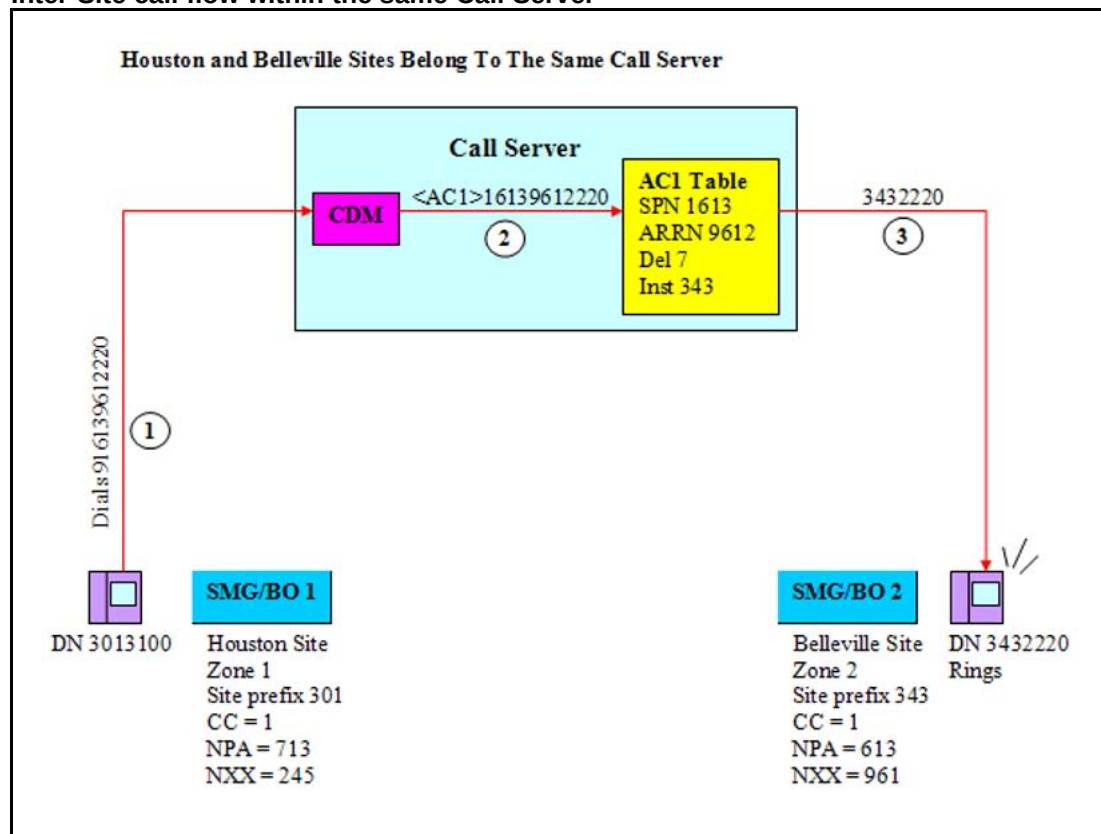
Figure 32 Inter-Site call flow within the same Call Server
