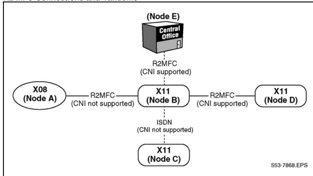
Figure 12 R2 MFC Connections and Tandems
