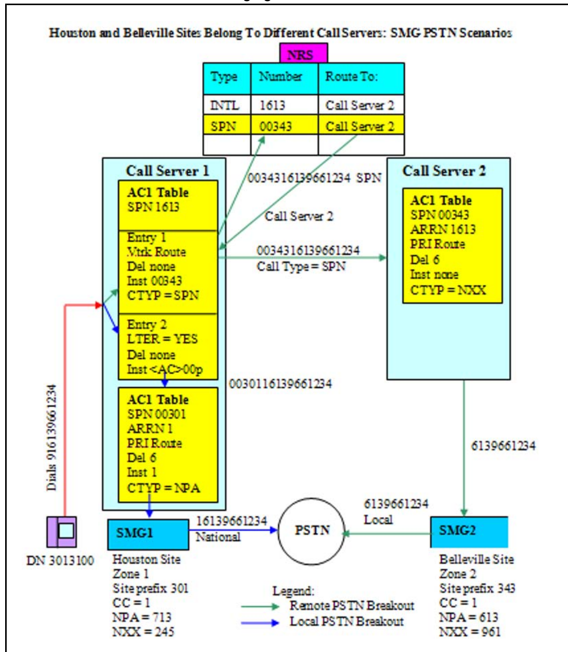
Figure 36 PSTN call flow with SMG sites belonging to different Call Servers
