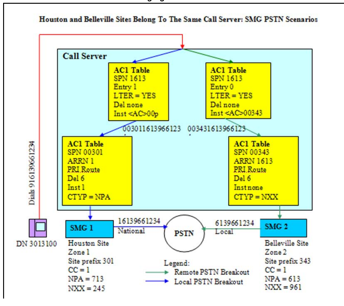
Figure 34 PSTN call flow with SMG sites belonging to the same Call Server
