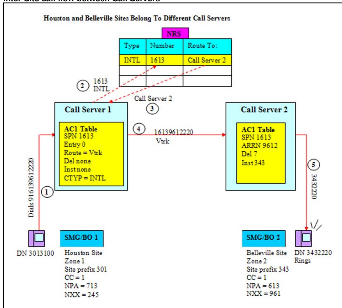
Figure 33 Inter-Site call flow between Call Servers
