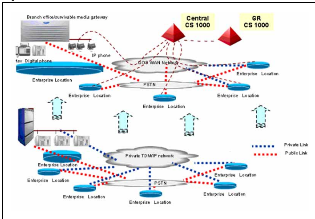
Figure 14 Migration from traditional multi CS model to ZBD model
