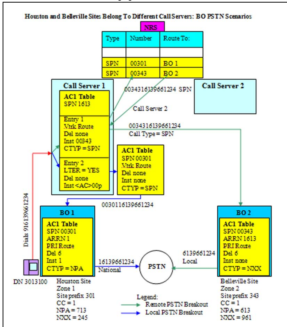
Figure 37 PSTN call flow with BO sites belonging to different Call Servers
