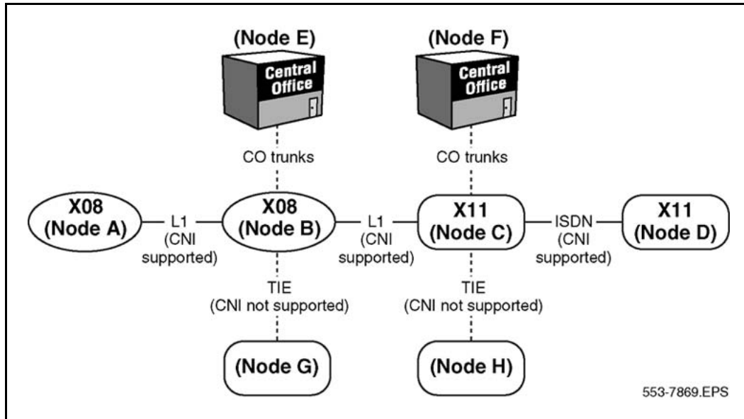
Figure 13 L1 MFC Connections and Tandems
