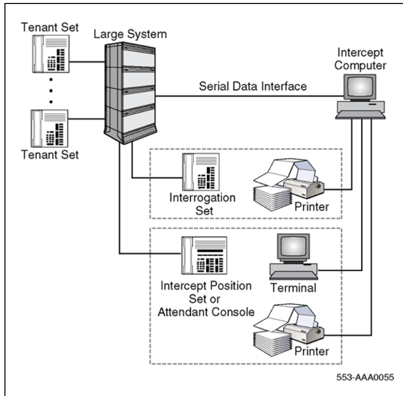
Figure 3 Intercept Computer Interface components
