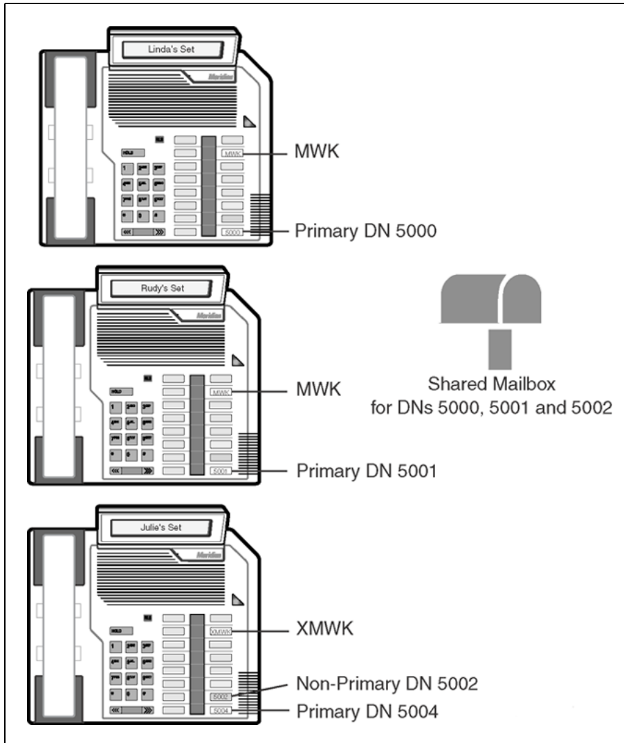
Figure 20 One mailbox for multiple DNs
