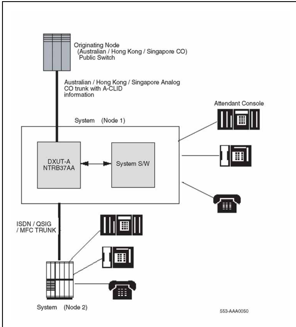
Figure 24 System structure for CLID delivery
