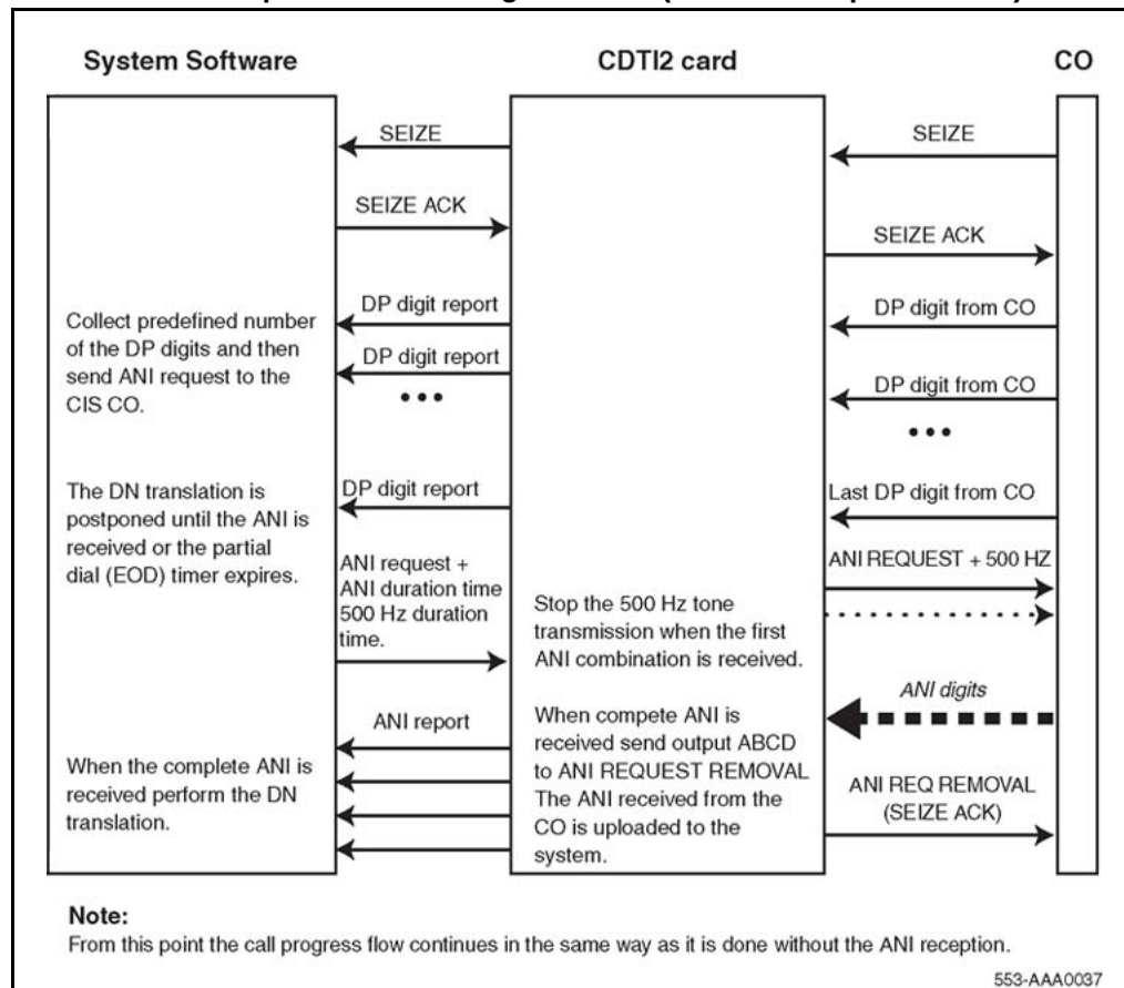
Figure 6 Automatic ANI request for incoming local call (decadic dial pulse mode)
