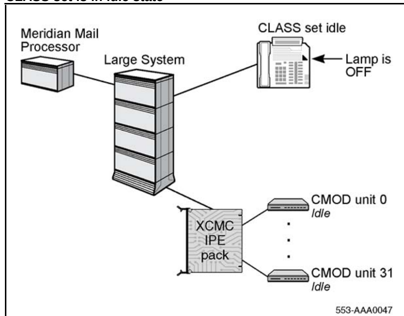
Figure 18 CLASS set is in idle state
