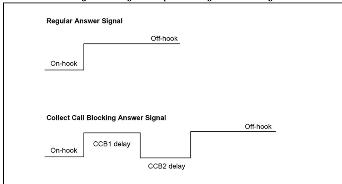
Figure 25 Collect Call Blocking answer signal compared to regular answer signal
