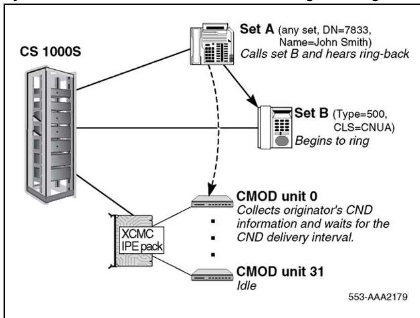
Figure 15 System resource allocation during the CND delivery interval
