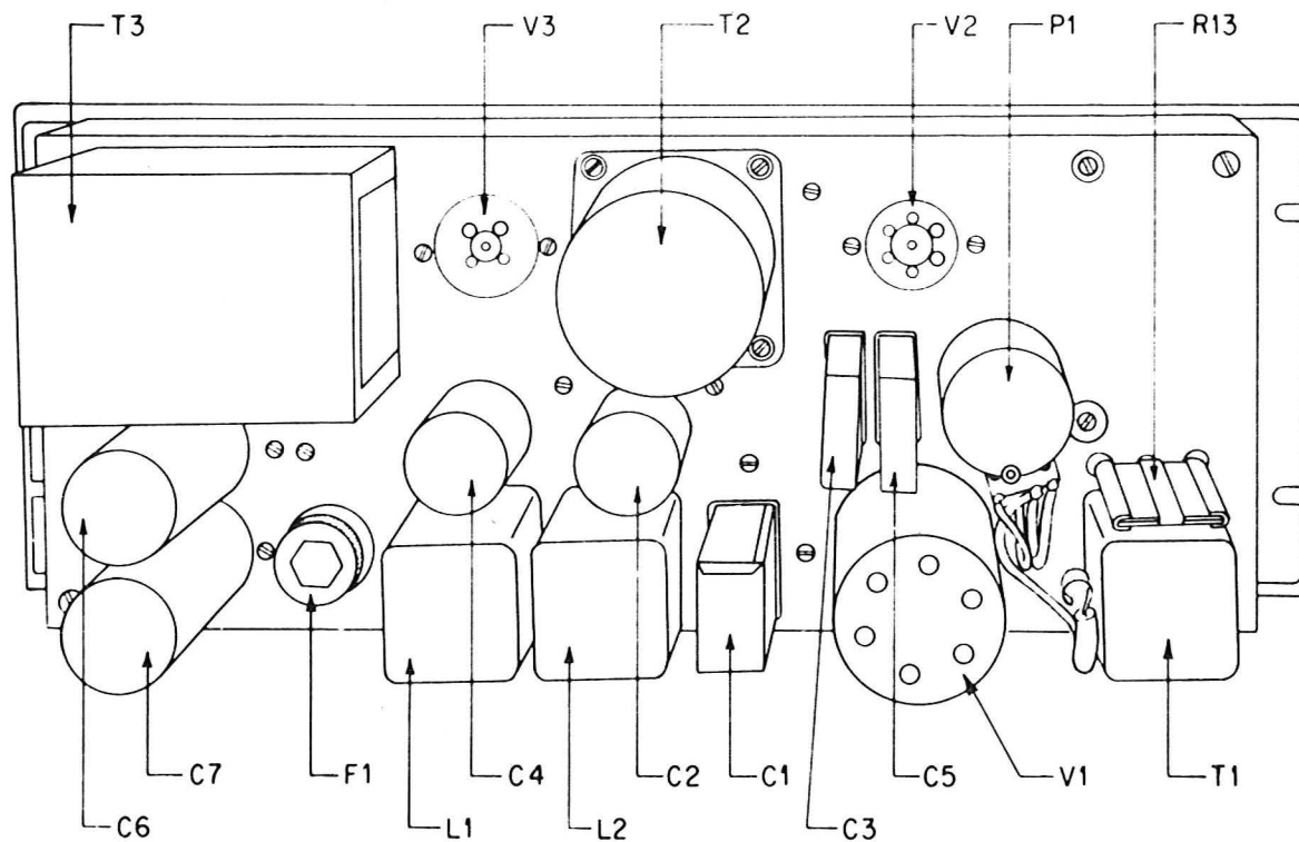
Fig. 1b - 106-Type Amplifier - Rear View
