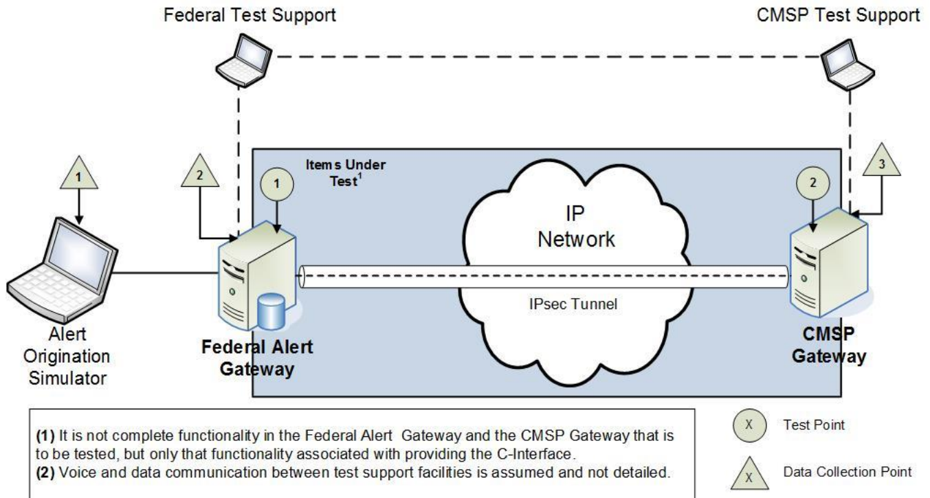
Figure 4.1: C-Interface Test Architecture for Single CMSP Gateway
