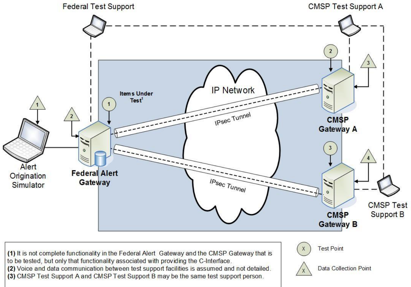
Figure 4.2: C-Interface Test Architecture for Dual CMSP Gateways
