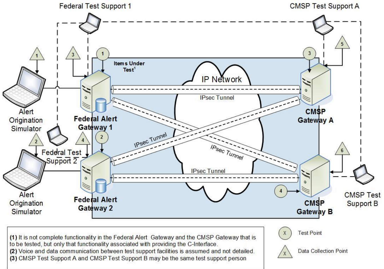
Figure 4.3: C-Interface Test Architecture for Dual Federal Alert Gateways and Dual CMSP Gateways
