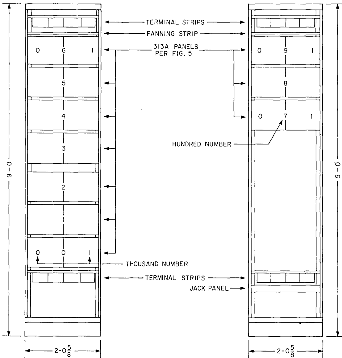
Fig. 9—Number Network Frames
