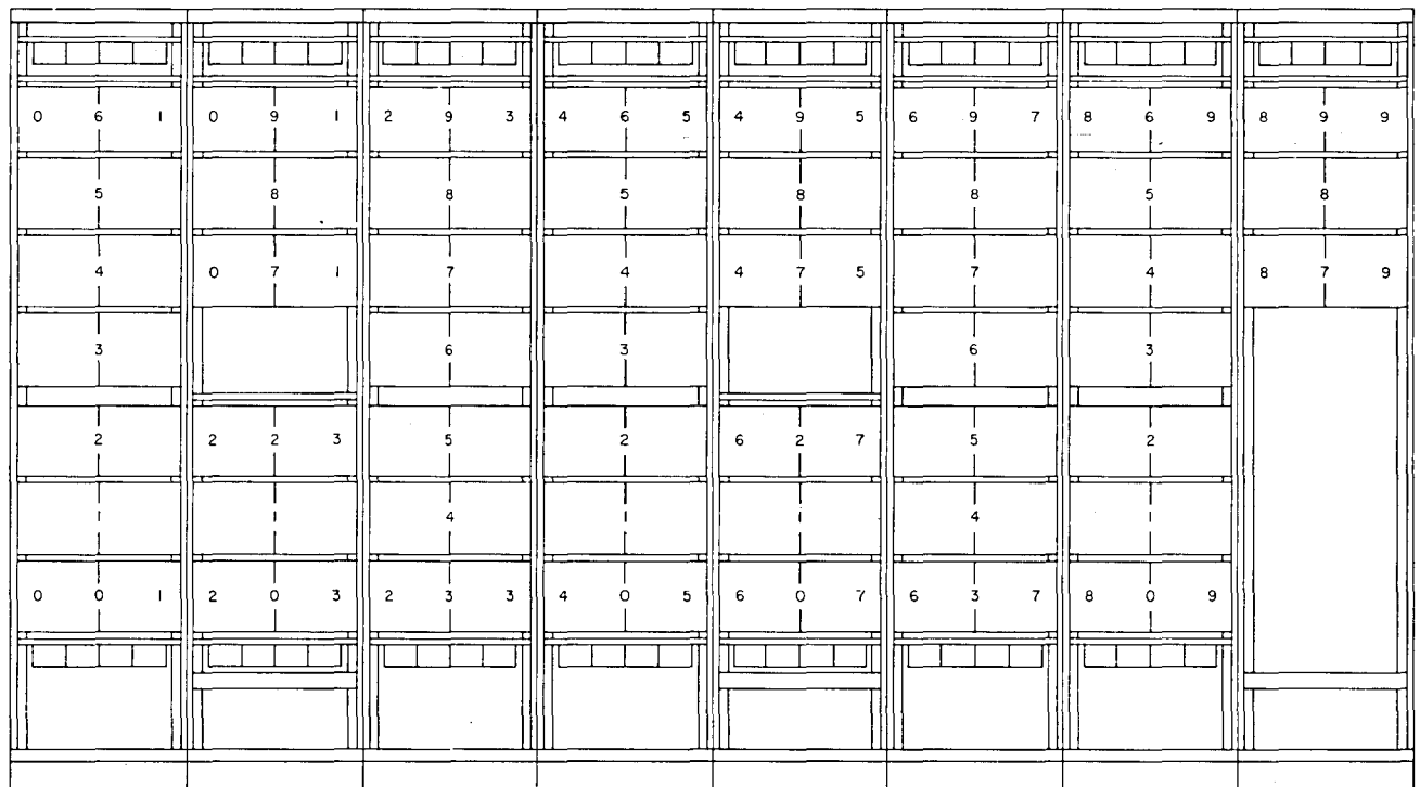
Fig. 10—Number Network Frames Arranged for 10,000 Numbers
