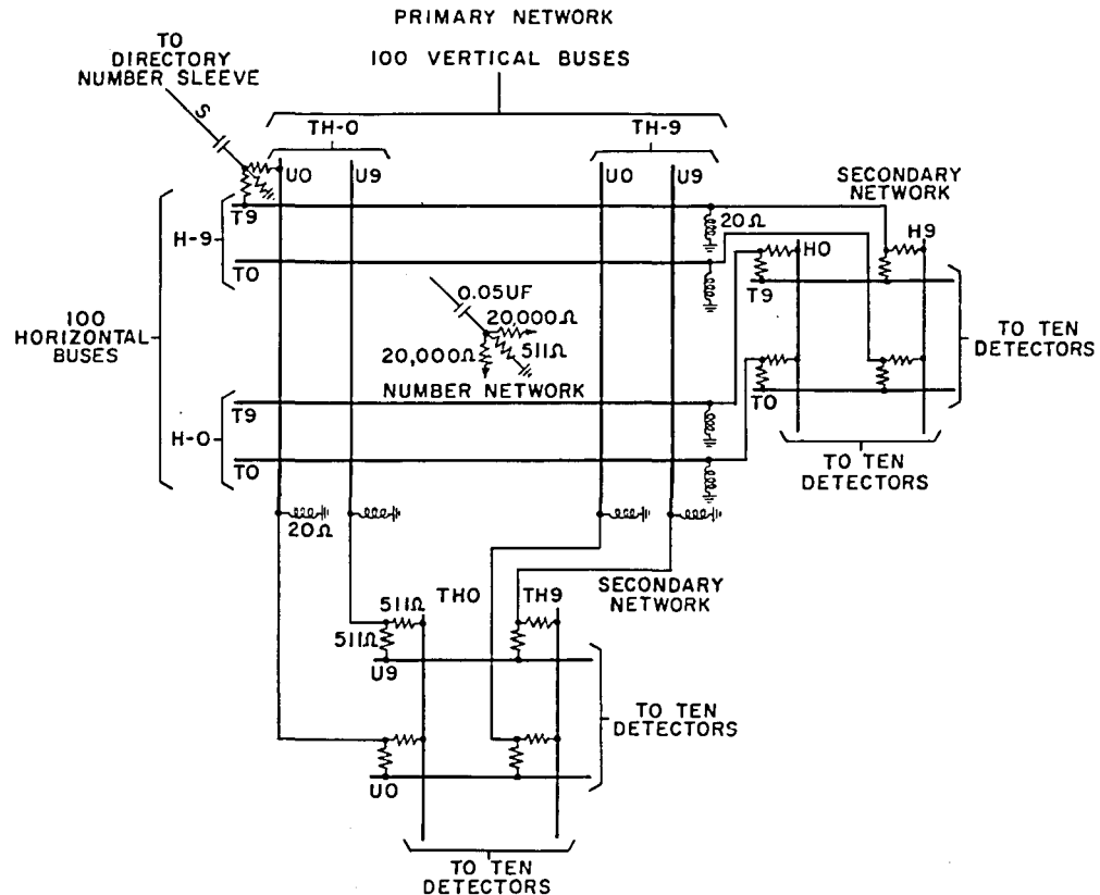
Fig. 2—Number Network System for 10,000 Numbers
