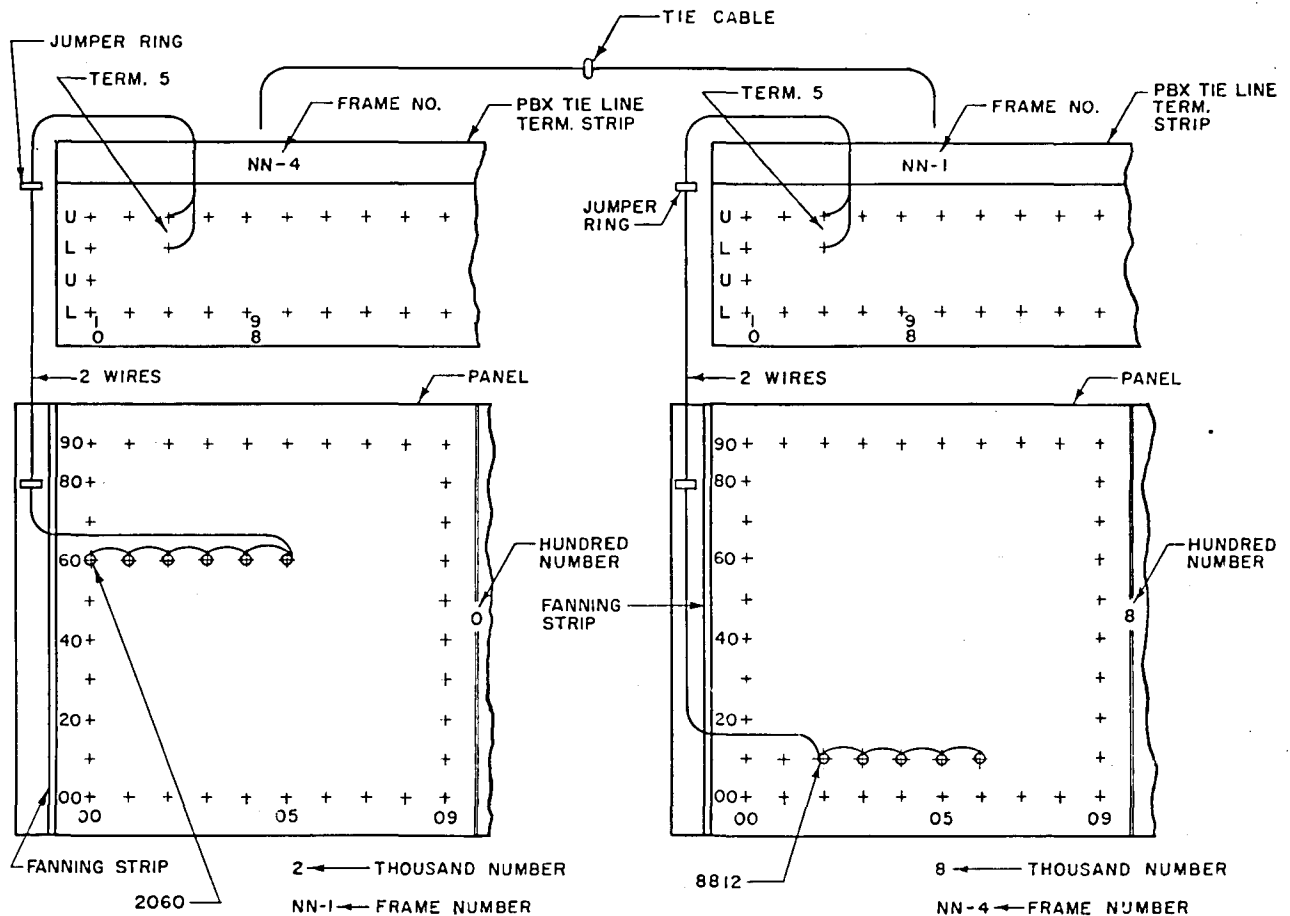
DIAGRAM OF TYPICAL PBX CONNECTION BILLING NO. 2060 CONSECUTIVE NO. 2060 TO 2065 NON-CONSECUTIVE NO. 8812 TO 8816
