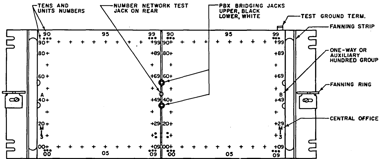
Fig. 6—"X" or Miscellaneous Number Network Panel (313A)—200 Numbers
