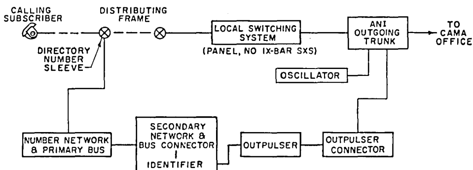
Fig. 1—Automatic Number Identification—Block Diagram
