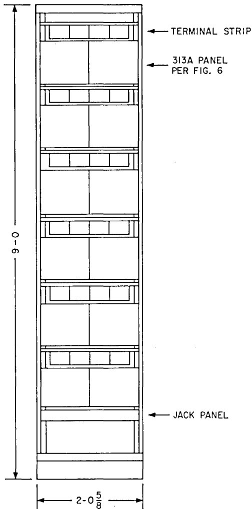
Fig. 11—Miscellaneous Number Network Frame
