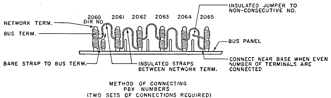
Fig. 8—PBX Cross-Connections
