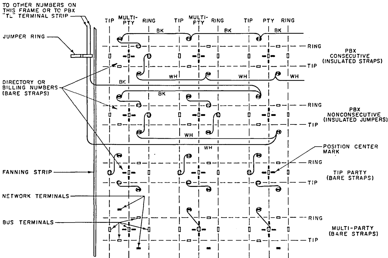
Fig. 7—Number Network—Cross-Connections
