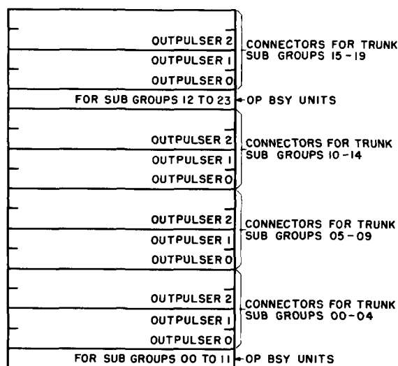
Fig. 2—Typical Arrangement of Outputpulser Connectors on Relay Rack for 3 Outputpulsers (4 Ultimately) and 20 Trunk Subgroups
