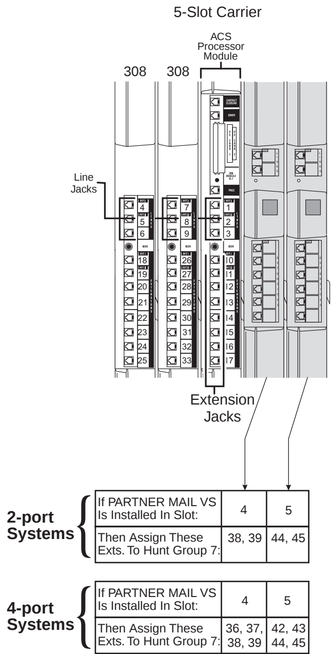
Figure D-1. Dial Plan for PARTNER Advanced Communications System Release 2.0 or Later
