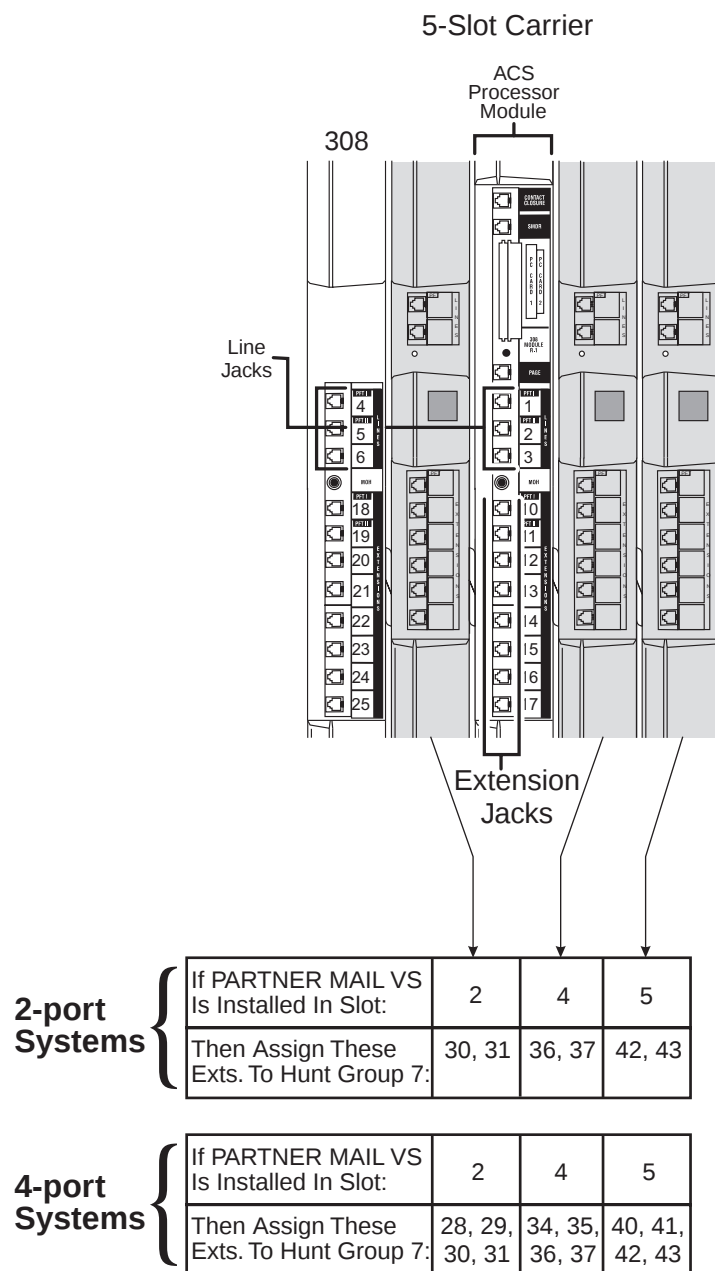
Figure D-2. Dial Plan for PARTNER Advanced Communications System Release 2.0 or Later
