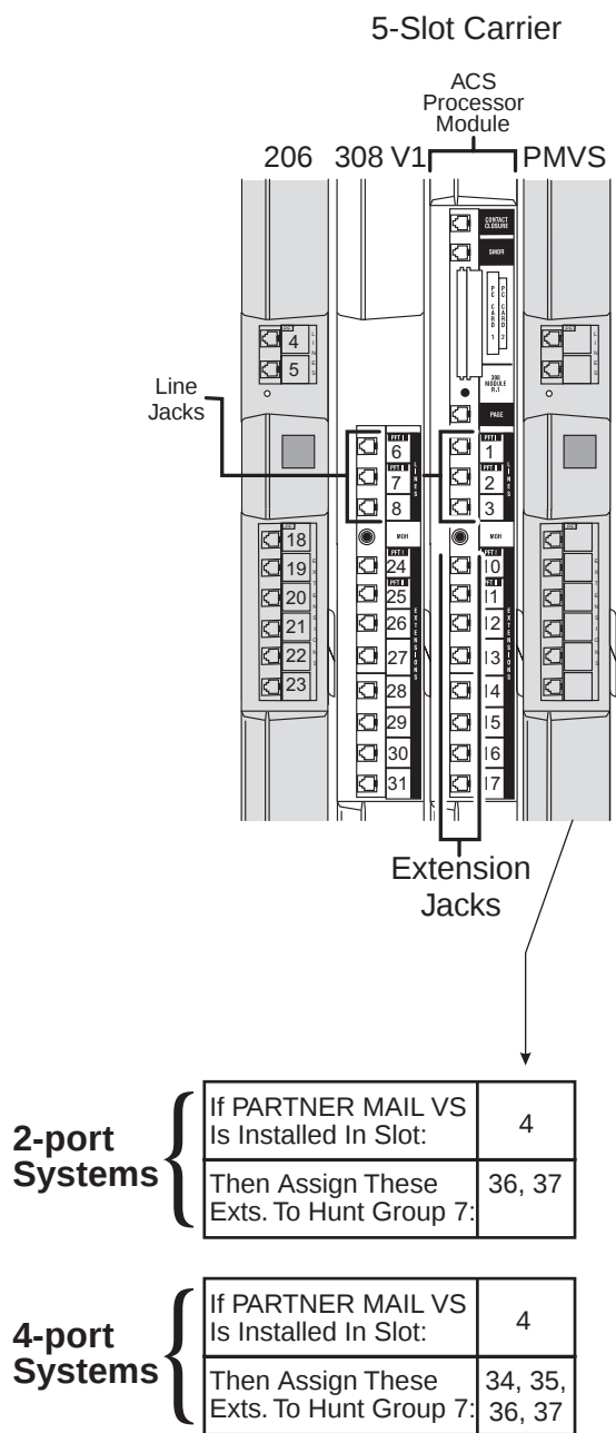
Figure D-6. Dial Plan for Systems with Fax Tone Detect and a Voice Messaging System Module
