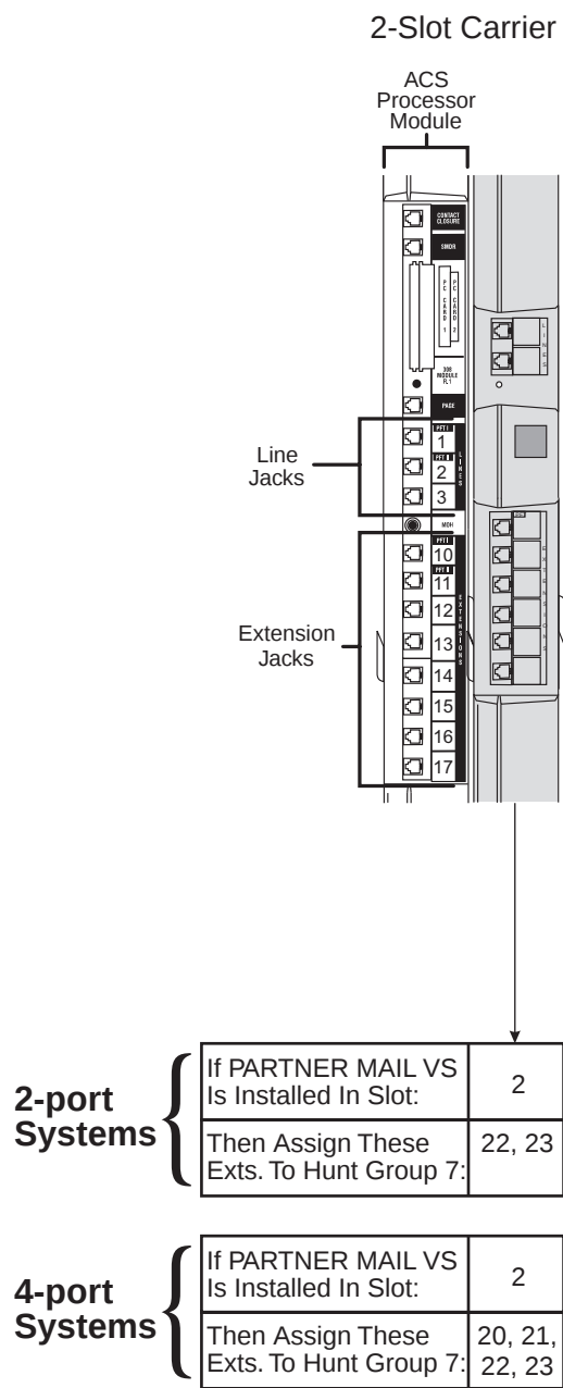
Figure D-4. Dial Plan for PARTNER Endeavor Release 1.0 and PARTNER Advanced Communications System Release 1.0, 1.1, 2.0 or Later
