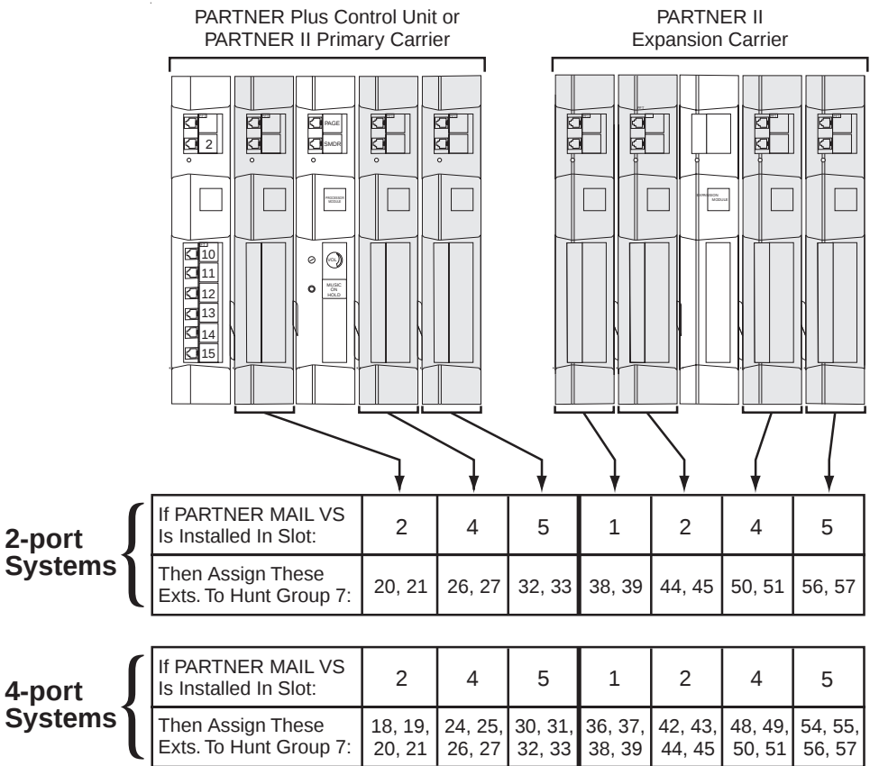
Figure D-5. Voice Messaging System Extensions for PARTNER Plus and PARTNER II Communications Systems
