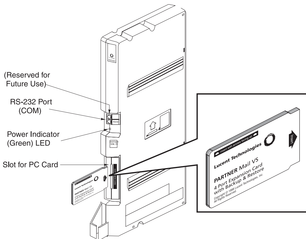
Figure 2-2. Installing the PC Card
