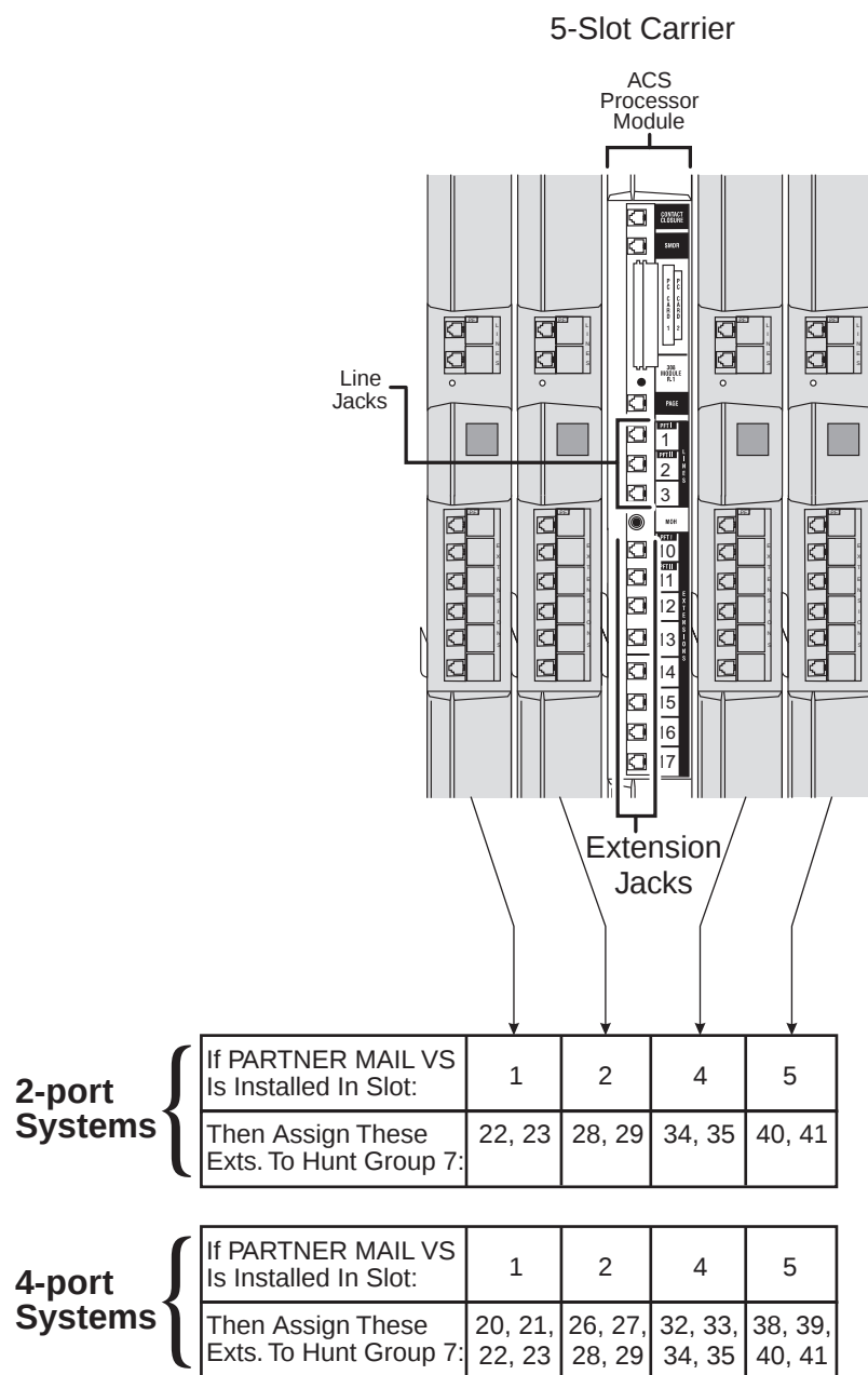
Figure D-3. Dial Plan for PARTNER Endeavor Release 1.0 and PARTNER Advanced Communications System Release 1.0, 1.1, 2.0 or Later
