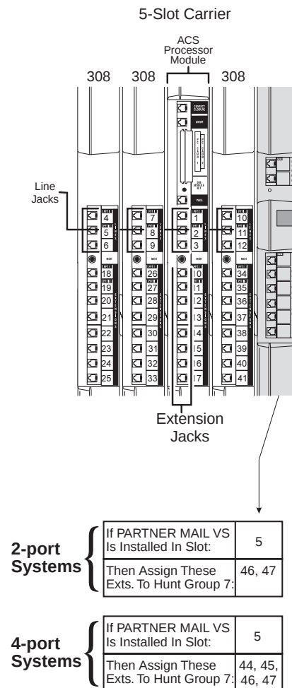
Figure 2-1. Voice Messaging System Extensions for PARTNER Advanced Communications System Release 2.0 or later with 308 and PARTNER MAIL Voice Messaging System Modules
