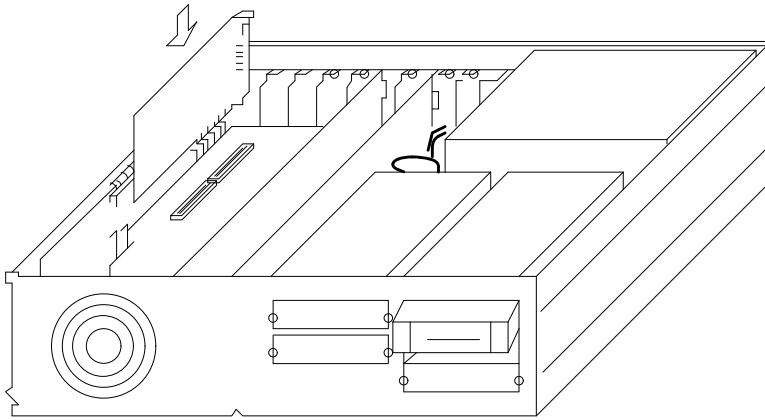
Figure 3-3. Inserting the DCP Board into a 6386/25 Expansion Slot
