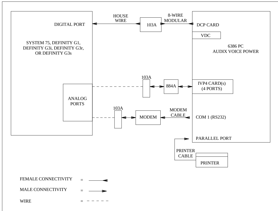
Figure 1-1. Connectivity Diagram for the System 75, DEFINITY G1, and G3 Switches
