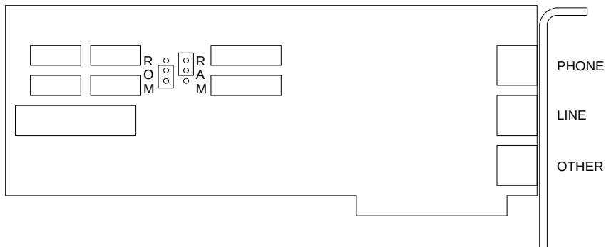
Figure 3-1. DCP Board ROM and RAM Jumper Location
