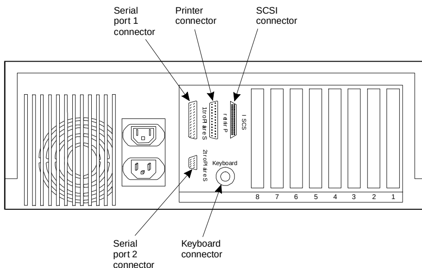
Figure 11-4. Back View of the MAP/5
