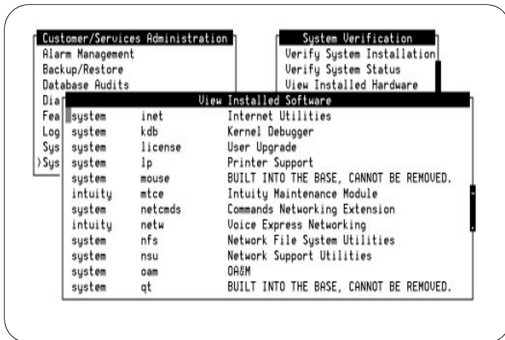
Figure 2-3. View Installed Software, Line-by-Line Listing Showing UNIX Multi-User (system, license, User Upgrade)
