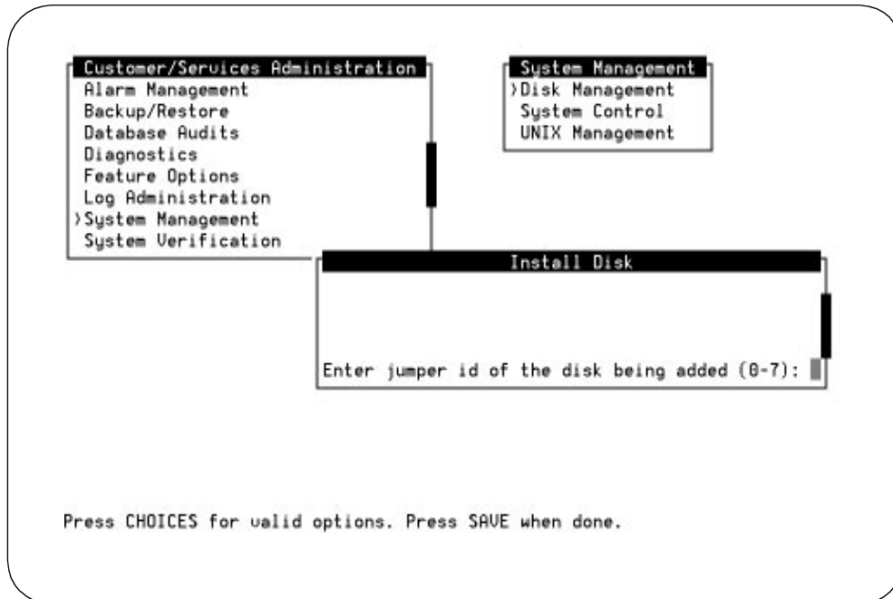
Figure B-18. Install Disk Screen
