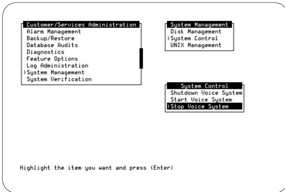
Figure B-10. System Control Screen
