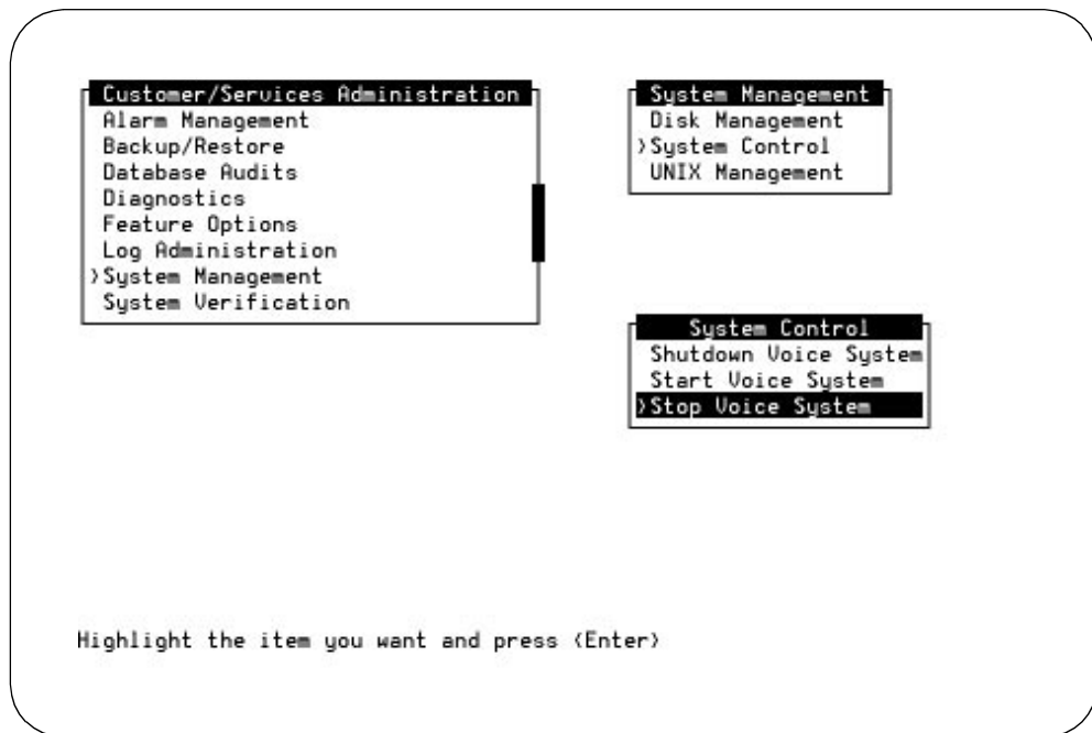
Figure B-33. System Control Screen
