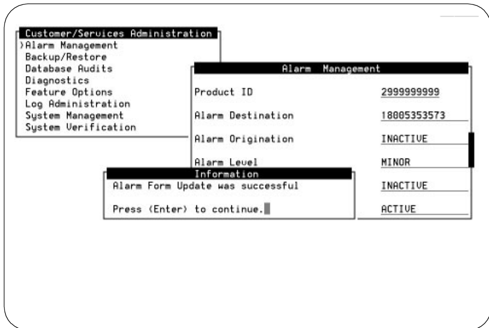
Figure B-32. Alarm Management Screen Update Information Screen
