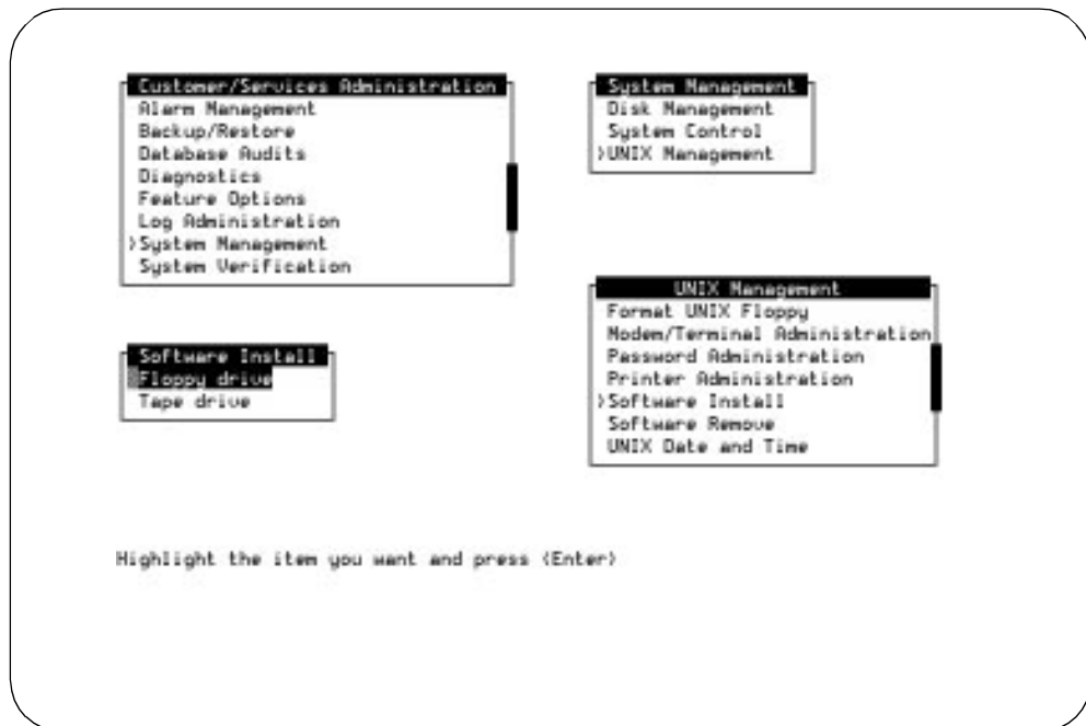
Figure B-35. Software Install Screen
