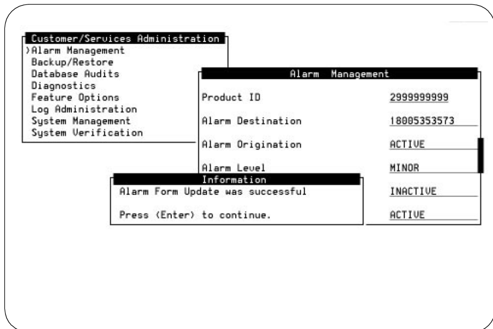
Figure B-27. Alarm Management Screen Update Information Screen
