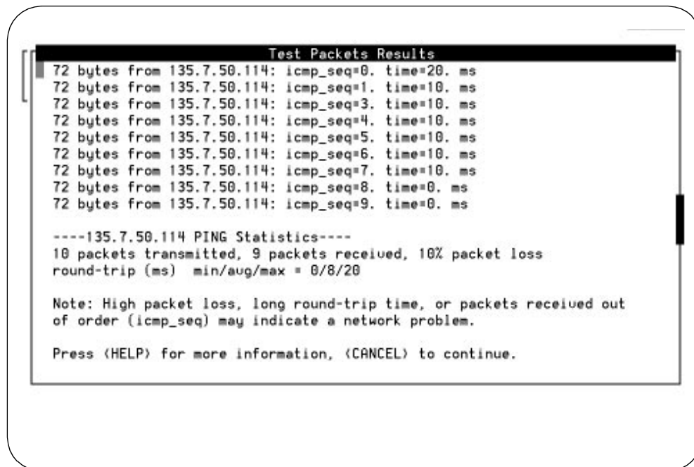
Figure 5-8. Test Packet Results Screen
