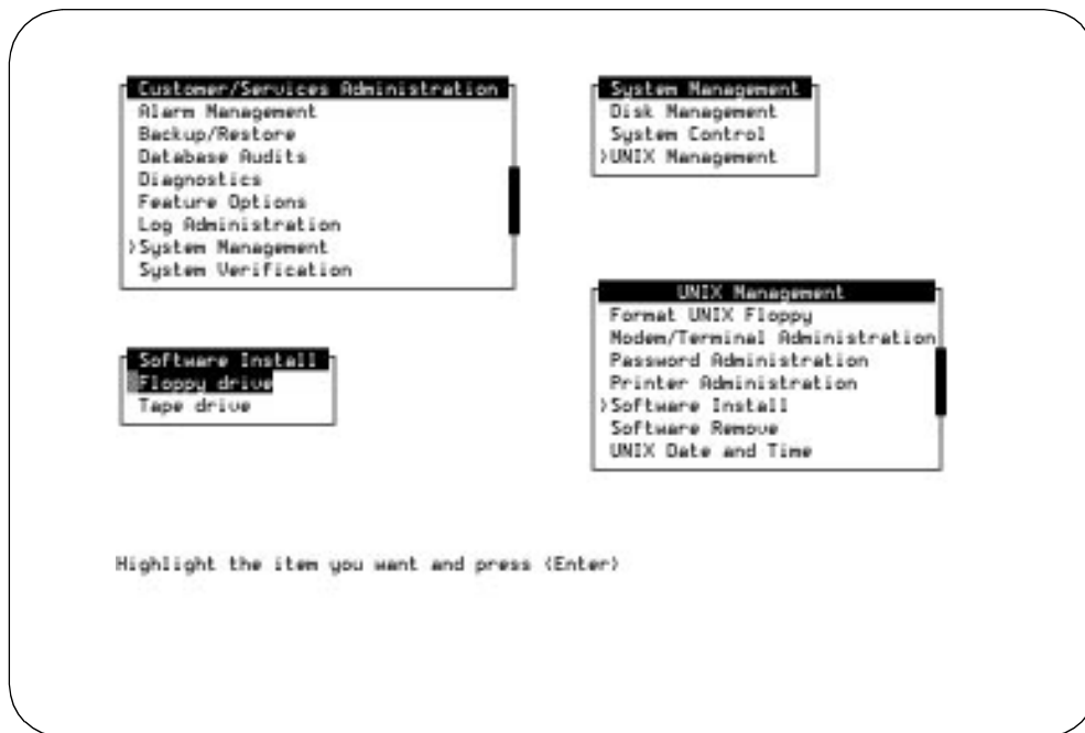
Figure B-16. Software Install Screen
