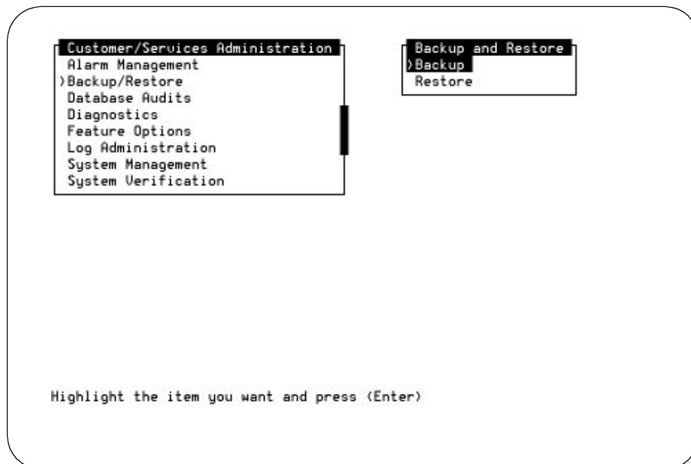
Figure B-20. Backup and Restore Screen
