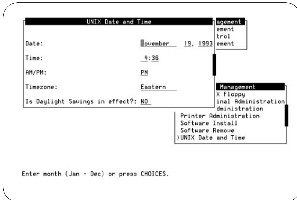
Figure B-23. UNIX Date and Time Screen
