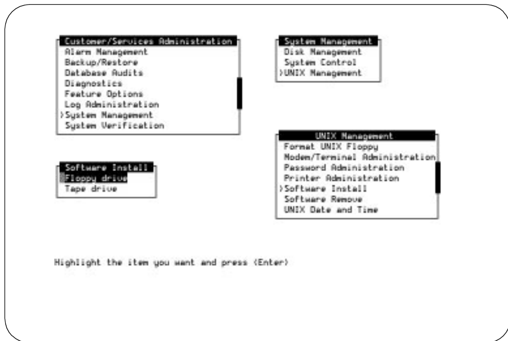
Figure B-15. Software Install Screen
