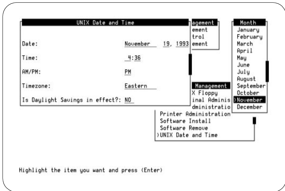
Figure B-24. UNIX Date and Time Screen With the Months Choices Screen
