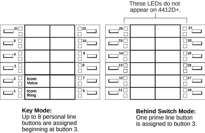
Figure G-3. 4412D+, 4424D+, and 4424LD+ Telephones (Key and Behind Switch Modes)
