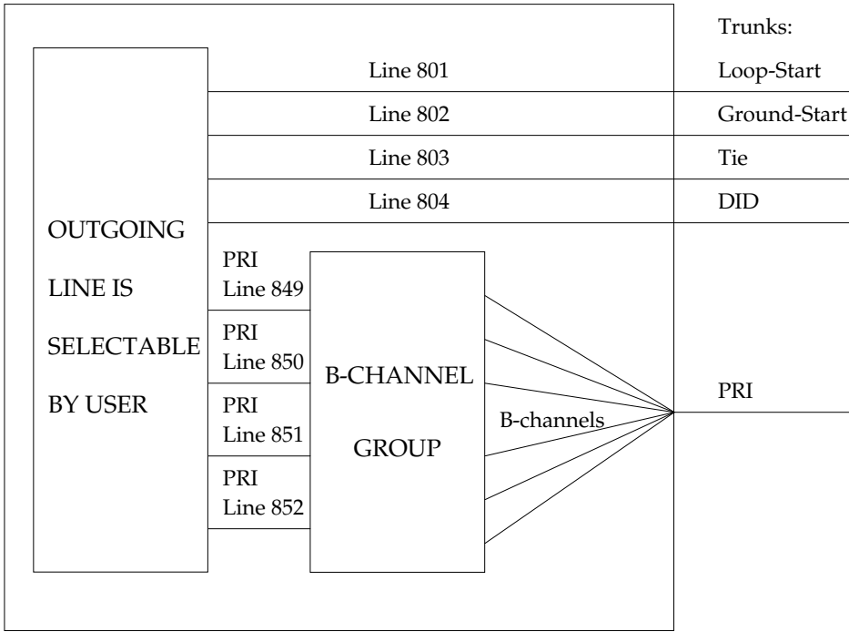
Figure 34. PRI Lines and B Channel Groups
