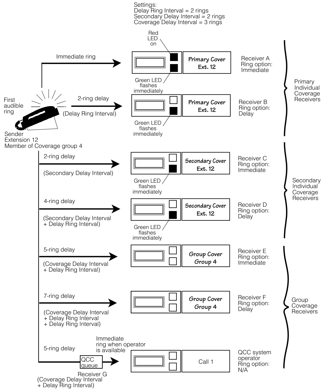
Figure 7. Individual (Primary and Secondary) and Group Coverage Ringing Patterns
