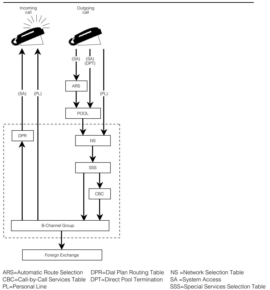
Figure 35. PRI Call Processing
