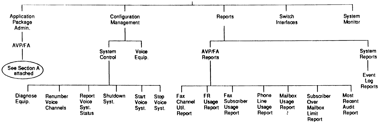
Menu Tree for Maint Login, Section B
