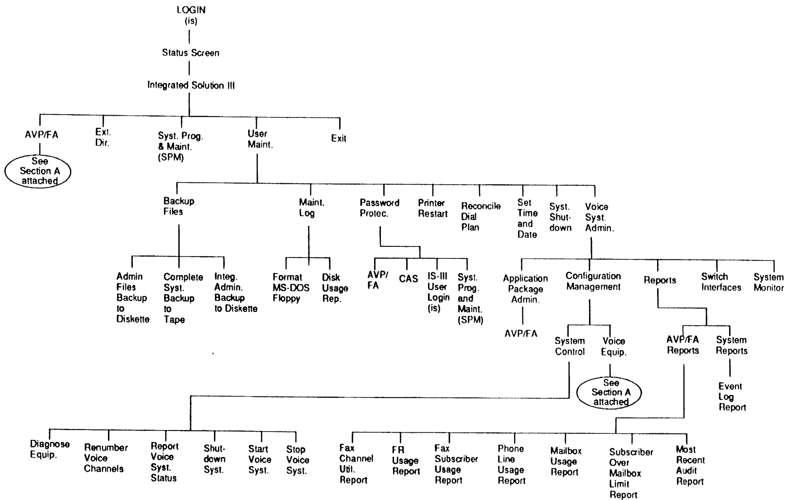
Menu Tree for IS Login
