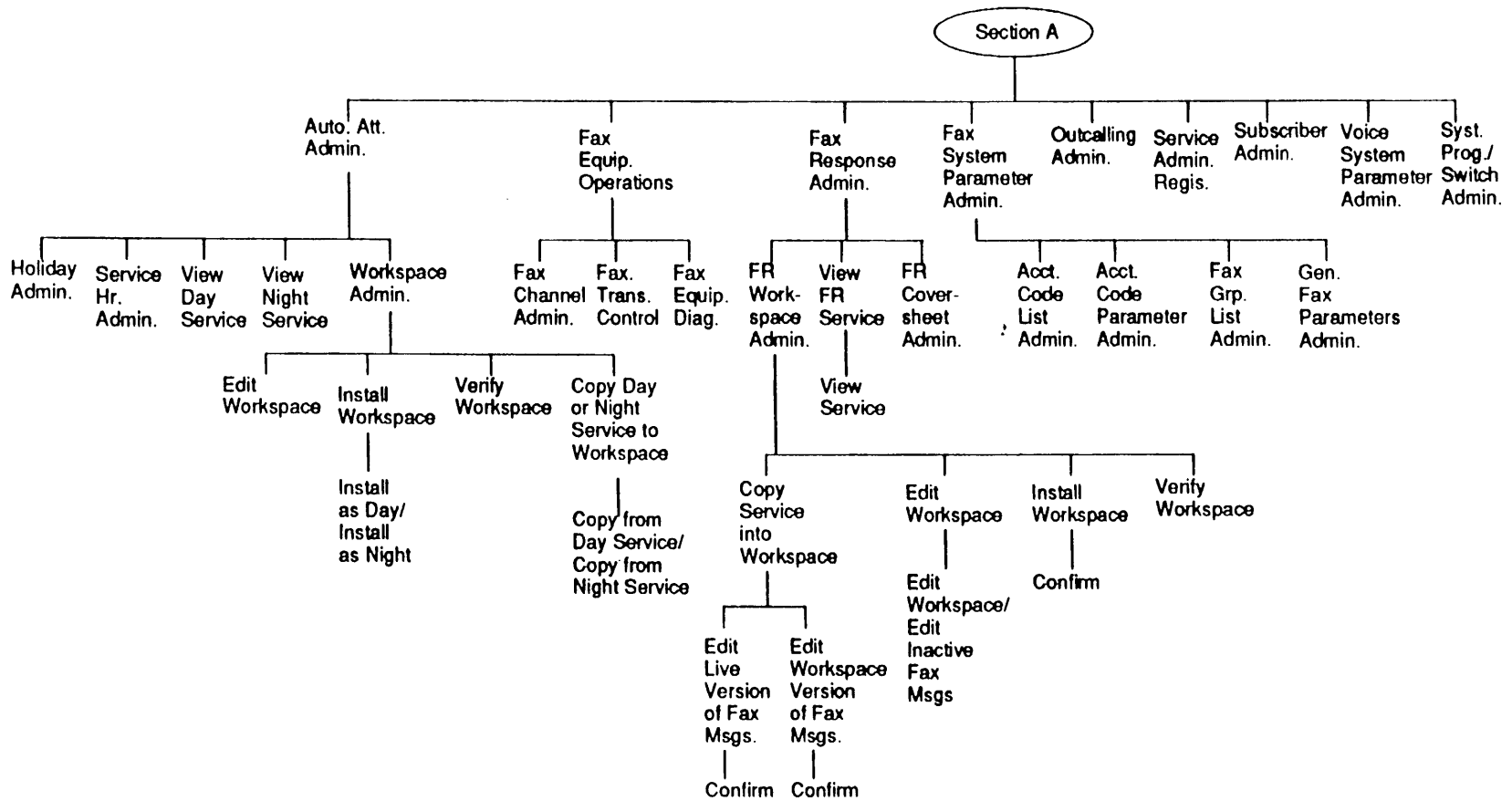
Menu Tree for Maint Login, Section A
