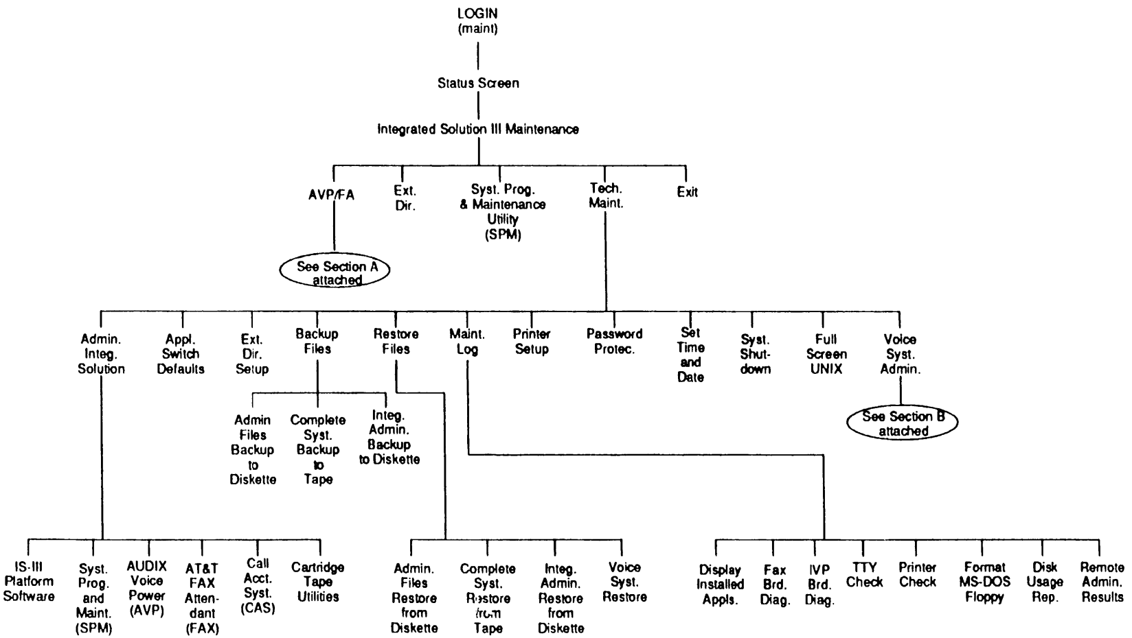
Menu Tree for Maint Login
