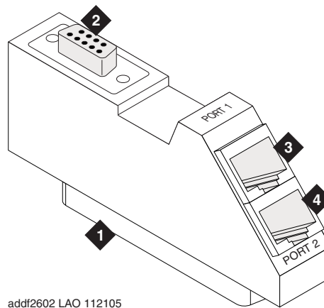
Figure 82: IP Media Resource 320 I/O adapter
