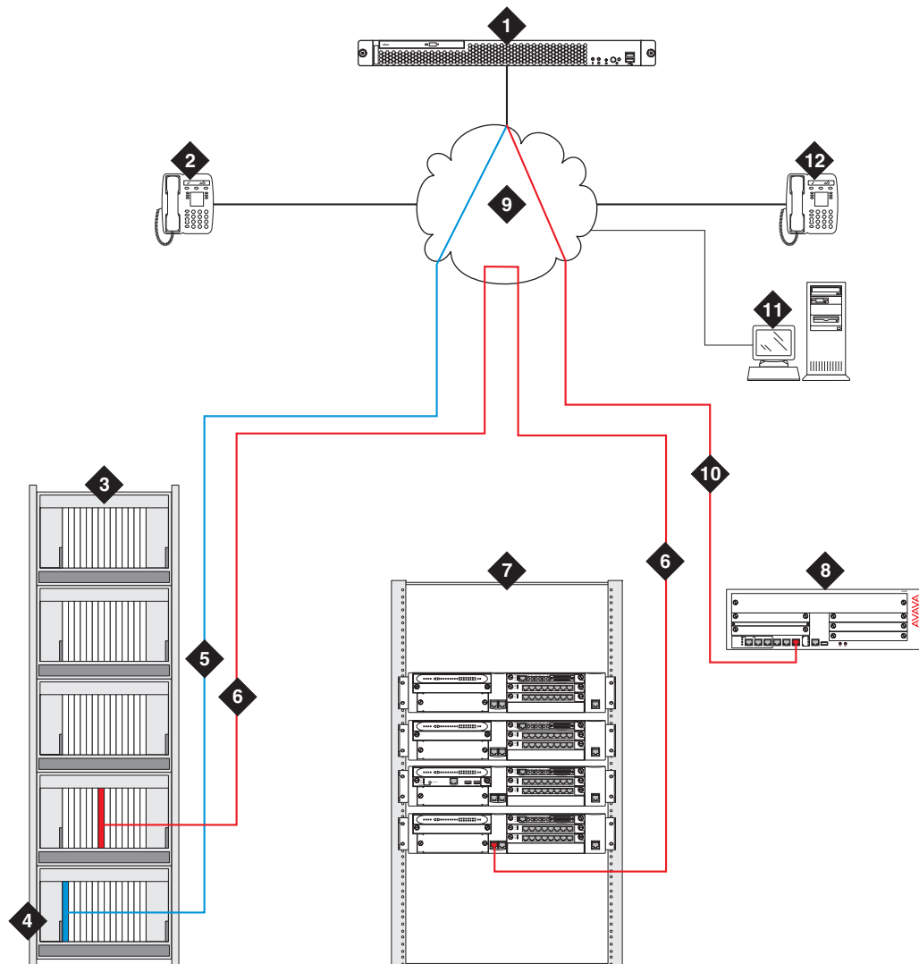
Figure 14: Mixed S8500 configuration with both Processor Ethernet and C-LAN connections
