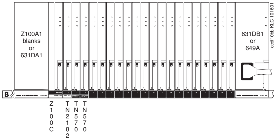
Figure 77: Port carrier (J58890BB)
