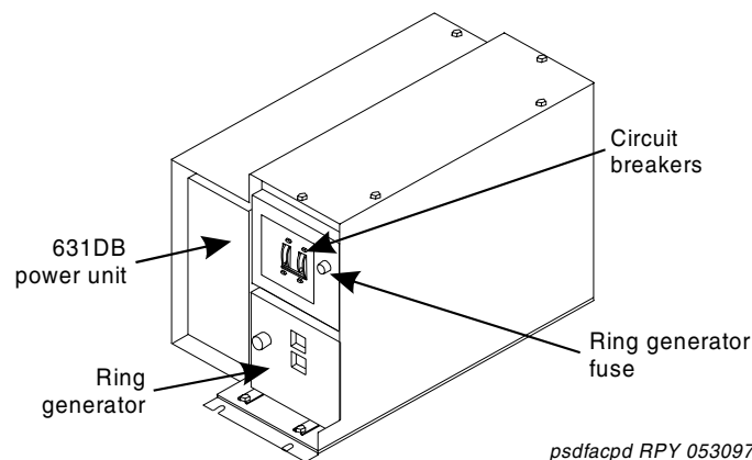
Figure 101: AC power-distribution unit (J58890CE-2) (front)
