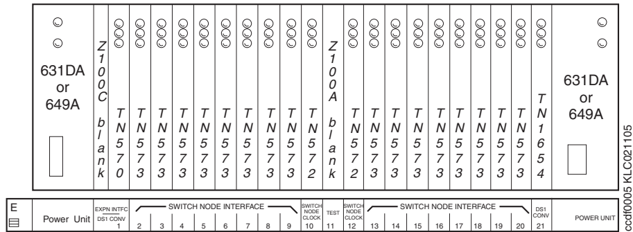
Figure 78: Switch node carrier (J58890SA)
