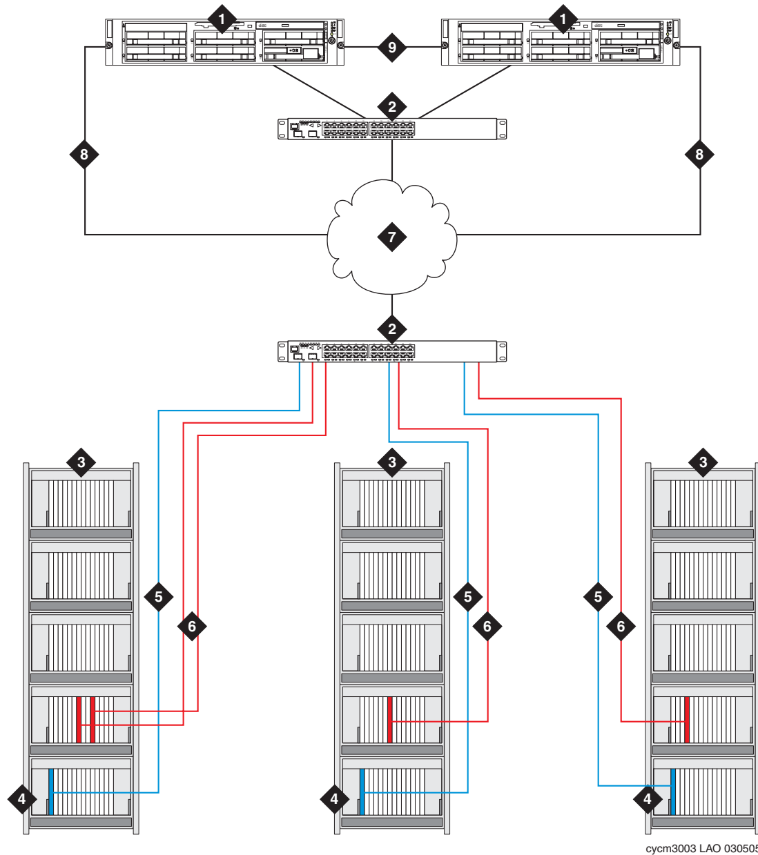
Figure notes: S8700-series IP-PNC single control network
