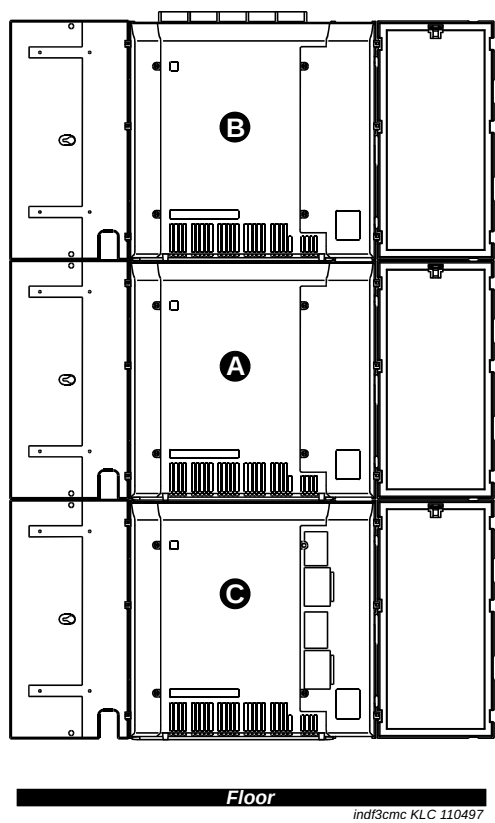
Figure 66: Typical vertical installation, front view of the CMC1 Media Gateway, DEFINITY Server CSI configuration
