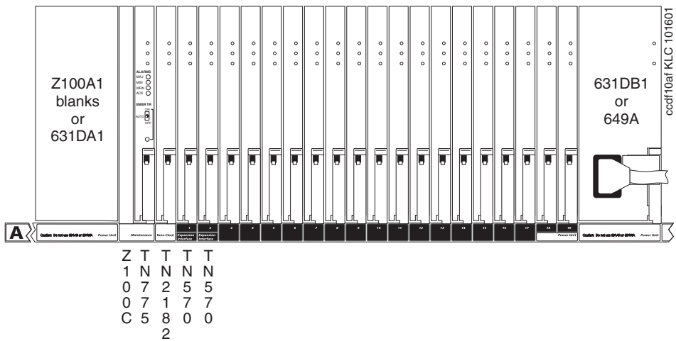
Figure 76: Expansion control carrier (J58890AF)
