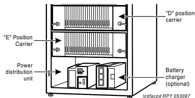
Figure 103: AC power distribution in MCC1 cabinets
