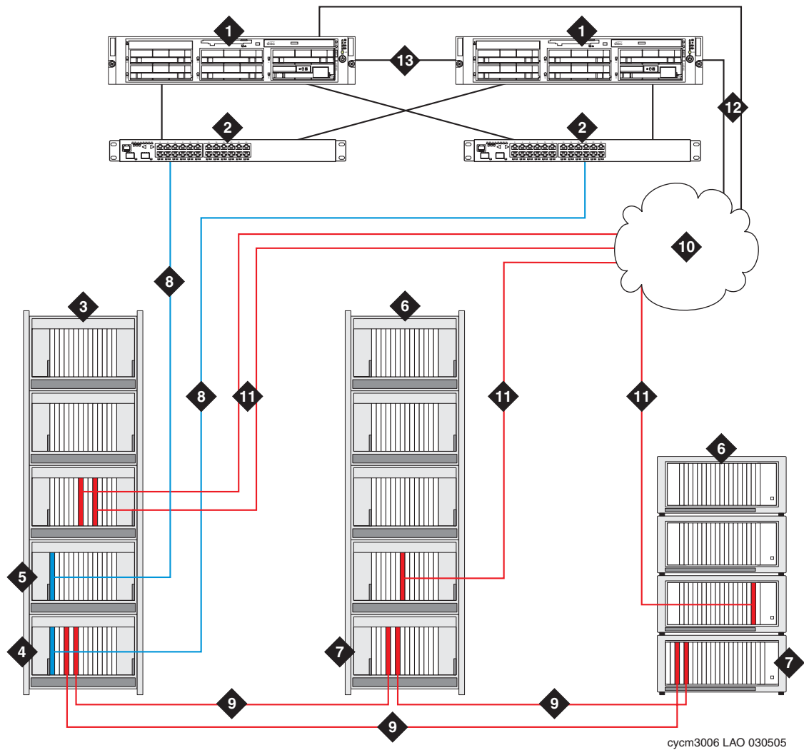
Figure notes: S8700-series direct-connect duplicated control network
