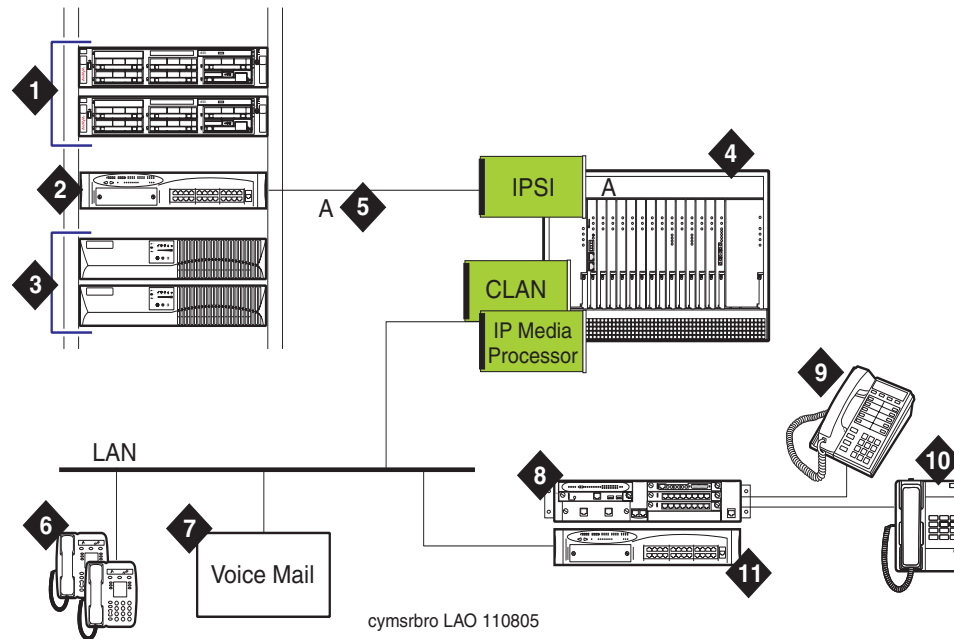
Figure 113: Branch office configuration
