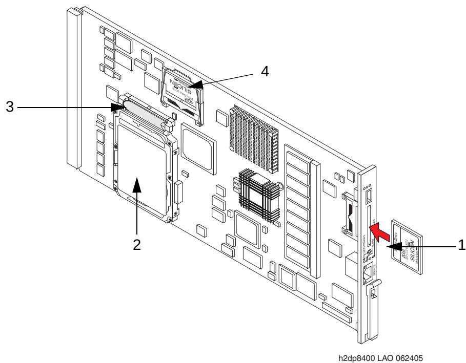
Figure 4: S8400 Media Server
