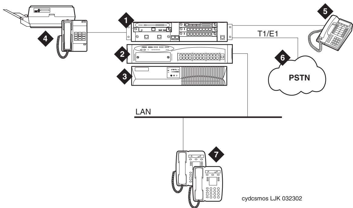
Figure 110: A small-business solution with the Avaya S8300 Media Server in the G700, G350, or G250 Media Gateway (G700 shown)
