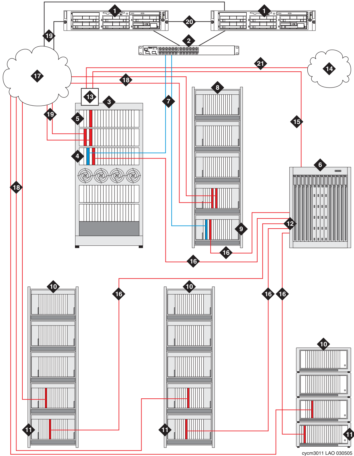
Figure 32: S8700-series ATM single control network
