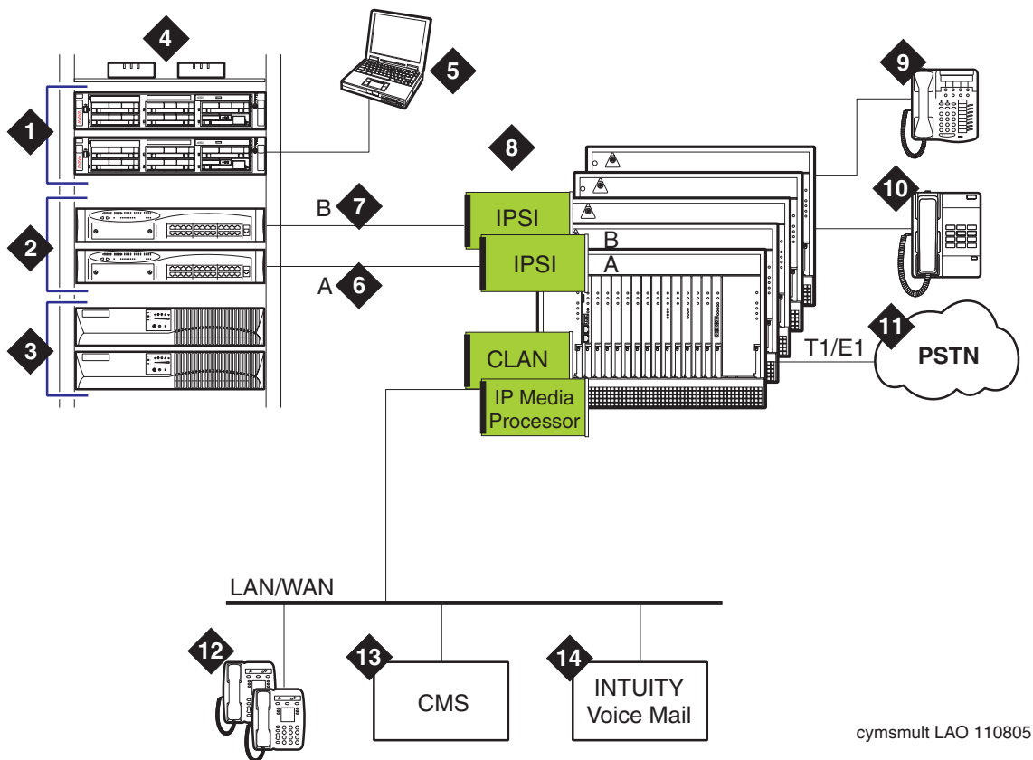
Figure 112: A large-business solution using the Avaya S8710 or S8720 Media Server and the MCC1 Media Gateway (S8710 shown)
