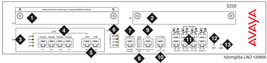
Figure 51: The Avaya G250-Analog Media Gateway Chassis
