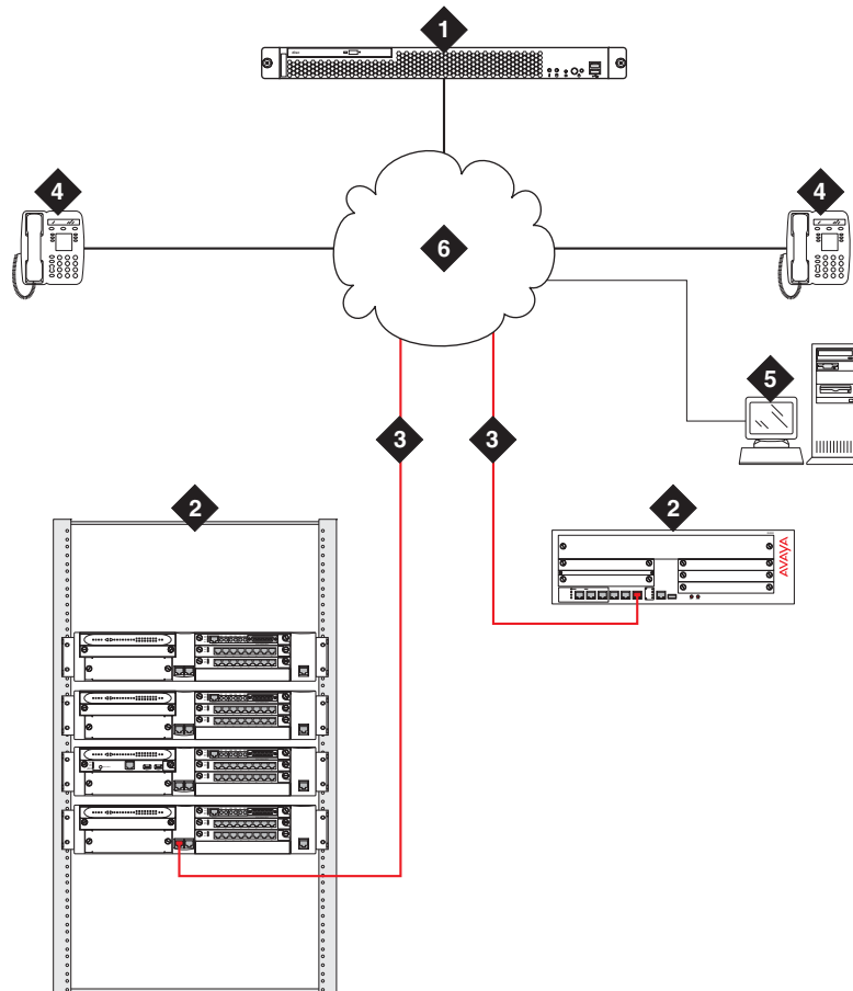
Figure 13: S8500 Configuration with Processor Ethernet connections only
