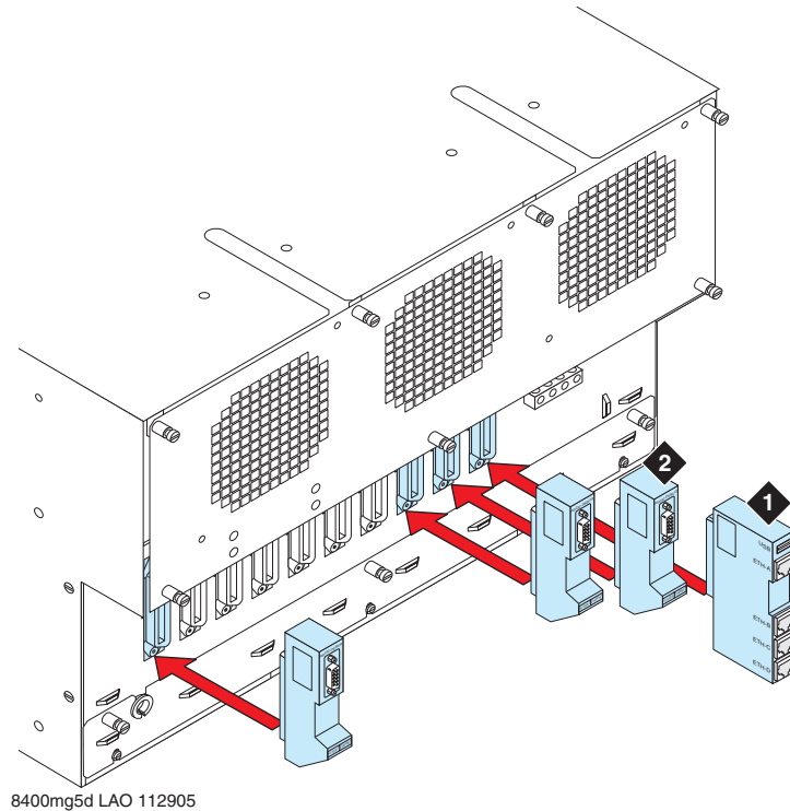
Figure 7: TN8412AP and TN8400AP backplane connectors on a G600 Media Gateway
