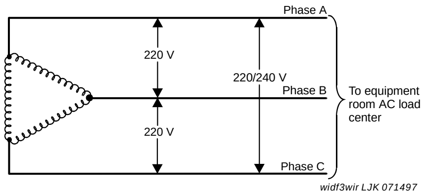
Figure 100: International delta, 220- or 240-VAC, 50-Hz source
