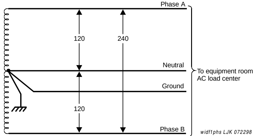
Figure 97: Single-phase, 120- to 240-VAC, 60-Hz source
