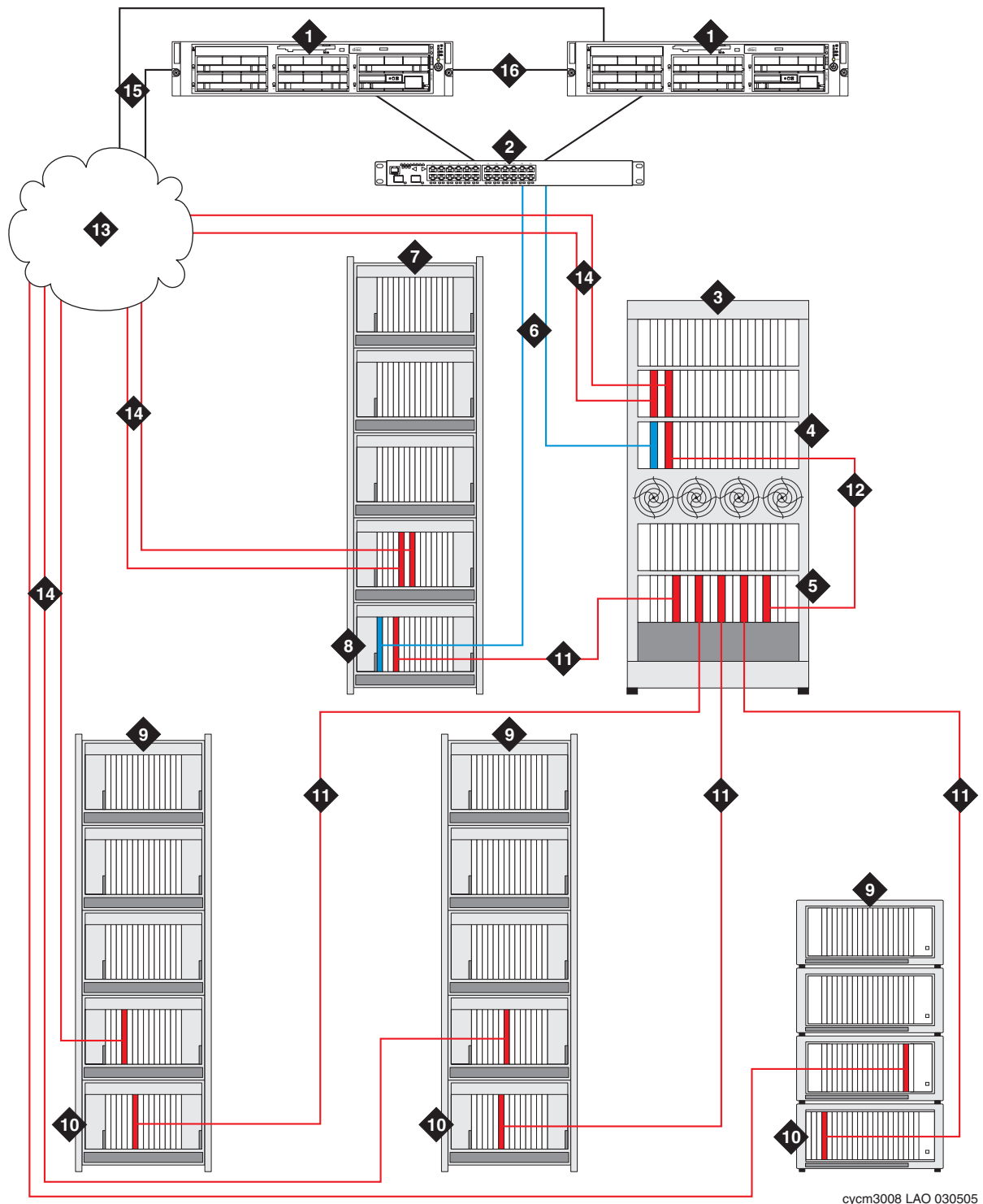
Figure 29: S8700-series Center Stage Switch single control network
