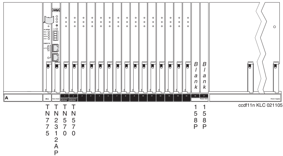
Figure 71: Expansion control cabinet (J58890N)
