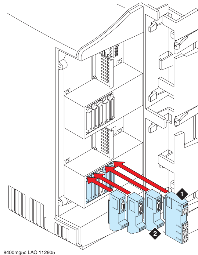
Figure 6: TN8412AP and TN8400AP backplane connectors on a CMC1
