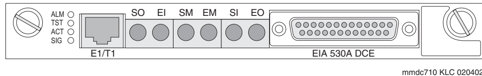
Figure 84: Avaya MM710 T1/E1 Media Module
