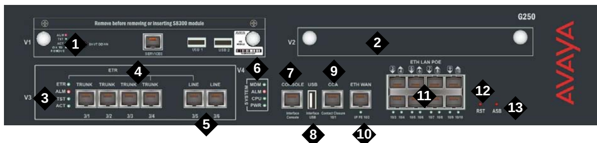
Figure 3: S8300 Media Server in a G250 Media Gateway (analog version)
