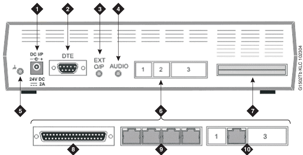
Figure 49: G150 4T+4A (16 VoIP) Back Panel
