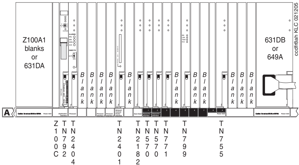
Figure 75: Control carrier (J58890AH)
