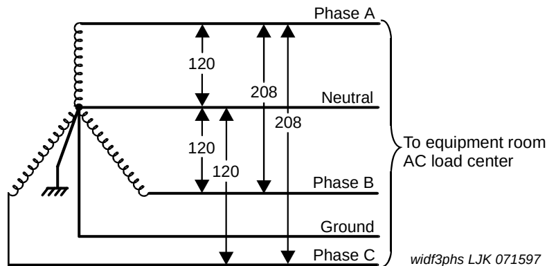
Figure 98: 3-phase, 120- to 208-VAC, 60-Hz source
