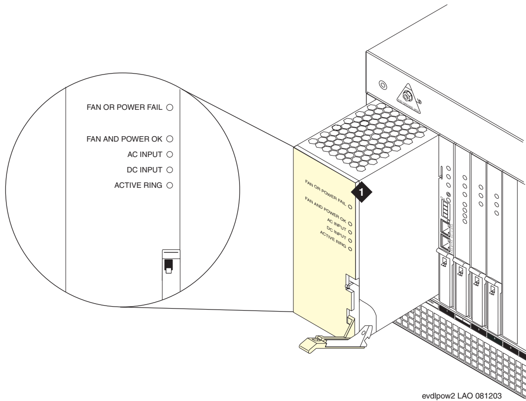
Figure 79: 655A faceplate LEDs
