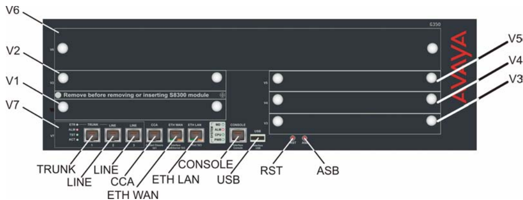
Figure 55: G350 chassis
