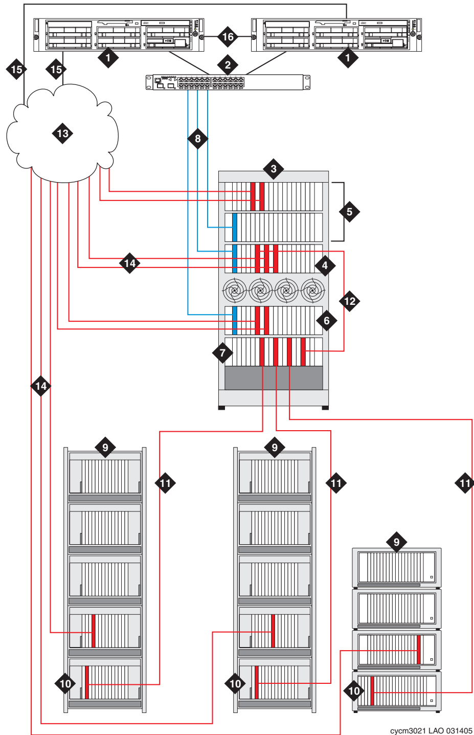
Figure 43: MCC1 Media Gateway with IP- and fiber-PNC PNs example
