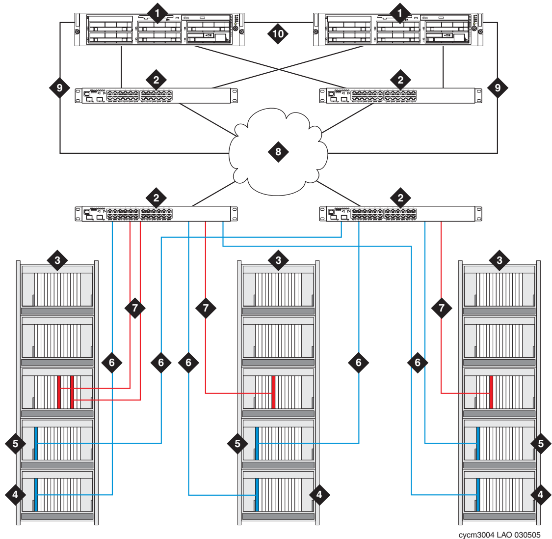
Figure notes: S8700-series IP-PNC duplicated control network
