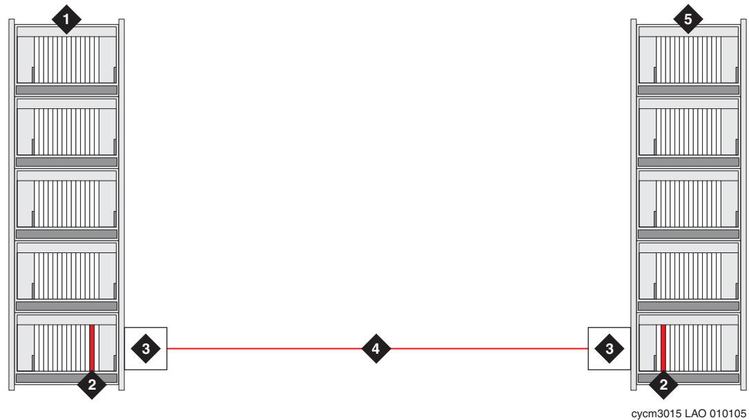
Figure 35: TN570B Expansion Interface PN connections up to 200 ft.
