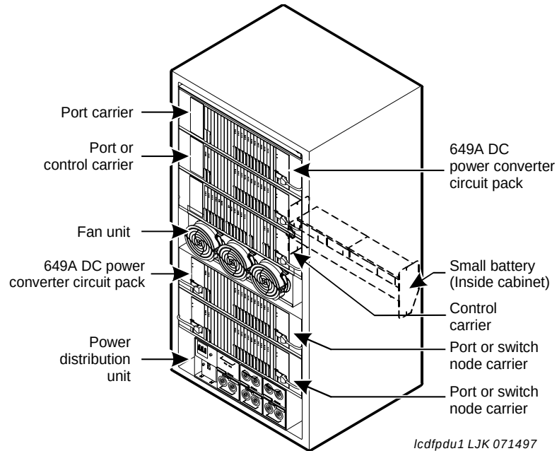
Figure 108: Power distribution in MCC1
