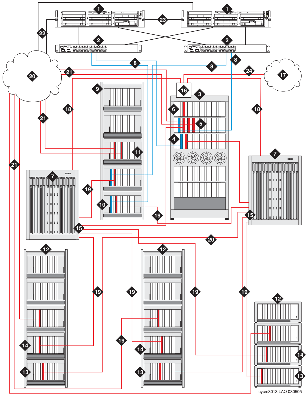
Figure 34: S8700-series ATM duplicated control and duplicated voice-bearer networks
