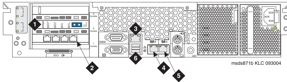
Figure 16: S8710 Media Server (back view)
