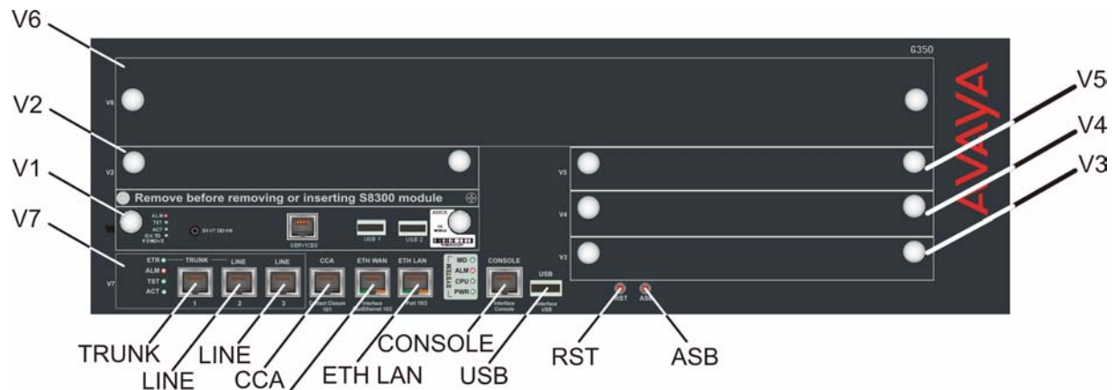
Figure 2: S8300 Media Server in a G350 Media Gateway
