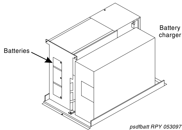
Figure 102: Battery charger (optional part of J58890CE-2) (front)
