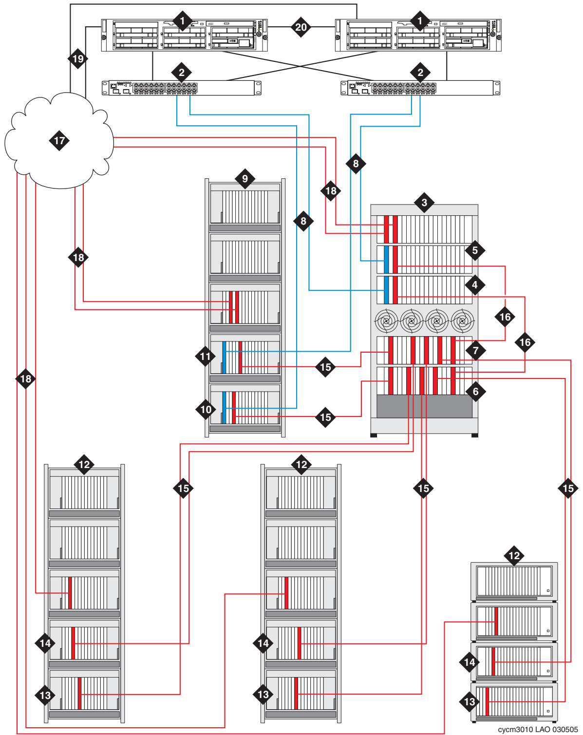
Figure 31: S8700-series Center Stage Switch duplicated control and duplicated voice-bearer networks
