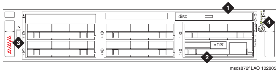
Figure 17: S8720 Media Server (front view)
