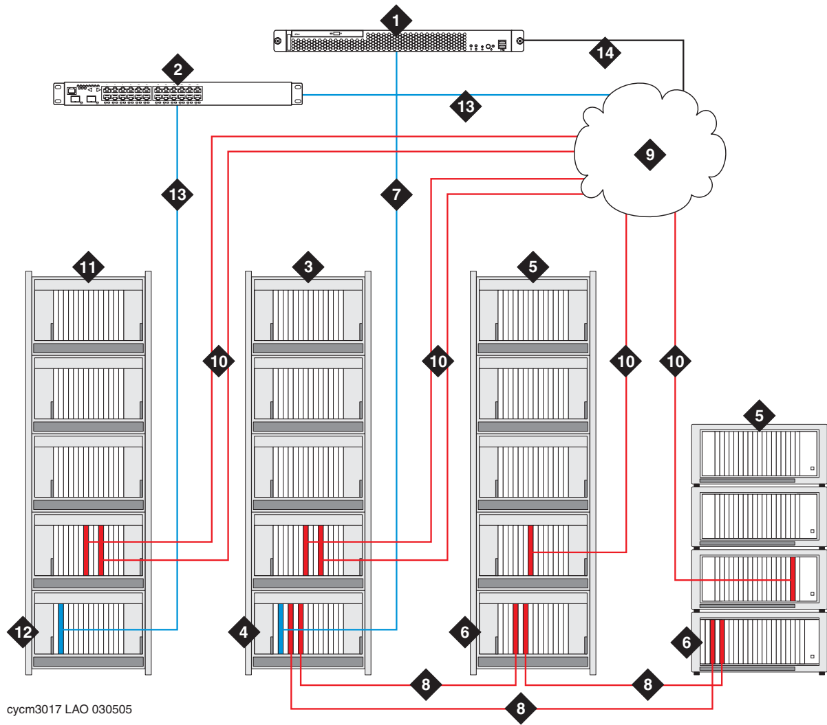
Figure notes: Direct- and IP-PNC PNs example (with S8500 Media Server)
