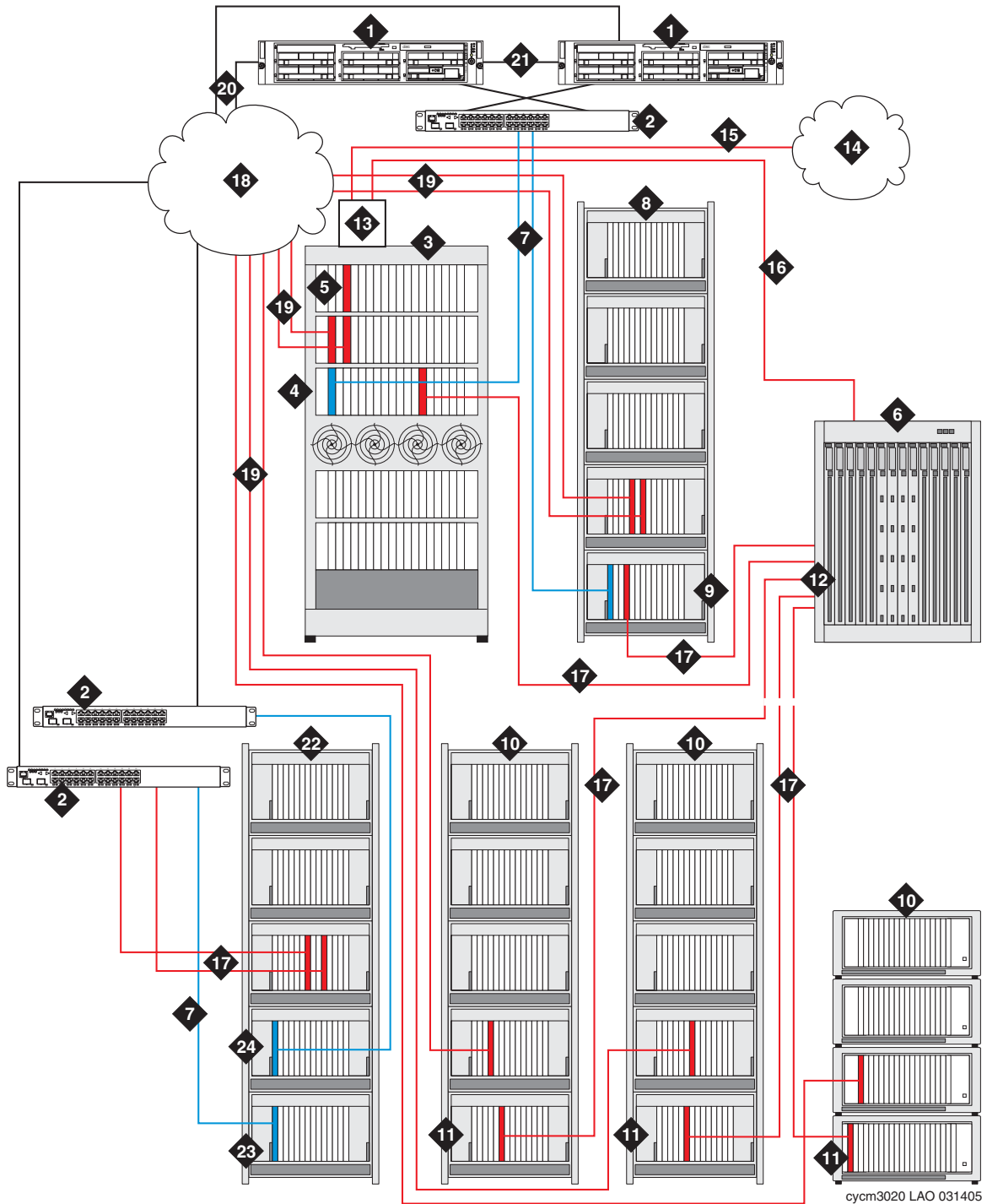
Figure 41: Example of ATM-connect PNs with single control network and IP-PNC PNs with duplicated control network
