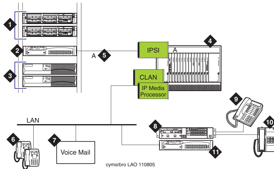
Figure 58: The G700 Media Gateway connecting to the S8700-series Media Server
