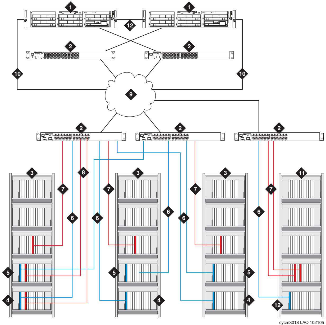
Figure notes: IP-PNC PNs with single, duplicated control networks, and duplicated control/bearer network (with S8700-series Media Server)
