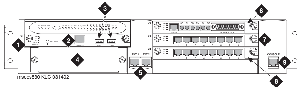
Figure 1: S8300 Media Server in a G700 Media Gateway
