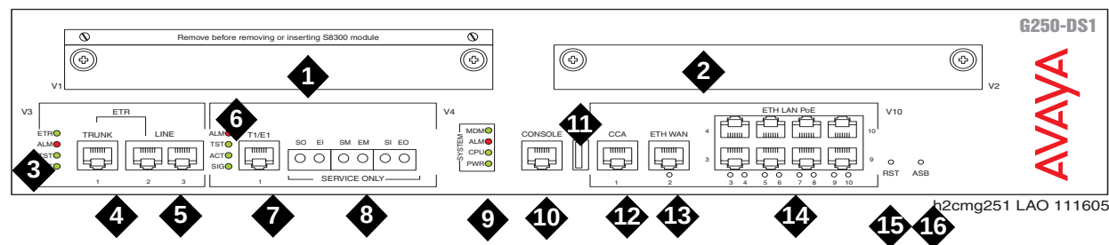
Figure 54: The Avaya G250-DS1 Media Gateway Chassis
