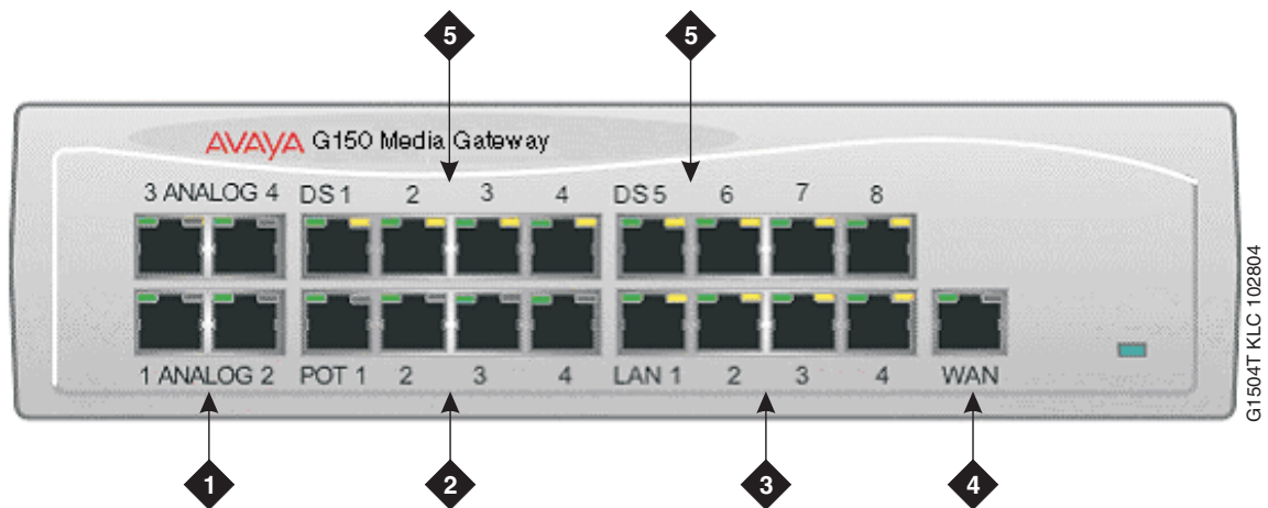
Figure 48: G150 4T+4A (16 VoIP) Front Panel
