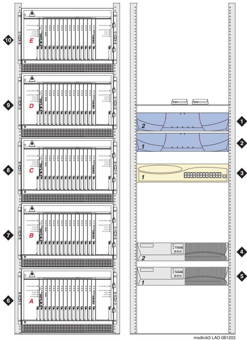
Figure 63: G650 stack
