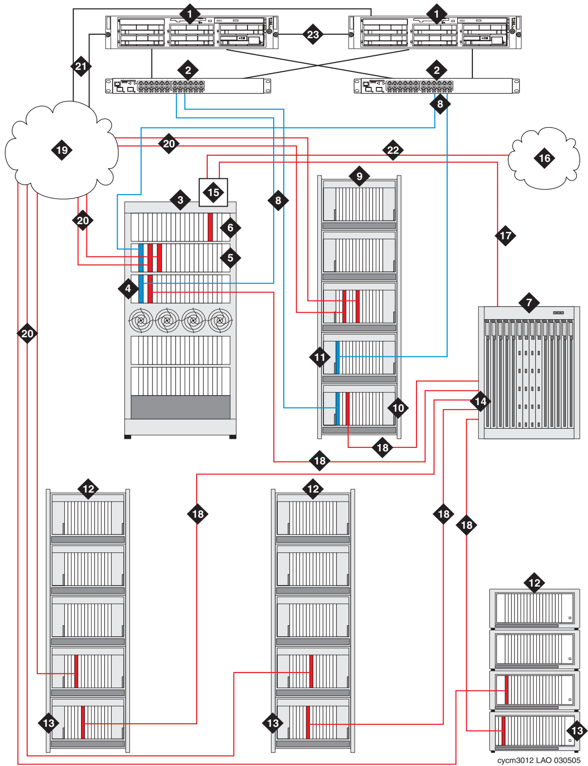
Figure 33: S8700-series ATM duplicated control networks
