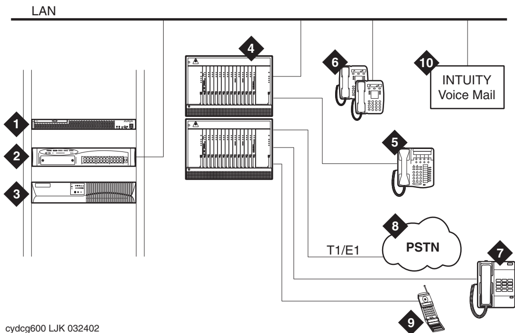
Figure 111: A medium-sized business solution using the Avaya S8500 Media Server and the G650 Media Gateway
