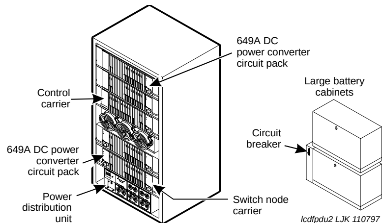
Figure 109: DC power distribution in MCC1s
