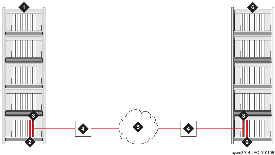
Figure 37: TN1654 DS1 Converter/TN570B Expansion Interface PN connections up to 200 miles.
