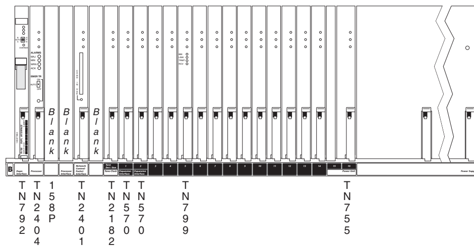
Figure 70: Duplicated control cabinet (J58890M)
