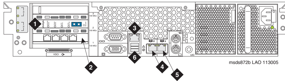
Figure 18: S8720 Media Server (back view) with hardware duplication
