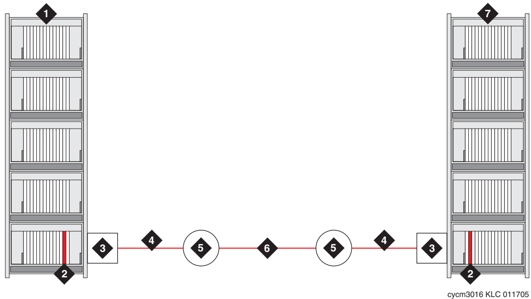
Figure 36: TN570B Expansion Interface PN connections up to 4900/25000 ft. and 22 miles.
