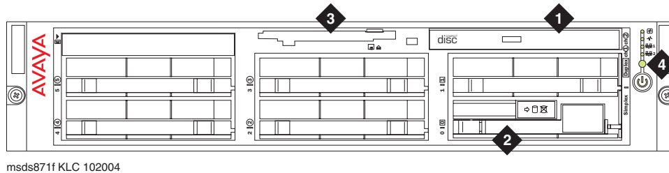
Figure 15: S8710 Media Server (front view)
