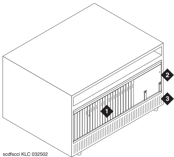
Figure 67: Typical SCC1 Media Gateway
