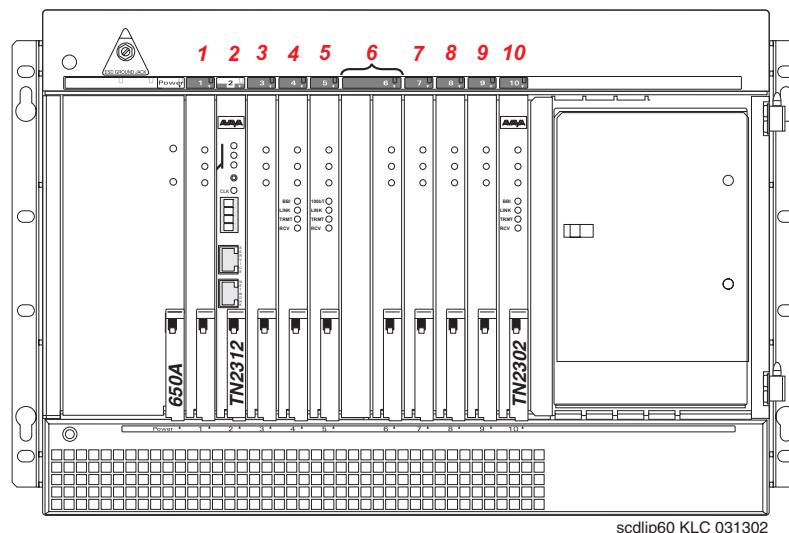
Figure 60: G600 Media Gateway
