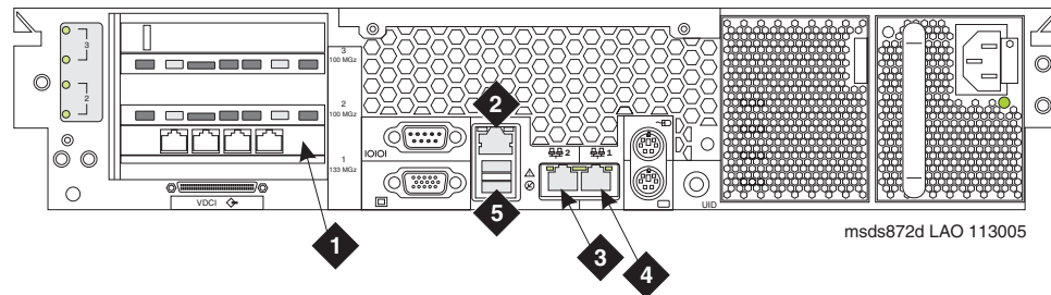
Figure 19: S8720 Media Server (back view) with software duplication
