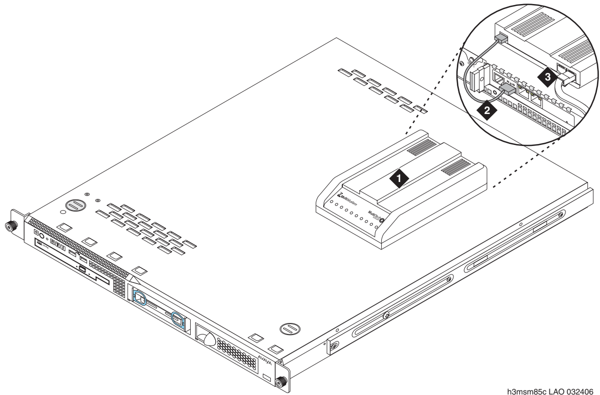
Figure 12: Modem connectivity to the S8500C
