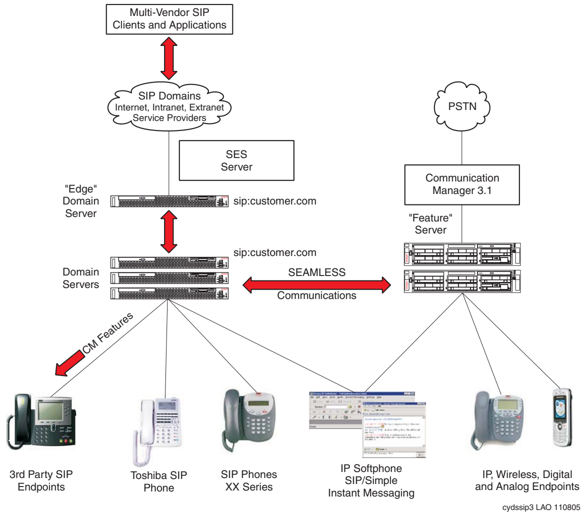
Figure 44: SIP Architecture
