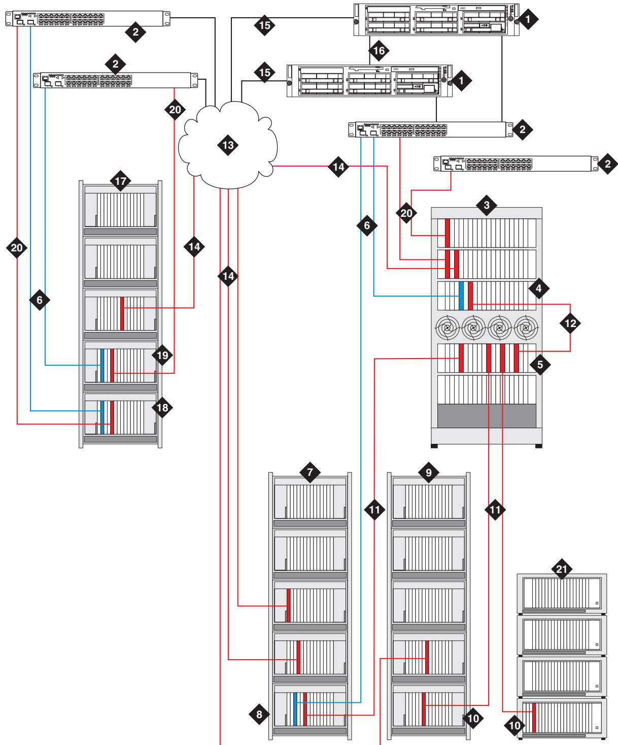
Figure 40: CSS-connected PNs (single control network) and IP-PNC PN (duplicated control and duplicated bearer network) example
