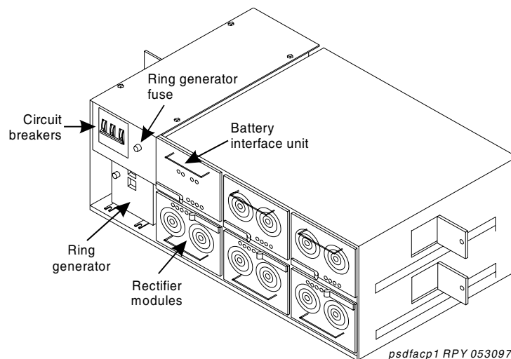
Figure 104: AC power-distribution unit (J58890CH-1) (front)
