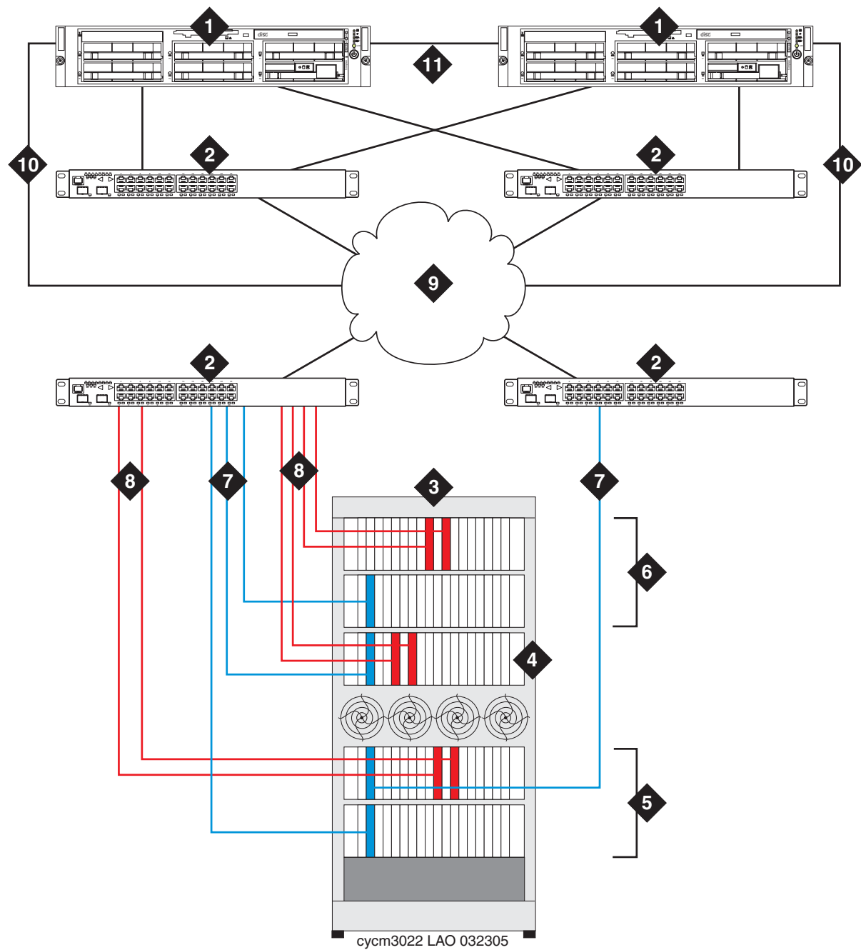
Figure 42: MCC1 Media Gateway with carriers as IP-PNC PNs (duplicated control network) example
