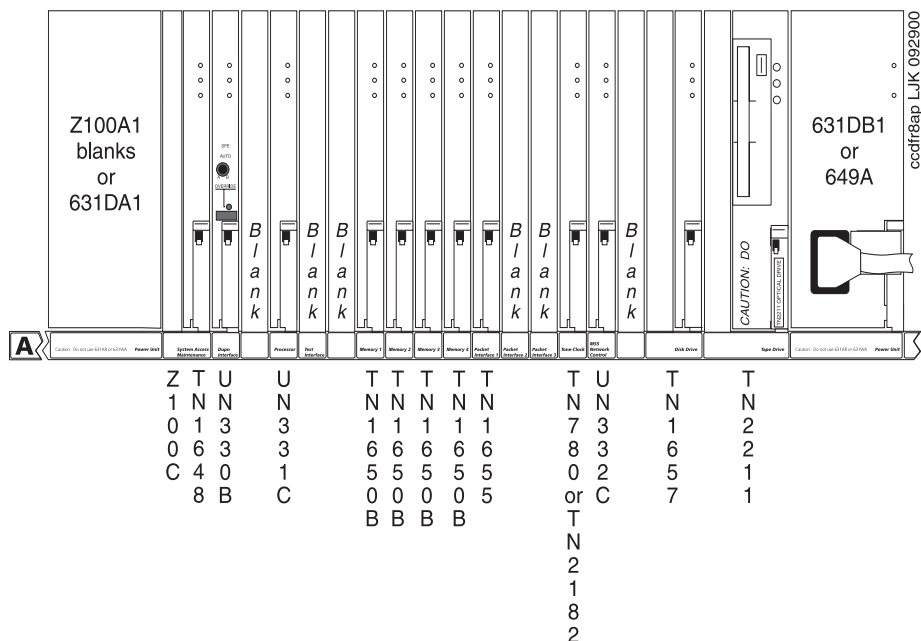
Figure 37. Processor Carrier (r model) (J58890AP) (Front)
