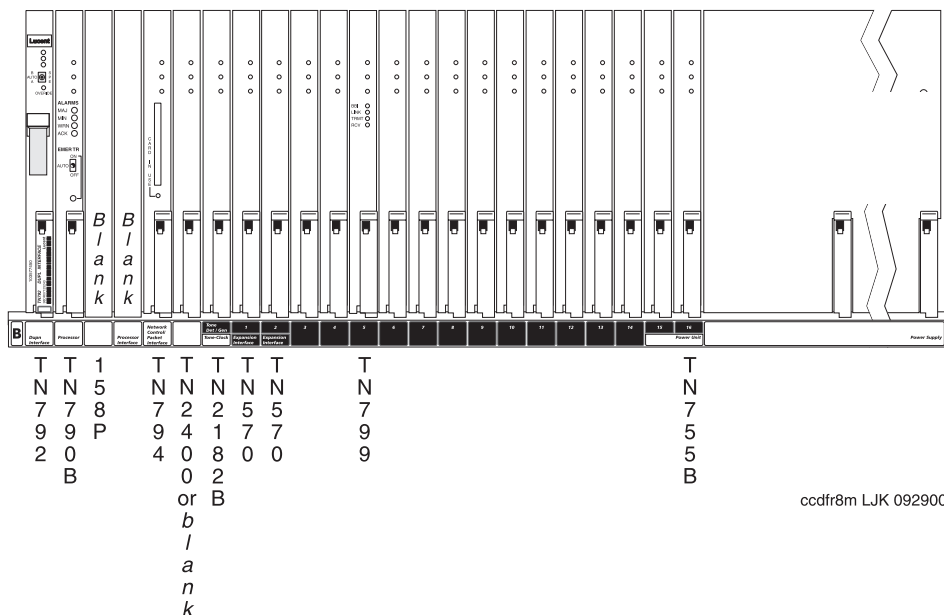
Figure 44. Duplicated Control Cabinet (J58890M) (Front)
