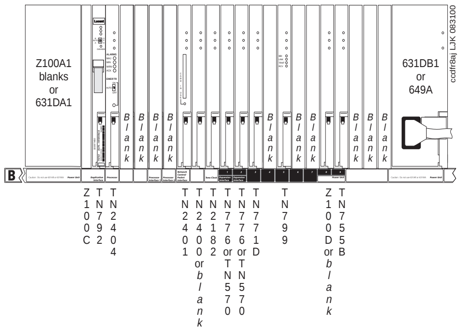
Figure 36. Duplicated Control Carrier (si model) (J58890AJ) (Front)
