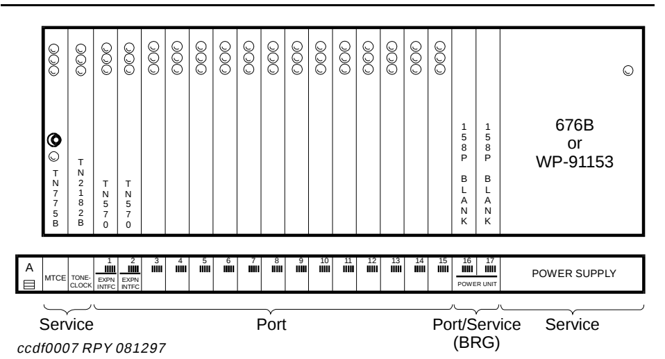
Figure 45. Expansion Control Cabinet (J58890N) (Front)
