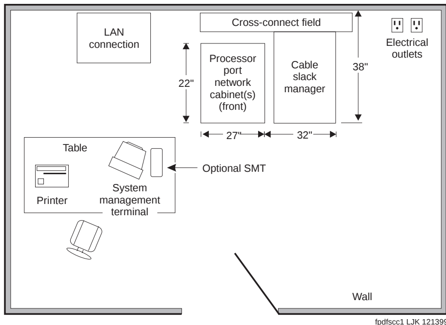
Figure 12. Typical Single-Carrier Cabinet Floor Plan
