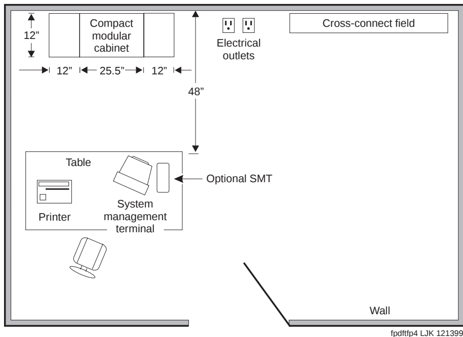
Figure 11. Typical Compact Modular Cabinet Floor Plan
