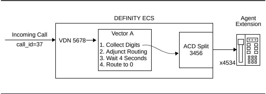
Figure B-12. Call Flow for Incoming Call to VDN Routed to ACD Split
