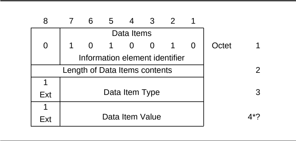
Figure 4-20. Data Item Information Element
