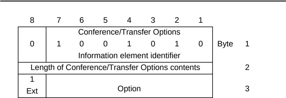
Figure 4-18. Conference/Transfer Options Information Element
