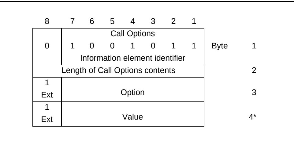
Figure 4-17. Call Options Information Element
