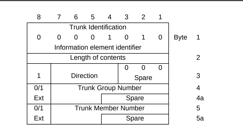
Figure 4-39. Trunk Identifier Information Elements
