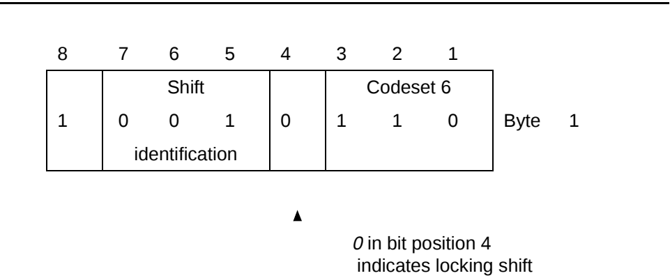
Figure 4-4. Locking Shift to Codeset 6
