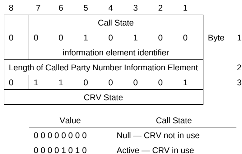
Figure 4-5. Call State Information Element
