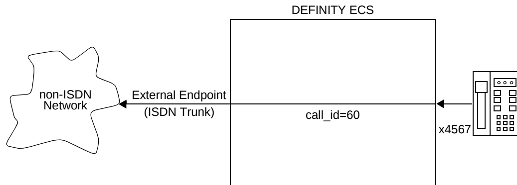
Figure B-48. Call Flow for Outgoing ISDN Call that Traverses a Non-ISDN Network
