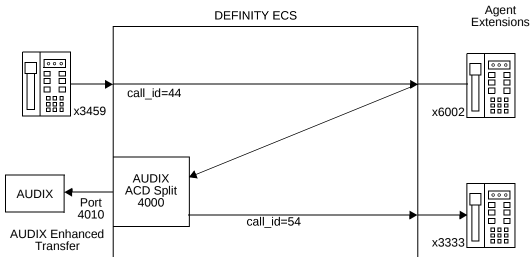
Figure B-31. Call Flow for Call Transferred out of AUDIX
