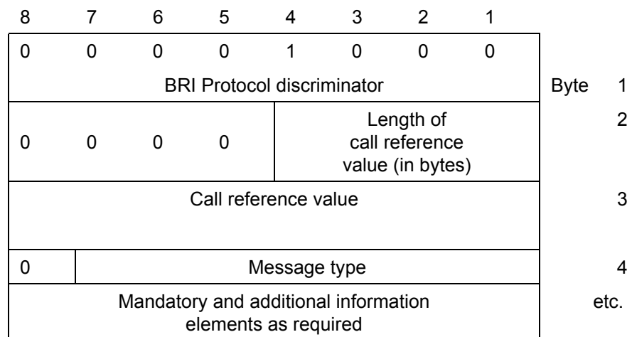
Figure 4-1: General Message Organization Example
