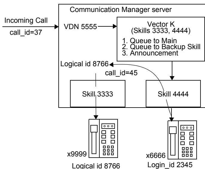
Figure B-37: Call Flow for Incoming Call to Skill VDN
