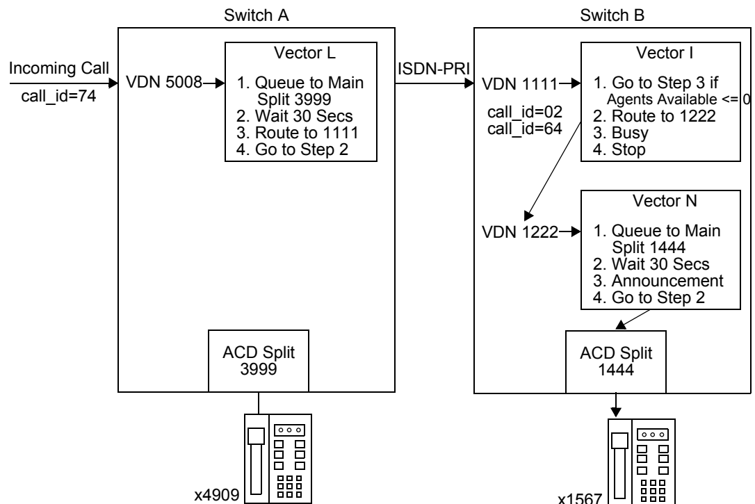
Figure B-35: Call Flow for Incoming Call to LookAhead Interflow Vector
