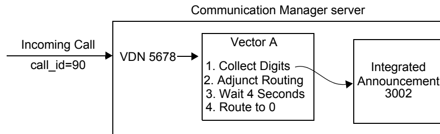
Figure B-7: Call Flow for Incoming Call to VDN Routed to Announcement
