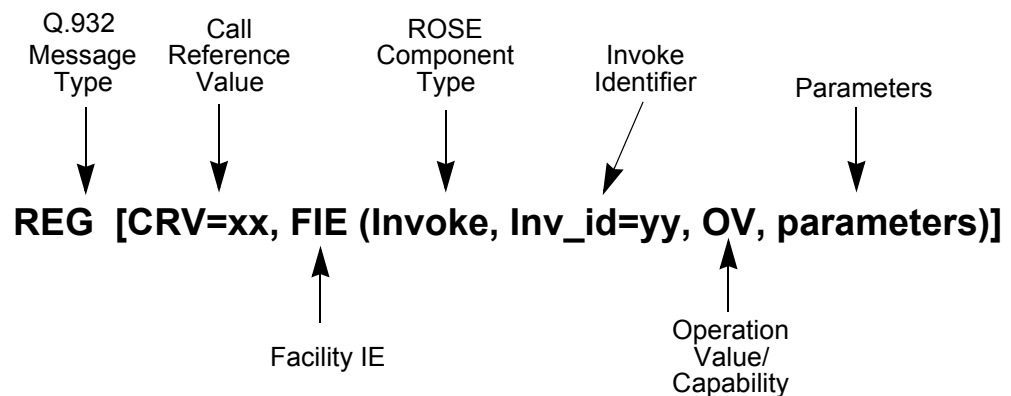
Figure B-1: Message Notation
