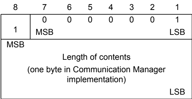
Figure 4-24: Long Form of the Length Field in Communication Manager Implementation (2 Bytes)
