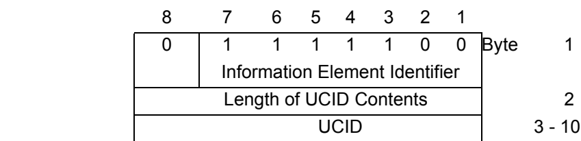
Figure 4-41: UCID Identifier Information Elements
