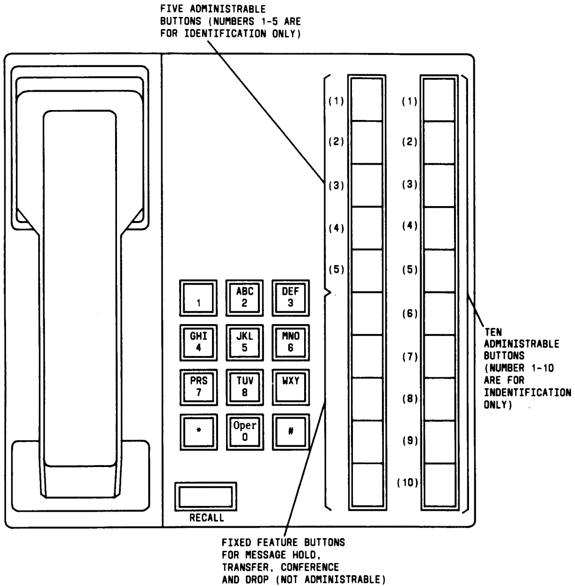
Figure 6-12. 20-Button MET Voice Terminal
