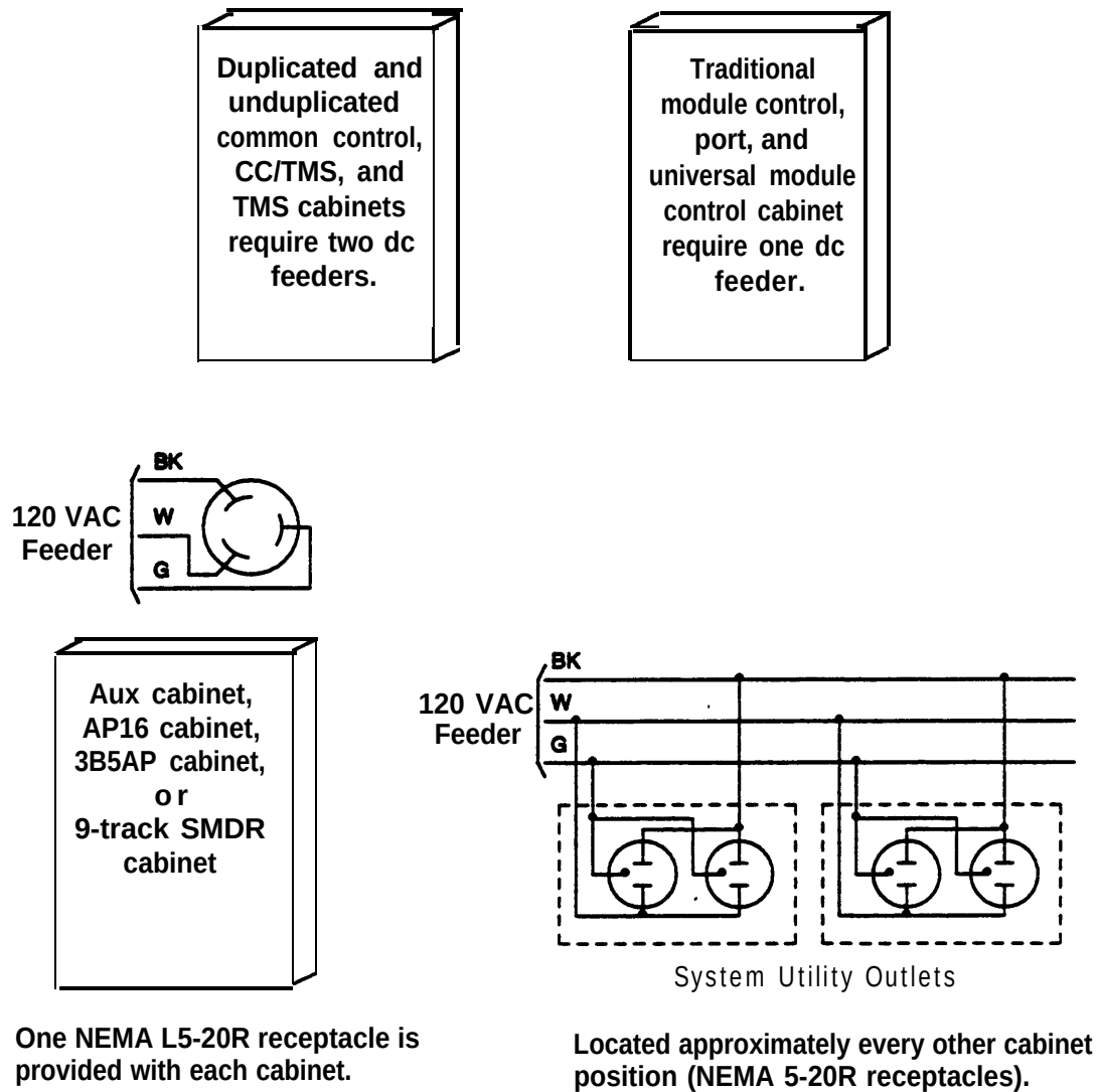
Figure 10-16. System Equipment Feeders with -48 Volt DC Standby Power
