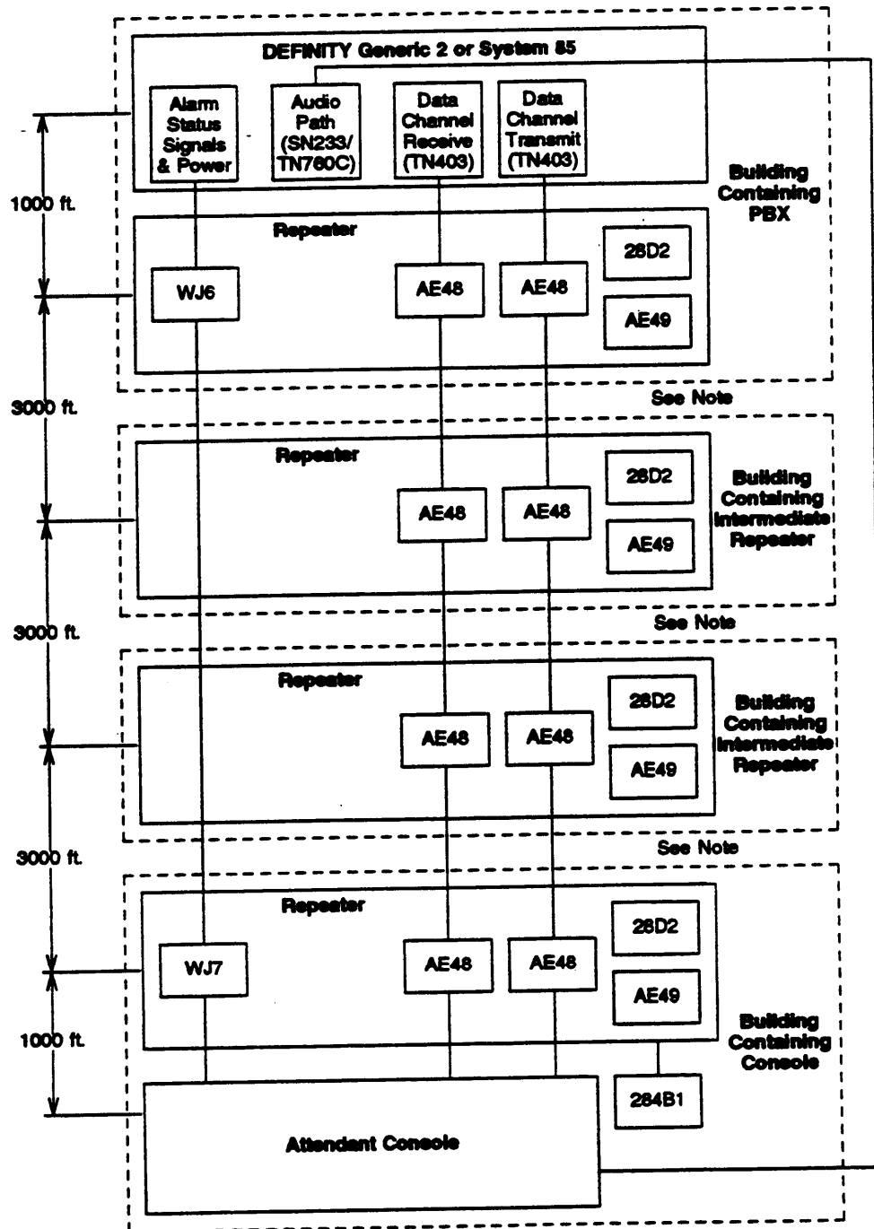
Figure 4-5. Off-Premises Attendant Console Using Cascaded Repeaters
