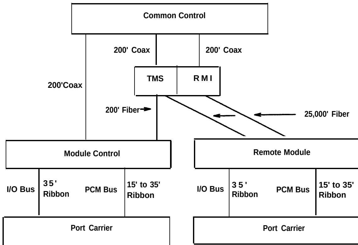
Figure 9-2. Distance Limits for Switch Modules
