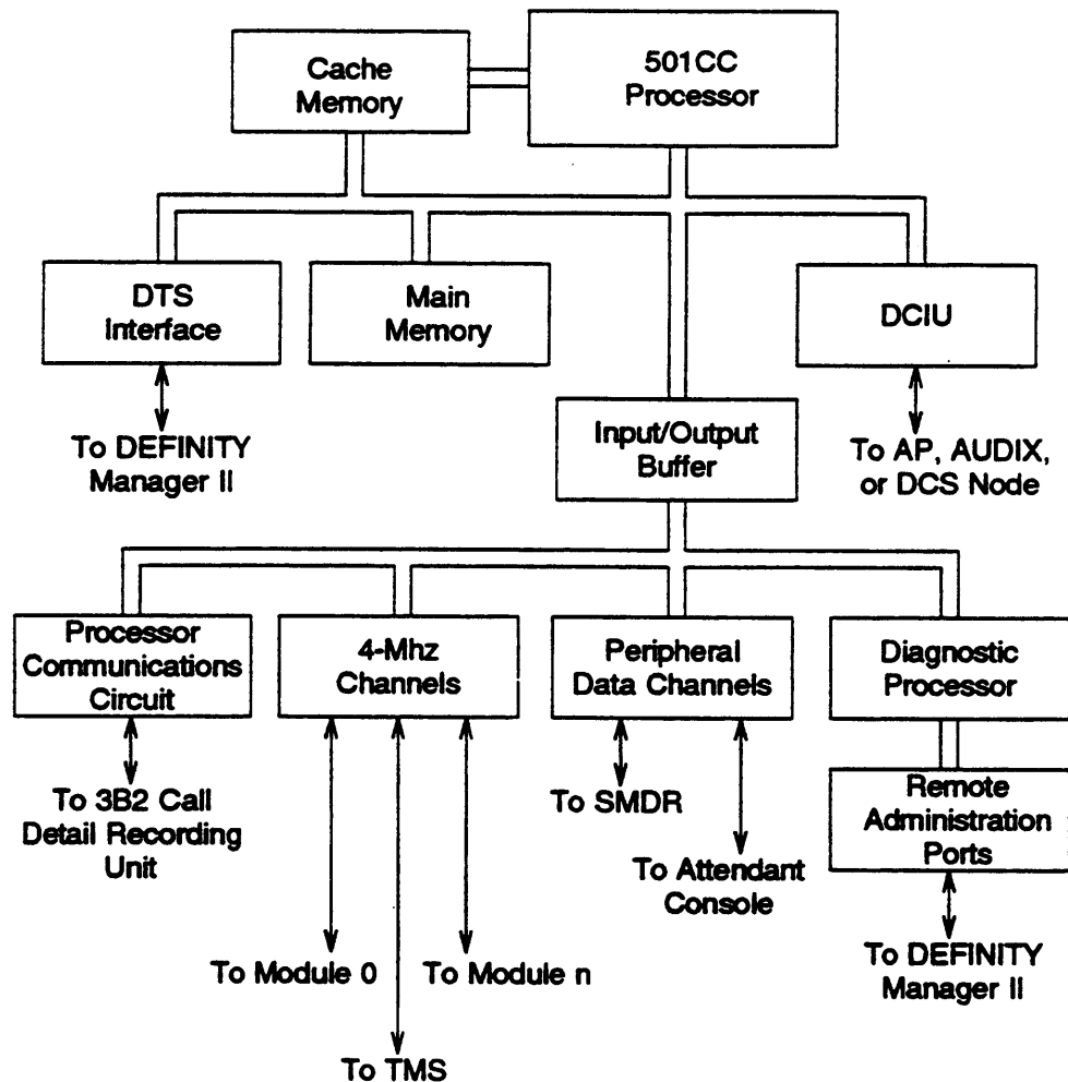
Figure 2-2. Common Control
