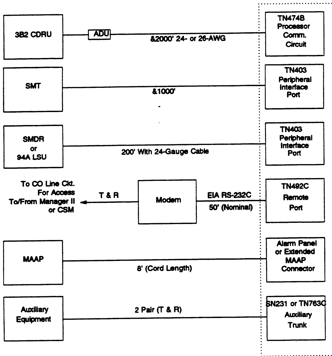
Figure 9-3. Distance Limits for Miscellaneous Peripherals
