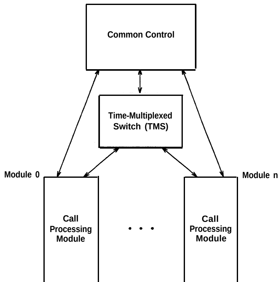
Figure 2-1. Multimodule Switch
