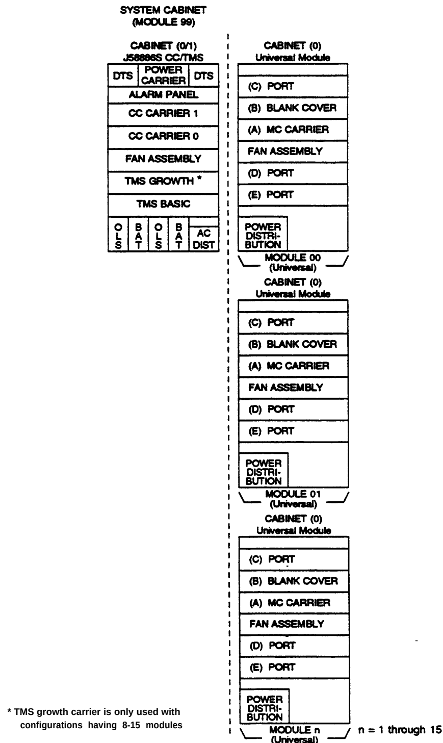
Figure 3-18. Sample Configuration for High Reliability, 1 through 15 Modules
