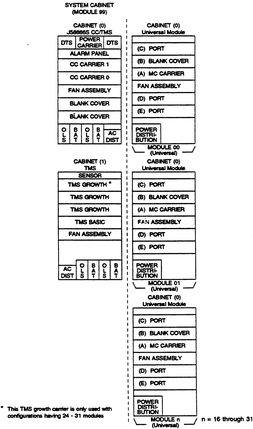
Figure 3-19. Sample Configuration for High Reliability, 16 through 31 Modules
