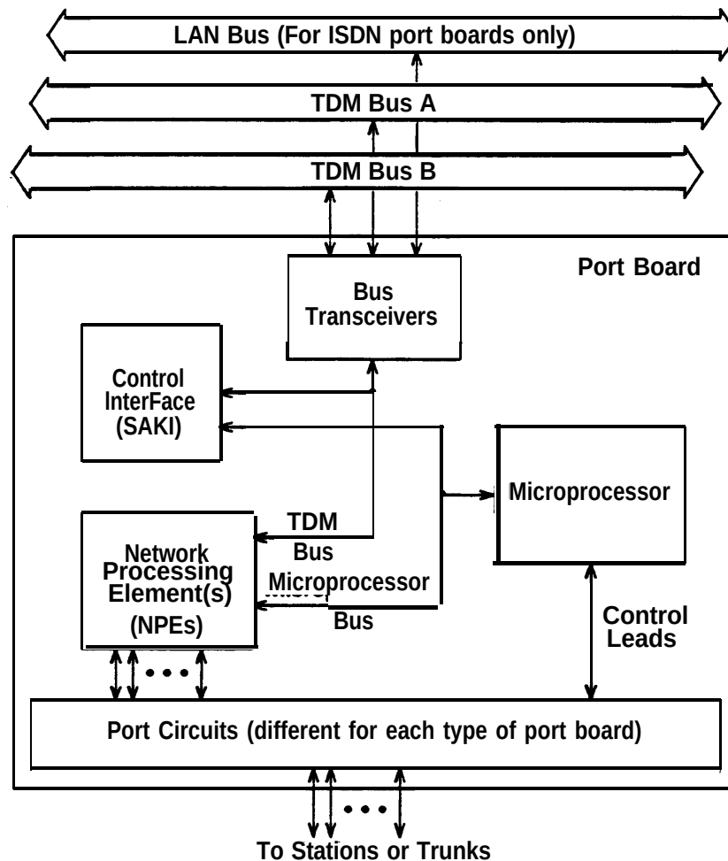
Figure 2-8. Port Board Architecture
