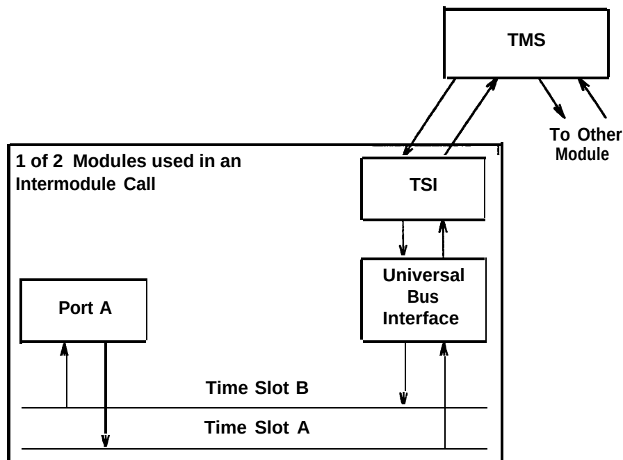
Figure 2-10. Intermodule Connection
