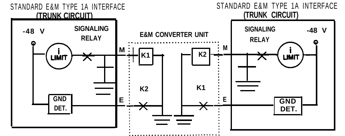
Figure 3-43. Type 1 E&M Signaling Using Trunk Circuits and a Converter Unit
