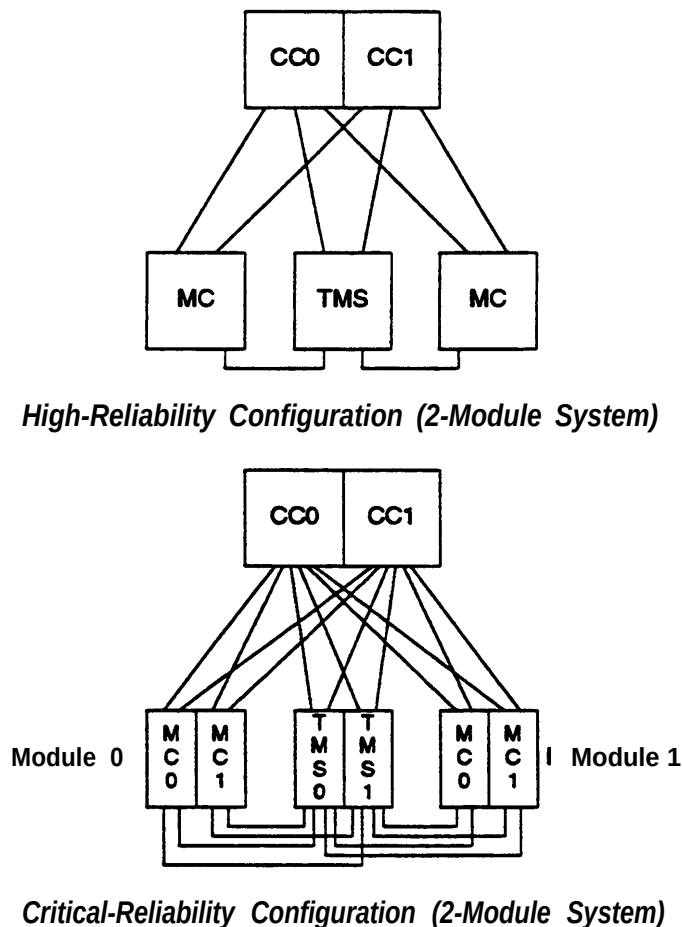
Figure 2-13. Intercabinet Connections for Systems With Duplication
