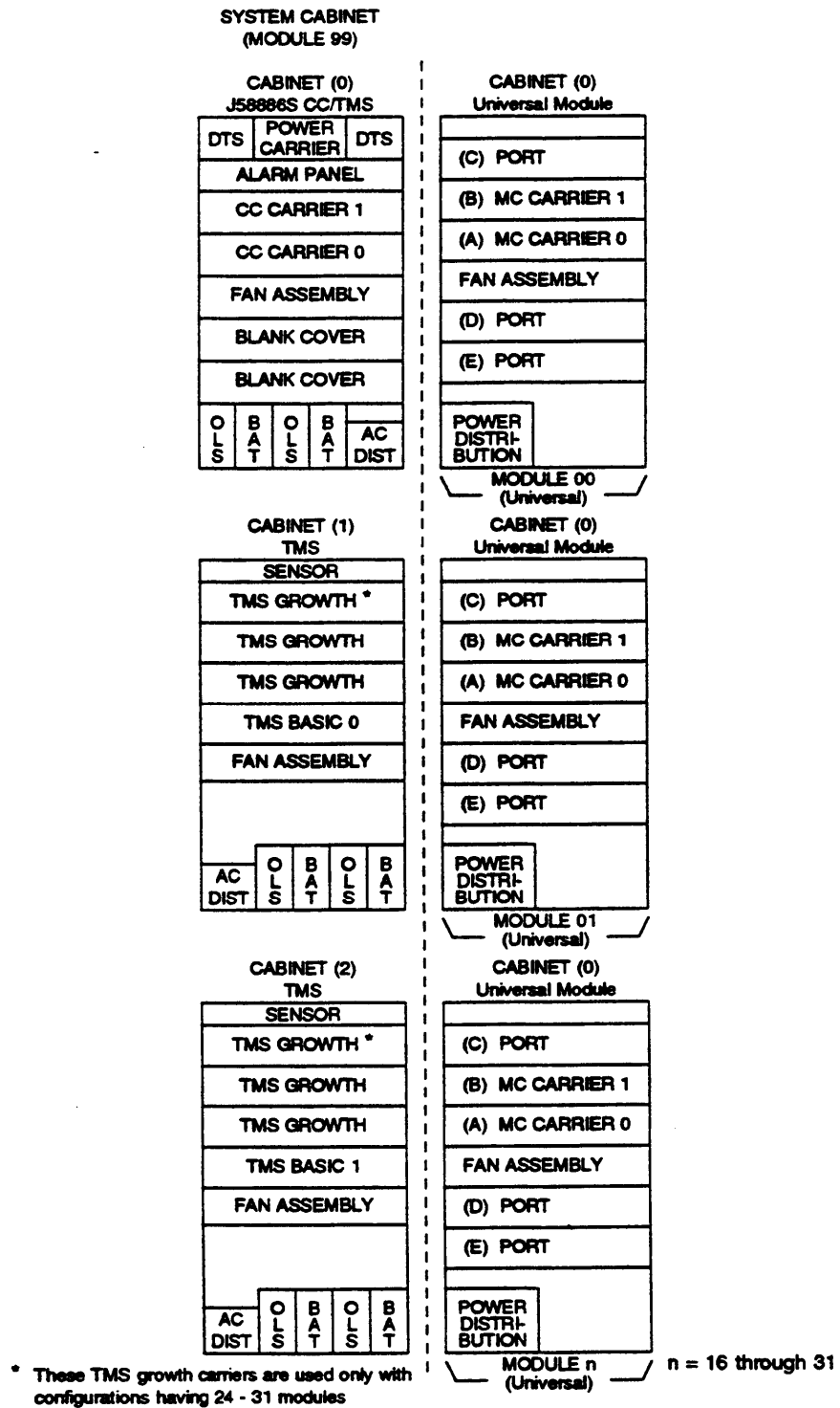
Figure 3-23. Sample Configuration for Critical Reliability, 16 through 31 Modules
