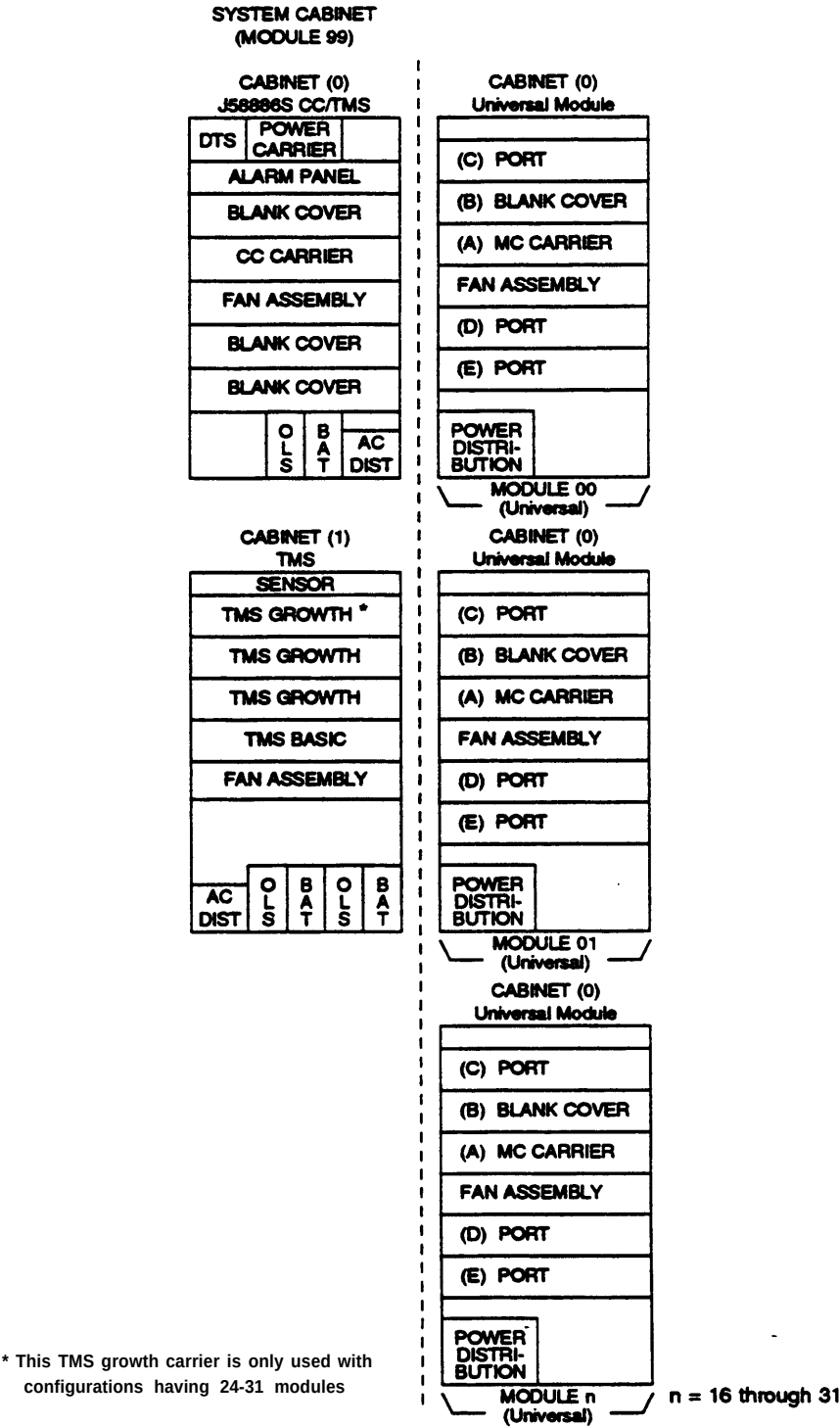
Figure 3-16. Sample Configuration for Standard Reliability, 16 through 31 Modules
