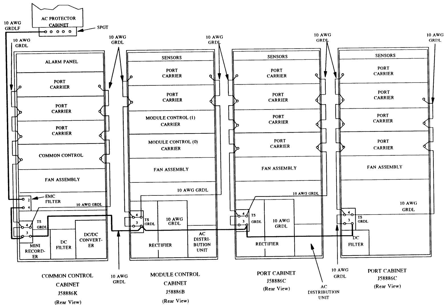
Figure 8-12. GRDLF — Unduplicated System
