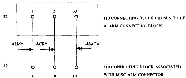
Figure 14-5. Cross-Connect
