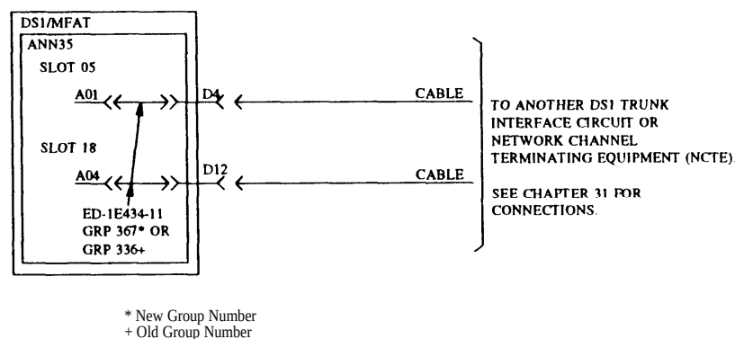
Figure 10-15. ANN35 ISDN Primary Rate Port Located in DS1/MFAT
