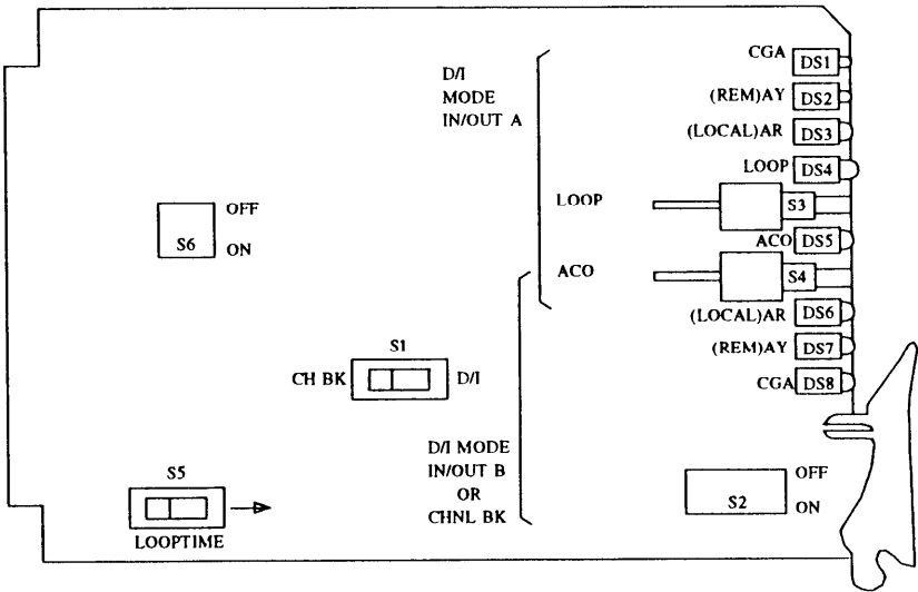
Figure 13-16. Switch Locations
