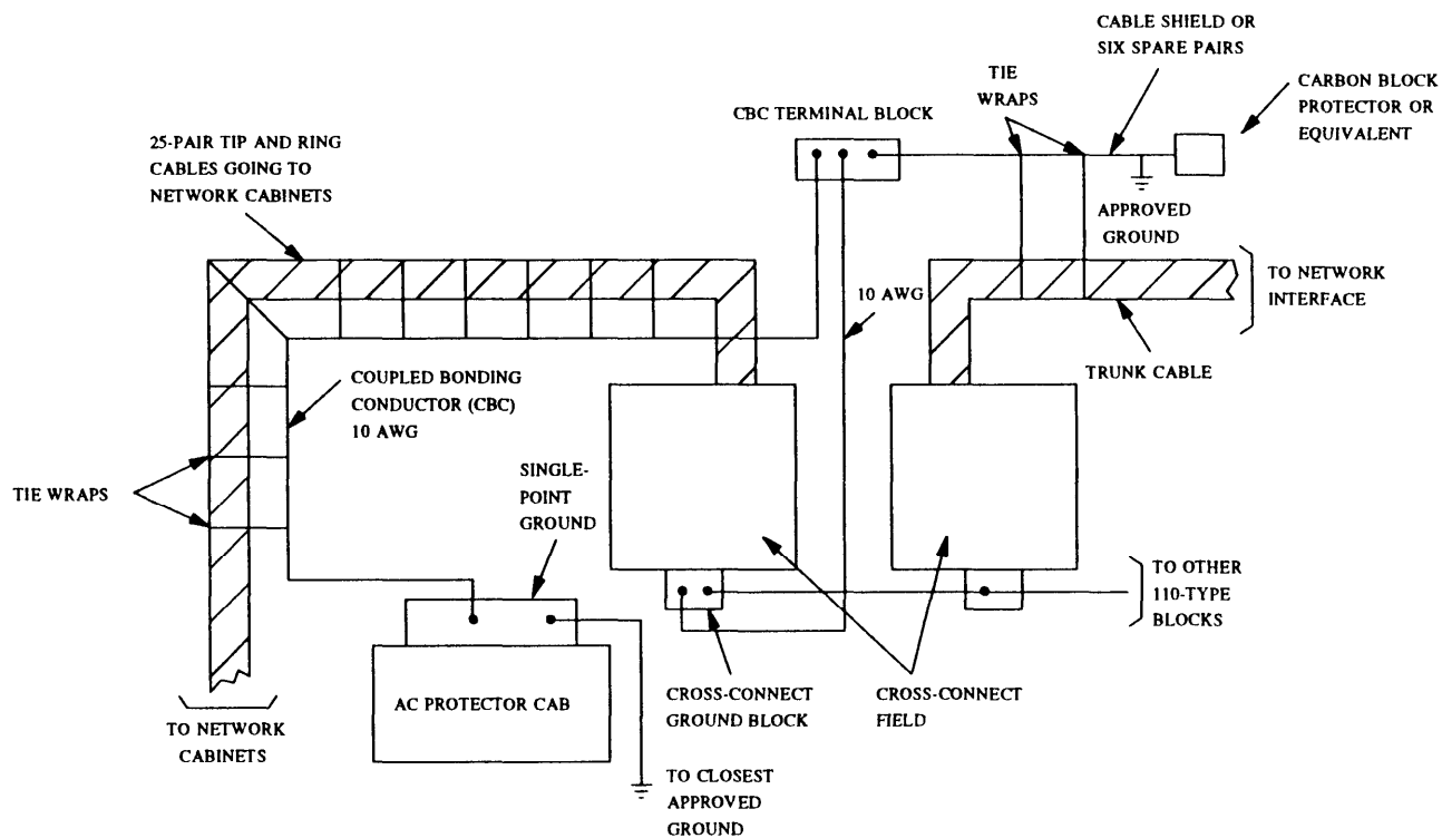
Figure 8-14. CBC Grounding
