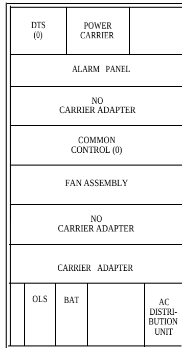
CC/TMS CABINET J58886S-2 (Front View)
