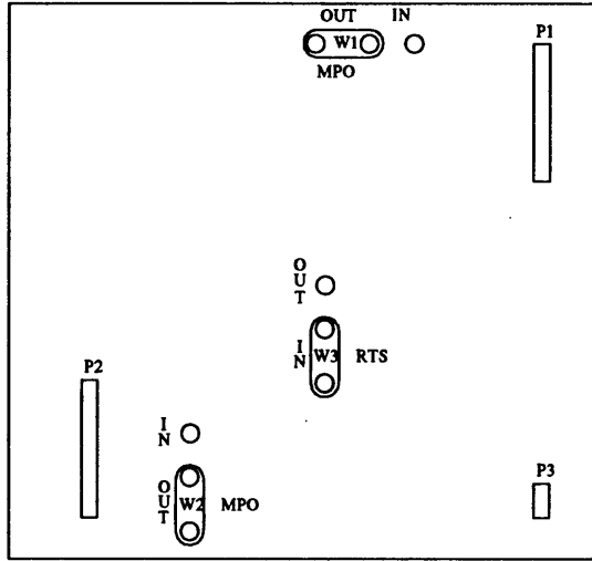
Figure 31-8. RS-422 Interface Subboard Switch Locations
