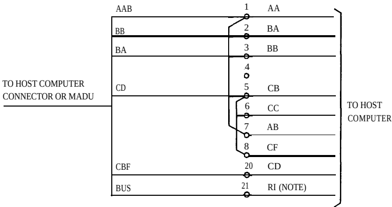
Figure 32-46. M48G Octopus Cable Connecting Information
