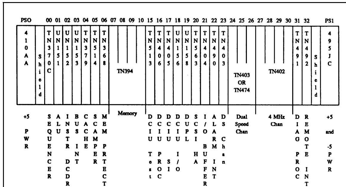
Figure 22-16. CC/TMS J58888AB-1 CC Circuit Pack Locations
