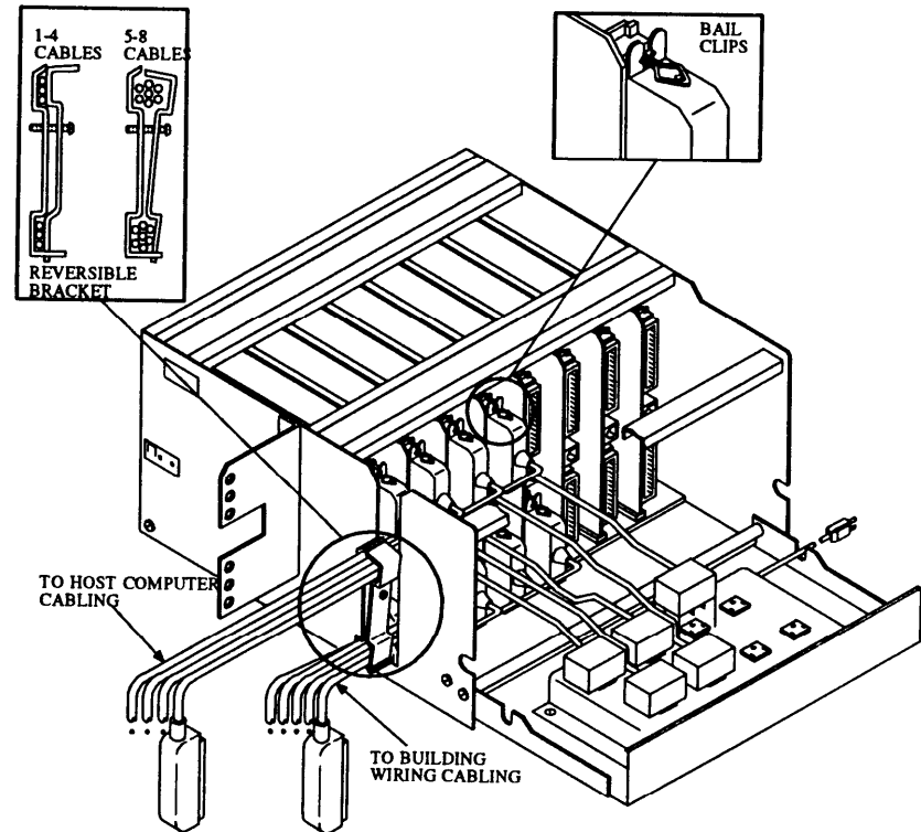
Figure 32-44. Cable Routing for Multiple Mounted MADU
