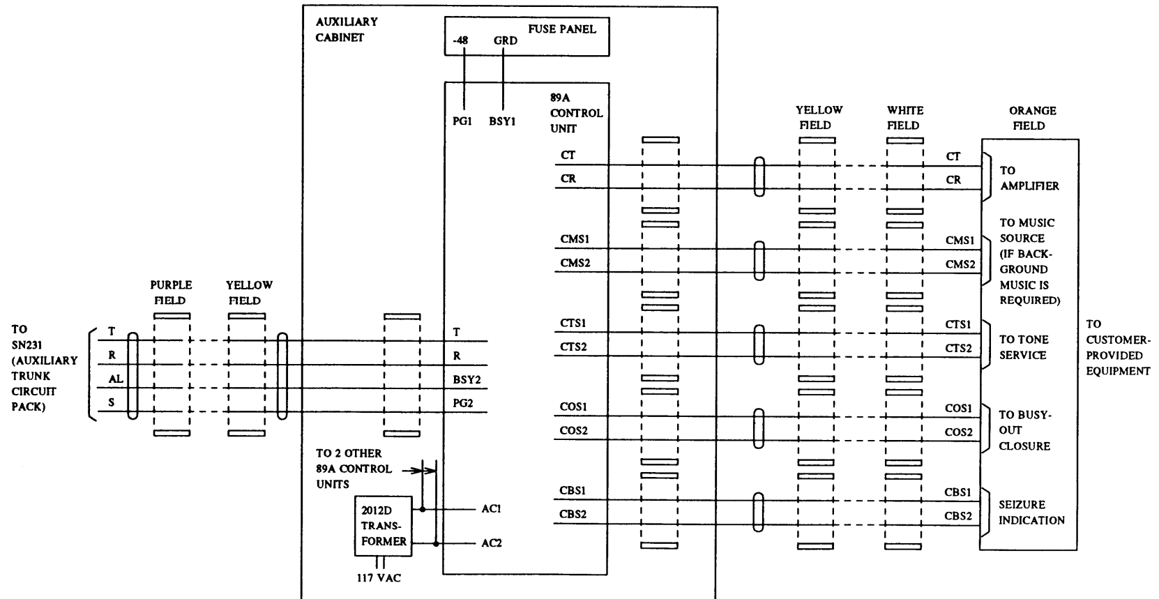
Figure 30-4. 89A Control Unit Connections — Loudspeaker Paging Feature
