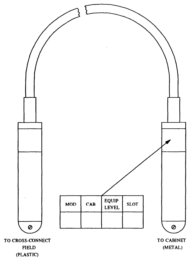
Figure 25-2. Circuit Pack Location Label on Connector Hood
