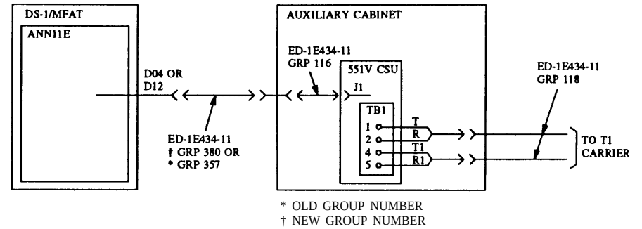
Figure 31-14. Equipment Located in Auxiliary Cabinet (Using a 551V CSU)
