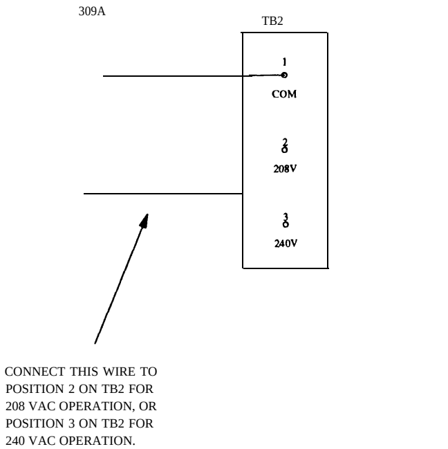
Figure 7-8. 309A/310A VAC Power Tap Input Connection
