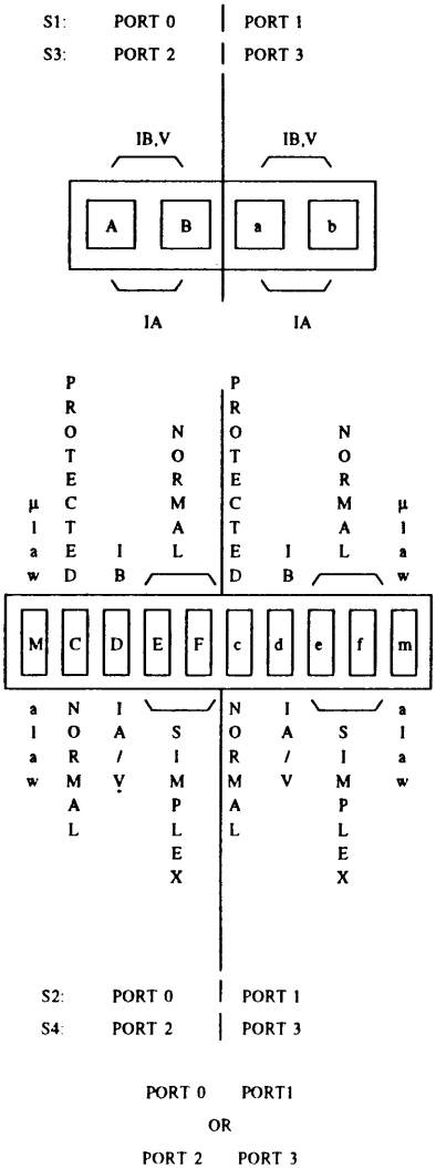
Figure 17-20. SN233C Port Settings
