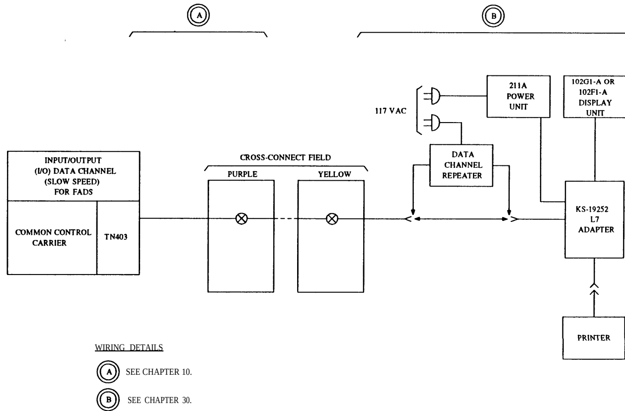
Figure 18-12. FADS
