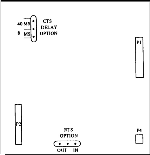
Figure 13-21. RS232C Switch Locations
