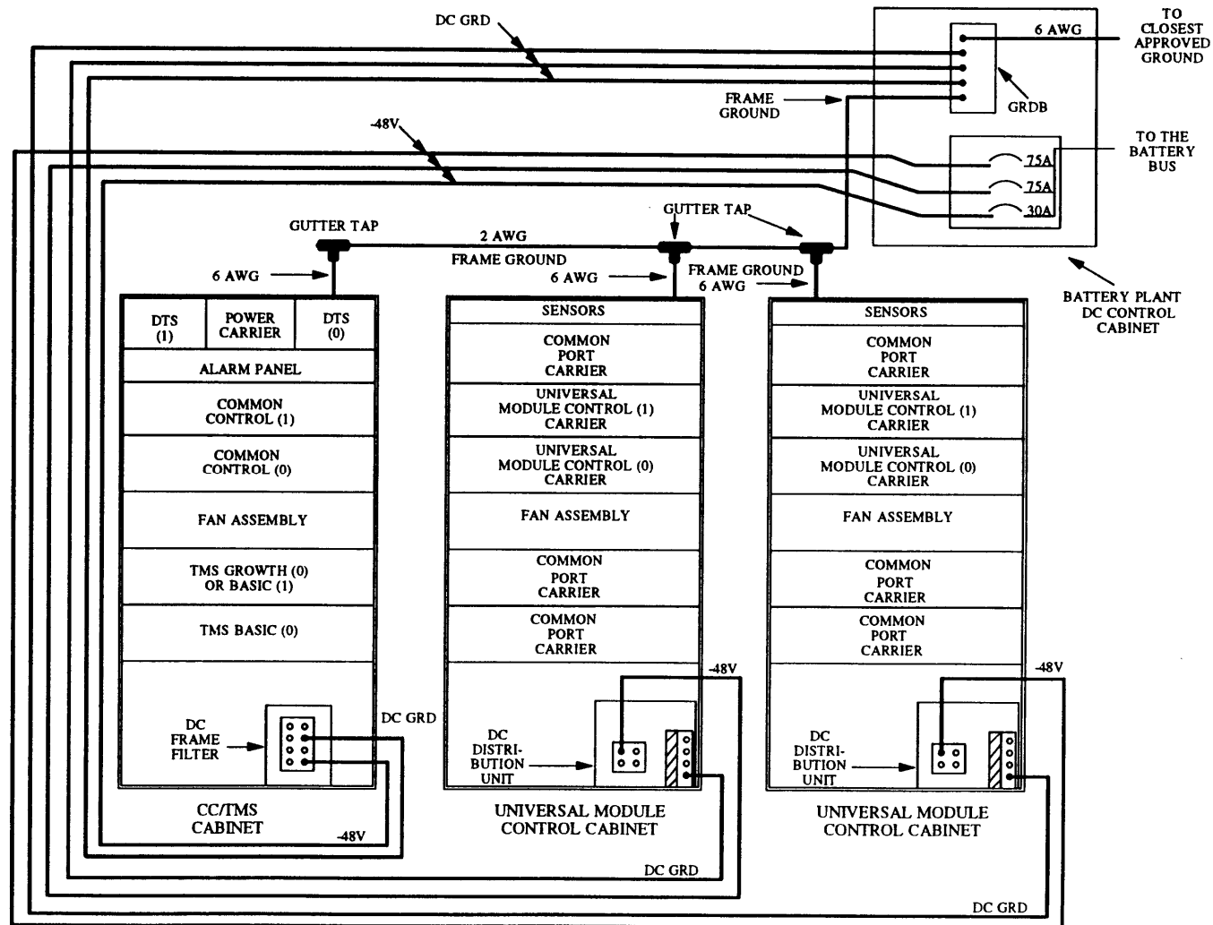
Figure 24-16. Typical DC Power and Grounding Scheme for DEFINITY Generic 2 (illustrated)
