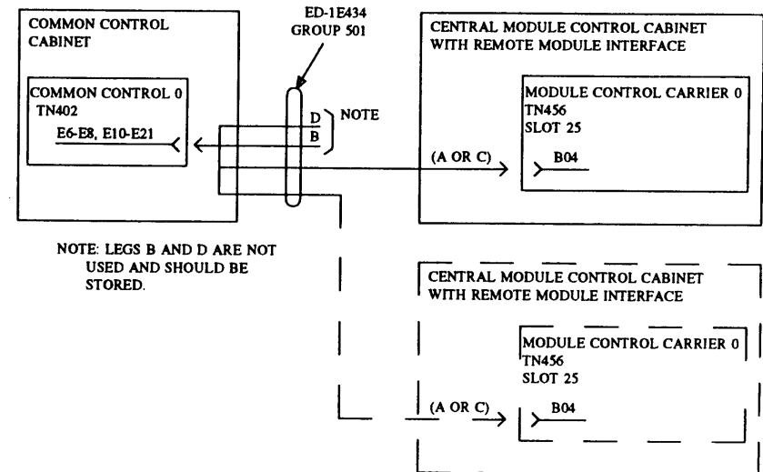
Figure 26-31. ED-1E434, Group 501 Connections for an All Unduplicated System (Phase 1)
