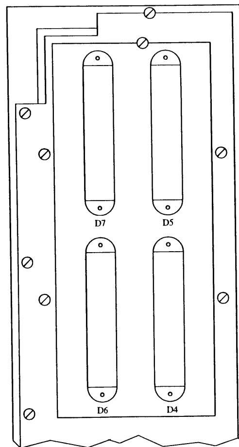
Figure 10-3. D4-D7 Connector Locations (New Cabinets)
