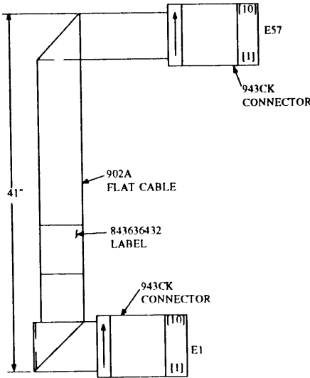
Figure 12-24. ED-1E434, Group 25 Cable
