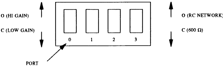
Figure 17-25. SN243B Switch
