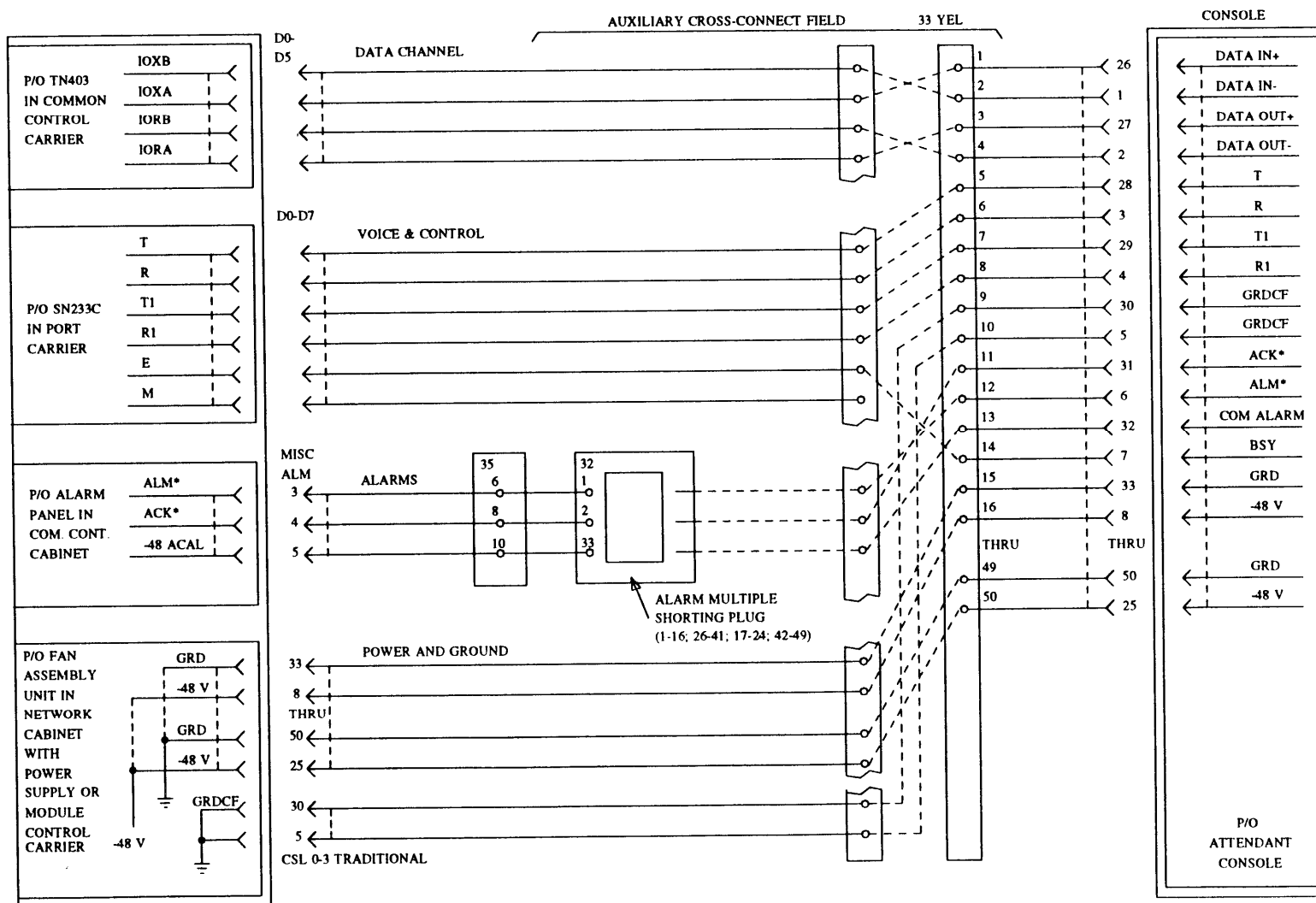
Figure 14-1. Console Connections
