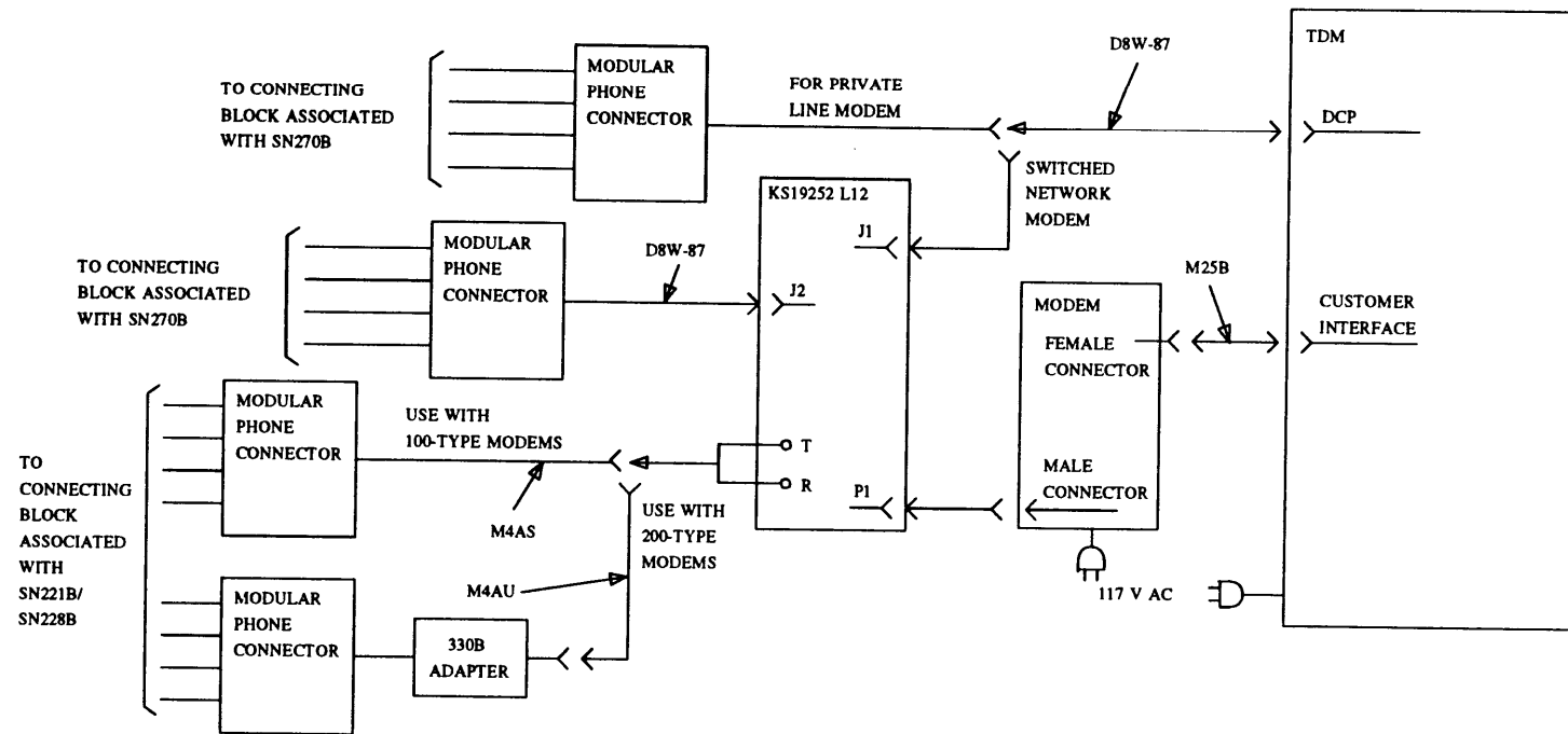
Figure 32-16. Connections
