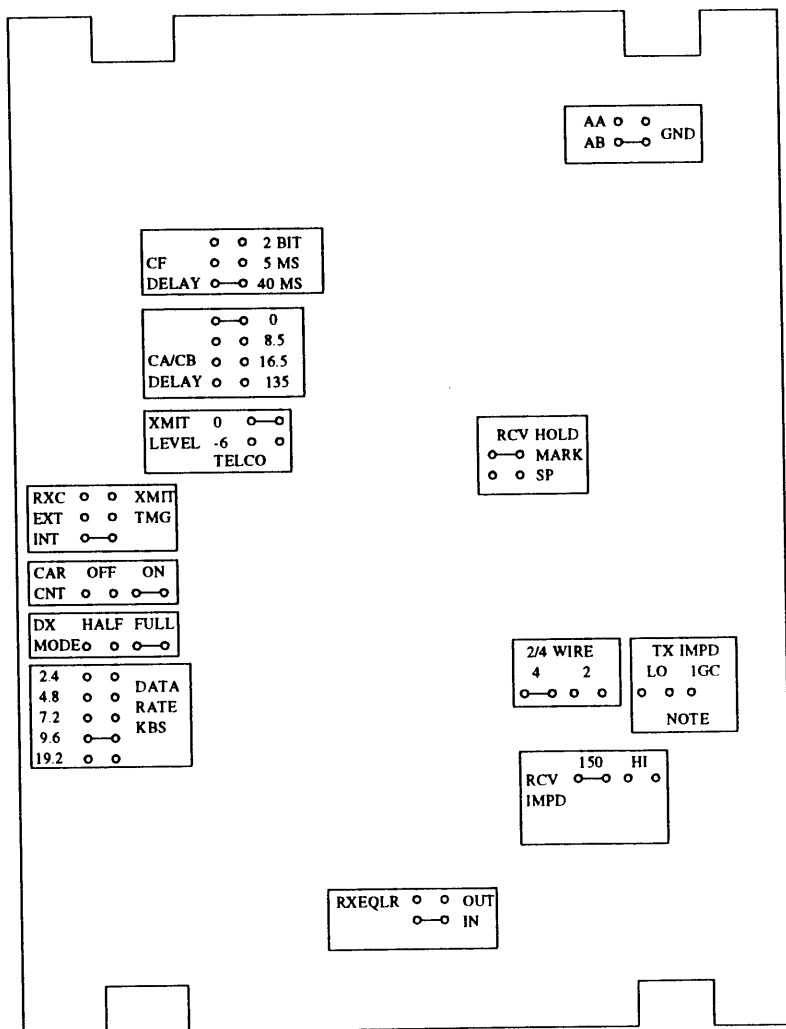
Figure 15-3. LDSU (48250) Options
