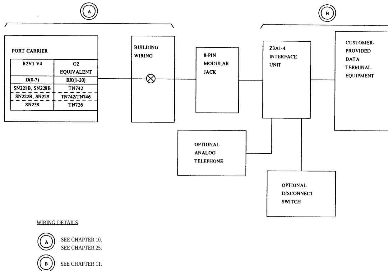
Figure 18-11. EIA Standard RS232C Interface to Customer-Provided Data Terminal Equipment
