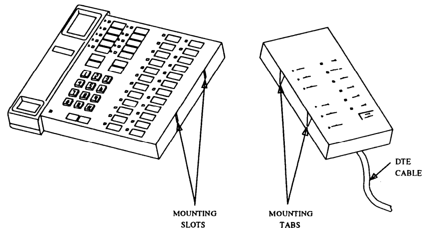
Figure 32-26. DTDM Attachment to Voice Terminal
