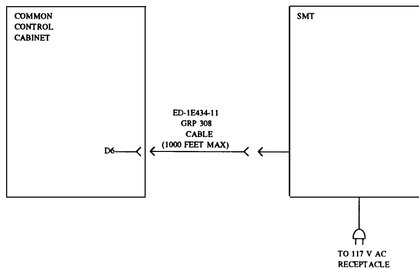
Figure 30-61. SMT Connections
