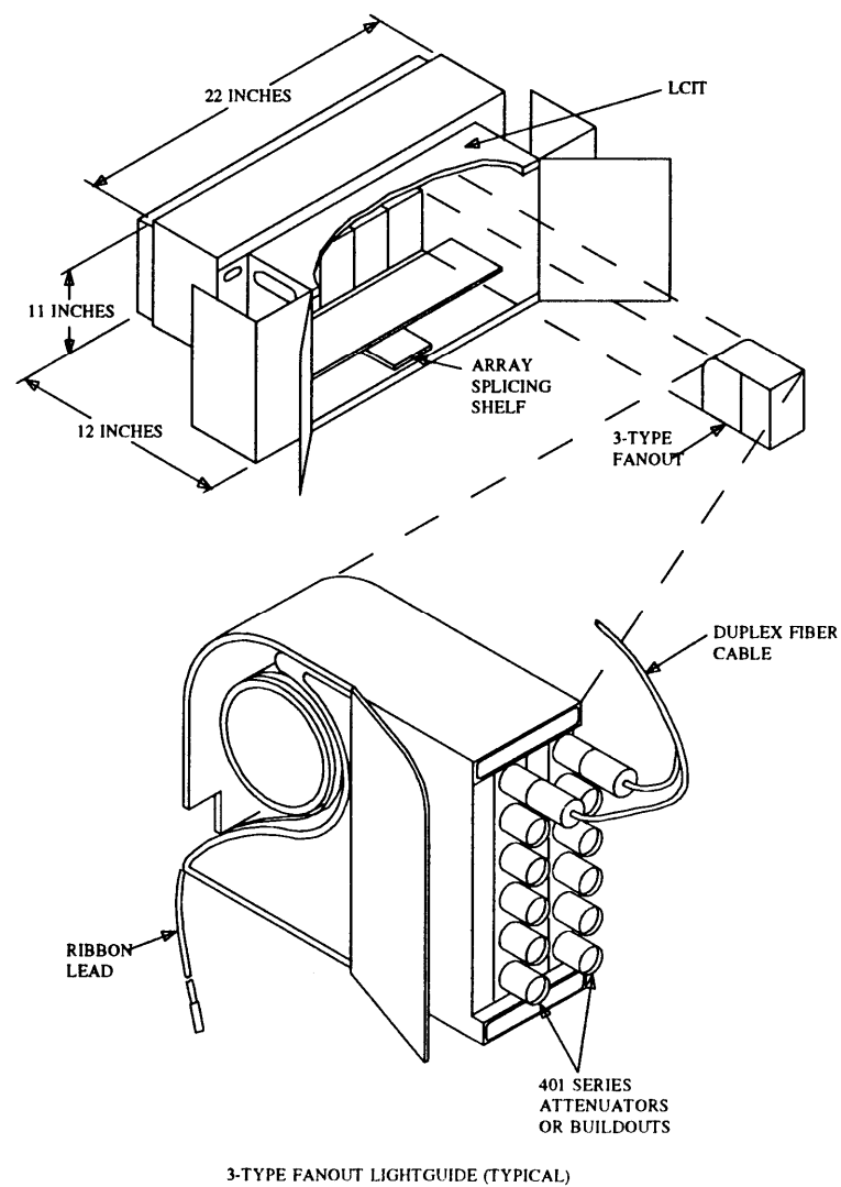
3-TYPE FANOUT LIGHTGUIDE (TYPICAL)
