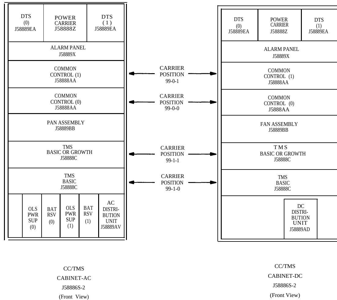
Figure 22-1. CC/TMS Cabinet — AC and DC
