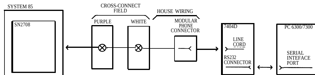
Figure 32-48. PC Switch/Connection Package I and II to System 85
