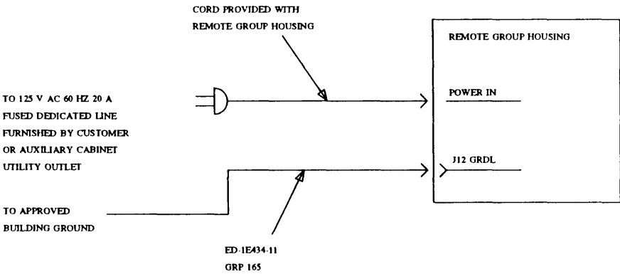
Figure 13-25. OLS with No Battery Reserve
