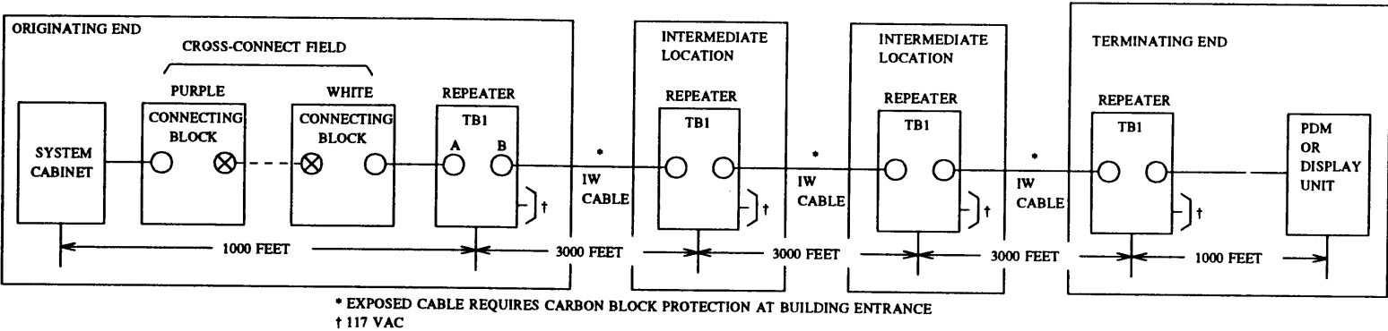
Figure 30-14. Requirements for Range Extension and Lightning Protection ( 11,000 Feet)
