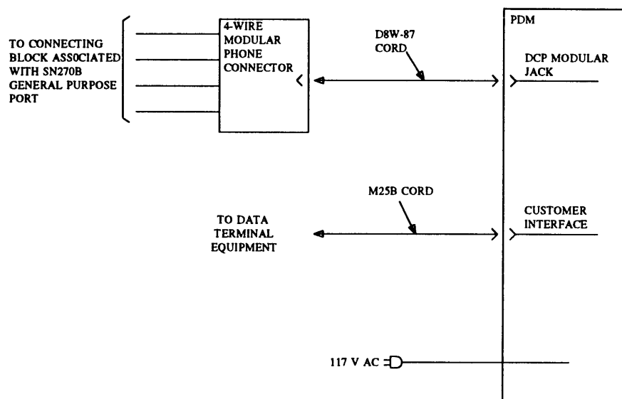
Figure 32-8. Stand-Alone Connections
