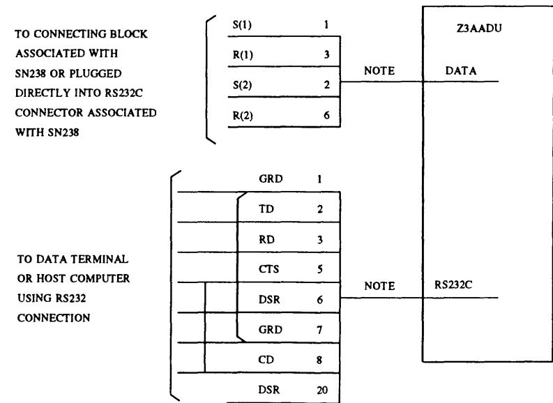
Figure 32-1. ADU Connections
