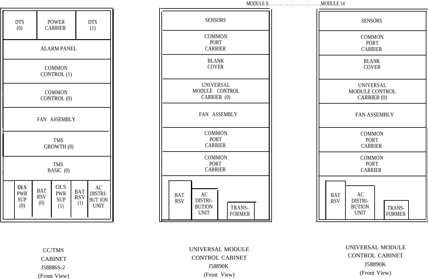
Figure 21-8. CC/TMS and UMC Cabinets - Duplicated CC and Unduplicated TMS, Multimodule
