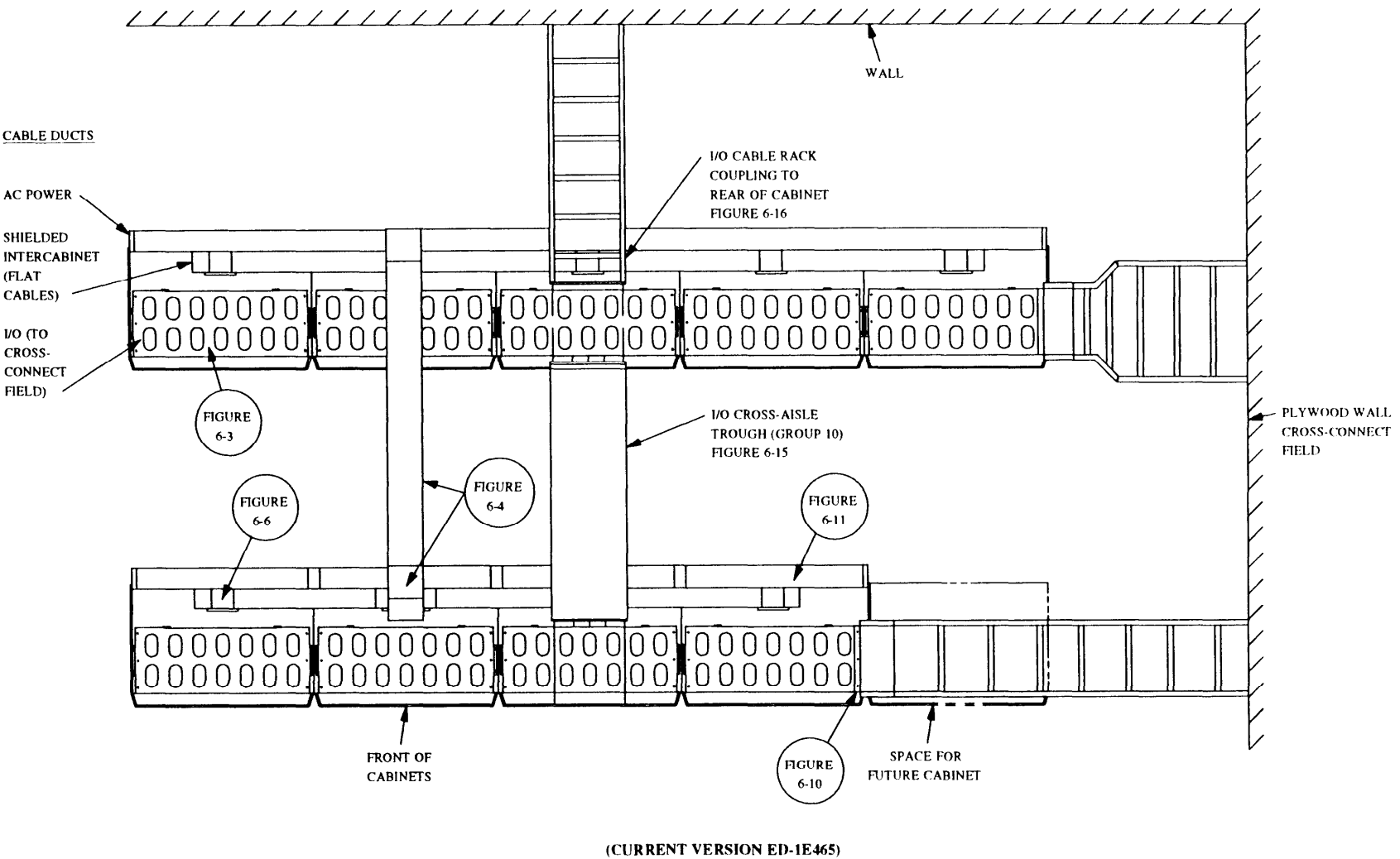
Figure 6-2. Overhead View of a Typical Ductwork Layout
