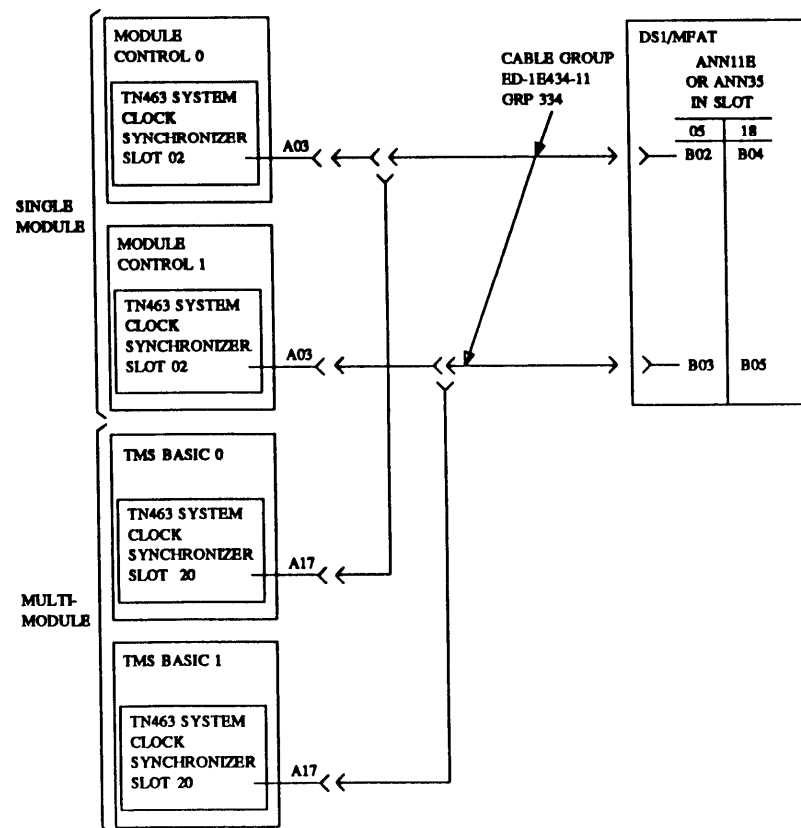
Figure 11-28. Synchronization Cabling — Primary Reference — Same Carrier
