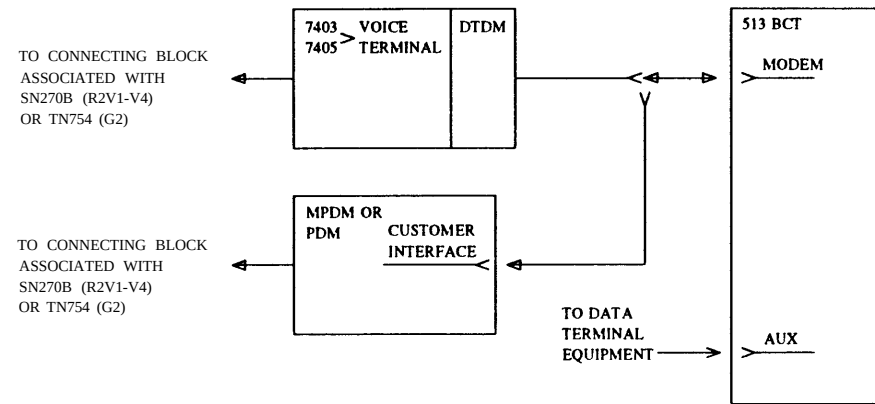
Figure 18-4. 513 BCT Terminal
