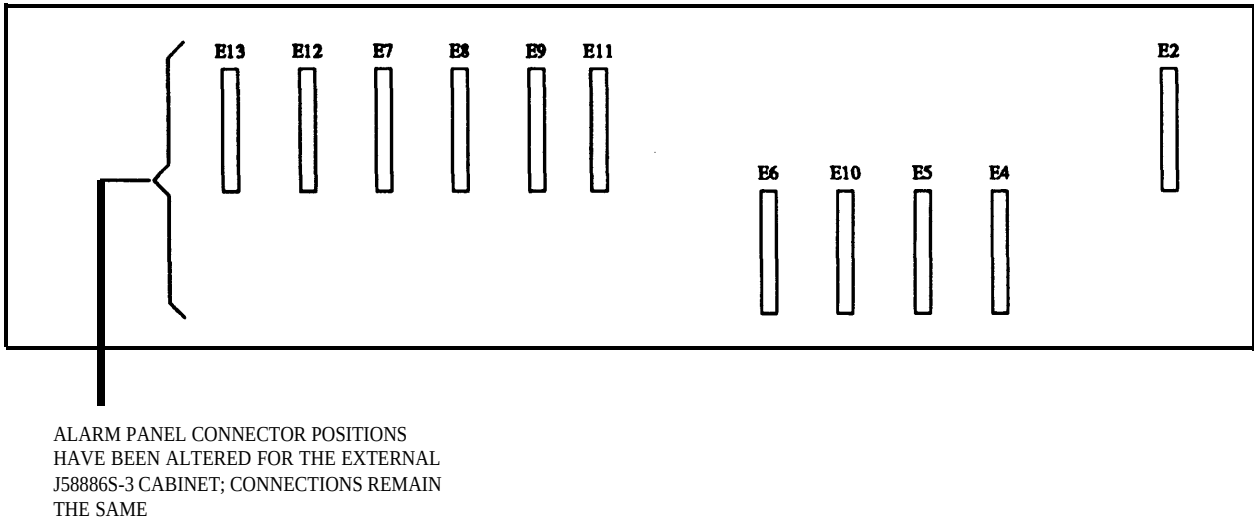
Figure 22-15. AC/DC Alarm Panel Connections (Rear View)
