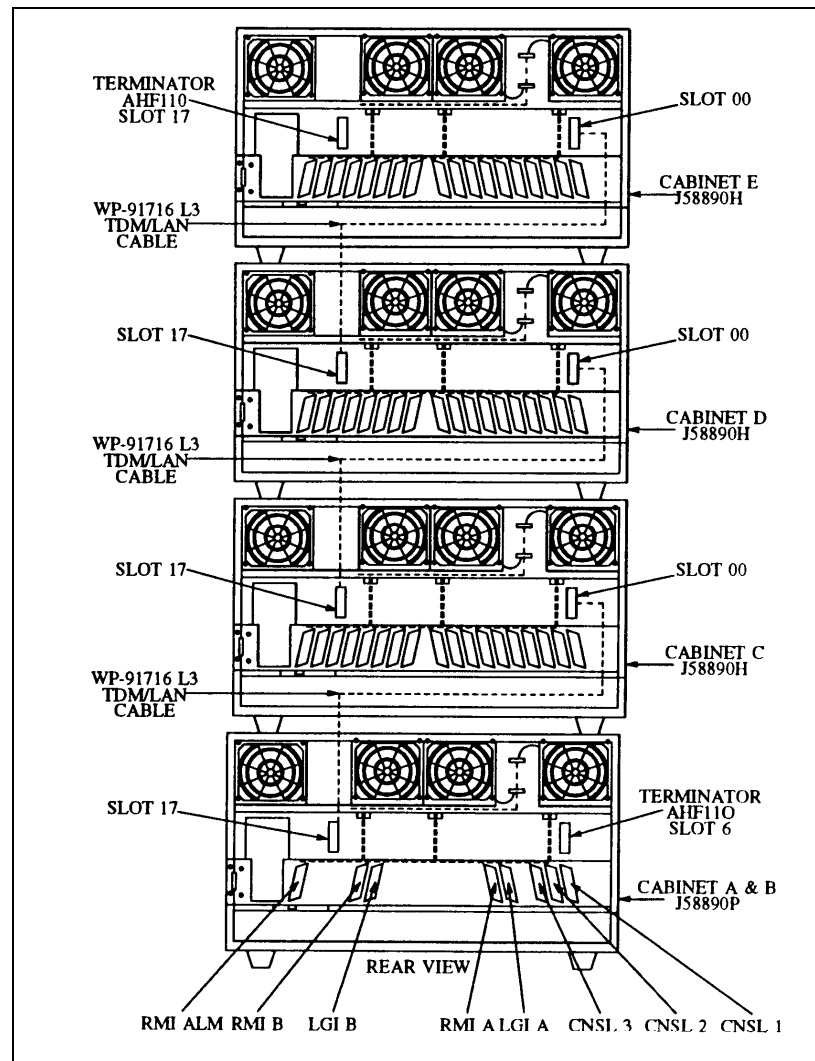
Figure 26-38. Single Carrier Cabinet Stack
