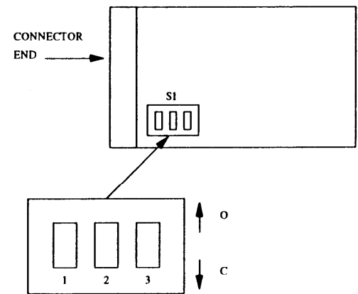
Figure 17-4. ANN15B and ANN16B S1 Switch
