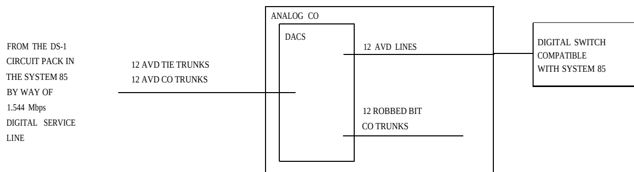
Figure 18-26. DS-1 Signaling System 85 Applications (Part 3 of 3)
