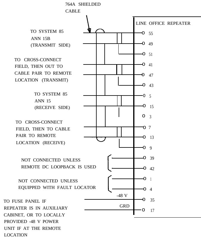
Figure 13-37. LOR Connections
