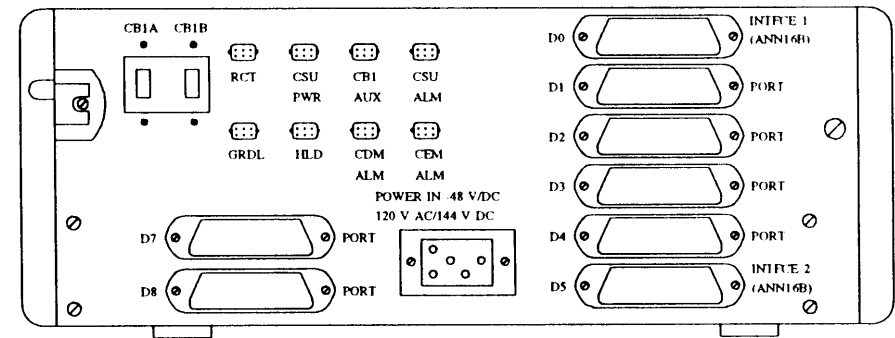
Figure 13-2. RGH (J58889AN-1)
