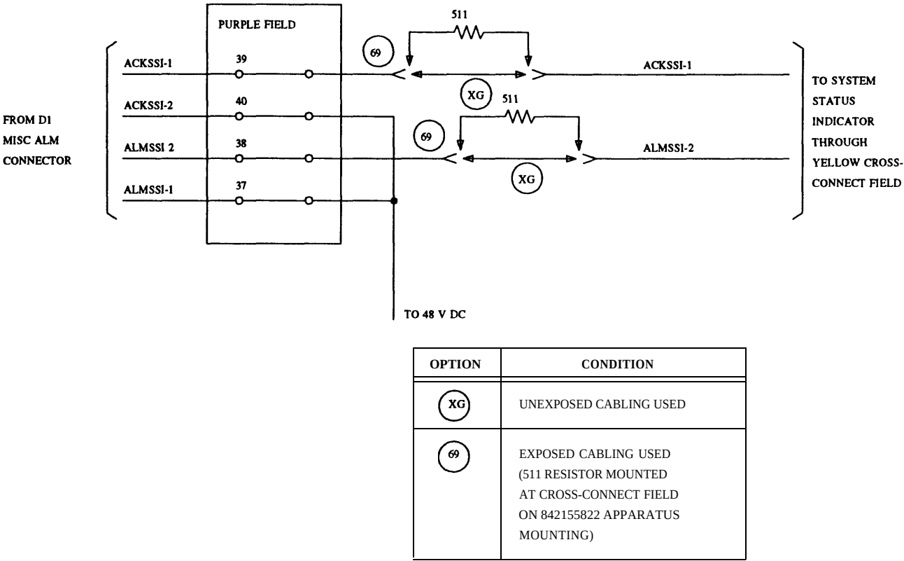
Figure 30-71. System Status Indicator Only
