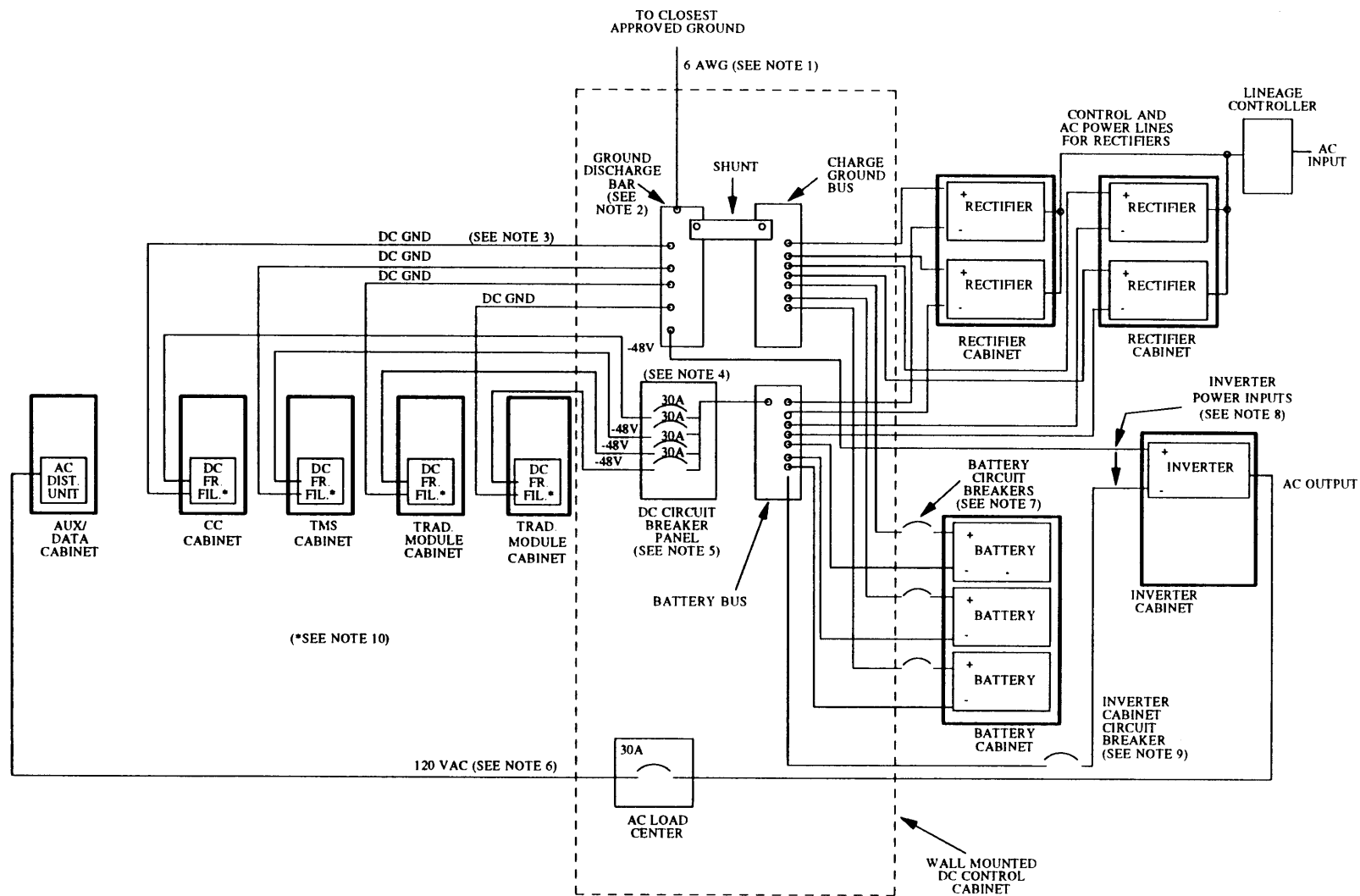
Figure 9-1. Typical Battery Plant for DC Systems
