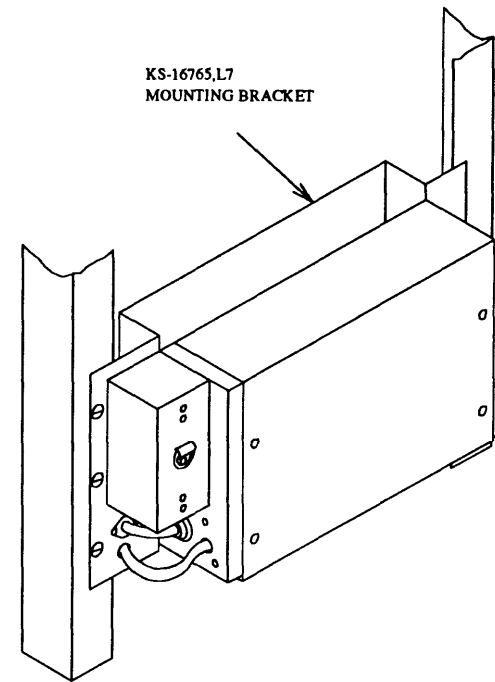
Figure 30-36. Recorded Announcement Unit KS-1 6765 Mounting Arrangement
