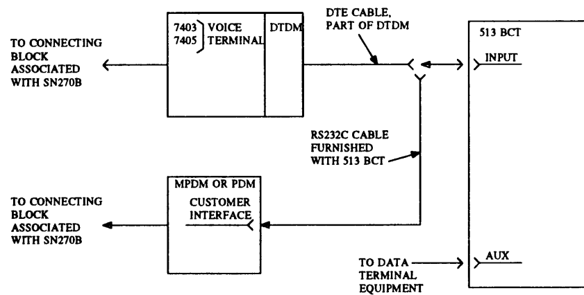
Figure 32-2. 513 BCT Connections
