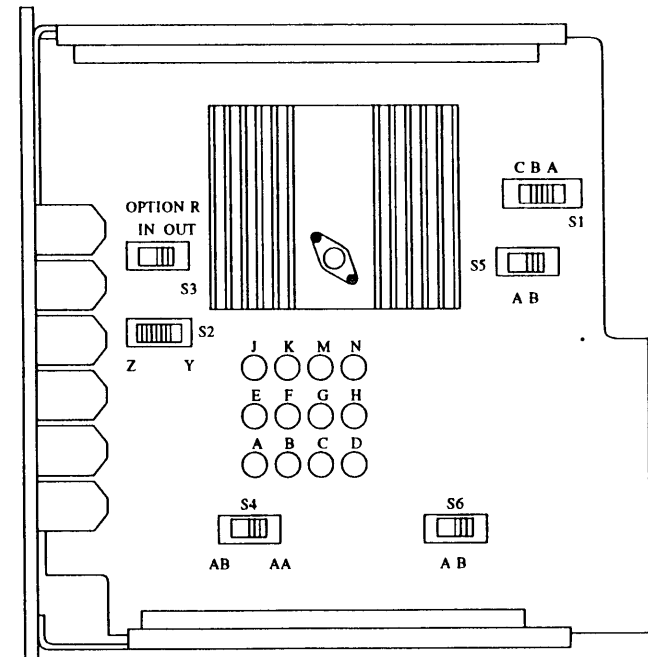
Figure 13-13. OR Board
