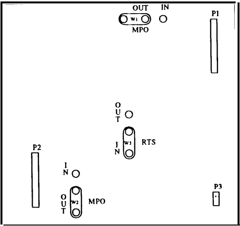
Figure 13-20. RS422 Switch Locations
