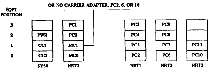
Figure 11-19. Carrier Configuration
