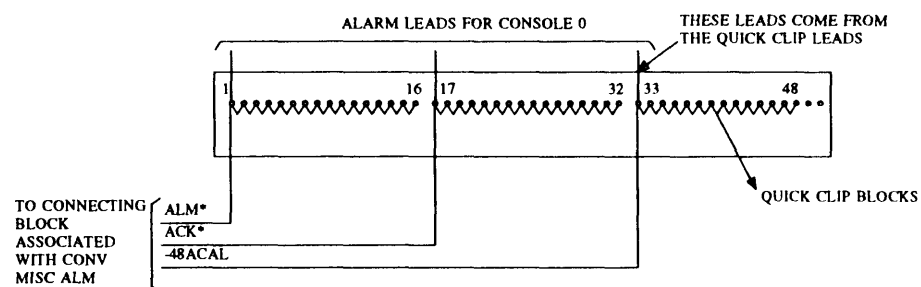
Figure 14-6. Quick-Clip Block Alarm Connections
