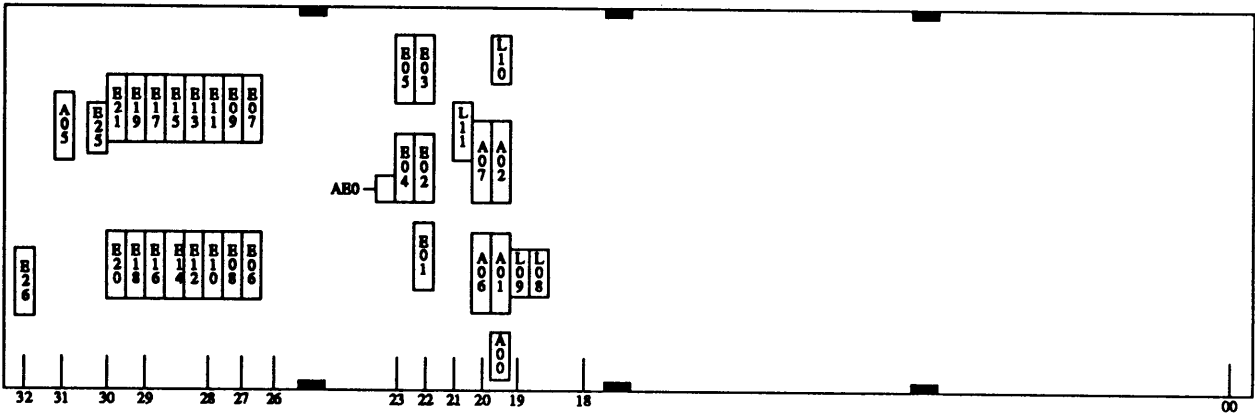
Figure 22-6. J58888E CC Carrier Connector Locations (Backplane)
