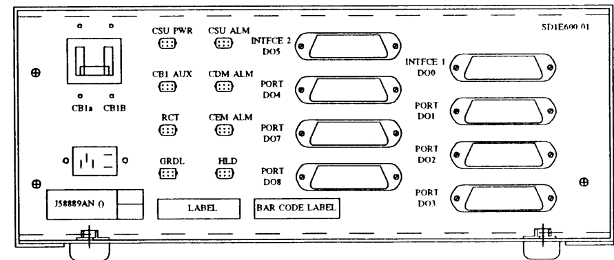
Figure 13-3. RGH (J58889AN-2)
