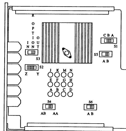
Figure 31-2. Office Repeater
