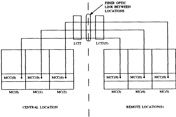
Figure 12-9. Assigned MC Carriers for Unduplicated System (Phase 1)
