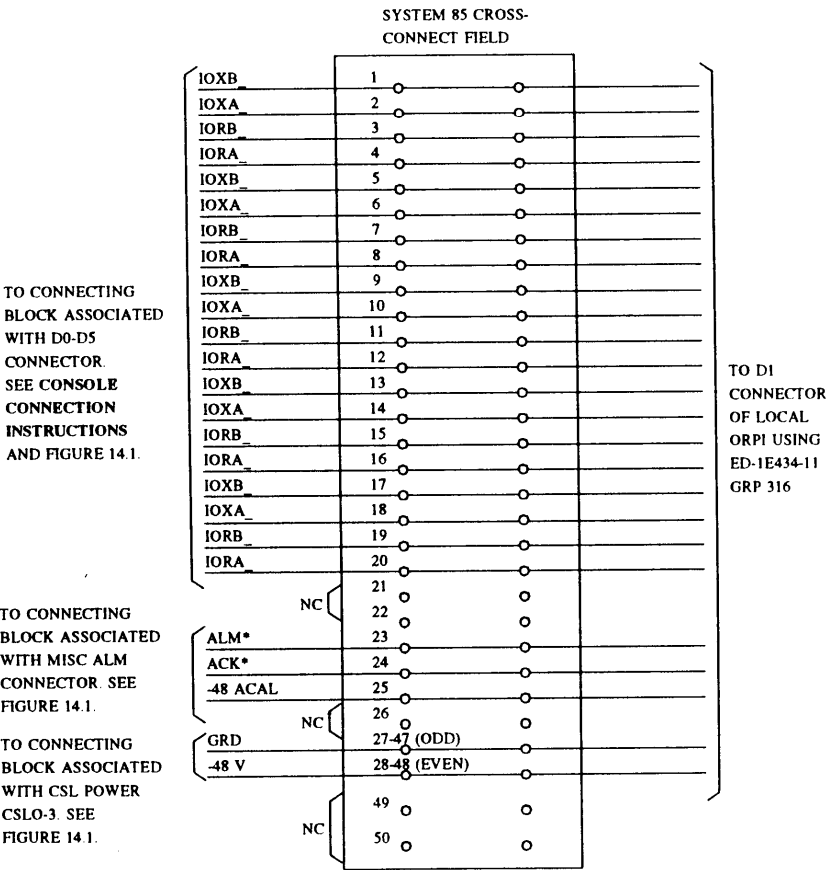
Figure 14-17. System 85 to ORPI Connections
