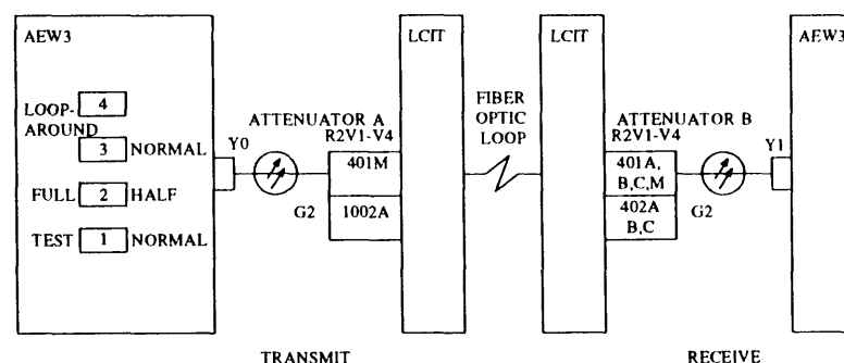
Figure 14-24. Attenuator Locations
