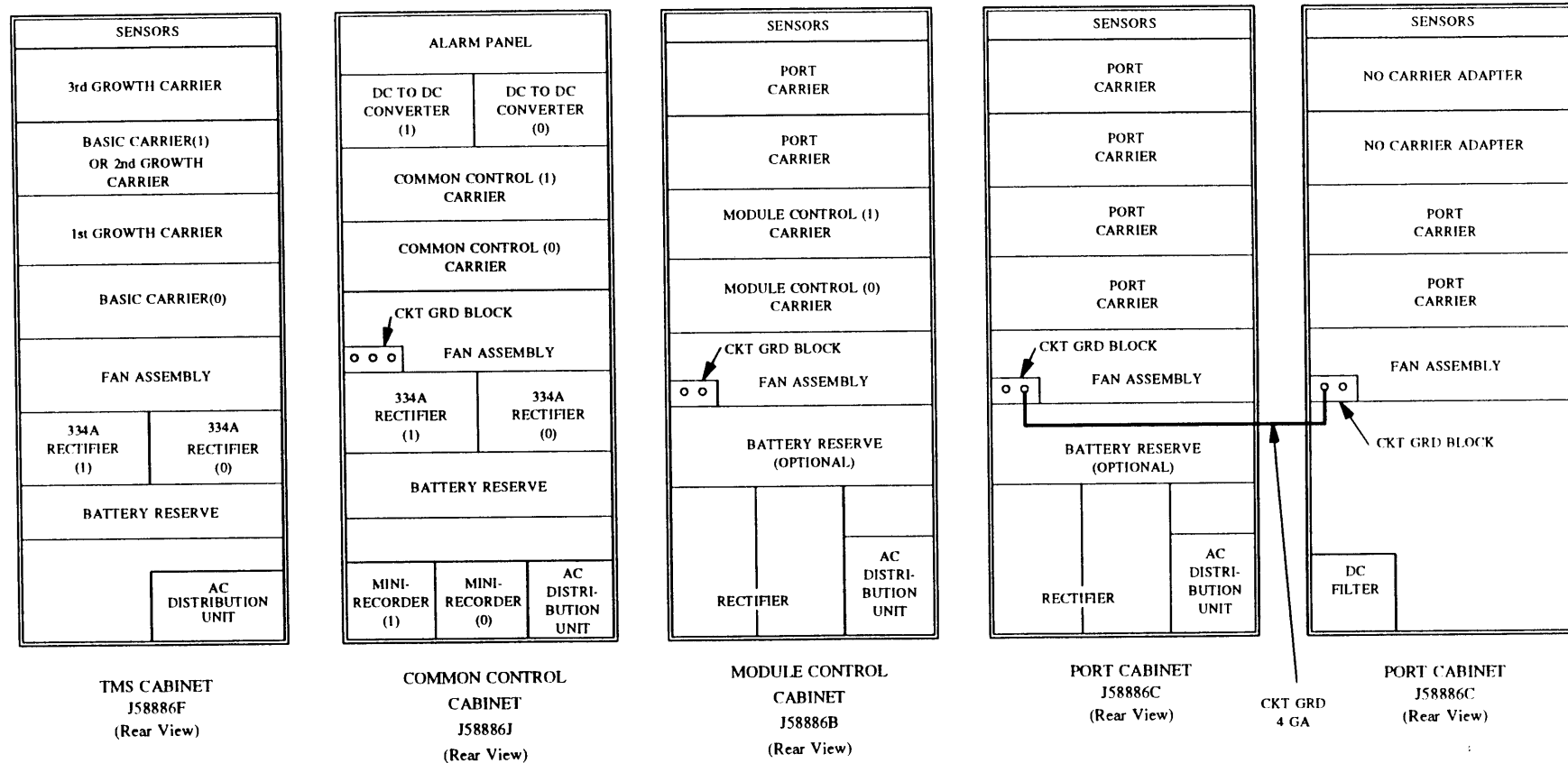
Figure 8-8. CT GRD for Cabinet Pairs — Duplicated System
