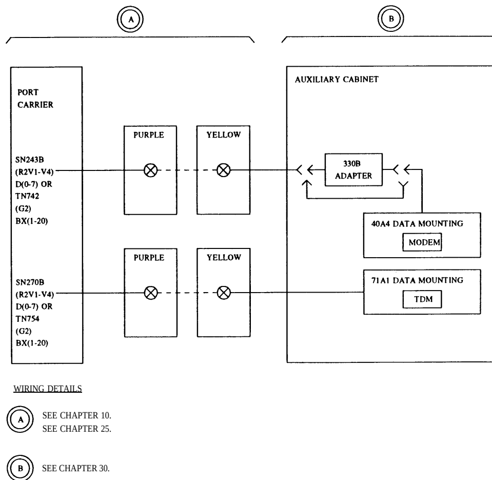
Figure 18-21. Modem Pooling
