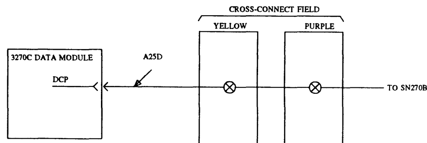
Figure 32-36. Connections to the System 85 (3270C Data Module)
