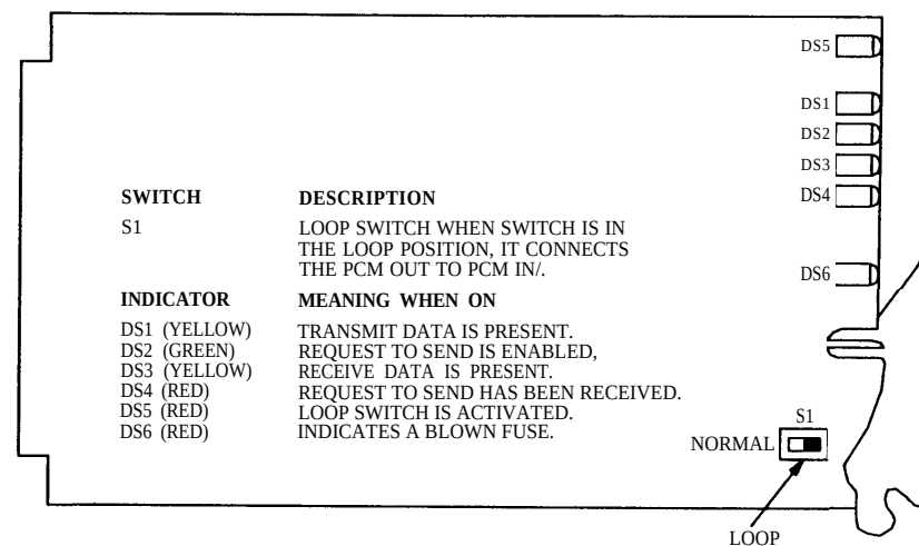
Figure 31-6. Switch Locations and Settings for 0 to 19.2 Kbps Asynchronous Data Channel Unit
