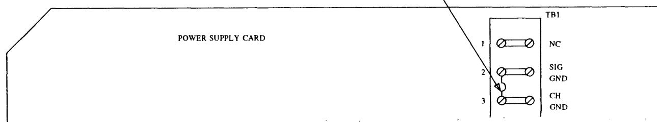
Figure 15-2. LADs (48230) — Options
