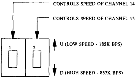
Figure 28-34. TN403 Switch
