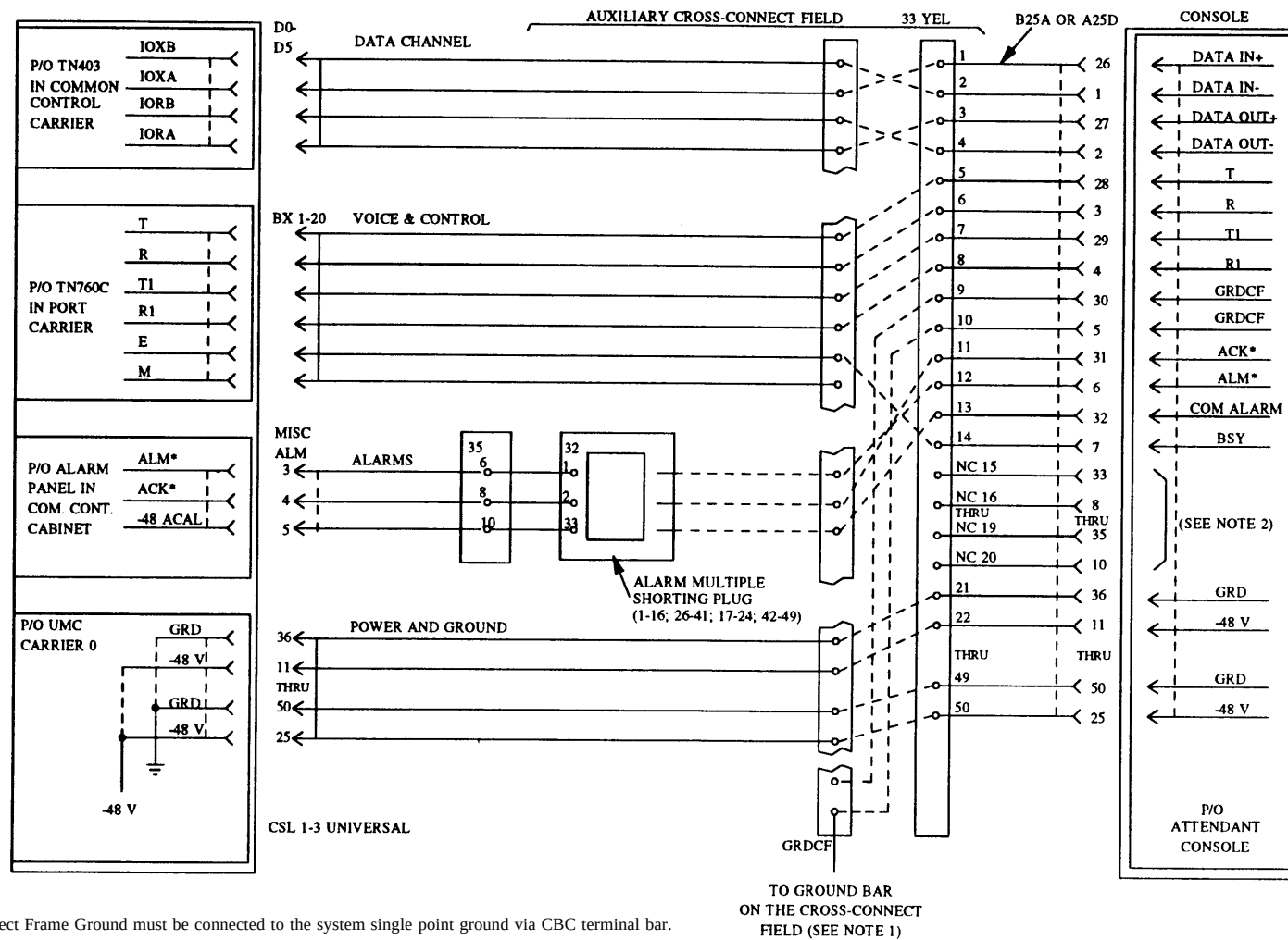
Figure 27-1. Console Connections
