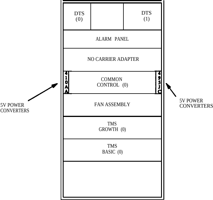
Figure 22-13. Unduplicated CC/TMS Cabinet with DC Power (Front View)
