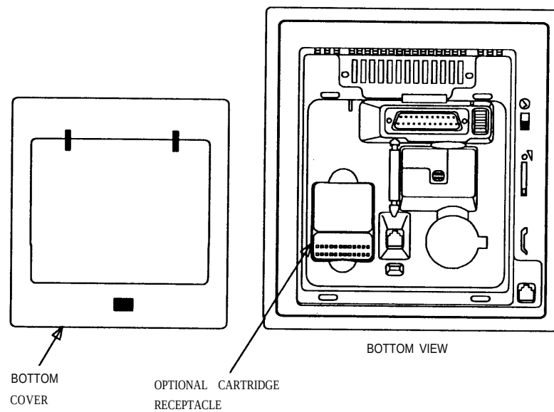
Figure 32-47. 7404D Cartridge Receptacle
