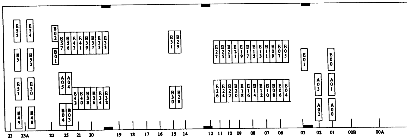
Figure 11-8. J58888M Traditional Module Control Carrier Connector Locations (Backplane)
