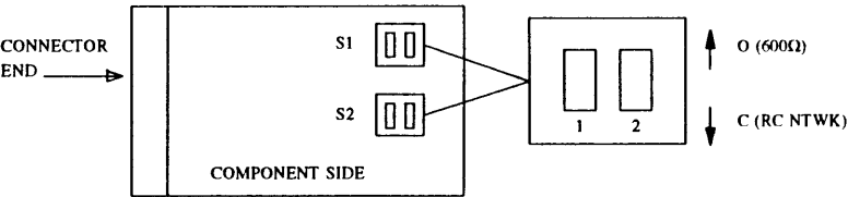
Figure 17-26. SN243 Switch and Location
