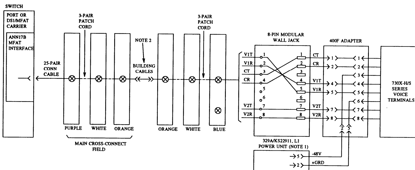
Figure 30-64. Typical Hybrid Electronic Voice Terminal (730X-H/S Series)
