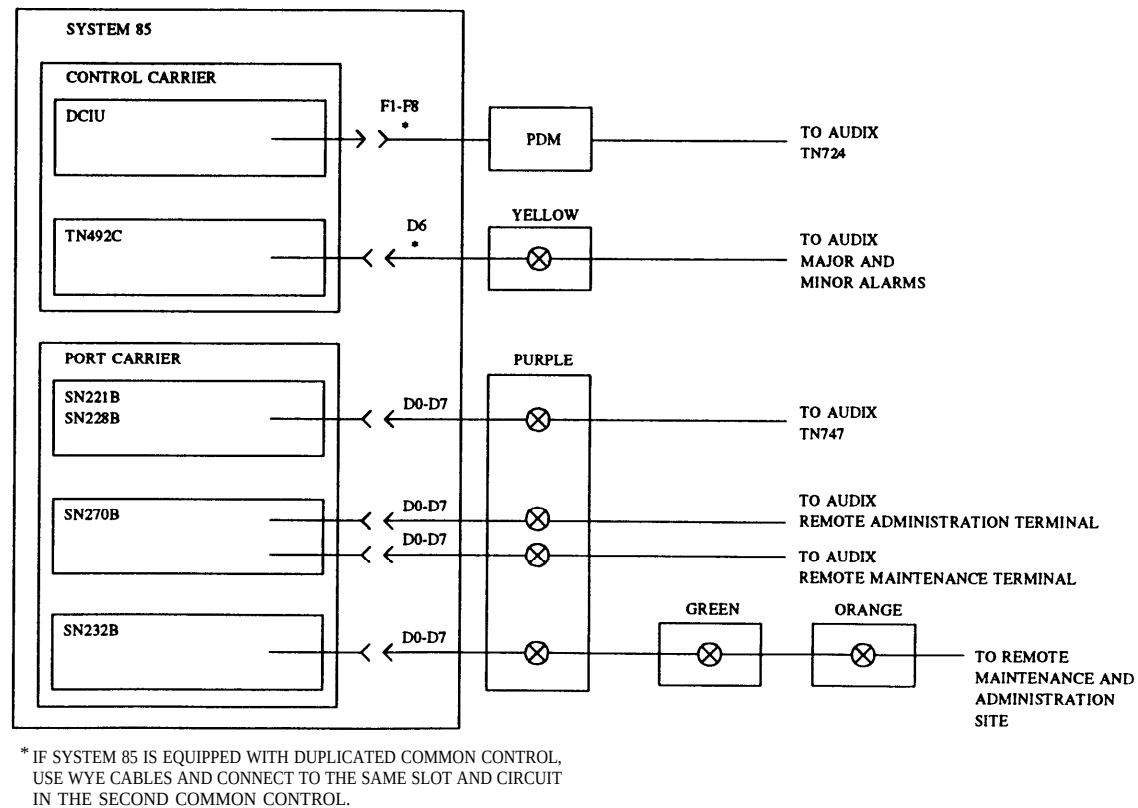
Figure 30-9. AUDIX Connections
