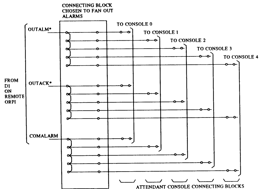
Figure 14-21. Fanning Out Alarm Leads
