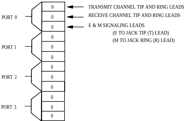
Figure 17-16. SN233B Jack Assignments
