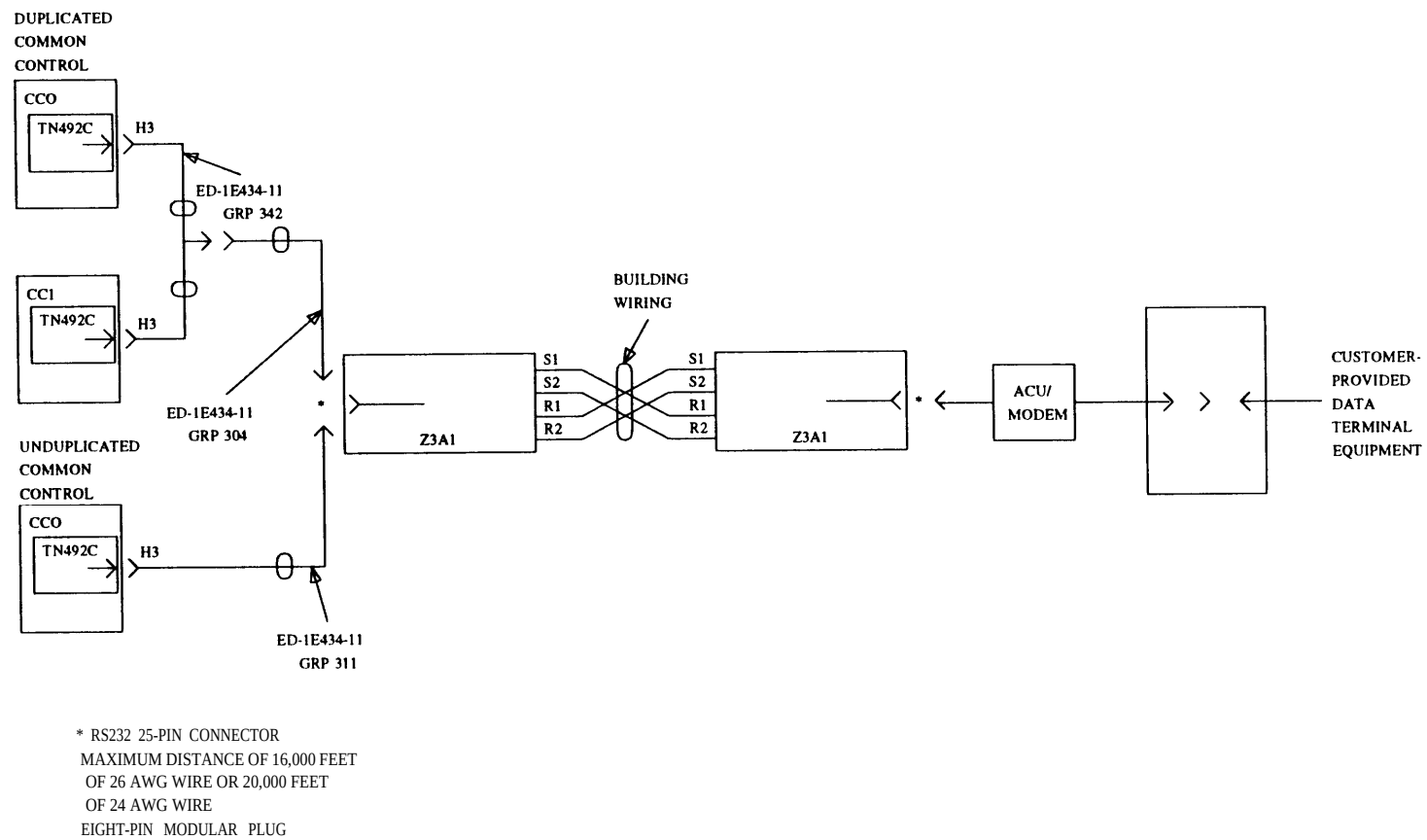
Figure 15-9. Customer-Provided Data Terminal Equipment to System Connections Through Z3A1 ADUs
