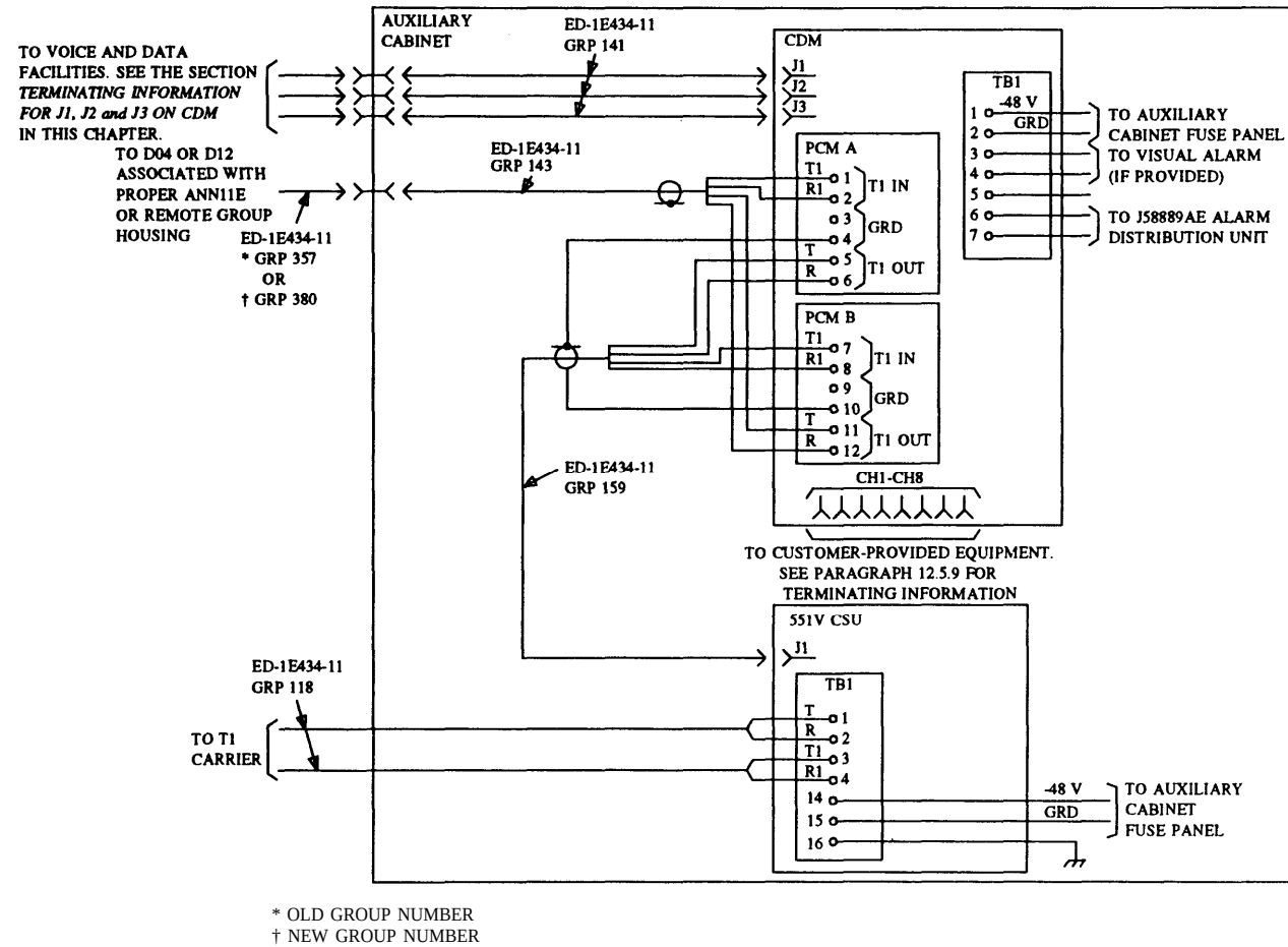
Figure 31-20. Equipment Located in an Auxiliary Equipment
