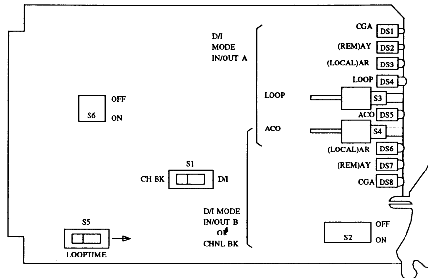
Figure 31-4. Alarm Unit (30005-001) Switch Diagram
