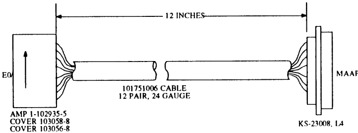
Figure 12-26. ED-1E434, Group 132 Cable
