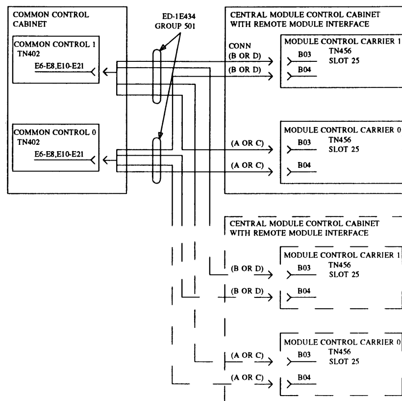
Figure 26-32. ED-1E434, Group 501 Connections for an All Duplicated System (Phase 1)
