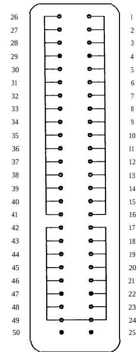
Figure 14-4. ED-1E434-11 Group 360 Multiple Alarm Shorting Plug
