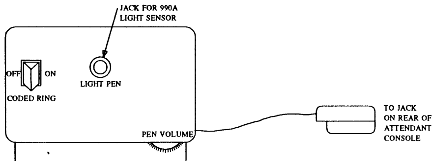
Figure 14-14. 2A Translator
