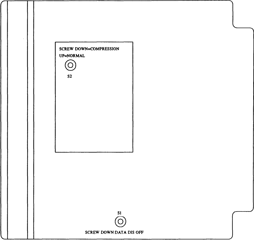
Figure 31-23. LORAIN Voice Gain Amplifier Switch Diagram
