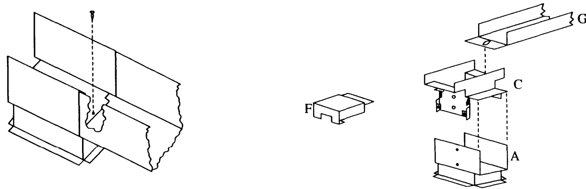
Figure 6-5. Mating Cross-Aisle Risers to Older R2 Cabinet Risers
