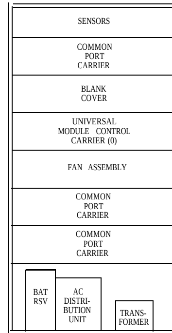
UNIVERSAL MODULE CONTROL CABINET J58890K (Front View)
