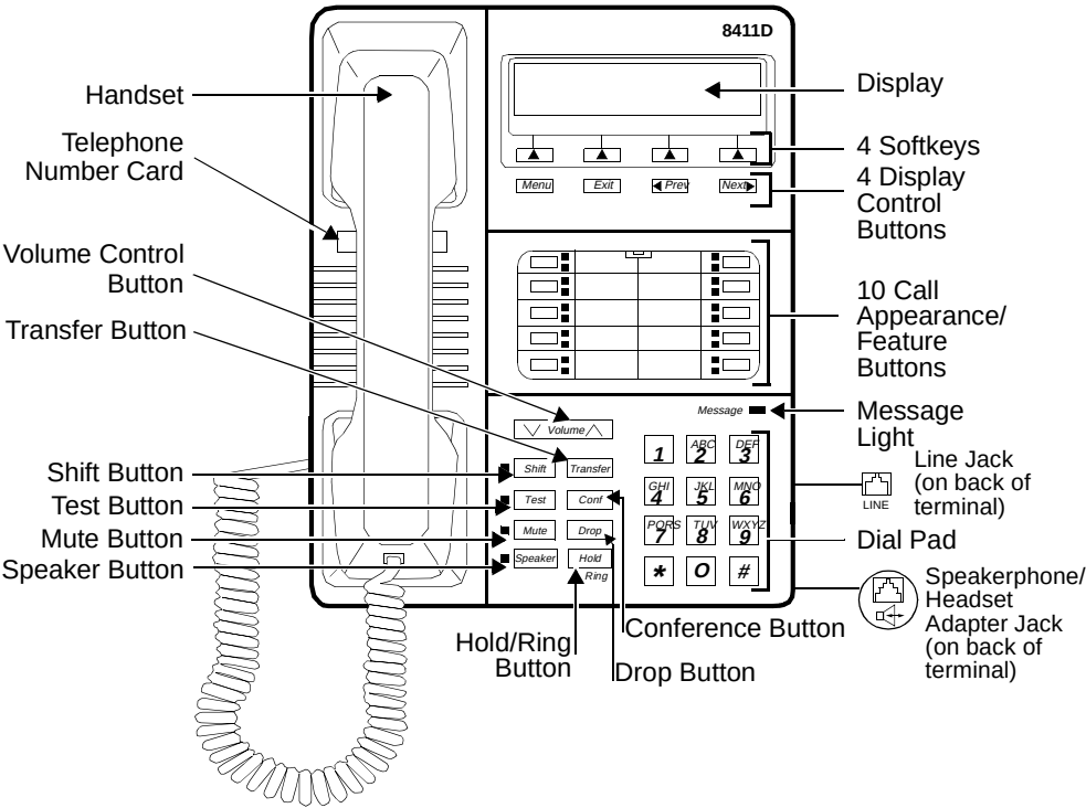
Figure 12-15. The 8411D Voice Terminal (With Display)
