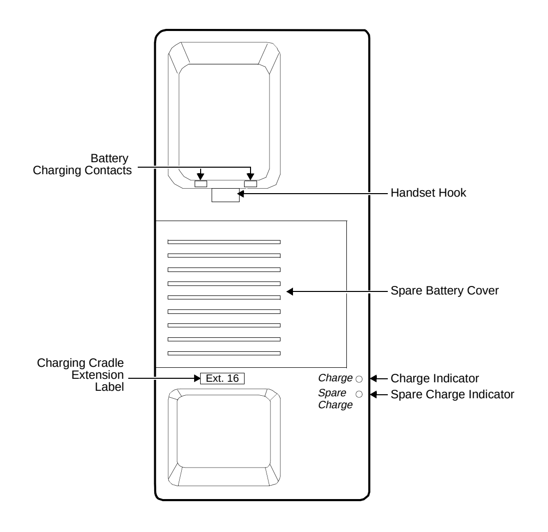
Figure 18-6. The MDW 9000 Telephone, Top View of Charging Cradle
