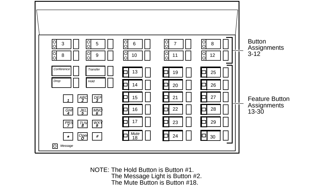
Figure 13-6. Button Numbering for Administering the 602 CALLMASTER Voice Terminal Connected to a System 85 or a DEFINITY G2
