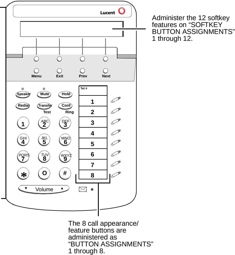
Figure 7-6. Button Numbering for Administering the 6408 Telephones Connected to a DEFINITY System Release 6.1 or Later
