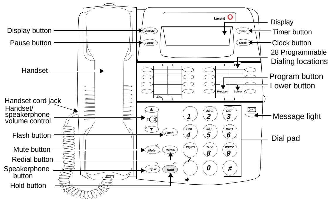
Figure 15-3. The 6230 Telephone
