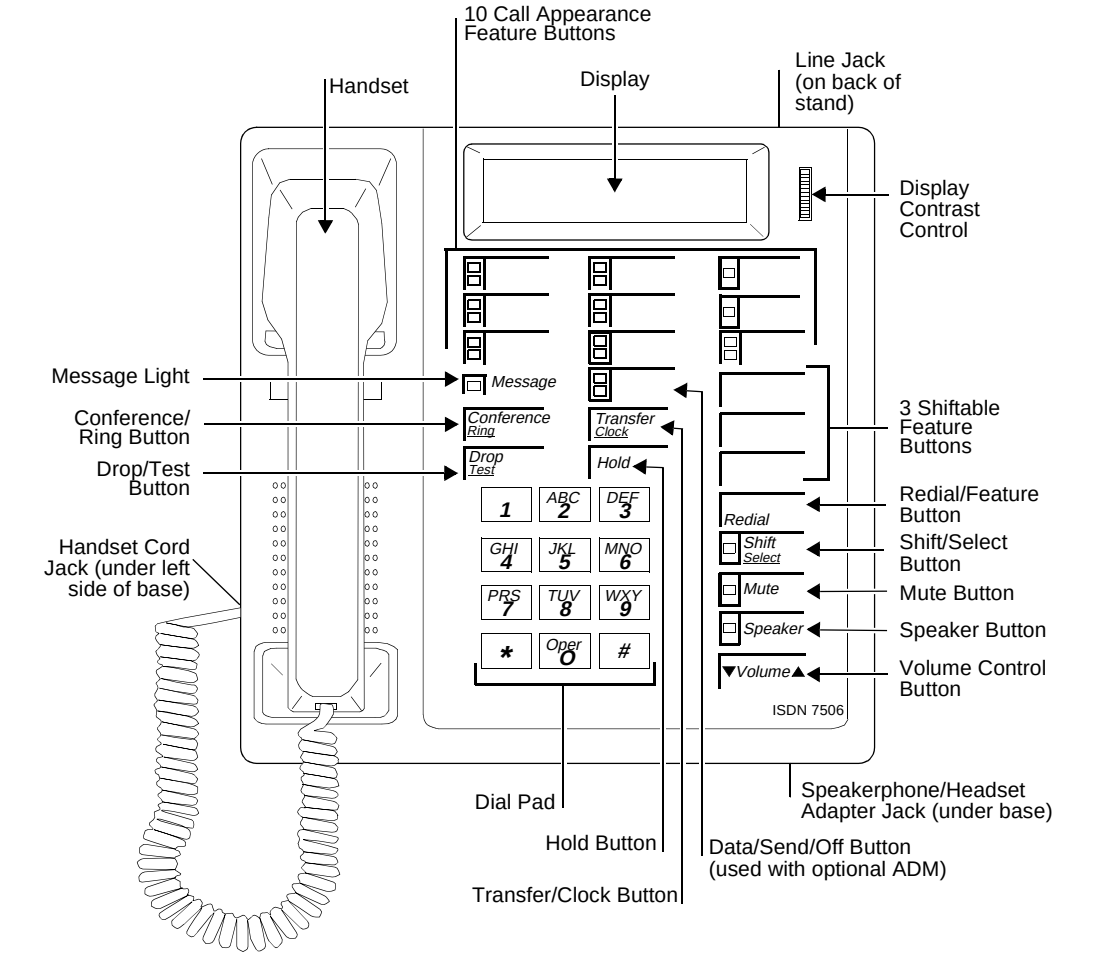
Figure 17-2. The 7506 Asynchronous Data Modular Display Terminal
