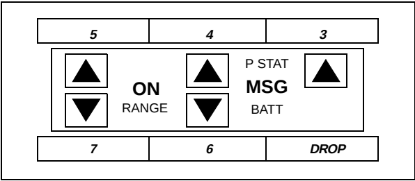
Figure 18-4. Button Numbering for a MDC 9000 Connected to System 85 or a DEFINITY Generic 2
