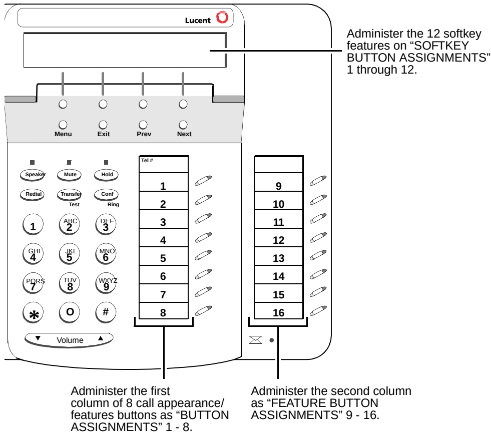
Figure 7-8. Button Numbering for Administering the 6416D+ or 6416D+M Telephone Connected to a DEFINITY System Release 6.1 or Later
