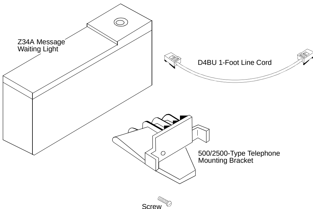
Figure 20-9. The Z34A Message Waiting Indicator
