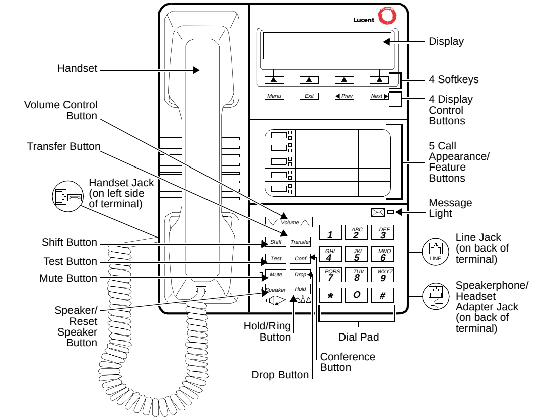
Figure 12-7. One Version of the 8405D and 8405D Plus Voice Terminal (With Display)
