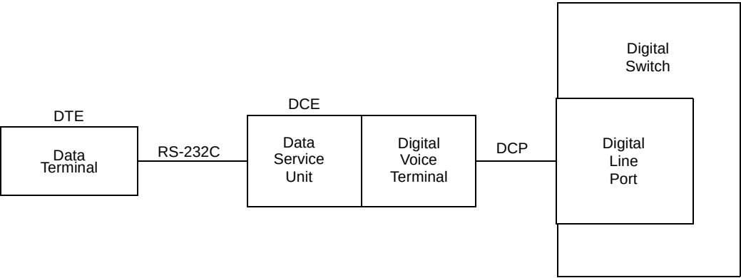
Figure 21-15. A Block Diagram of 703A Data Service Unit Interfaces
