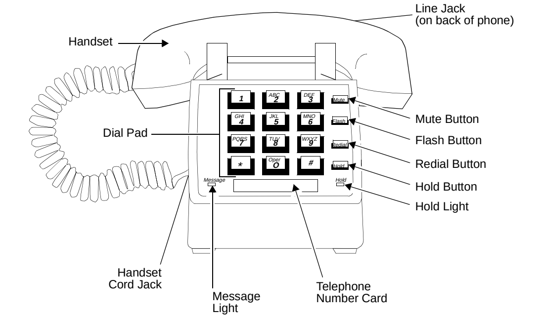
Figure 14-8. The 2500 YMGL and 2500 YMGM Telephones
