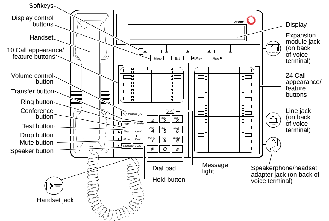
Figure 12-22. Another Version of the 8434DX Voice Terminal
