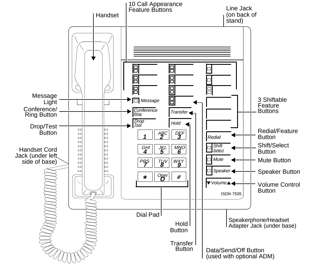
Figure 17-1. The 7505 Asynchronous Data Modular Terminal
