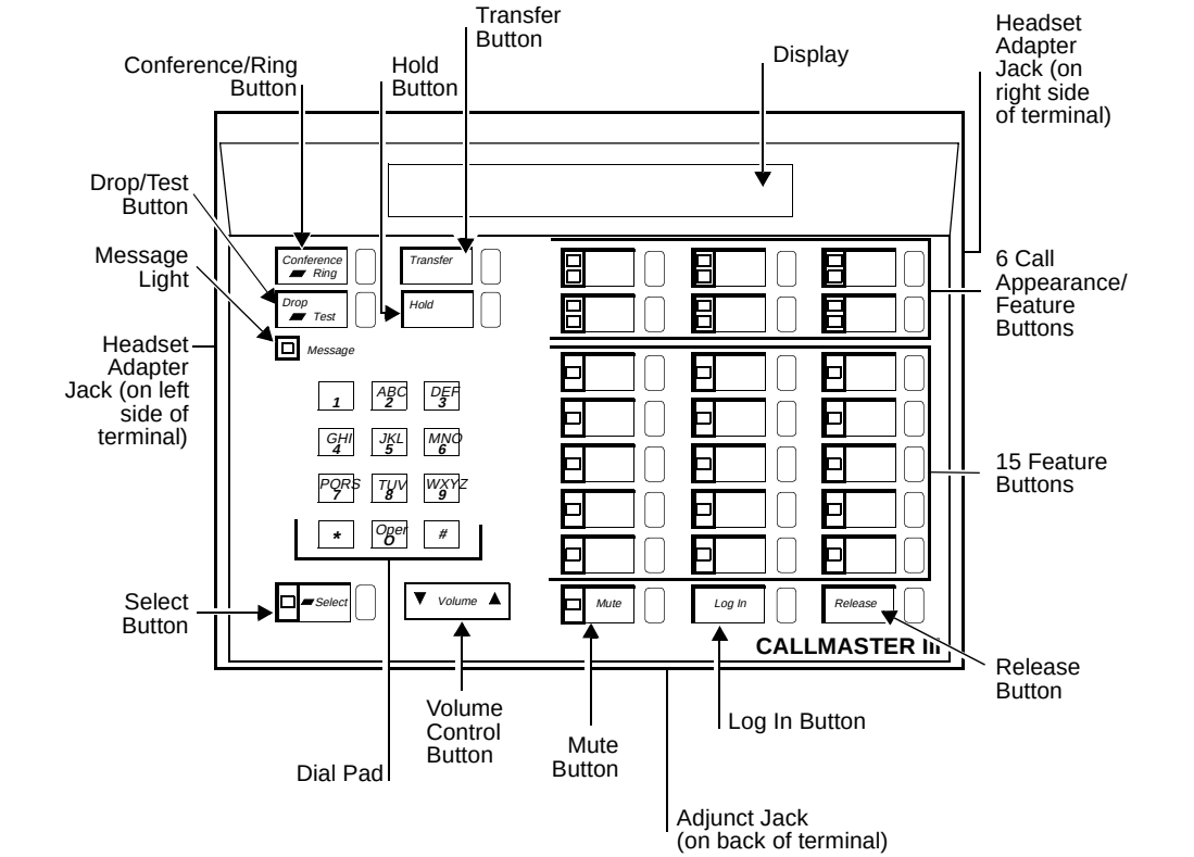
Figure 13-2. The CALLMASTER II and CALLMASTER III Voice Terminal
