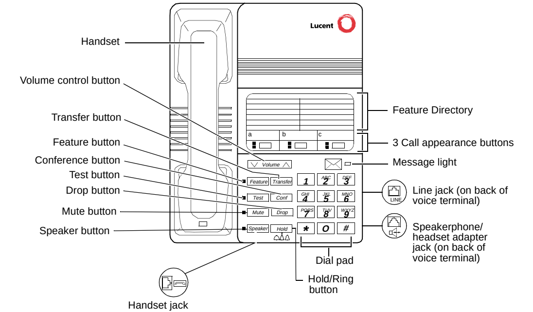
Figure 12-2. Another Version of the 8403 Voice Terminal
