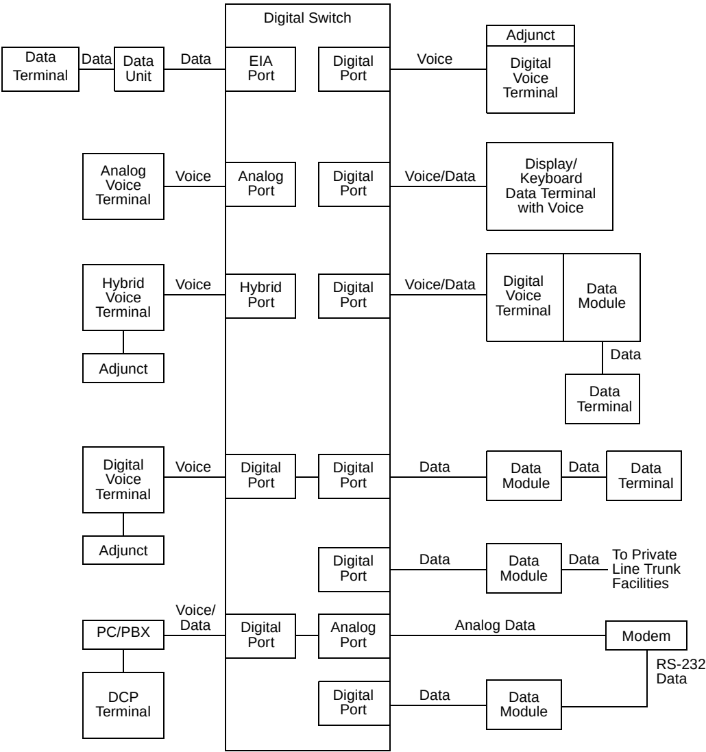
Figure 1-1. Interface Between System Switch and Typical Terminals/Adjuncts
