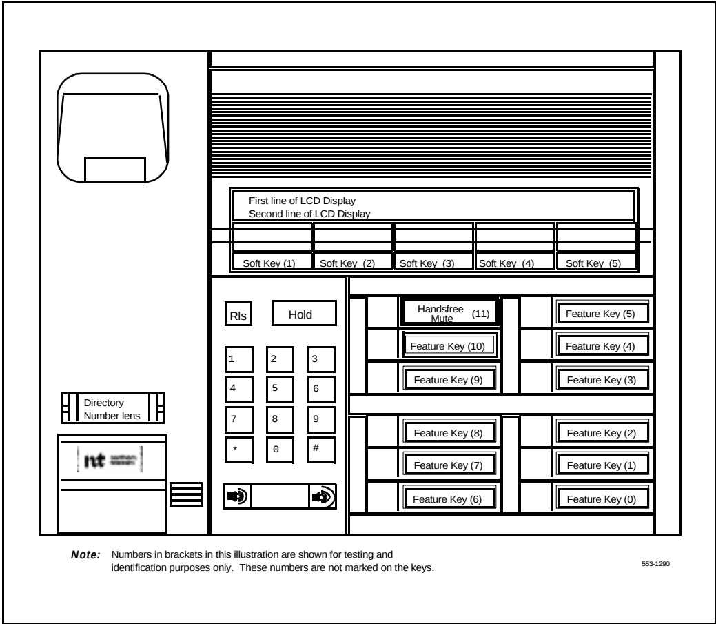
Figure 19 M2317 Telephone — key identification
