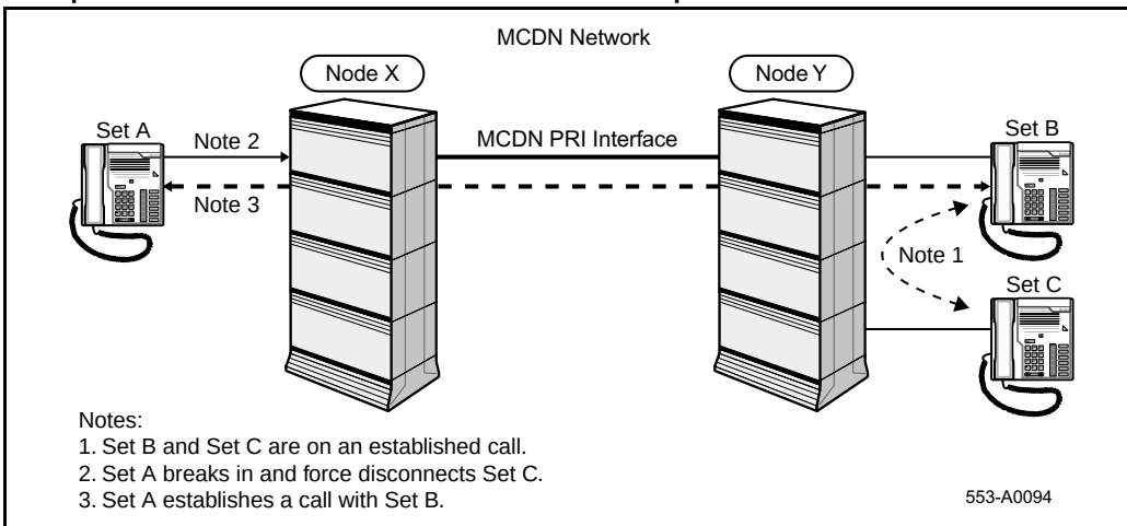
Figure 129 Example of a network break-in and force disconnect operation
