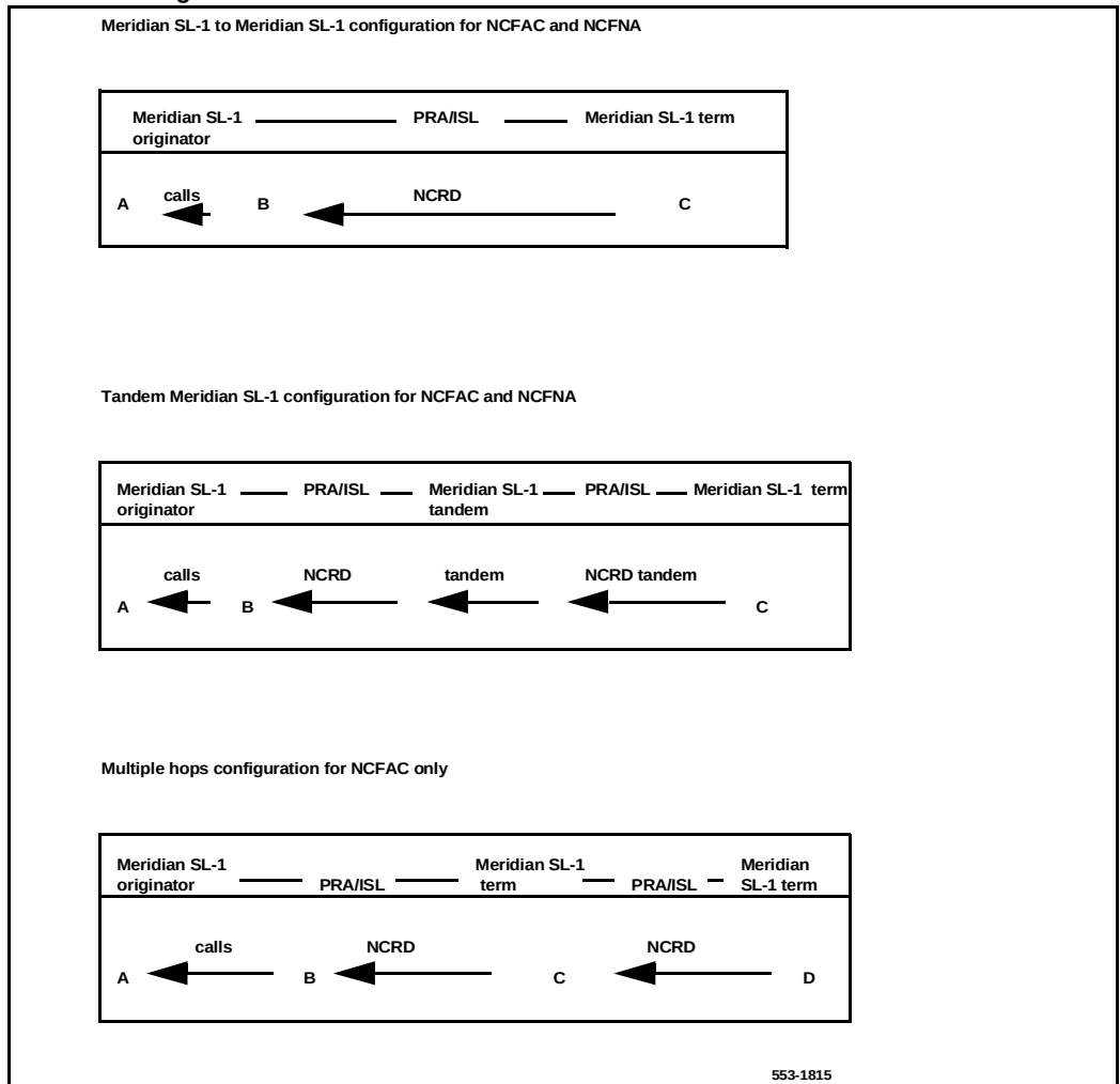
Figure 110 Network configurations for NCFAC and NCFNA
