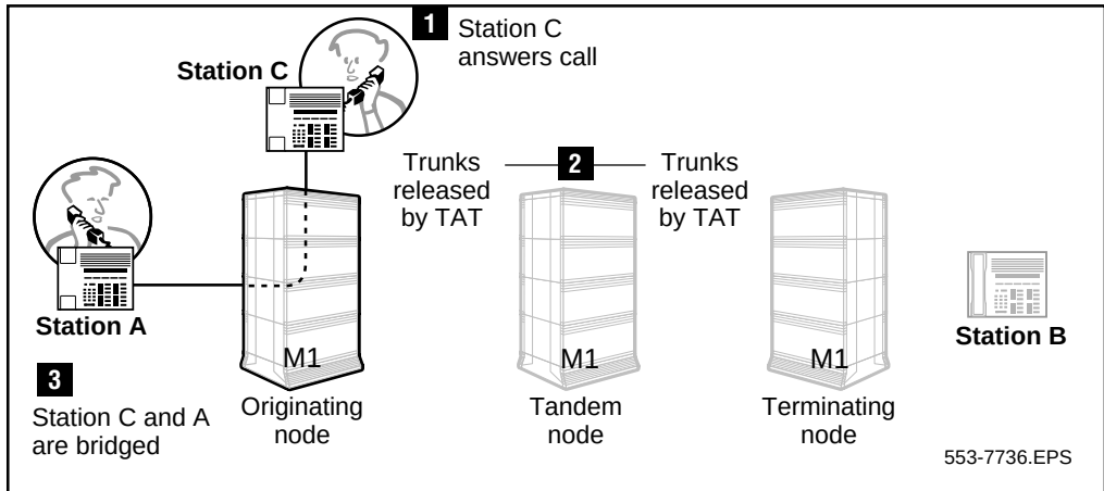
Figure 157 Results of anti-tromboning for network call transfer, M1/M1
