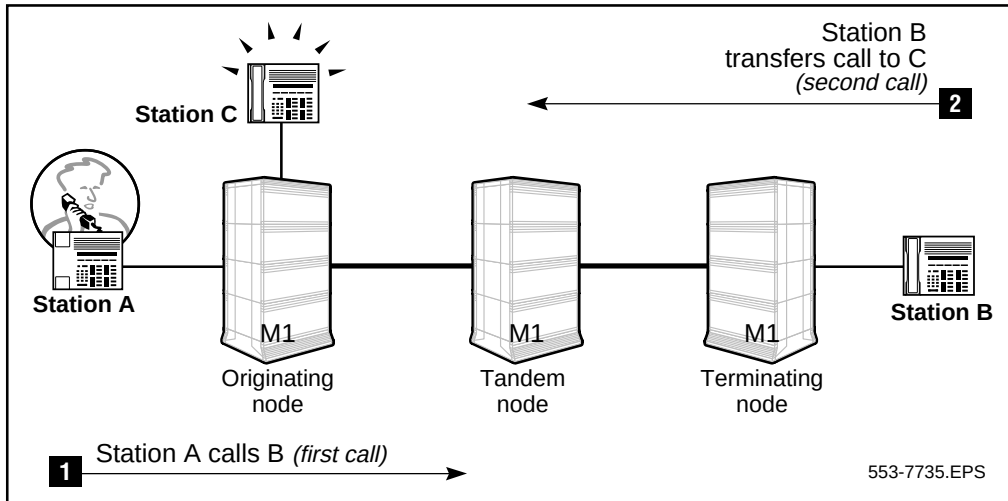
Figure 156 Anti-tromboning for network call transfer, M1/M1
