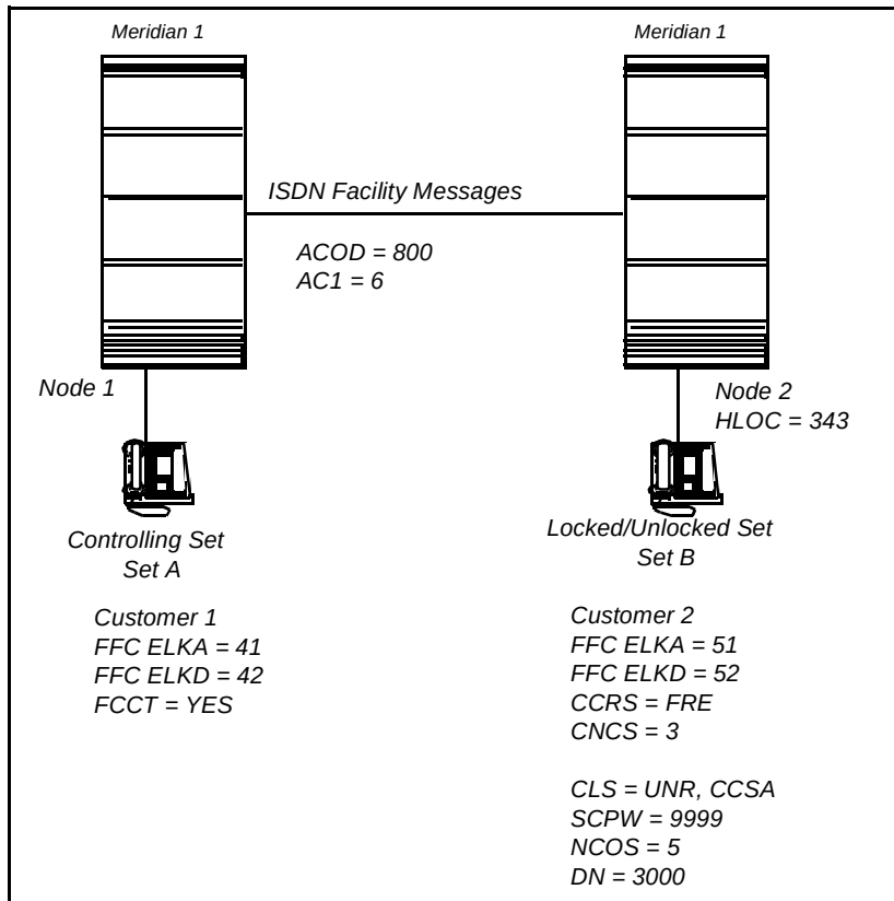
Figure 60 Network Electronic Lock
