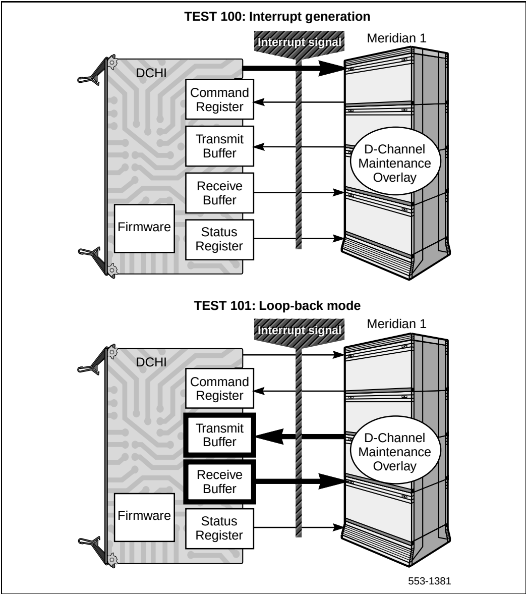
Figure 186 DCH tests 100 and 101
