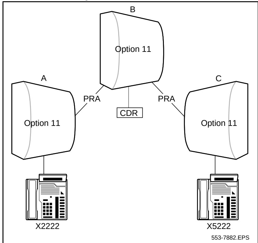
Figure 48 CDR in Multi-site Configuration
