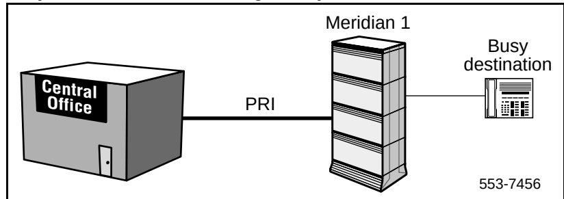
Figure 10 Busy set is a on node tandemed to a Central Office
