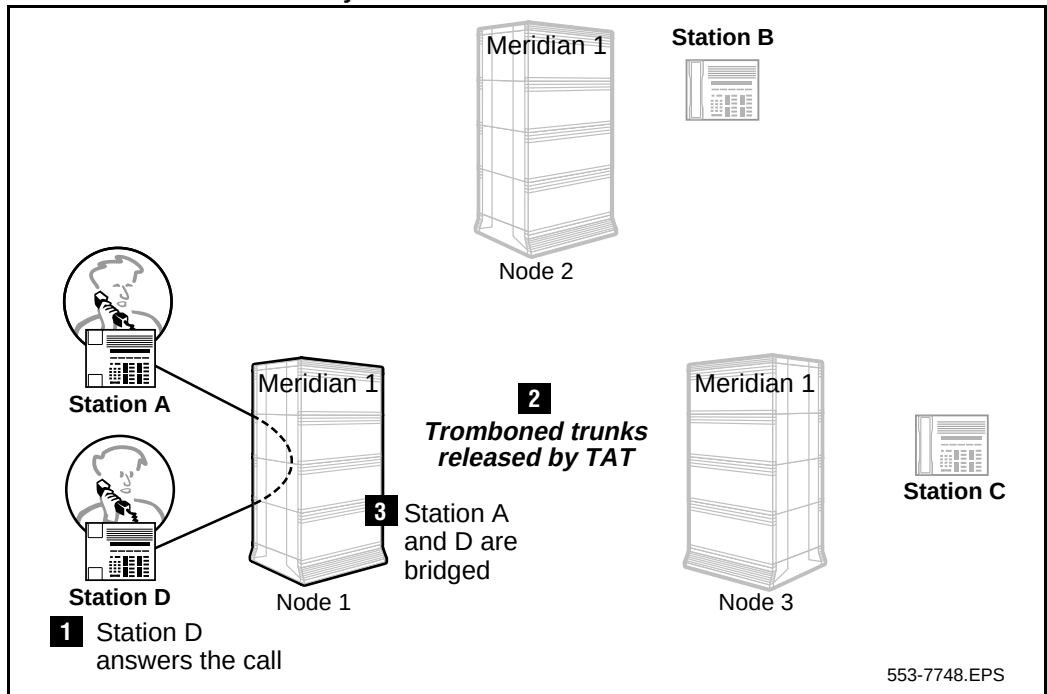
Figure 168 Tromboned trunks released by TAT
