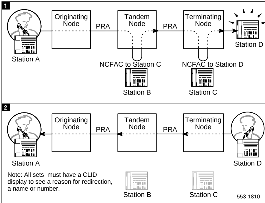
Figure 118 Tandem NCFAC intranode
