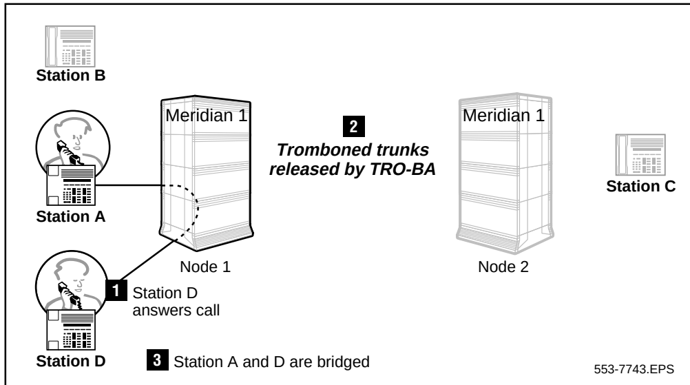
Figure 163 Tromboned trunks released by TRO-BA
