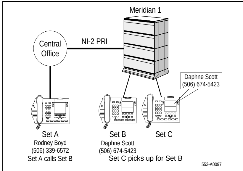
Figure 133 Call Pickup in a stand-alone environment
