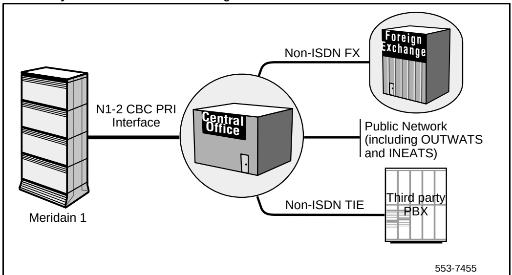
Figure 137 NI-2 Call By Call Service Selection configuration
