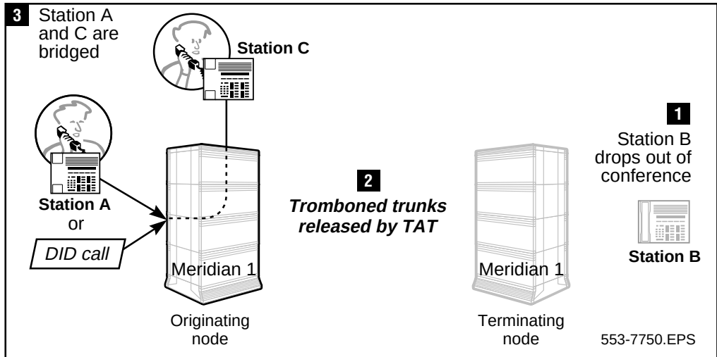
Figure 170 Conference call after TAT
