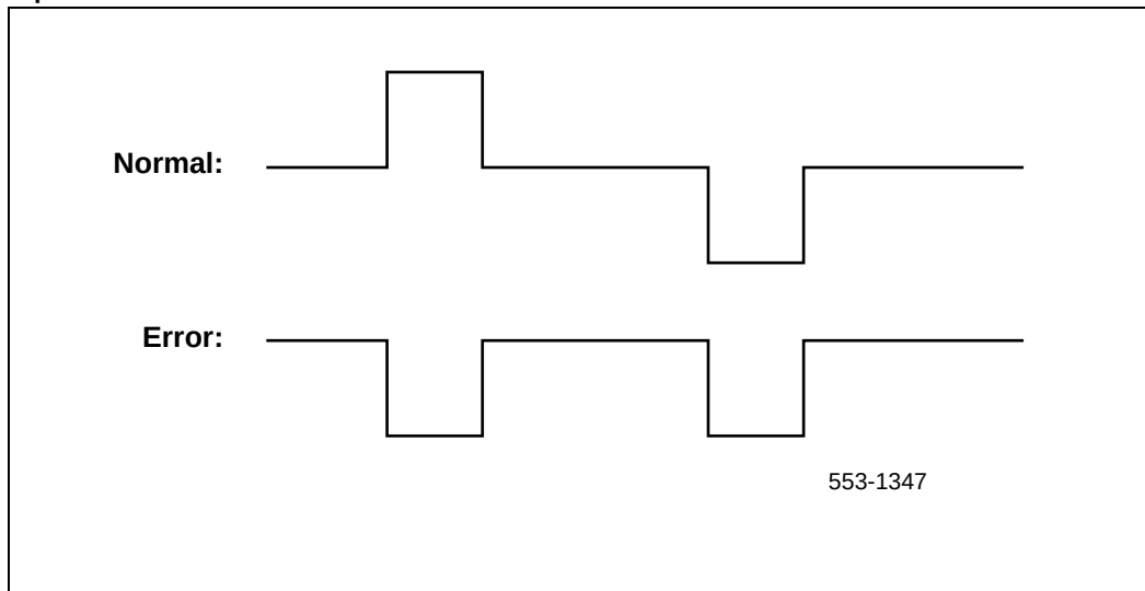
Figure 1 Bipolar violations
