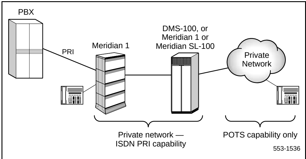
Figure 61 Private Network Hopoff
