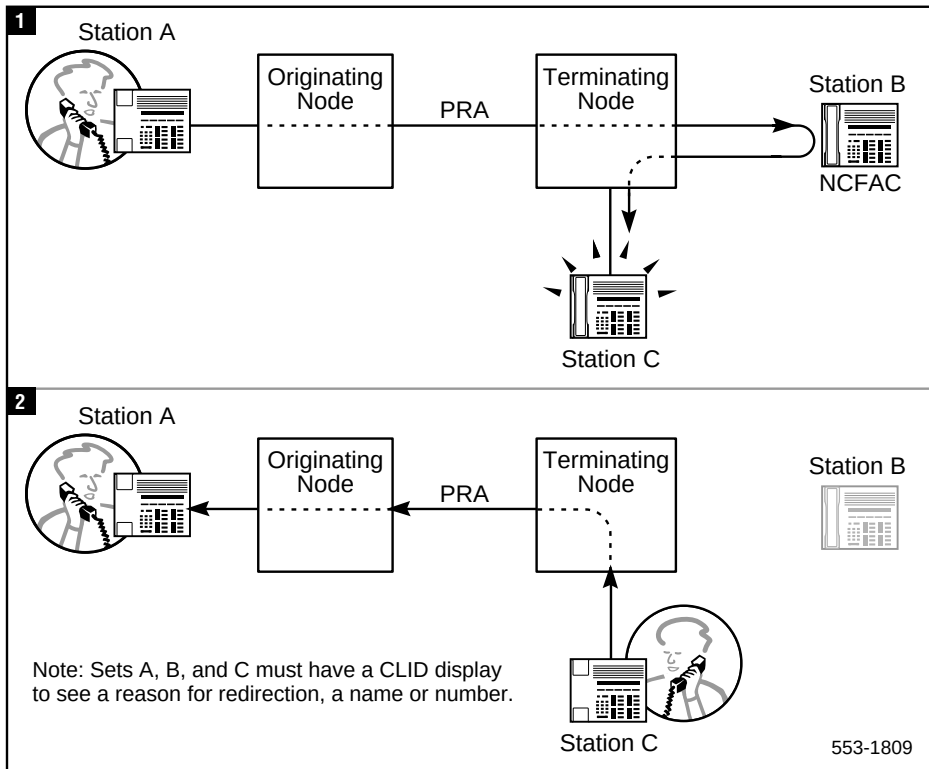
Figure 115 NCFAC intranode redirection
