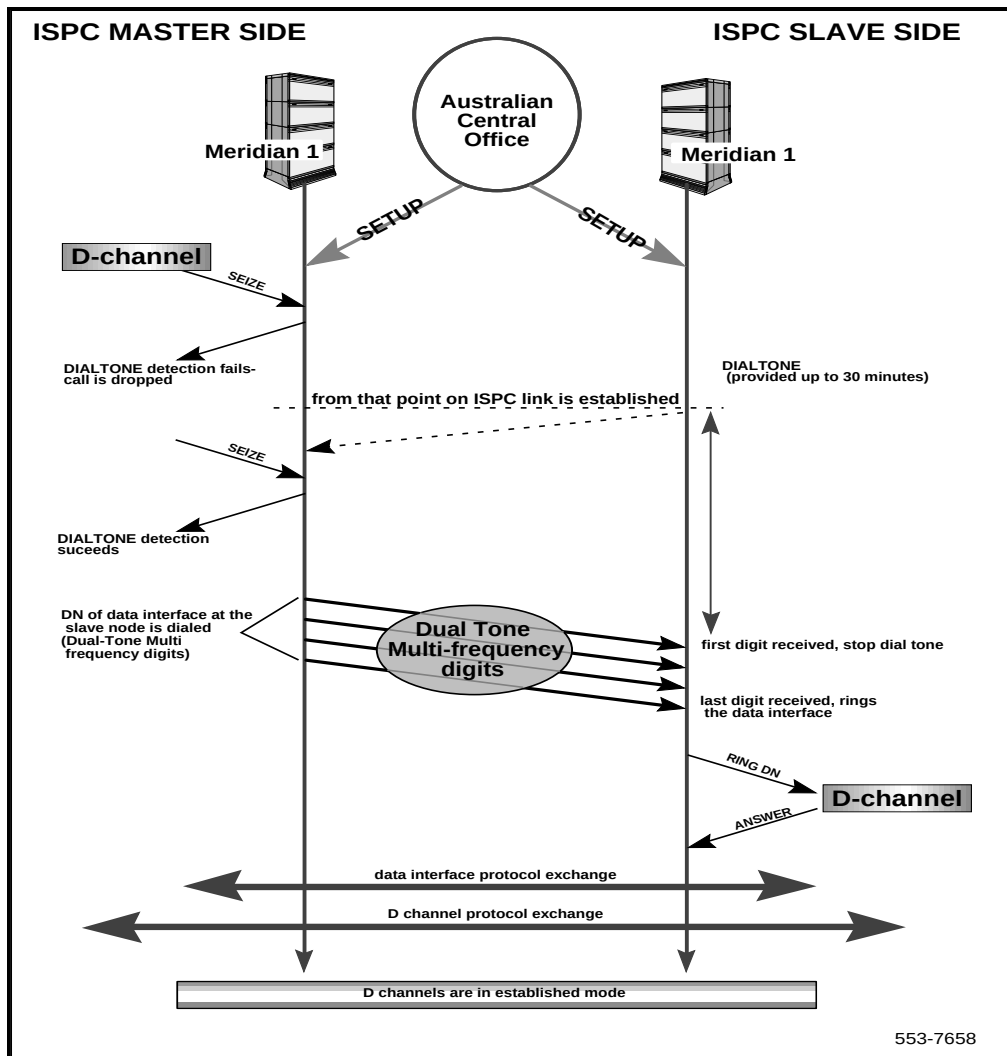
Figure 93 Mechanism Used to Synchronize Data Interfaces
