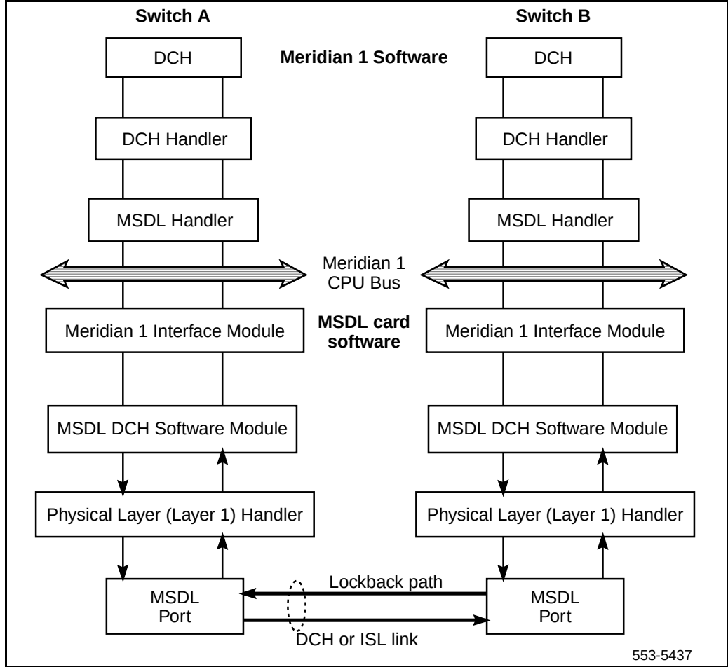
Figure 189 Remote loopback tests (NT6D80)
