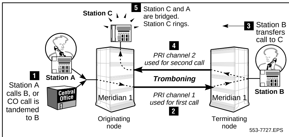
Figure 148 Before Trunk Anti-Tromboning operation
