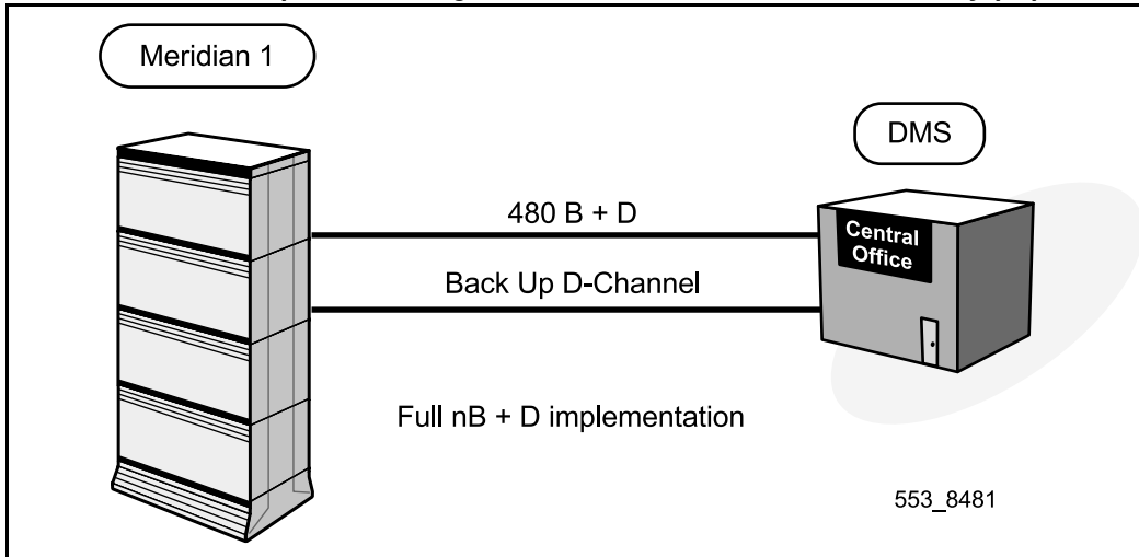
Figure 5 510 trunk members expansion configured for a Meridian 1 to DMS connectivity (E1)
