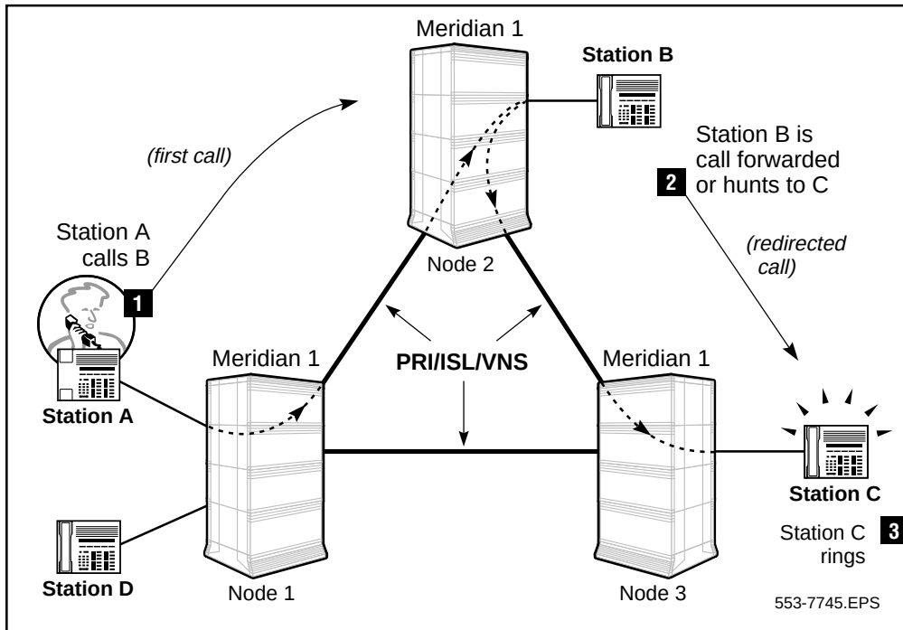
Figure 165 Call path before TRO-BA has been applied
