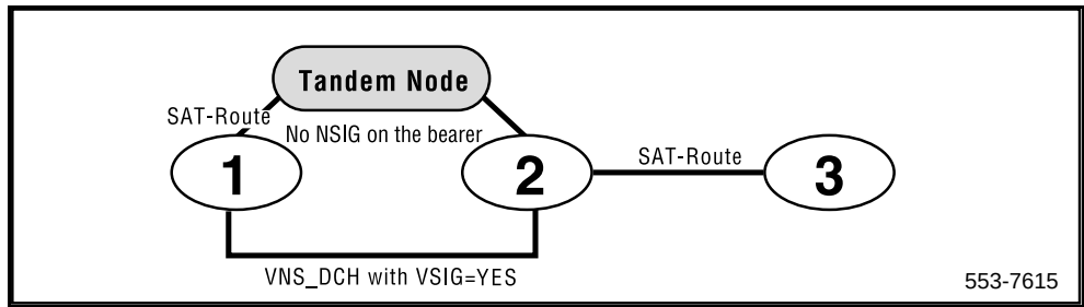
Figure 127 SAT-count is not updated when NSIG is not configured on the bearer (VSIG = YES and SIGO is set to STD)
