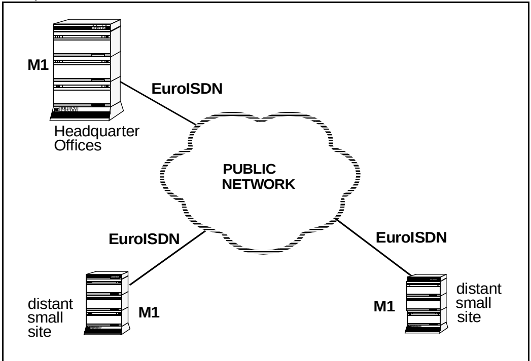
Figure 35 Example of a network where BNE is useful
