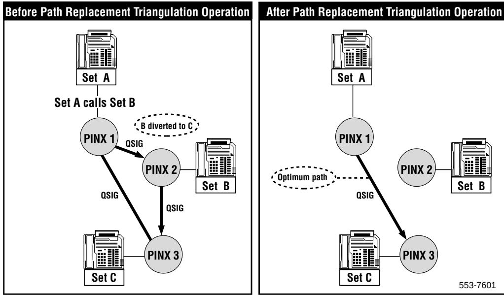
Figure 91 Tromboning Path Replacement
