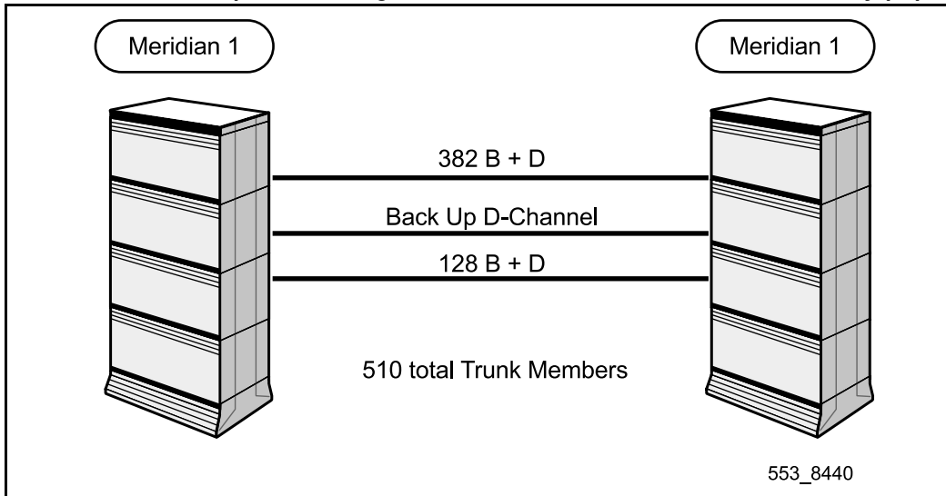
Figure 2 510 trunk members expansion configured for a Meridian 1 to Meridian 1 connectivity (T1)
