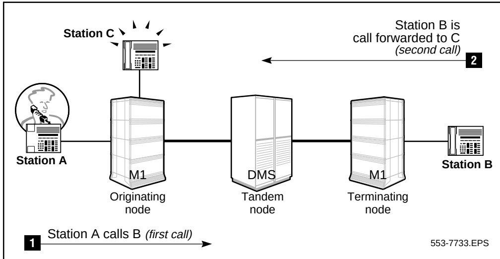
Figure 154 Anti-tromboning for Call Modification, DMS/M1
