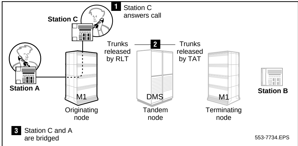
Figure 155 Results of anti-tromboning for network call transfer, DMS/M1
