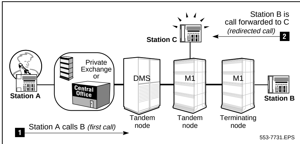
Figure 152 Anti-tromboning for Network Call Redirection (case 2), M1/DMS
