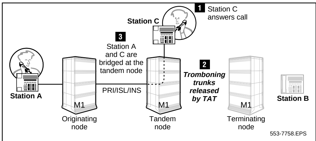
Figure 178 Network Call Redirection after TAT
