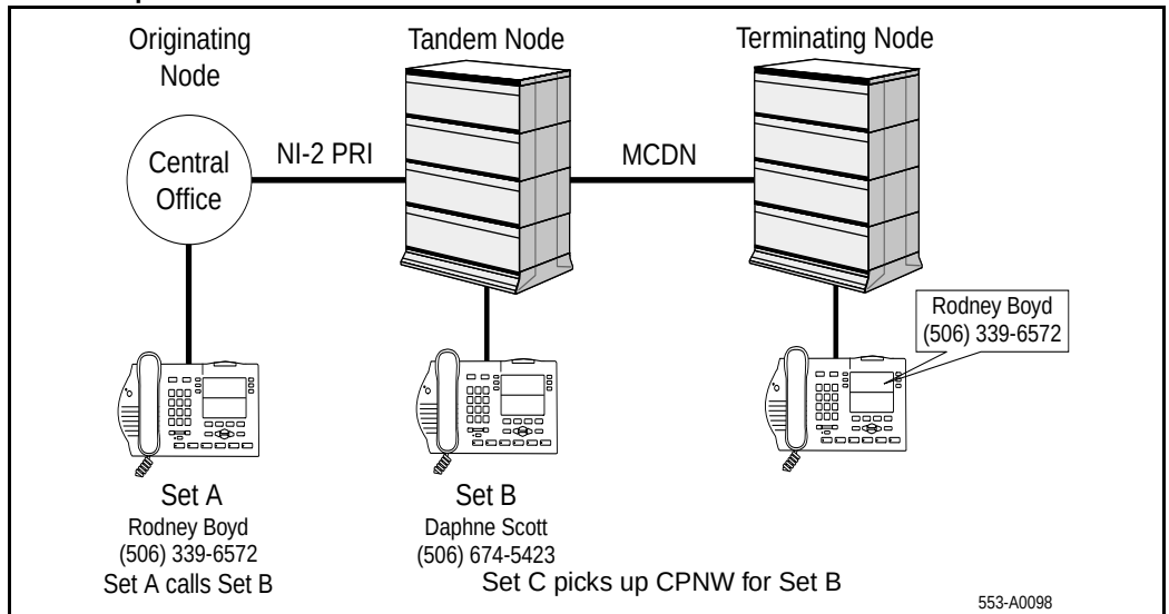
Figure 134 Call Pickup Network Wide
