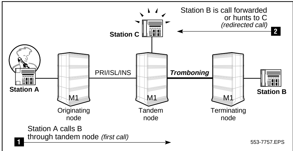
Figure 177 Network Call Redirection before TAT
