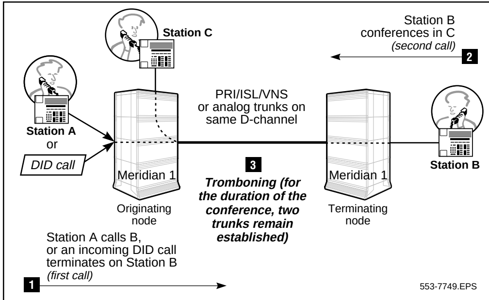
Figure 169 Conference call before TAT
