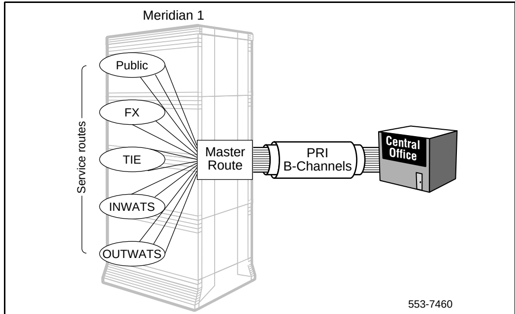
Figure 138 NI-2 CBC master route and service routes on the Meridian 1
