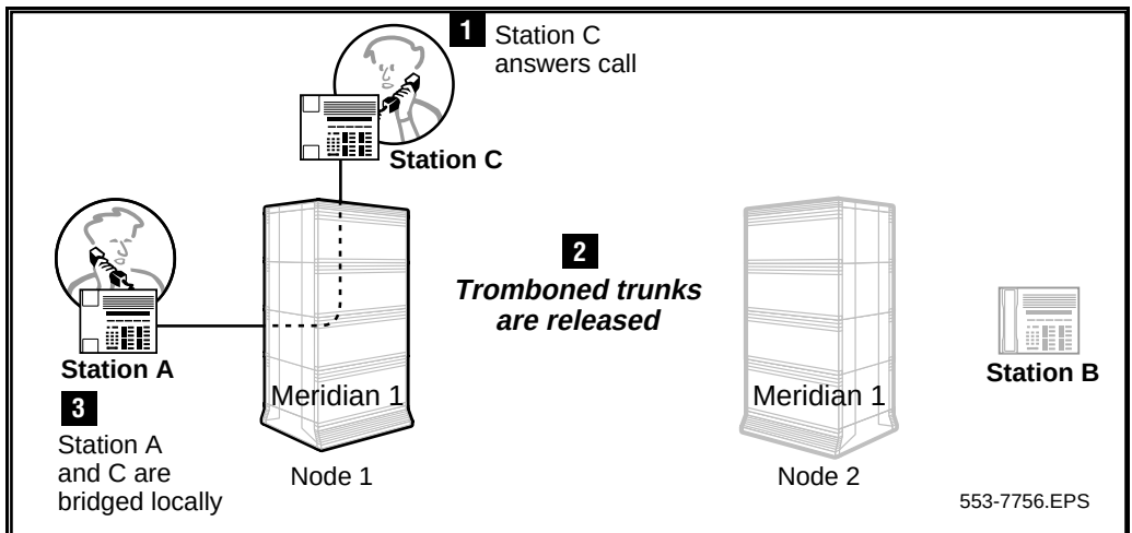
Figure 176 Network Call Pickup after TAT
