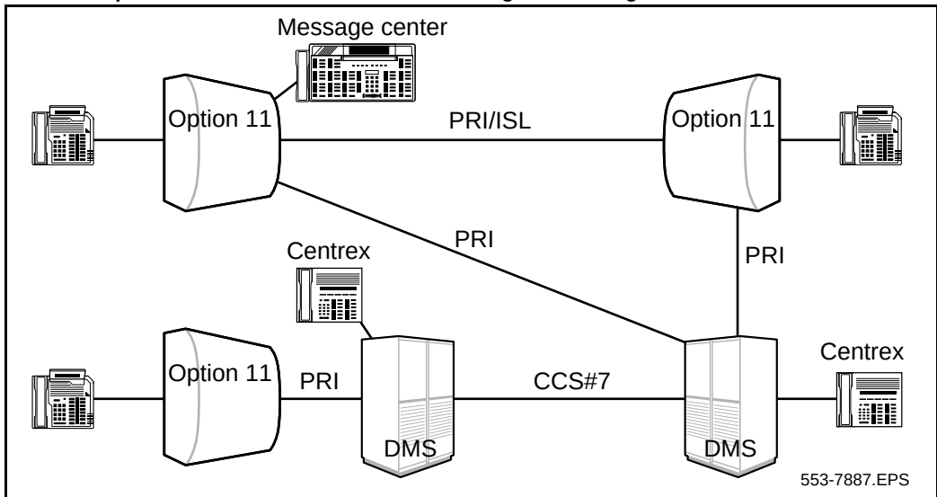
Figure 101 Private corporate network with Meridian 1 hosting the Message Center
