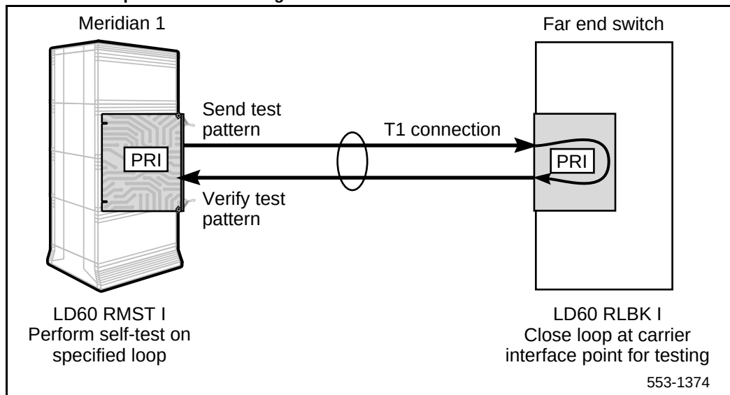
Figure 185 PRI remote loop-back and link diagnostic tests
