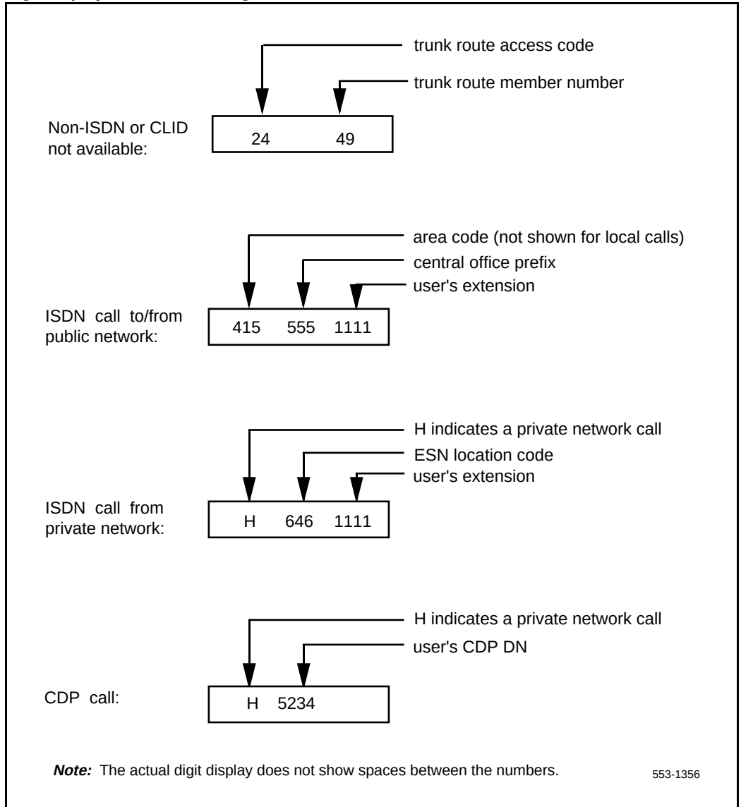
Figure 47 Digit display format for Calling Line Identification
