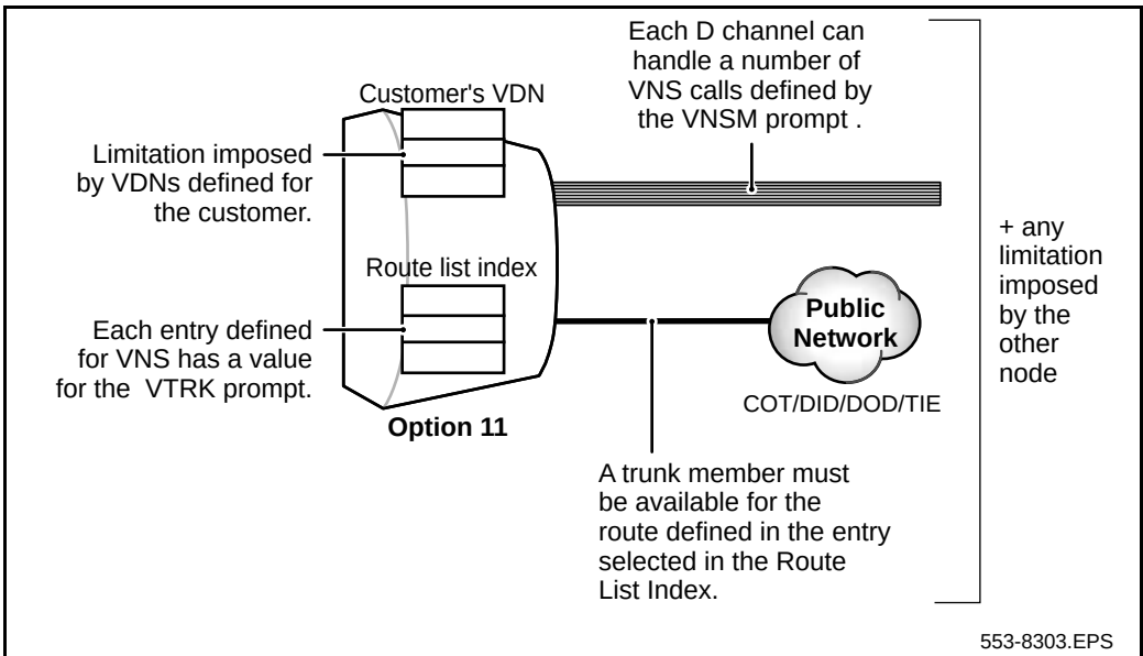
Figure 183 VNS Call Limitations
