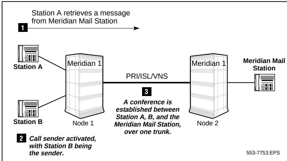
Figure 173 Call Sender operation, with Network Message Services active
