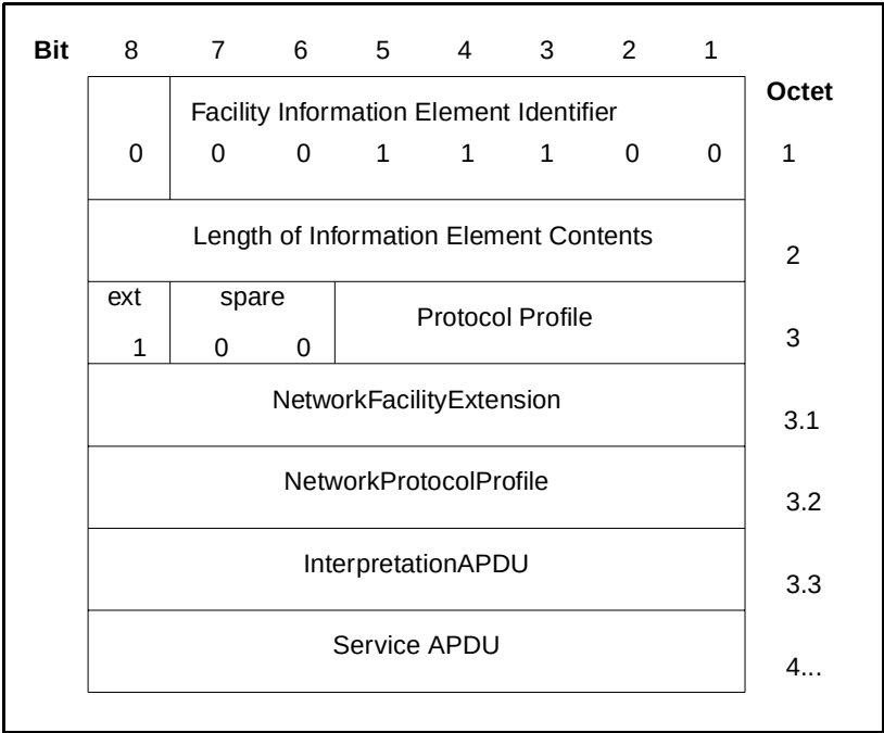
Figure 74 Facility IE layout
