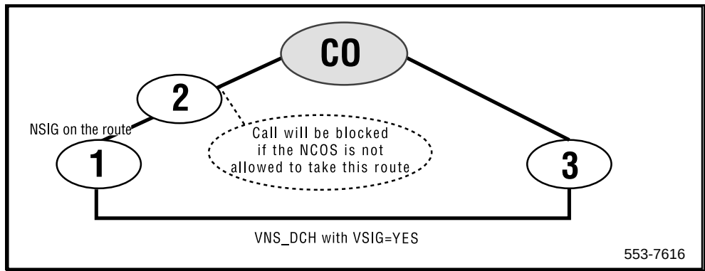
Figure 128 A scenario where the call is blocked, as NCOS is insufficient (VSIG = YES and SIGO is not set to STD)
