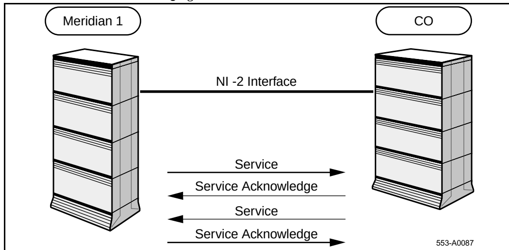
Figure 130 NI-2 B-channel Service messaging
