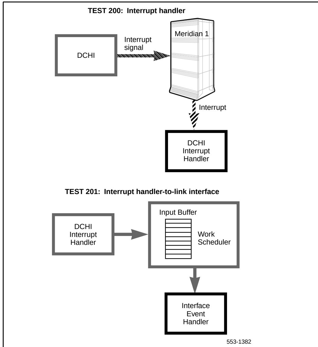
Figure 187 DCH tests 200 and 201
