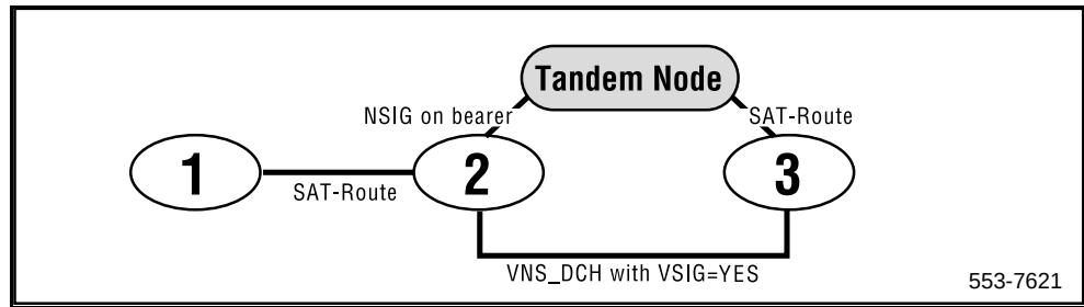
Figure 124 A scenario involving two SAT-Routes where VSIG = YES and SIGO is not set to STD
