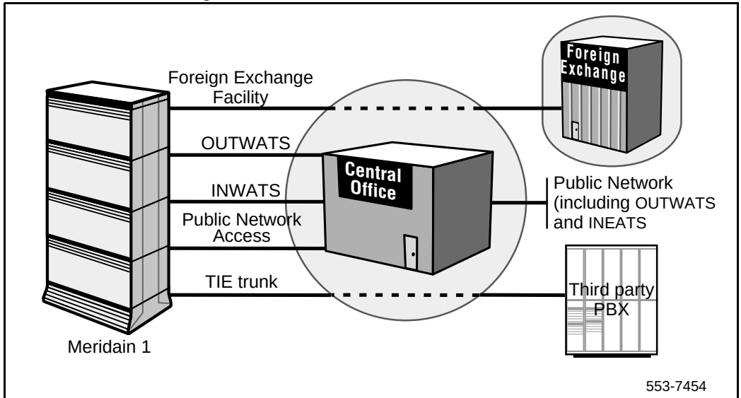
Figure 136 Dedicated facilities configuration
