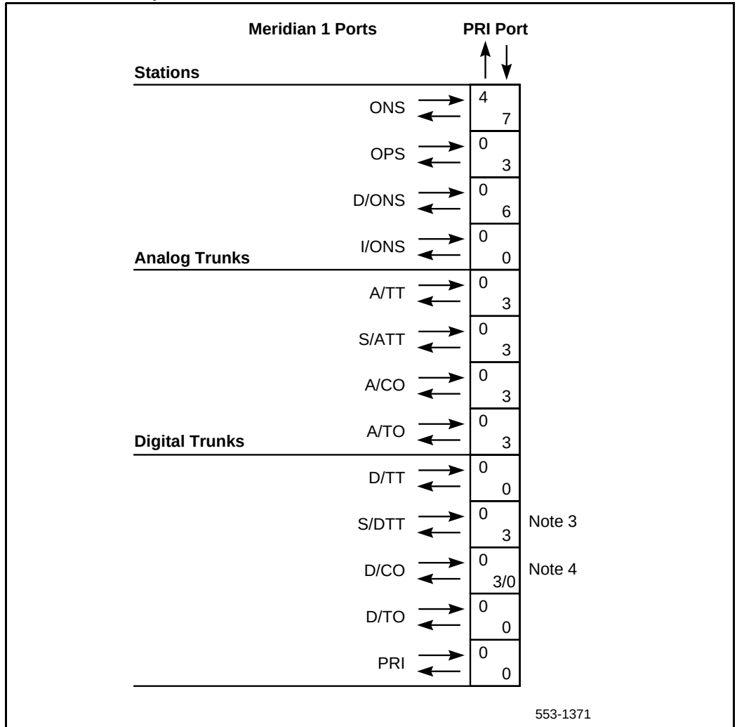
Figure 184 PRI loss and level plan
