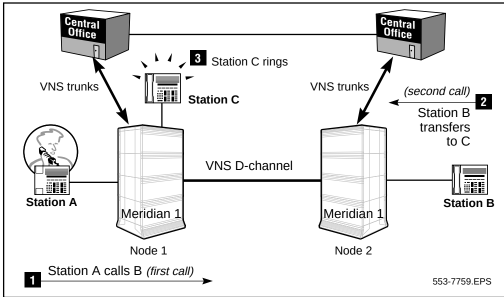
Figure 179 VNS before TAT
