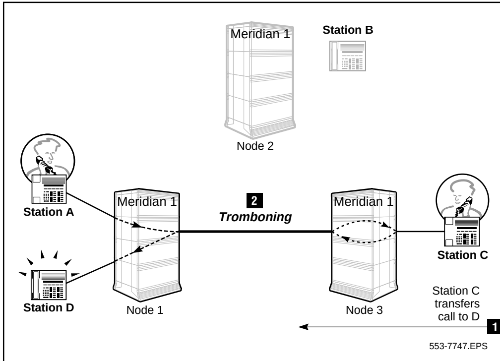
Figure 167 Tromboning of trunks after TRO-BA has been applied
