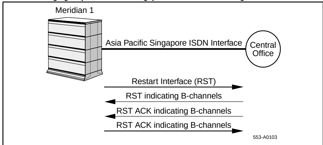
Figure 147 Restart messaging sequence for the Singapore ISDN Restart Message Enhancement
