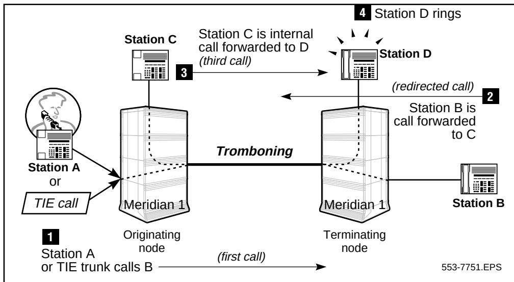
Figure 171 Internal Call Forward before TAT, Node 2 is a Meridian 1
