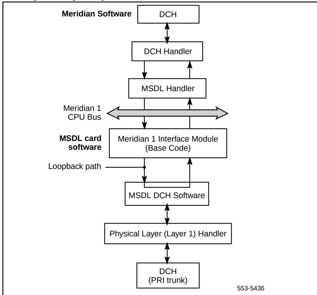
Figure 188 Local loopback test (NT6D80)
