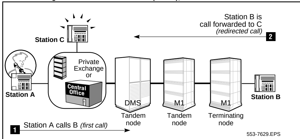
Figure 150 Anti-tromboning for Network Call Redirection (case 1), M1/DMS
