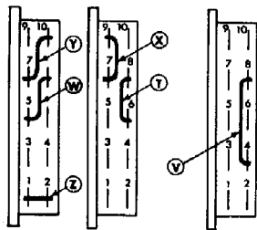
FIGURE 7. K400(D) KTU, Circuit Options
