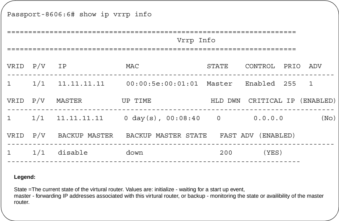
Figure 177 show ip vrrp info command output
