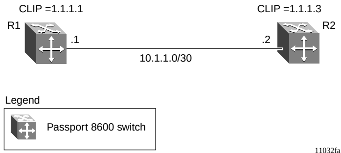
Figure 26 MD5 authentication example
