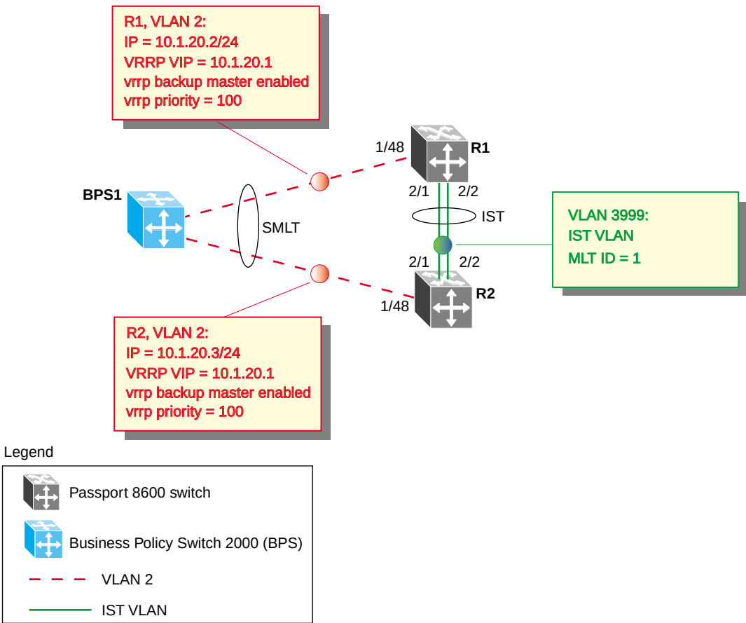
Figure 45 VRRP example with SMLT
