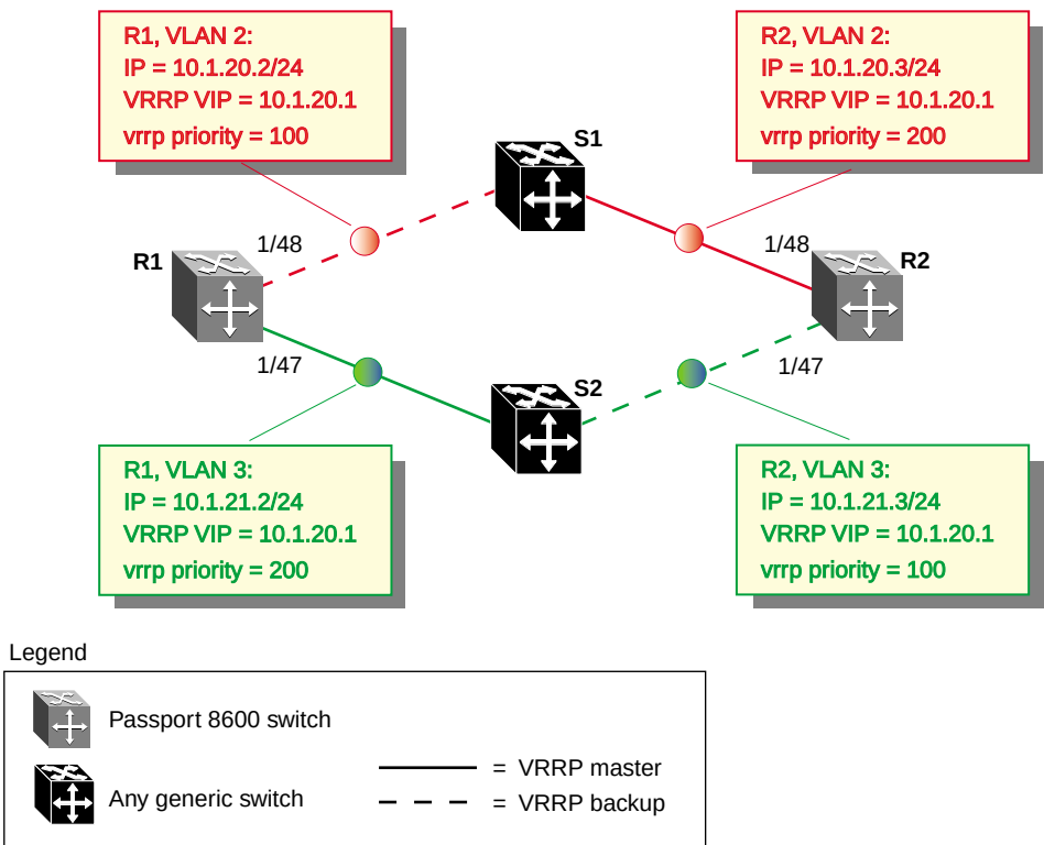
Figure 42 VRRP example
