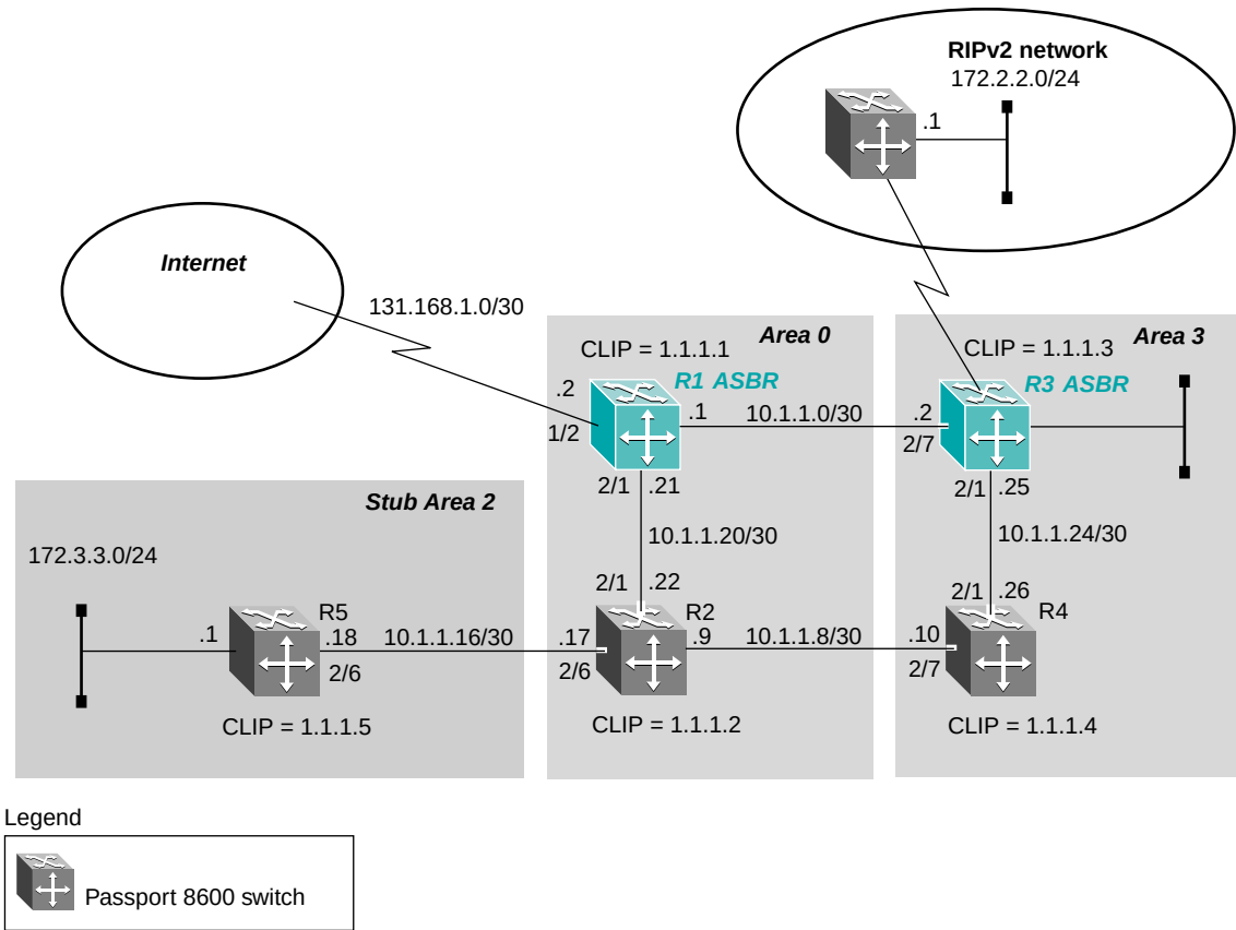
Figure 41 Multi-area complex configuration example
