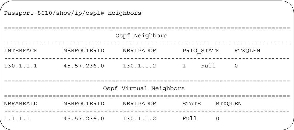
Figure 160 show ospf neighbors command output
