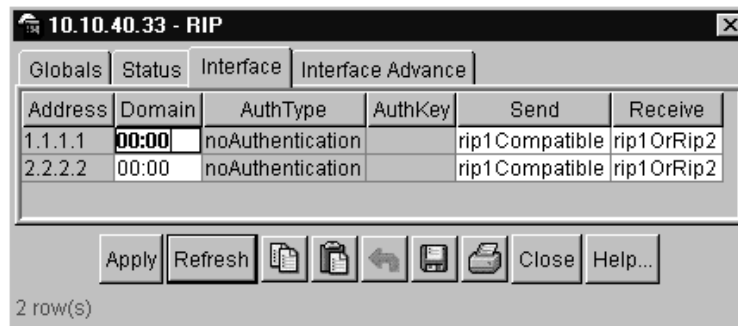
Figure 110 RIP dialog box—Interface tab
