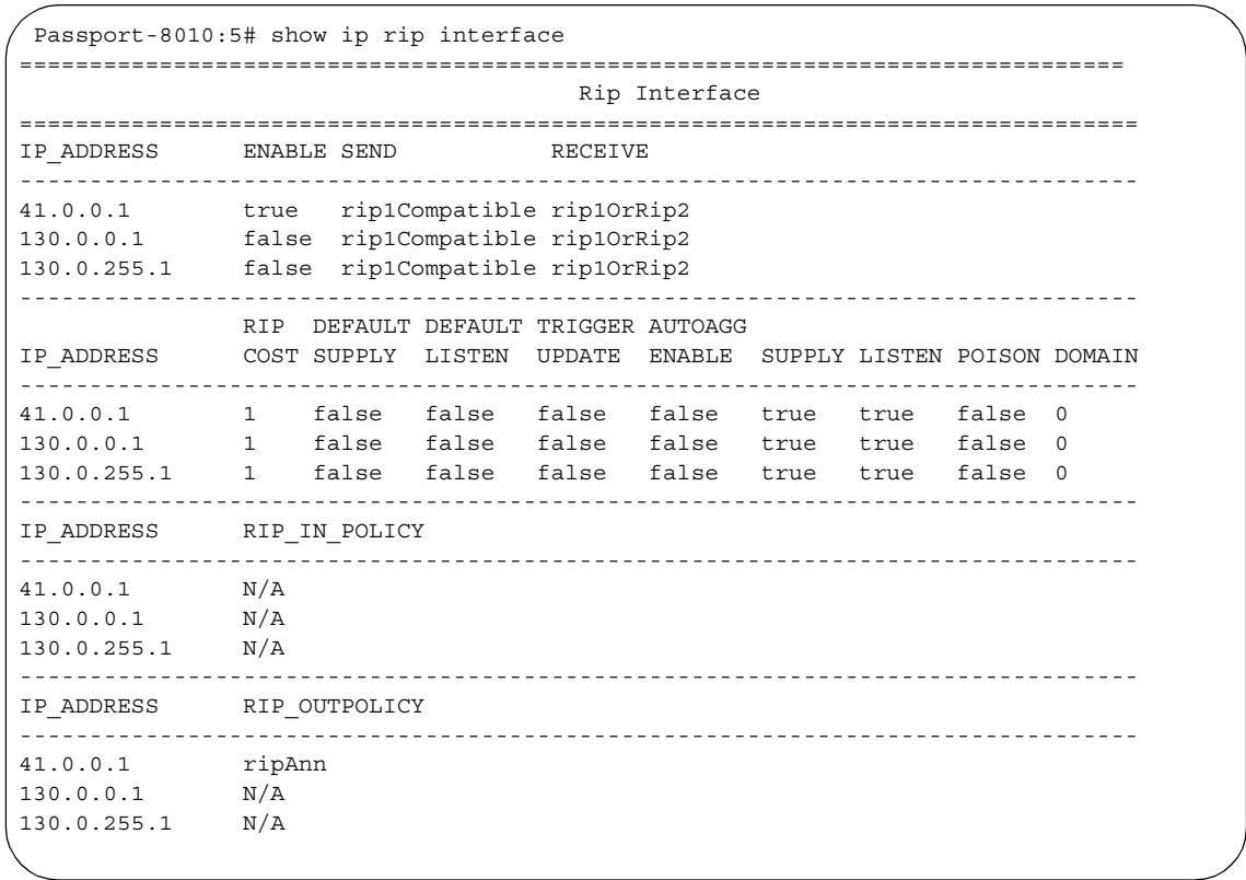
Figure 115 show ip rip interface command output
