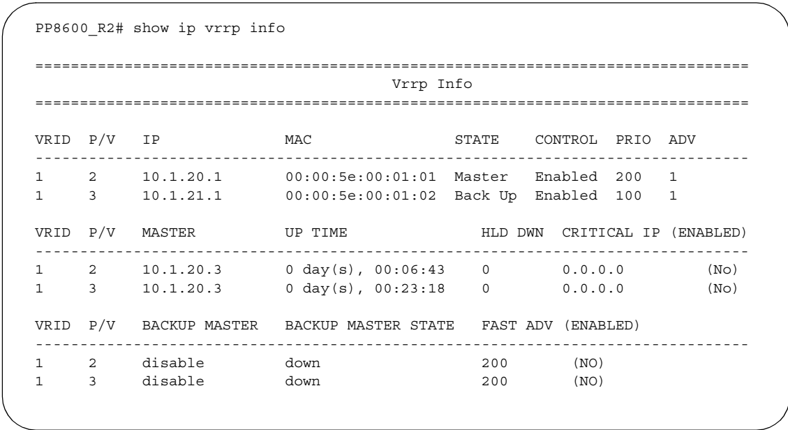
Figure 44 show ip vrrp info command for R2
