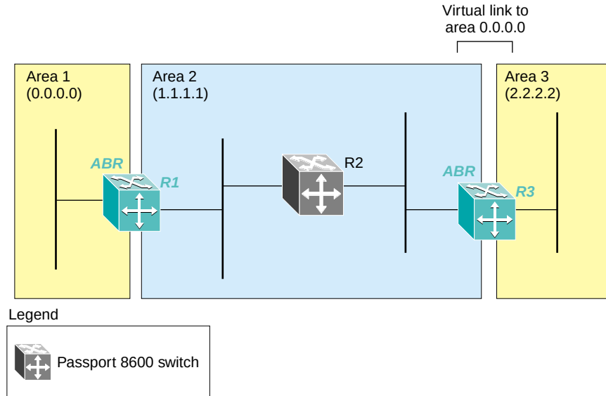
Figure 13 Virtual link between ABRs through a transit area
