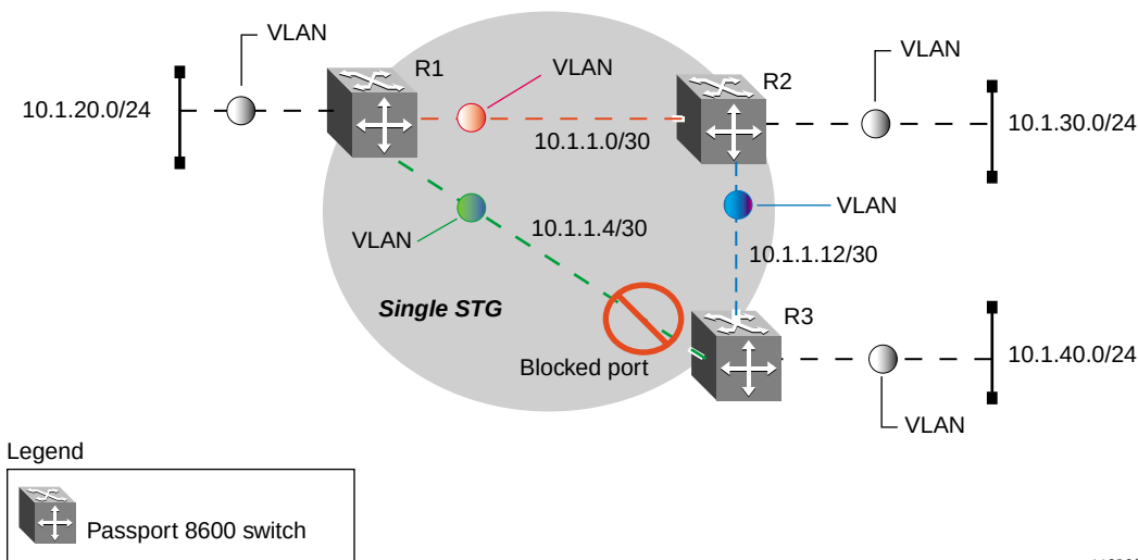
Figure 18 Single spanning tree group
