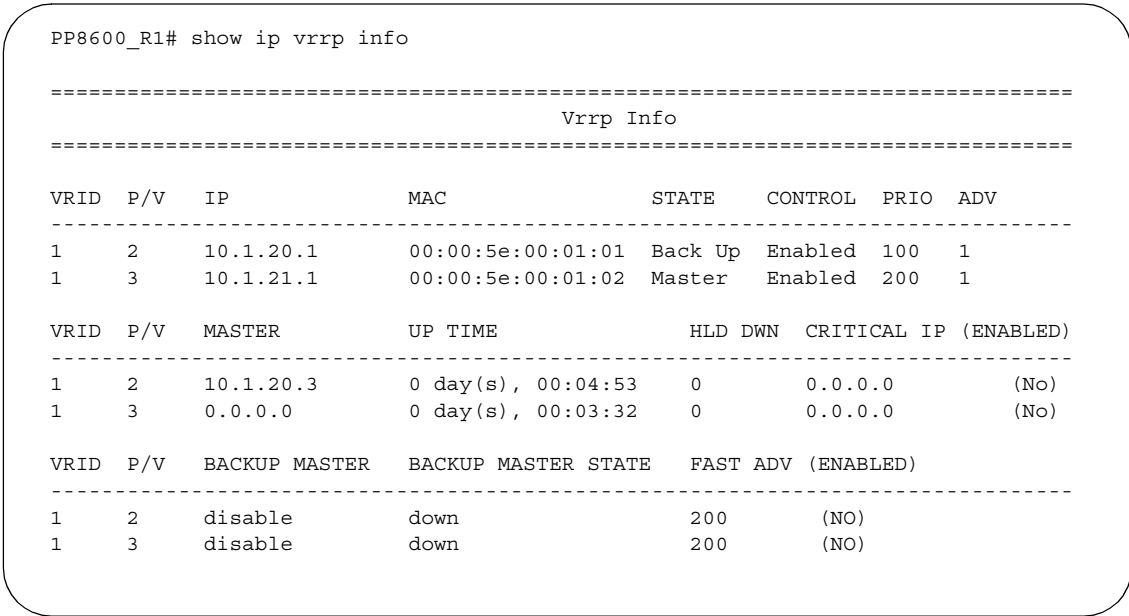
Figure 43 show ip vrrp info command for R1
