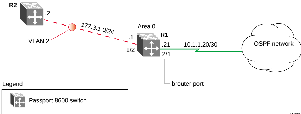
Figure 23 OSPF example
