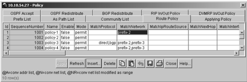
Figure 187 Policy dialog box—Route Policy tab
