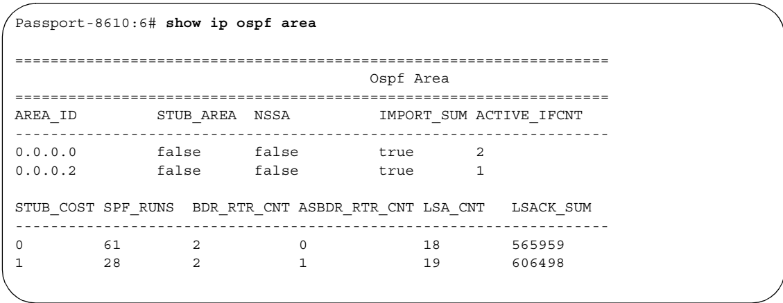
Figure 35 show ip OSPF area
