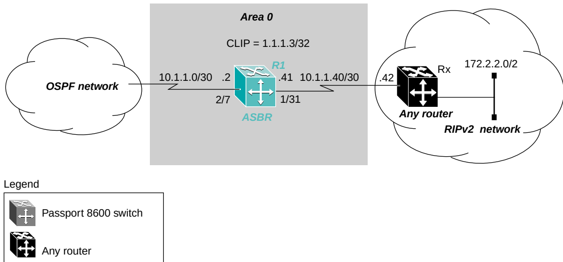
Figure 37 OSPF routes: OSPF/RIP and RIP/OSPF
