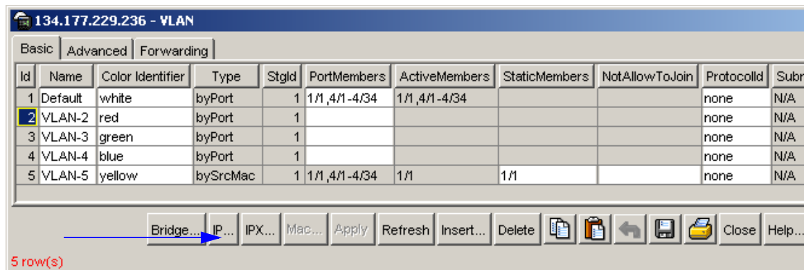
Figure 206 VLAN dialog box—Basic tab
