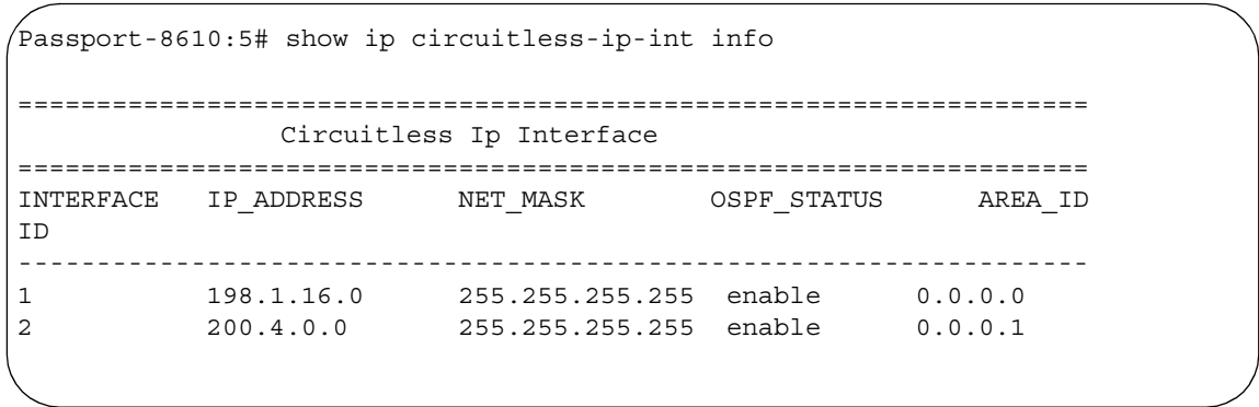
Figure 90 show ip circuitless-ip-int info command output
