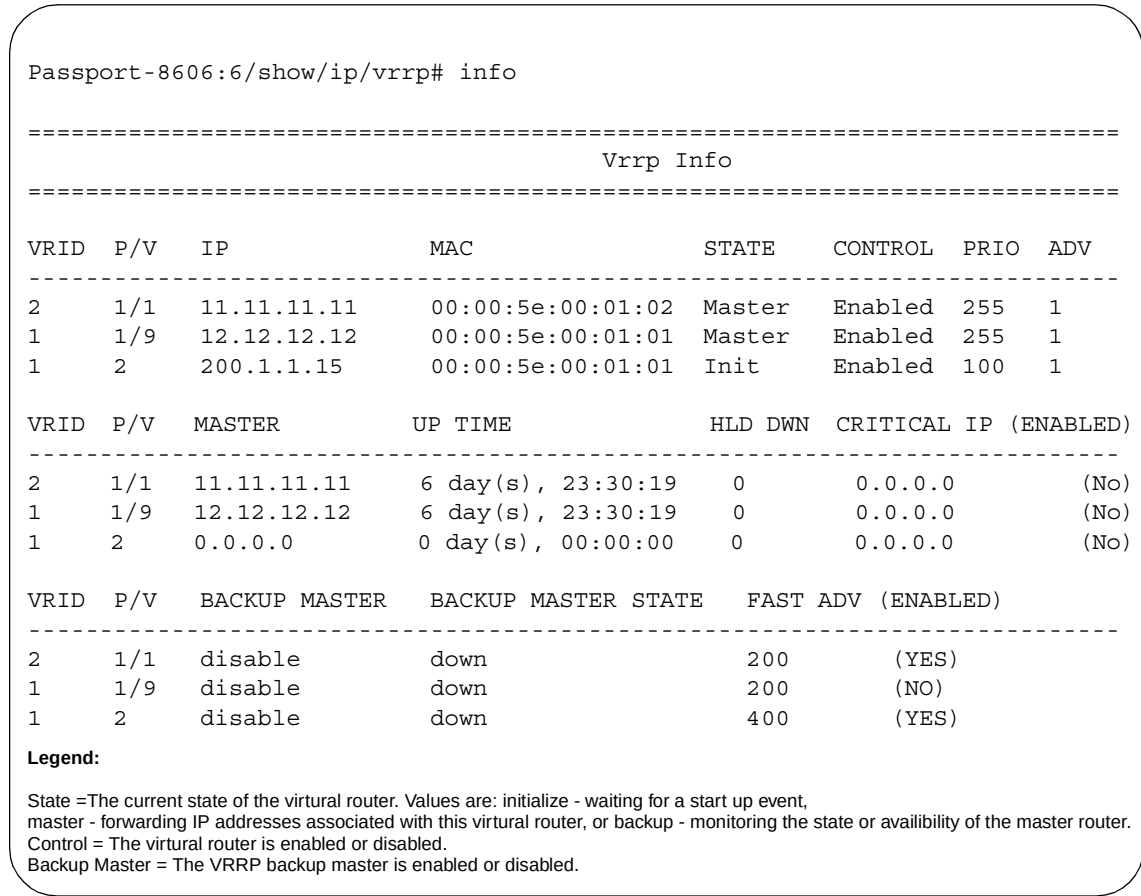
Figure 180 show ip vrrp info command output
