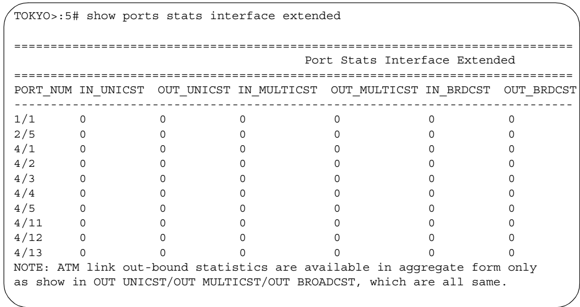
Figure 166 show ports stats interface extended command output
