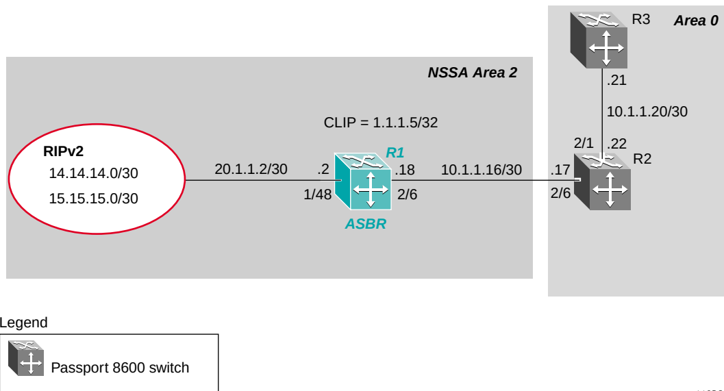
Figure 40 Controlling external routes advertised
