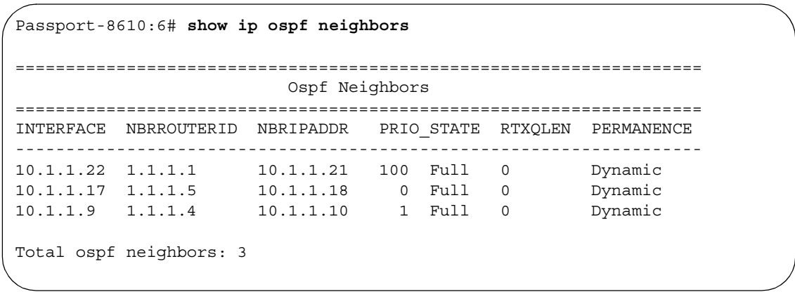
Figure 27 show ip OSPF neighbors
