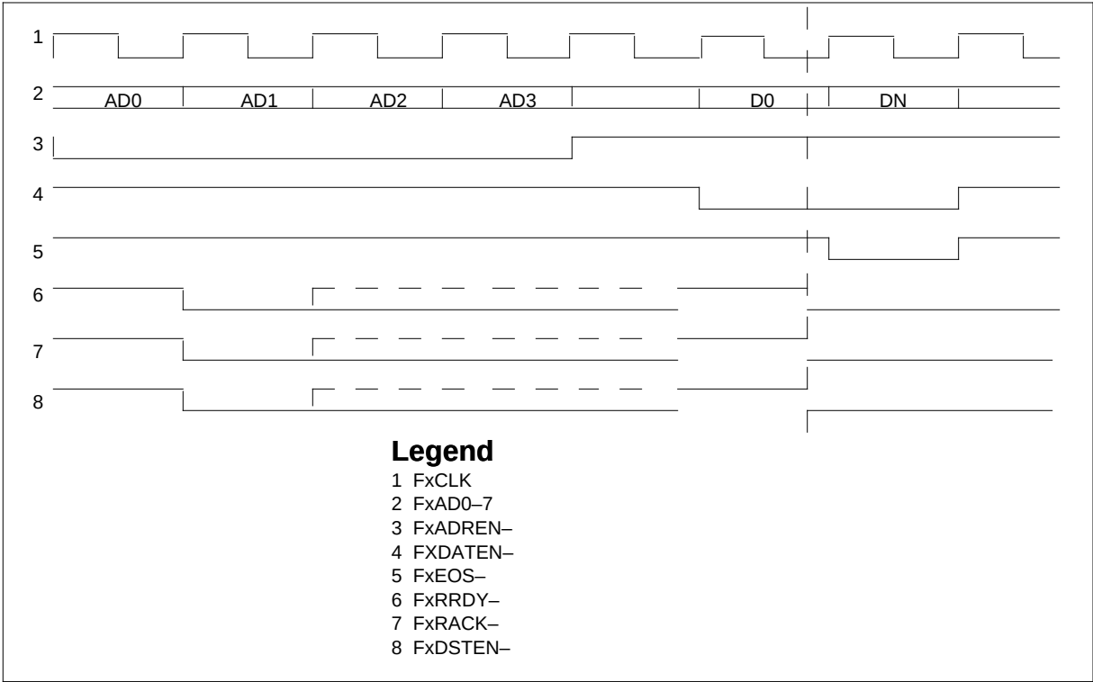
NT9X73AA RA to LIU7 F-bus protocol timing
