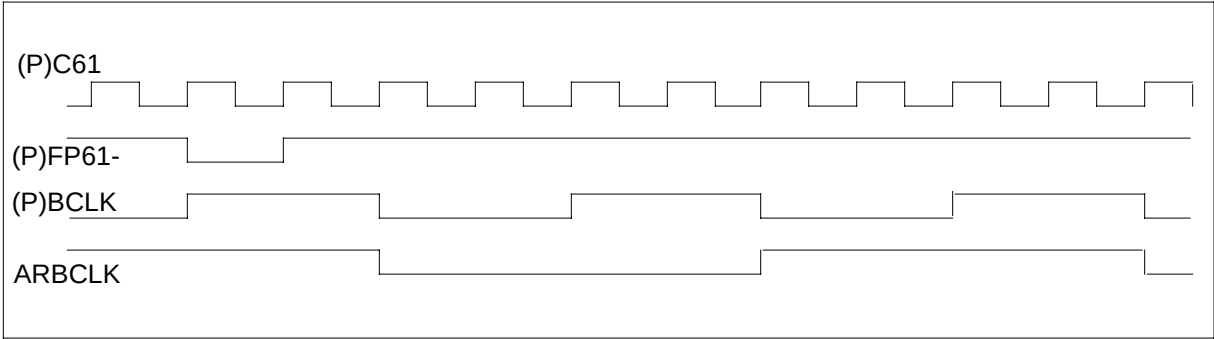
NT9X15AA clock signal relationships
