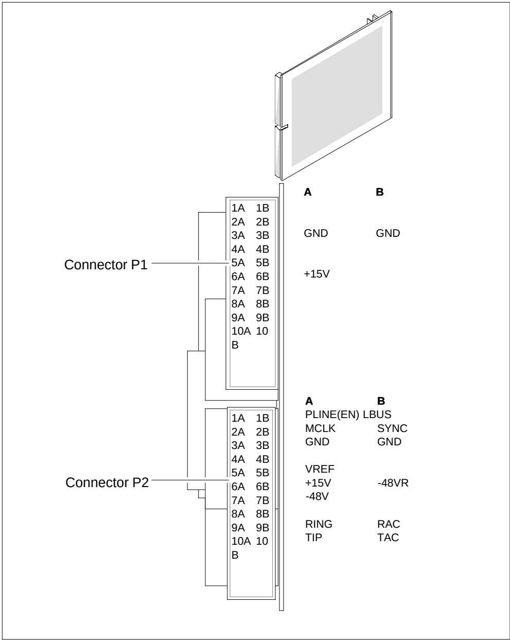
NT6X71AC pin numbers
