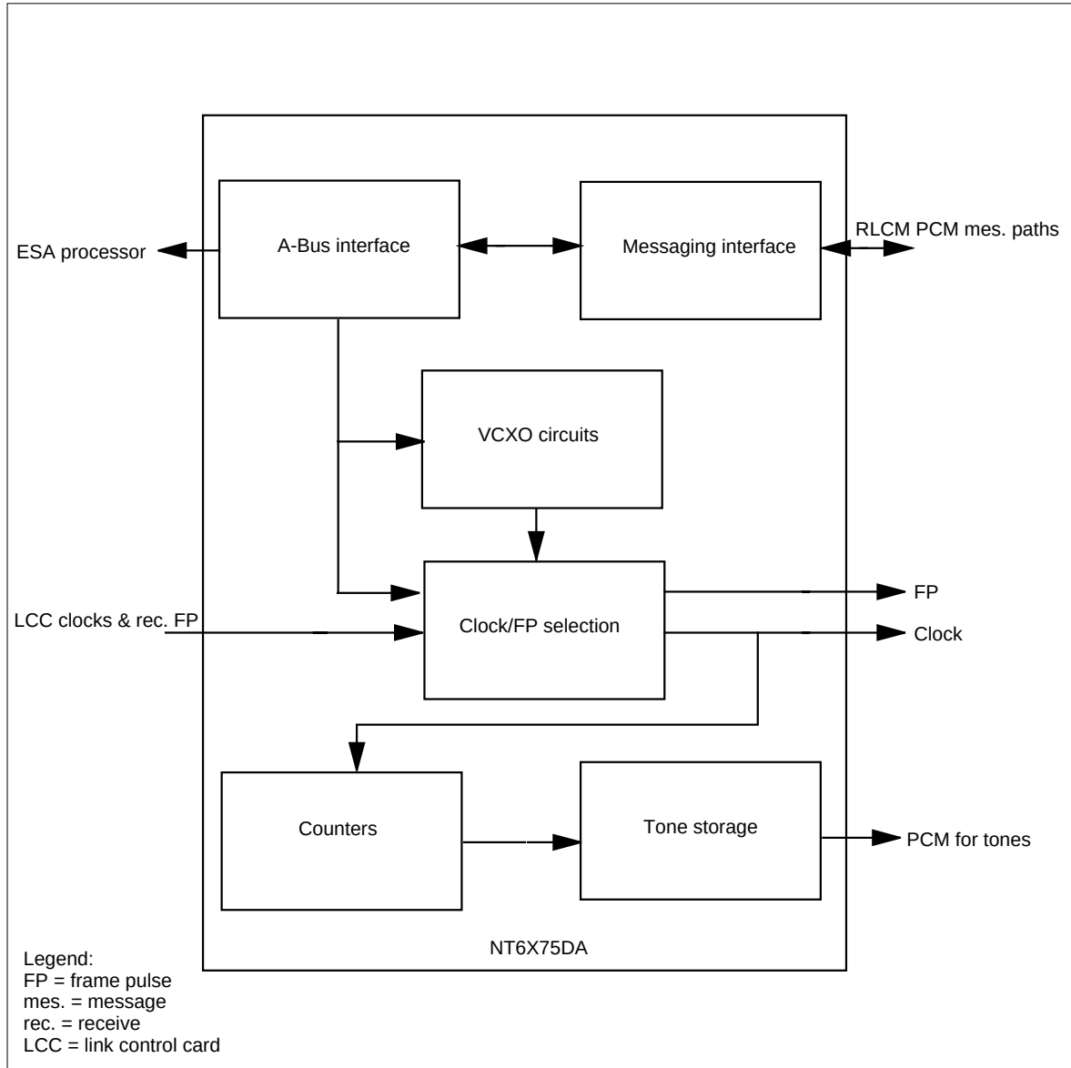
NT6X75DA functional block diagram
