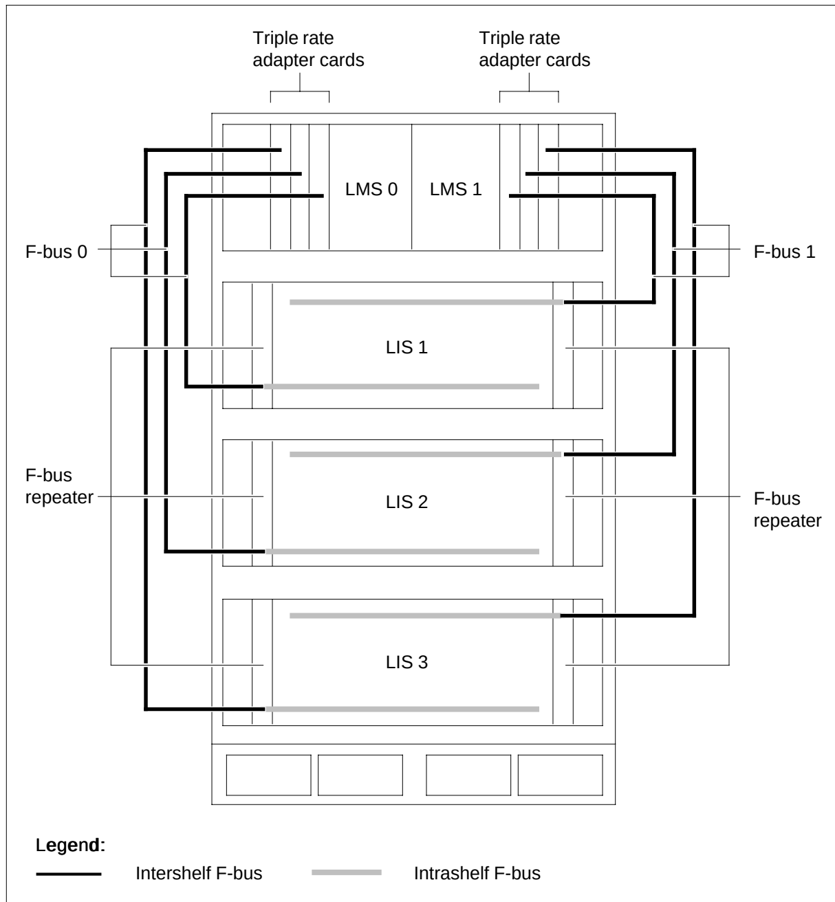
Triple F-bus configuration in an ELPP cabinet
