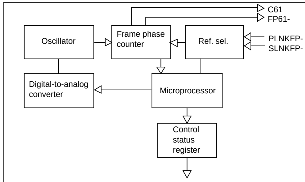
NT9X22CA operating blocks
