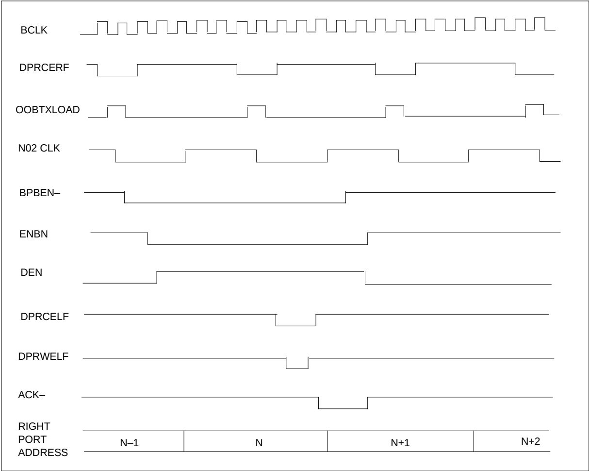
CLRPCM timing diagram
