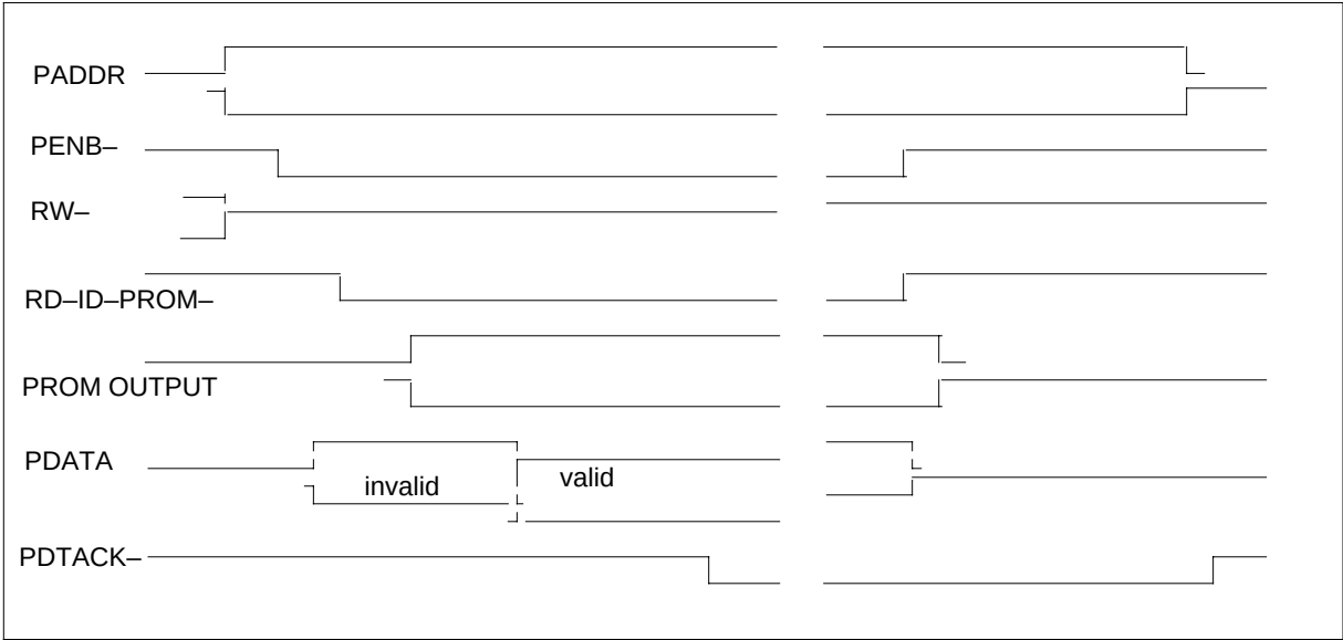
NT9X46AA ID PROM read timing
