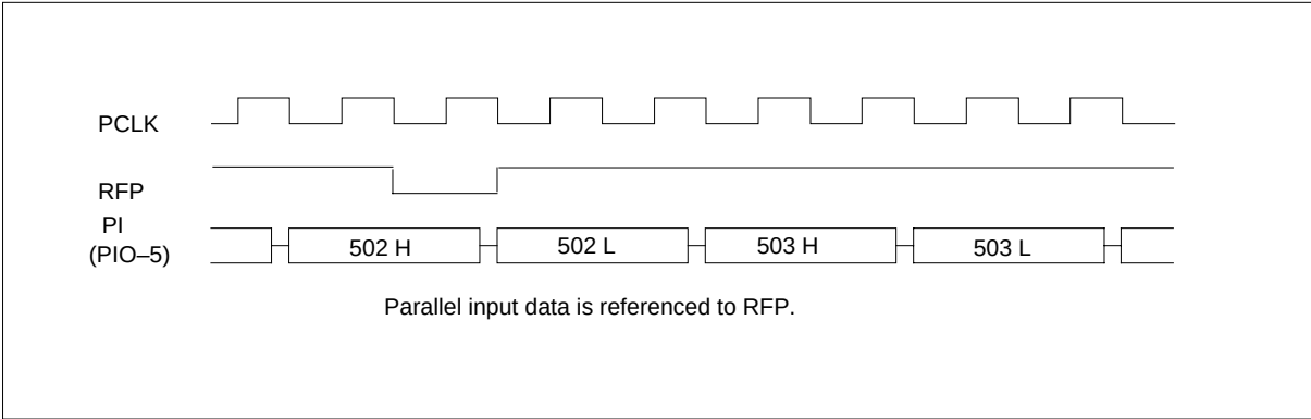
NT9X41BA parallel input port channel timing
