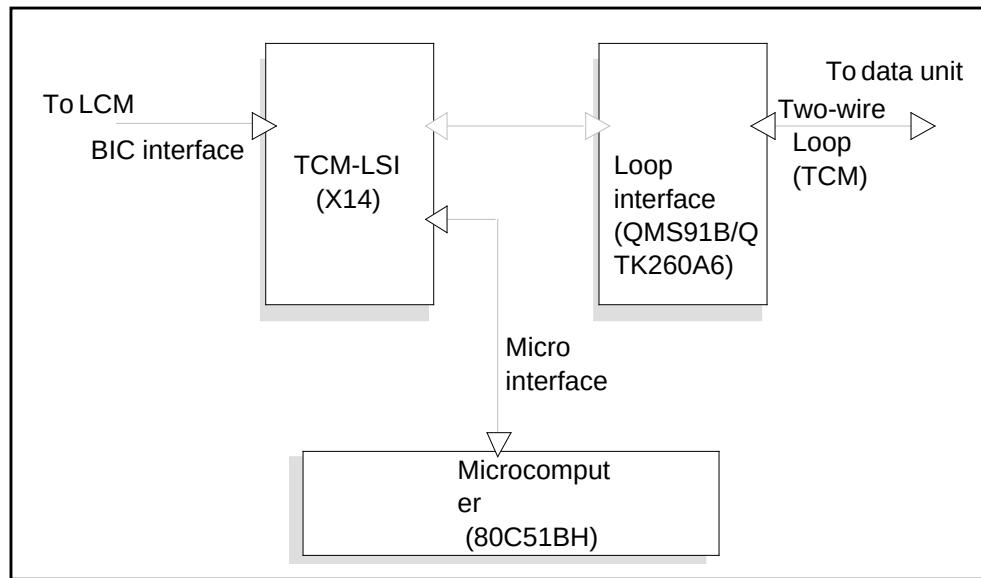
NT6X71AC functional blocks
