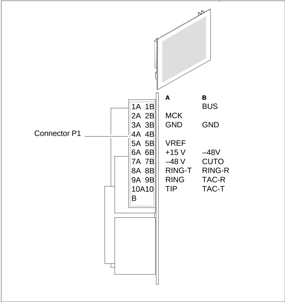
NT6X93CA pin numbers
