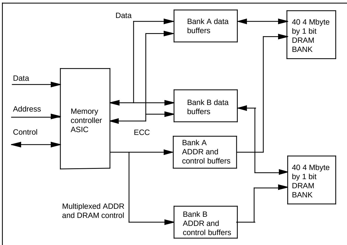
NT9X14FA functional blocks of memory modules 1, 2, and 3
