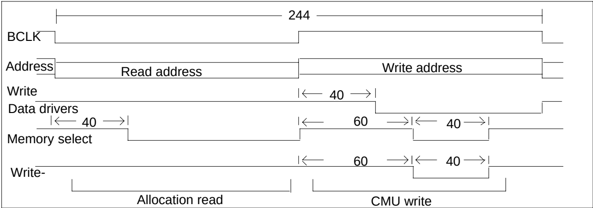
NT9X15AA RAM control signal timing (time is in ns)
