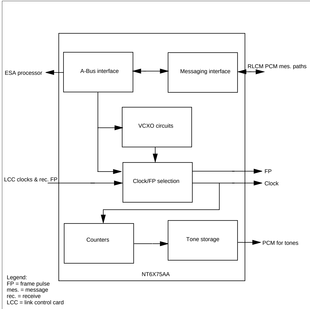
NT6X75AA functional block diagram
