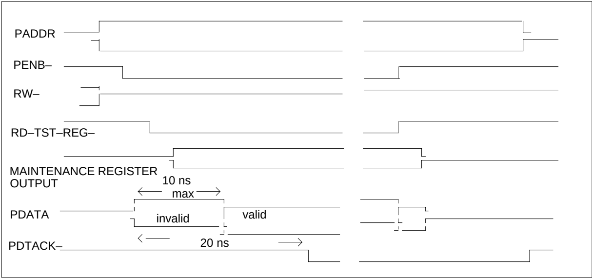
NT9X46AA maintenance register read timing
