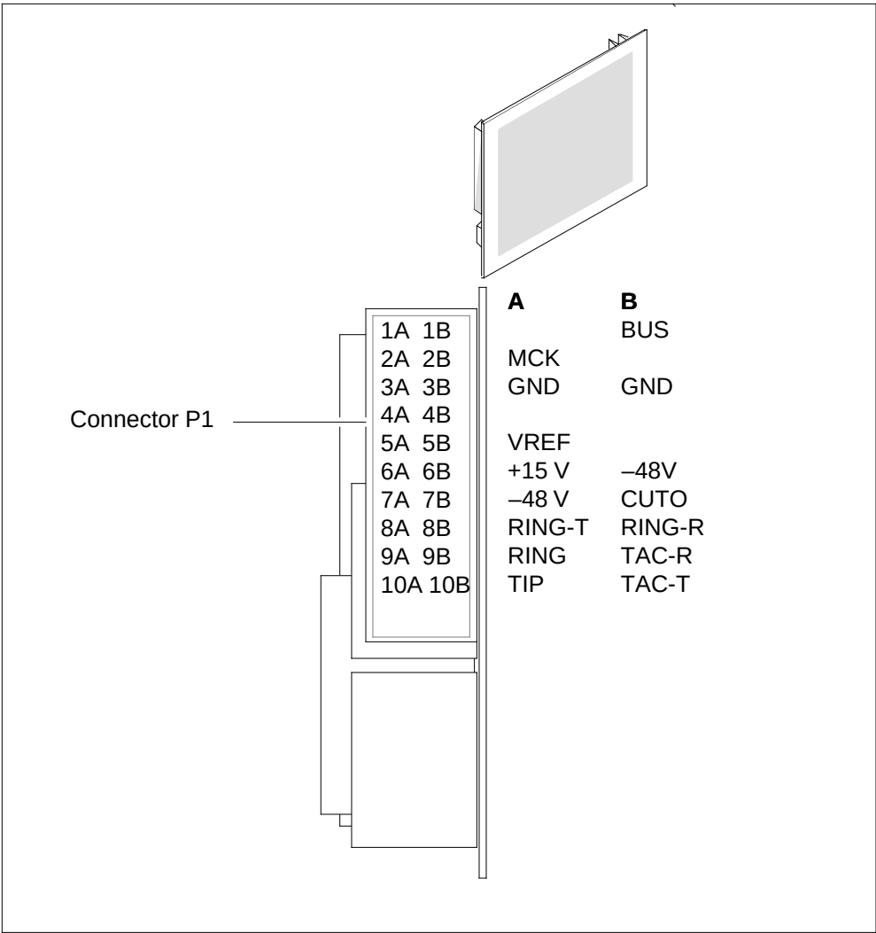
NT6X93AA pin numbers
