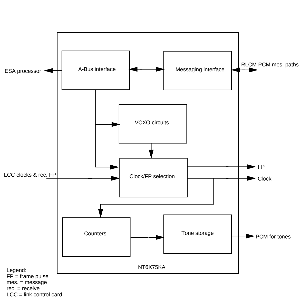
NT6X75KA functional block diagram
