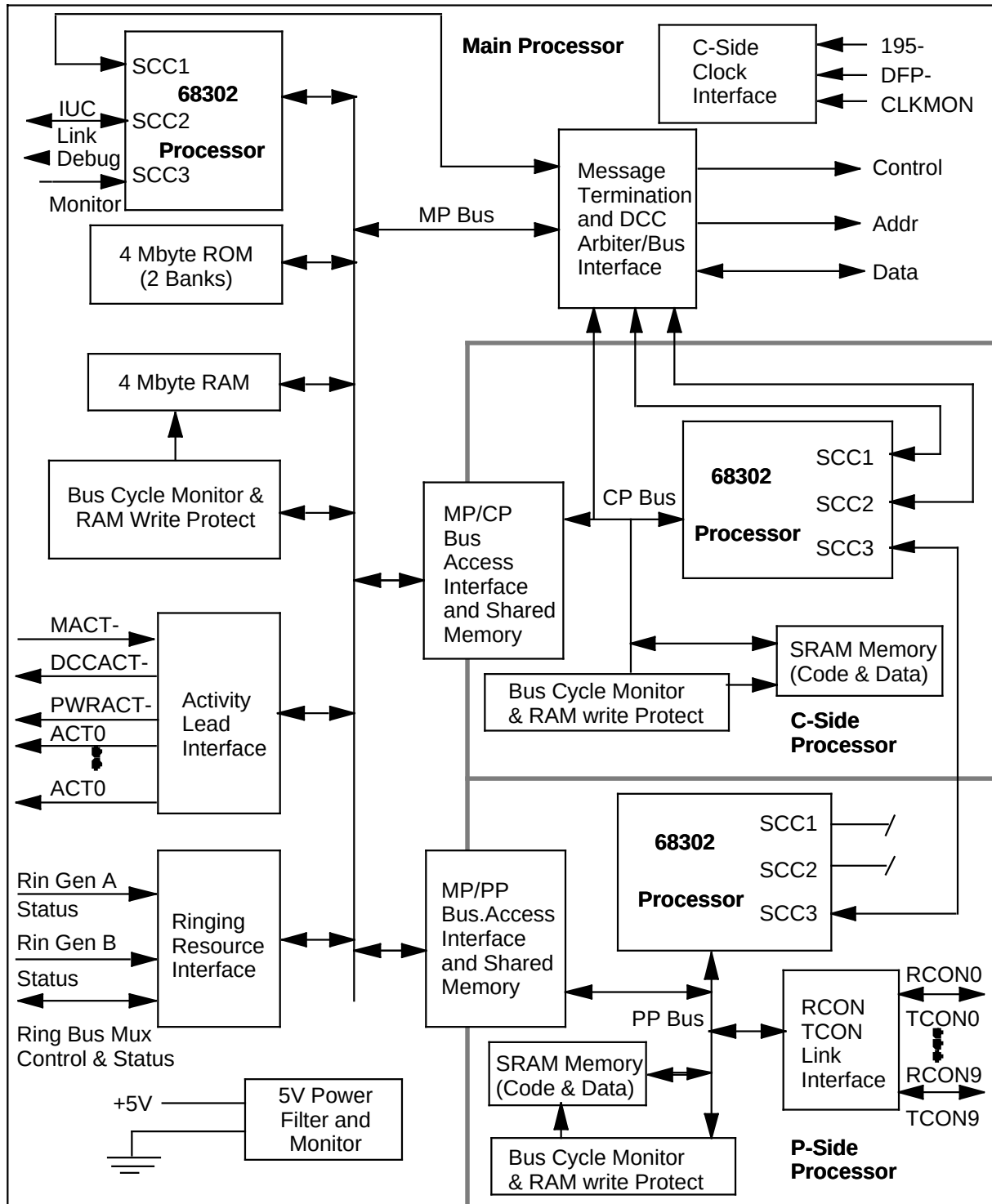
NT9X20BC functional block diagram
