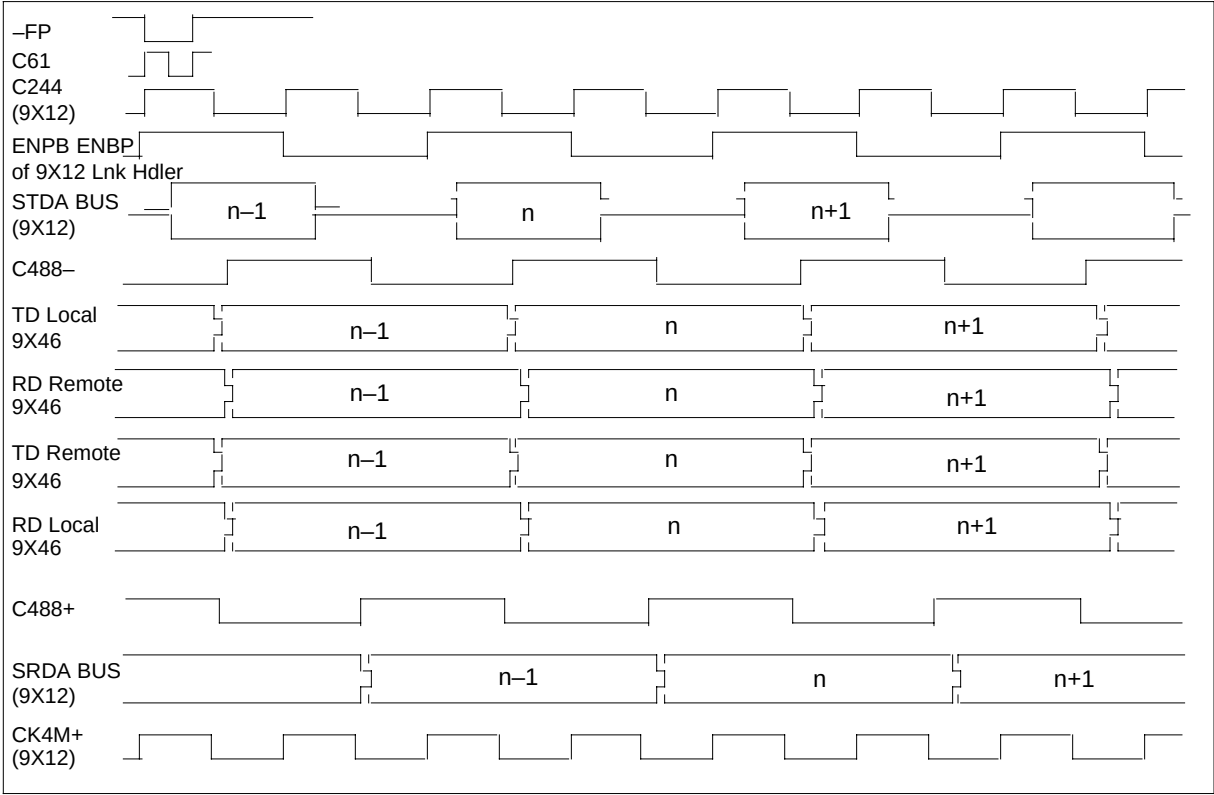
NT9X46AA remote data loop: NT9X12 to NT9X46AA to NT9X12 timing
