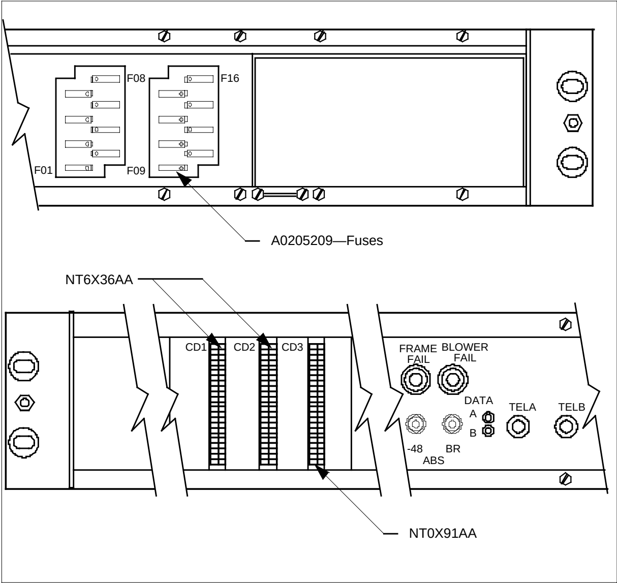
NT9X03AA front view
