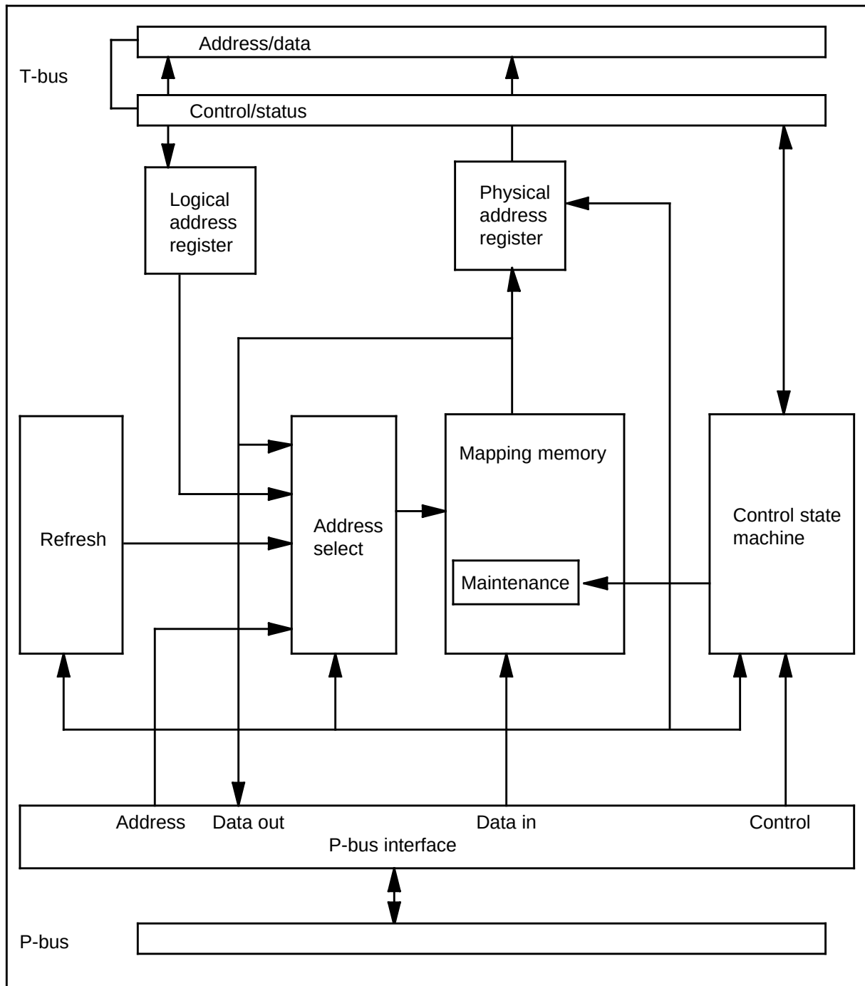
NT9X15AA functional blocks
