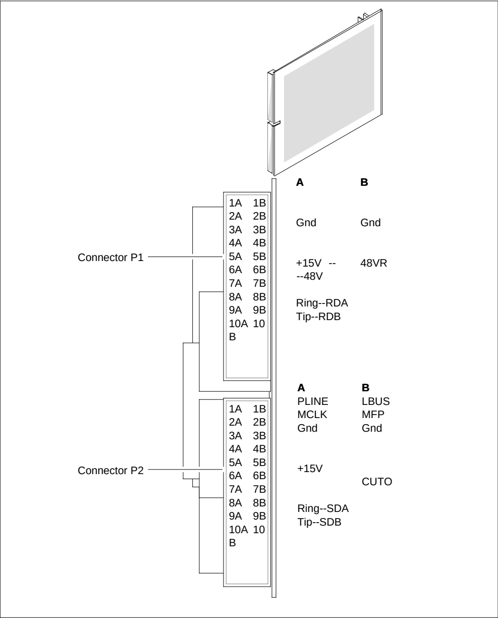
NT6X76AD pin numbers
