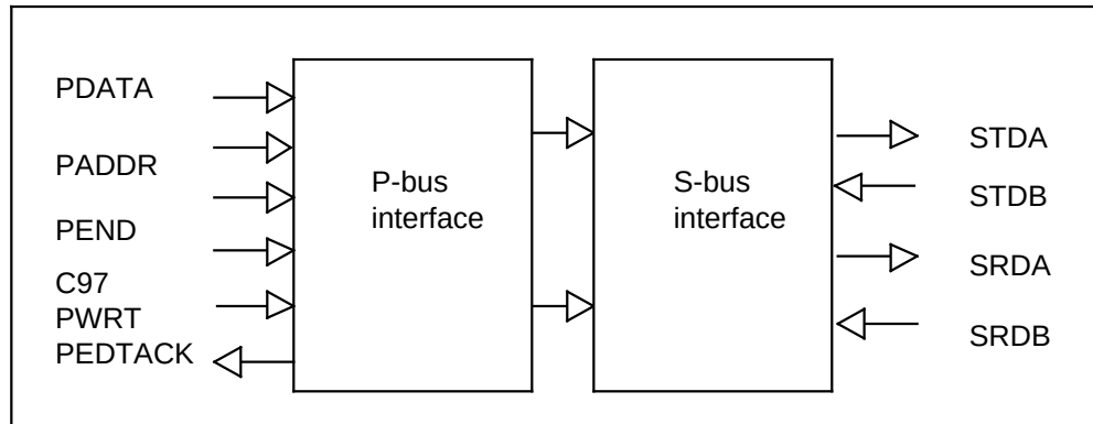
NT9X25AA functional blocks
