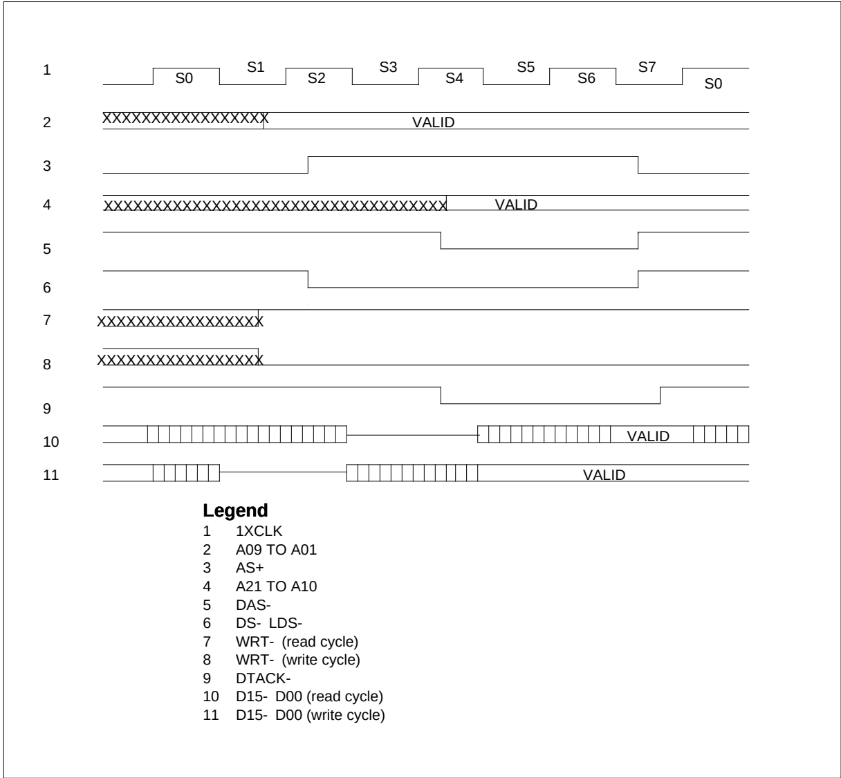
NT6X78AA timing of A-bus signals
