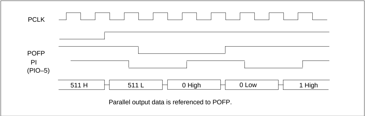
NT9X41BA parallel output port channel timing
