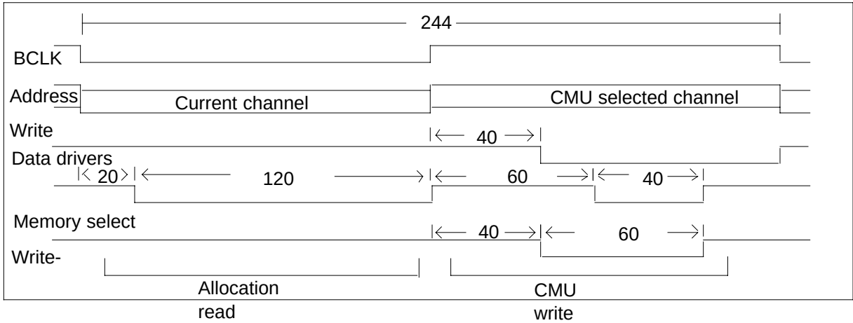
NT9X15AA CNM RAM cycle with CMU write (time is in ns)
