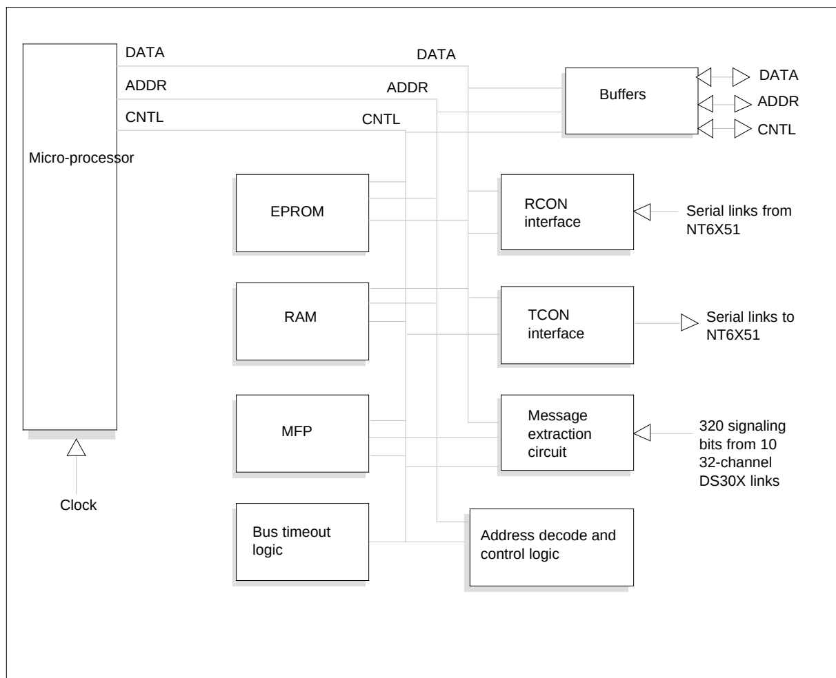
NT8X49AB functional block
