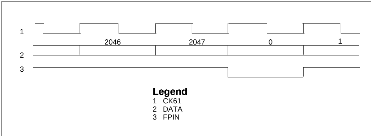
NT9X35CA V-bus timing
