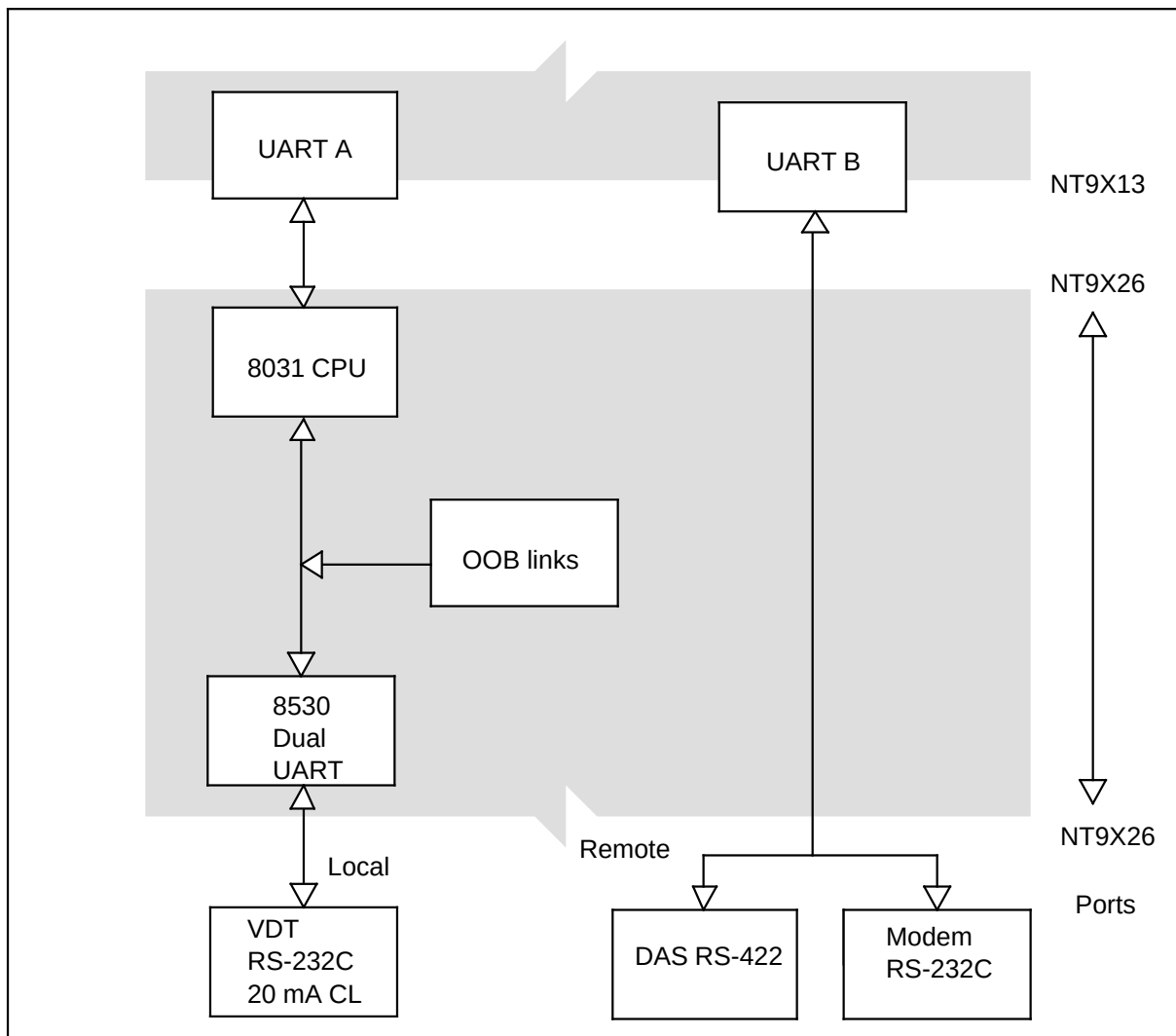
NT9X26AB functional blocks
