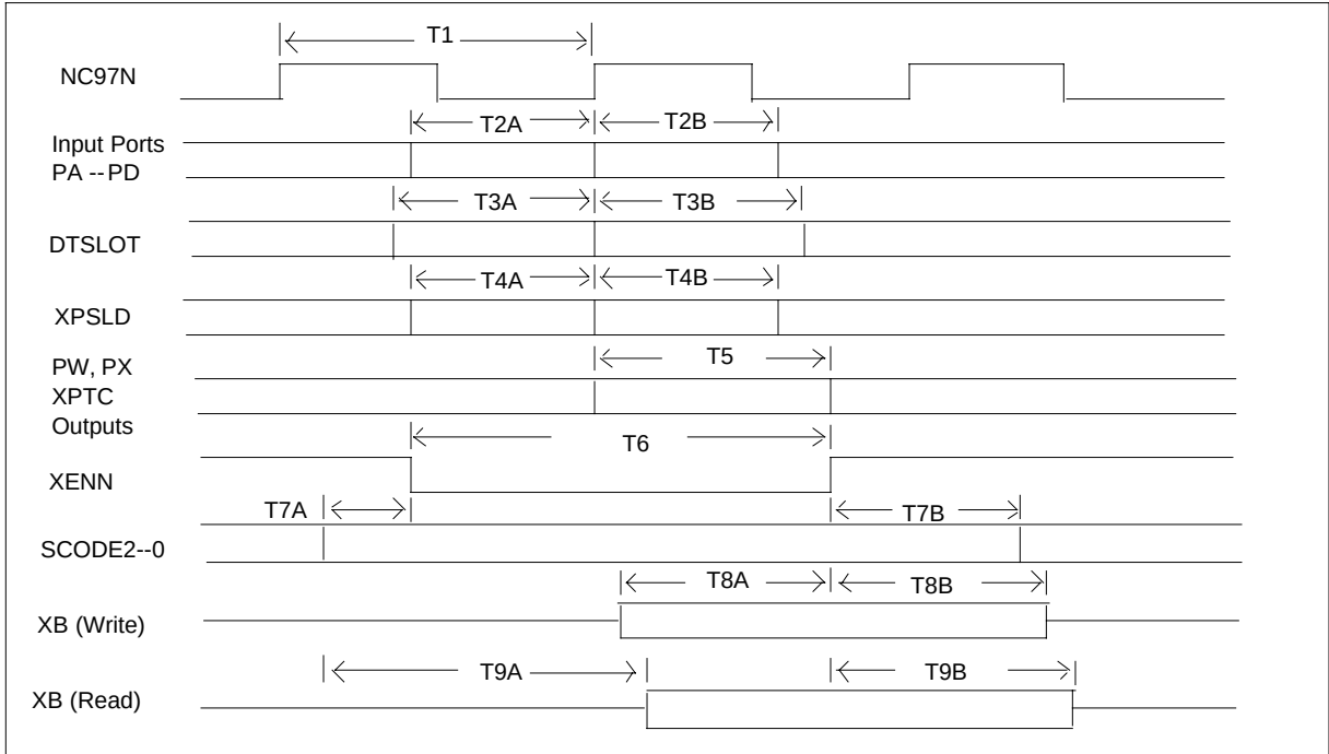
NT8X13AA timing
