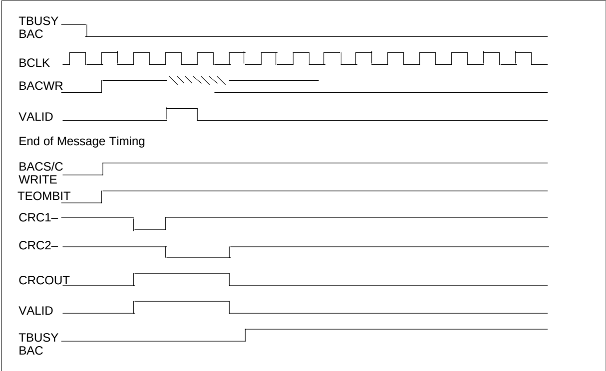
NT9X52AA P-bus to buffer data transfer timing
