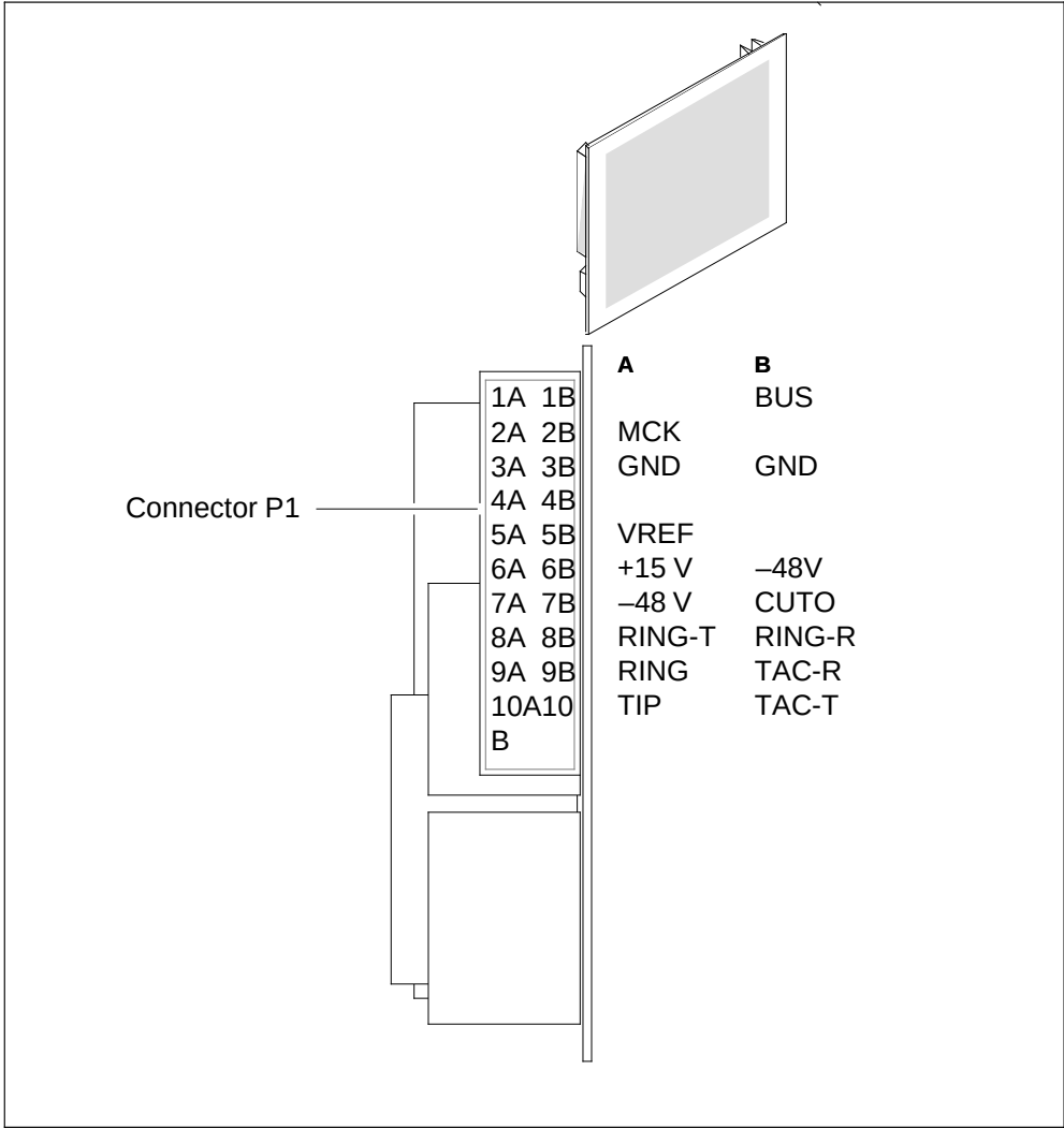
NT6X93BA pin numbers
