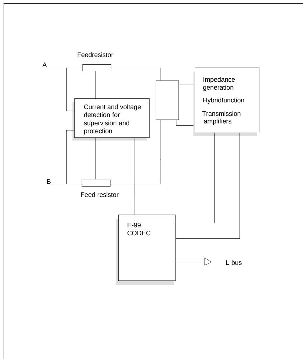
The NT6X93DA functional blocks
