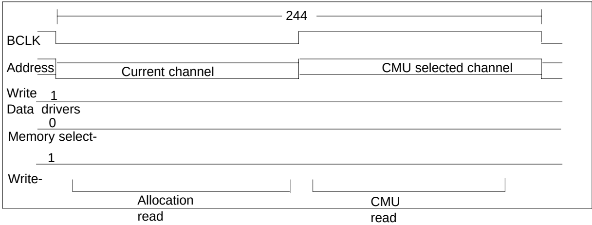
NT9X15AA CNM RAM cycle with CMU read (time is in ns)
