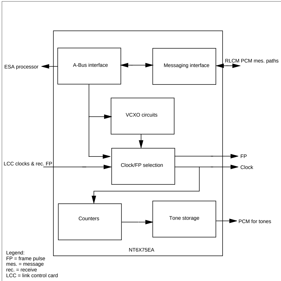
NT6X75EA functional block diagram
