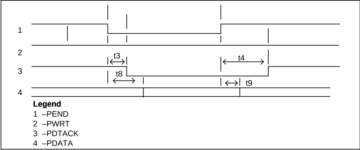
NT9X25AA processor READ cycle timing
