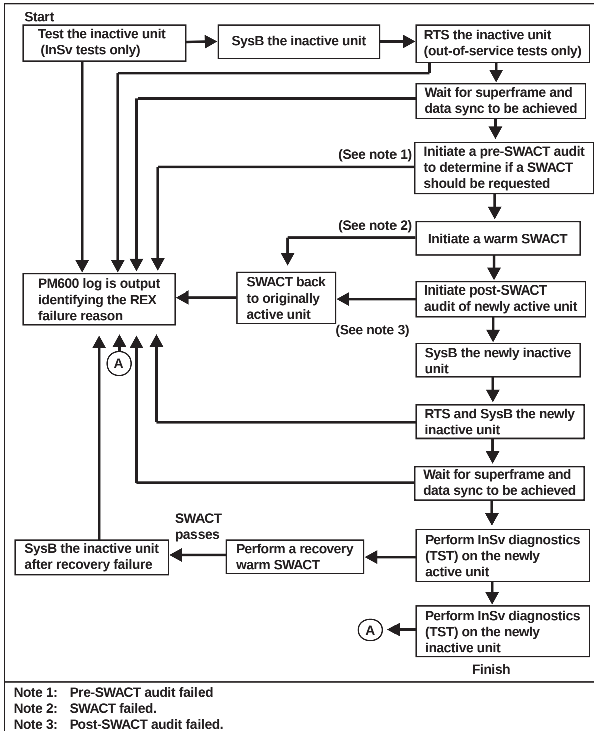
Figure 4-61 — REX test state machine actions
