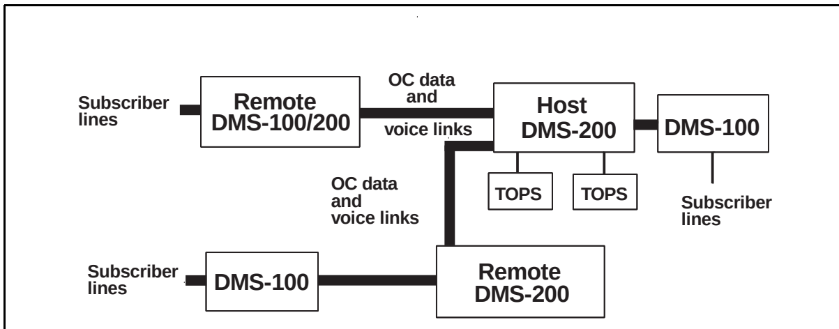
Figure 4-1 — Sample of OC system architecture
