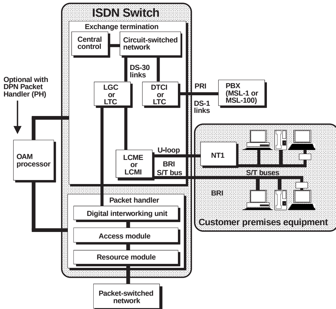
Figure 4-10 — Key components of the ISDN network (Example with DPN series of packet handler)
