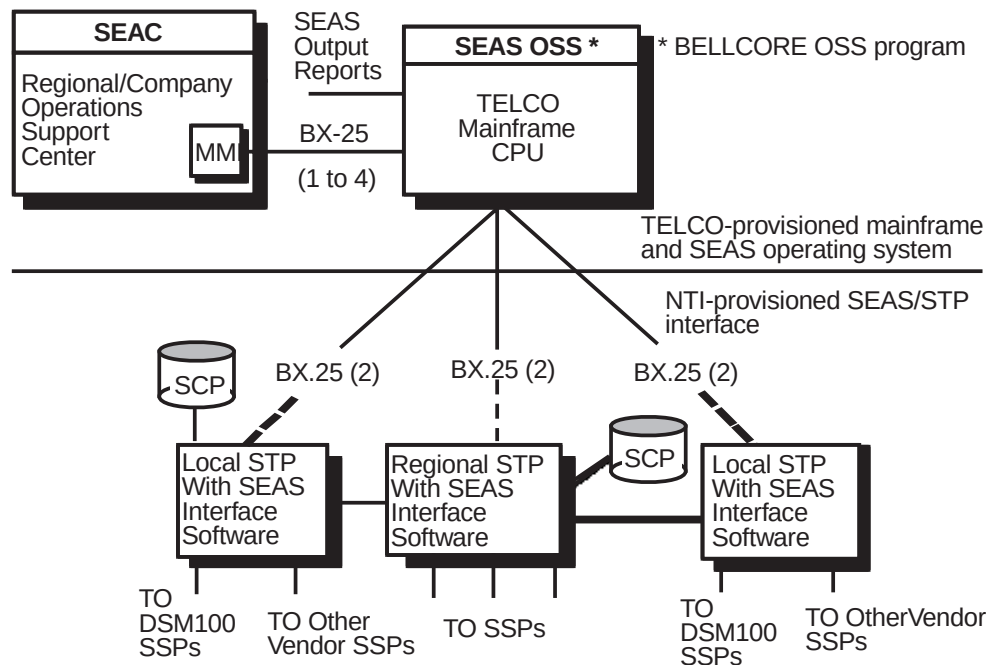
Figure 4-39 — SEAS Elements
