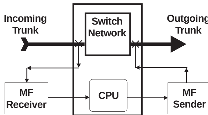
Figure 4-18 — Per-trunk signaling
