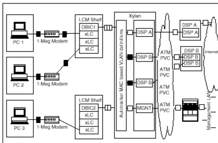
Figure 4-82 — VLAN configuration
