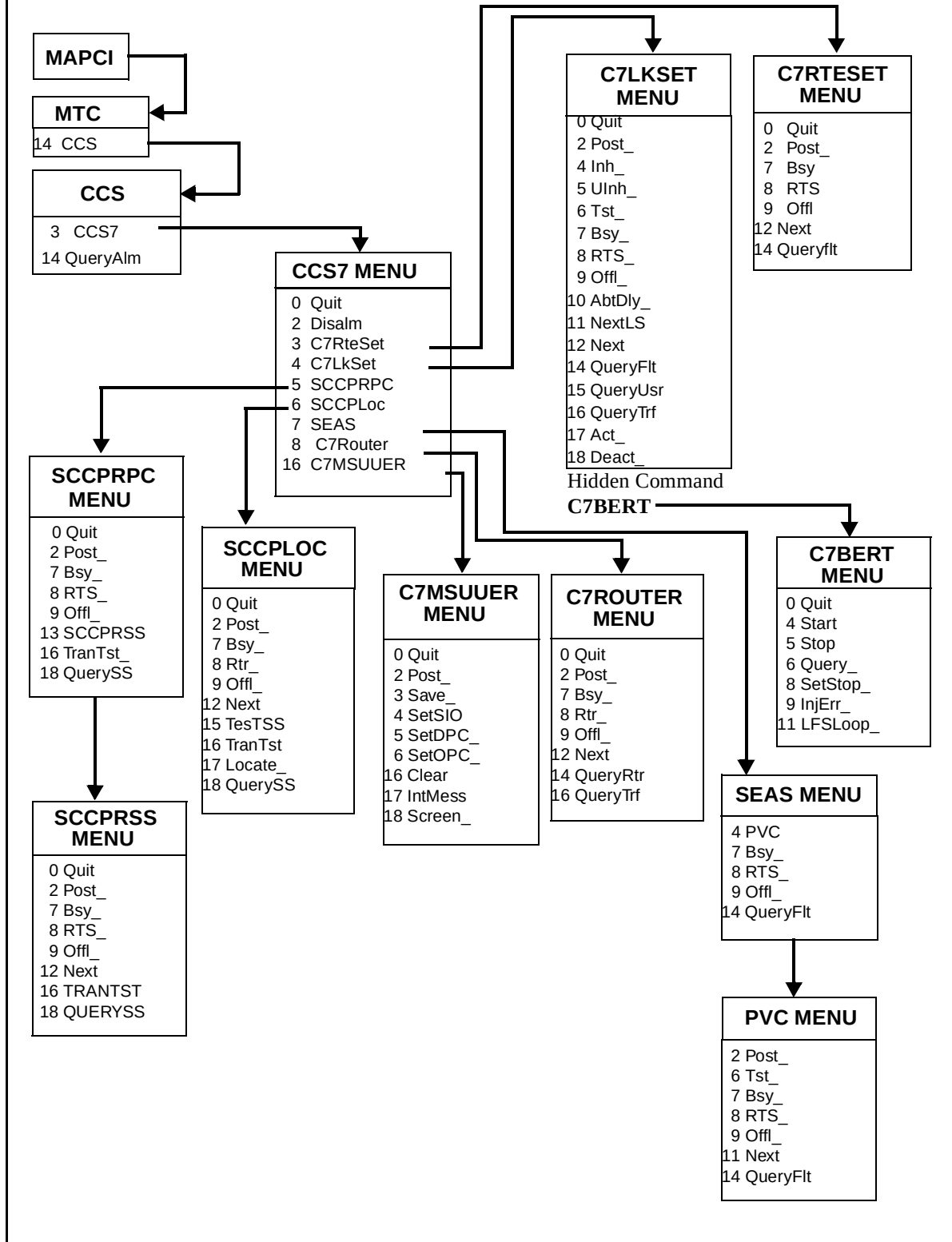
Figure 4-26 — MAP level SS7 hierarchy and
