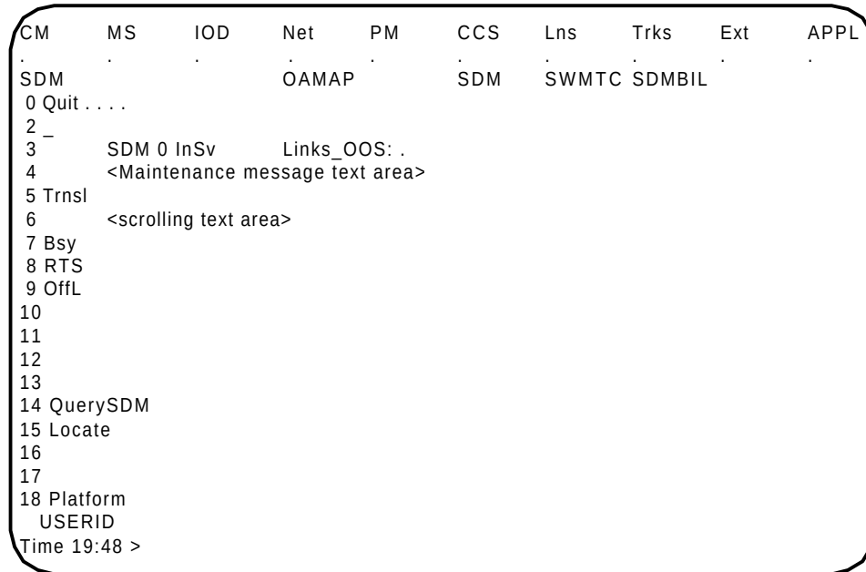
Figure 4-66 — SDM MAP level
