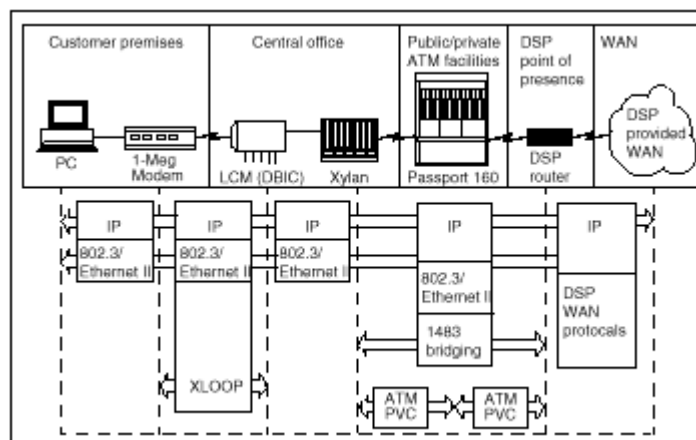
Figure 4-81 — Protocols in network
