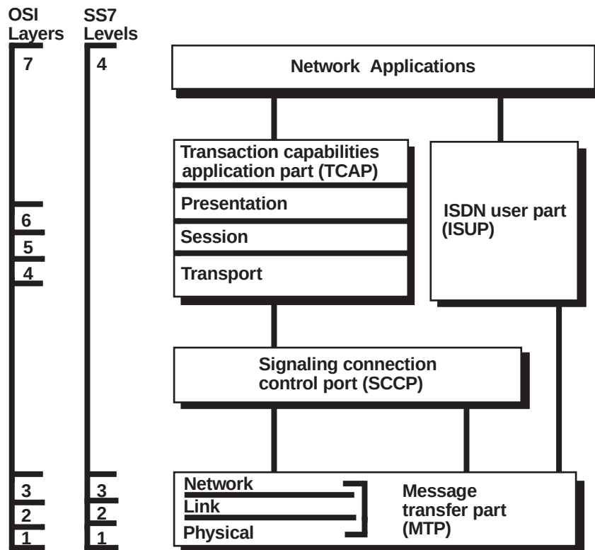
Figure 4-19 — SS7/OSI architecture
