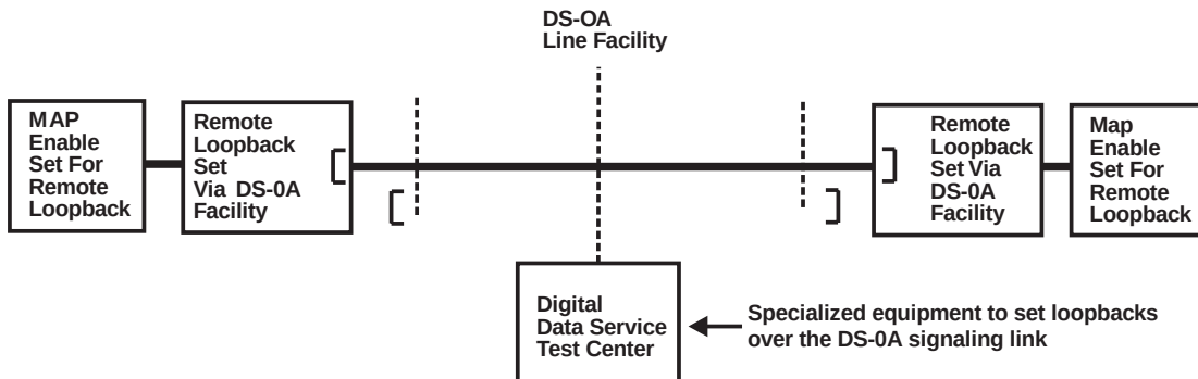
Figure 4-35 — DS0A Loopback & MTP BERT Testing — Typical remote testing from a DDS
