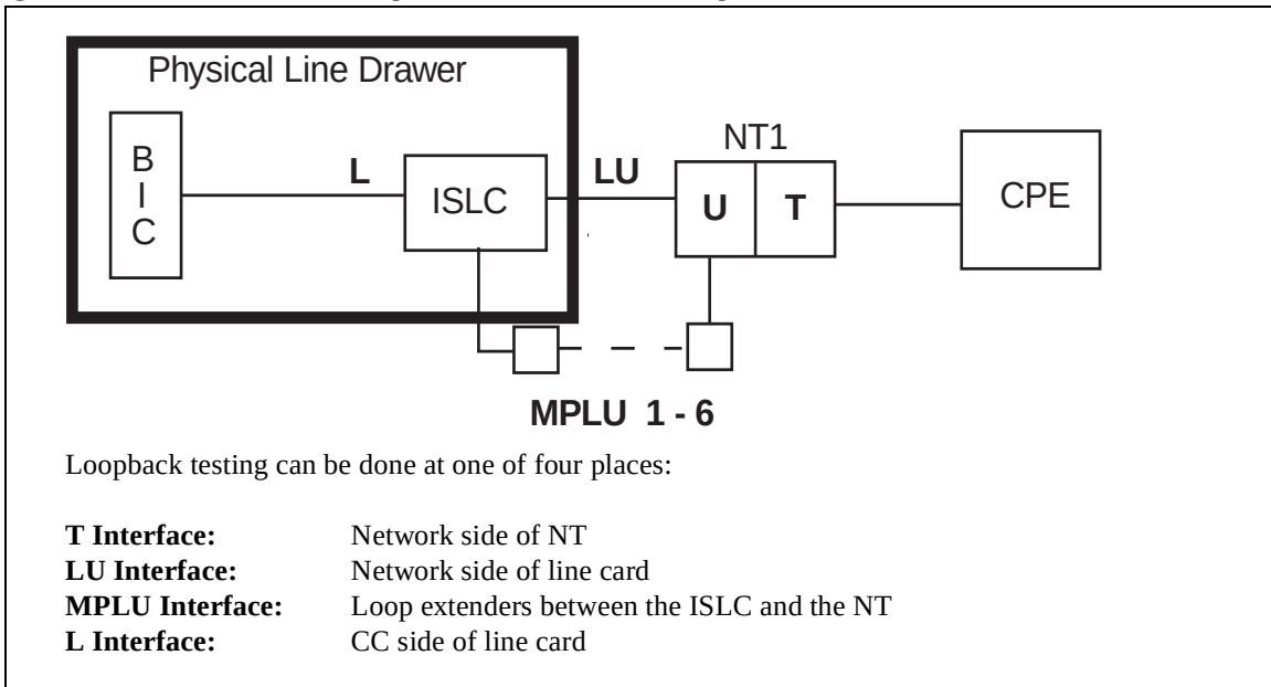
Figure 4-12 — Loopback reference points
