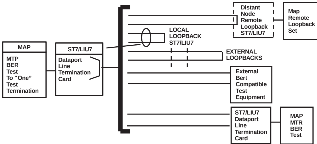
Figure 4-34 — DS0A Loopback & MTP BERT Testing — SS7 MTP BERT Tests and Terminations
