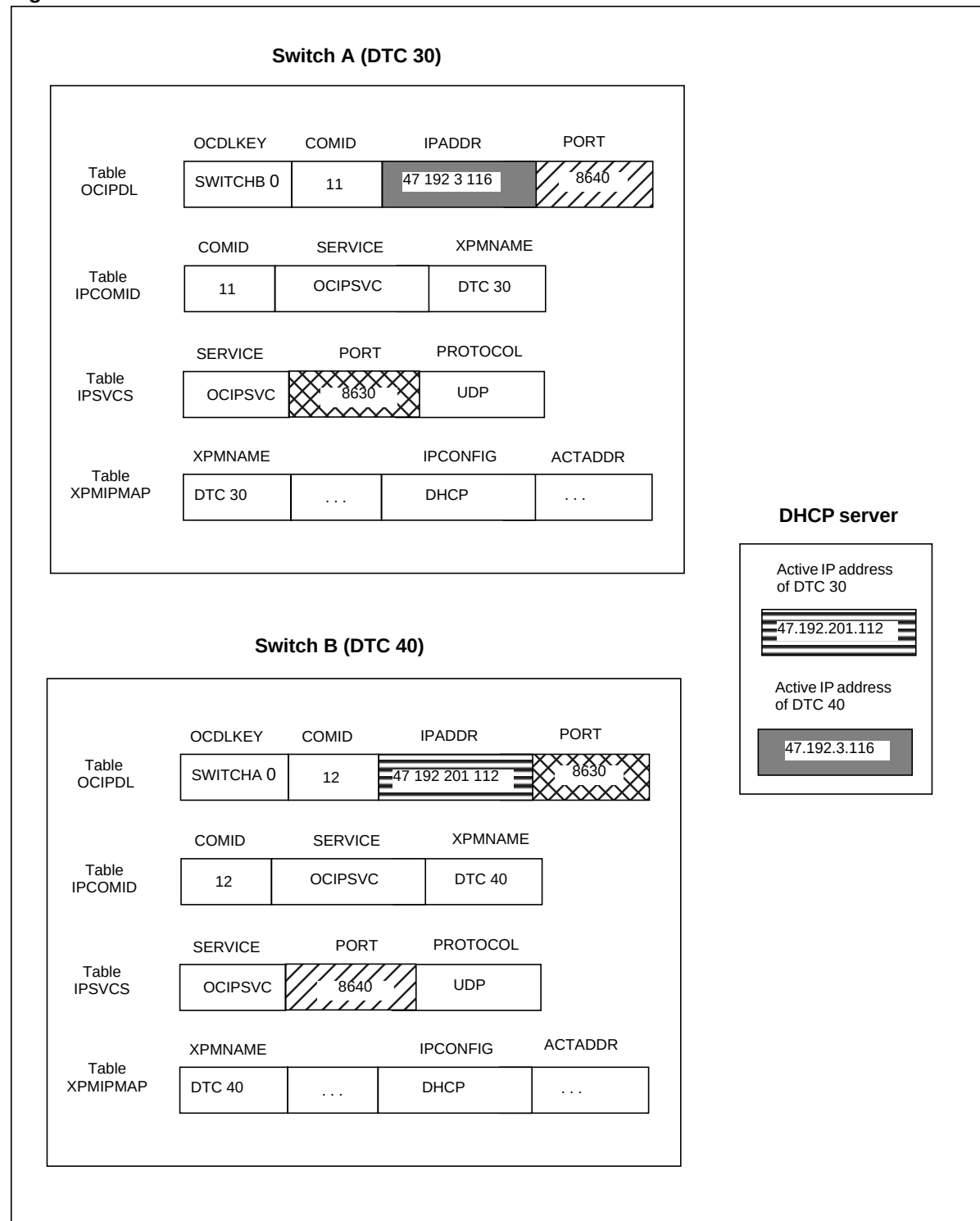
Figure 47 Parallel datafill for OC-IP data links—network method
