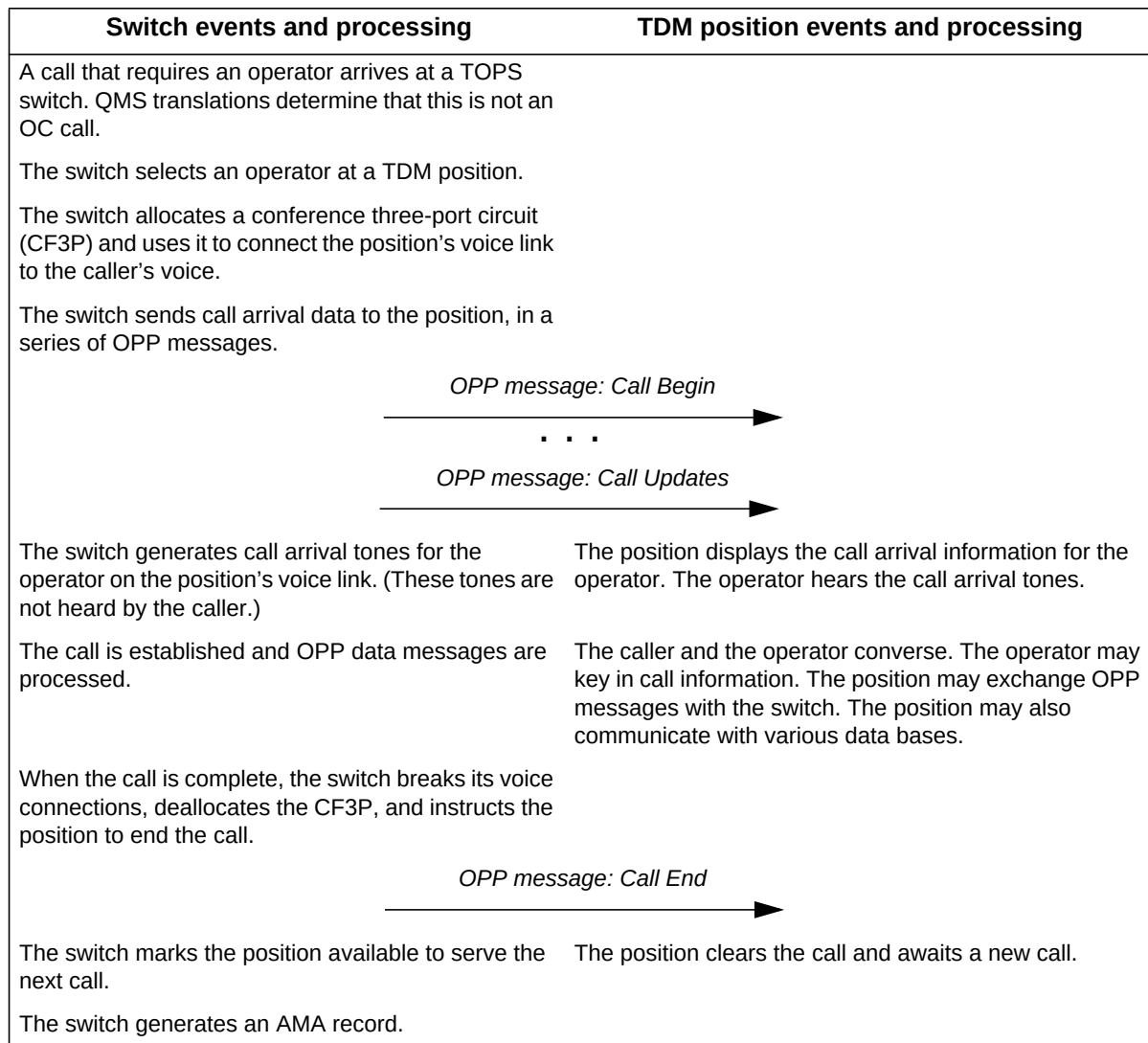
Figure 67 Example of traditional standalone call flow
