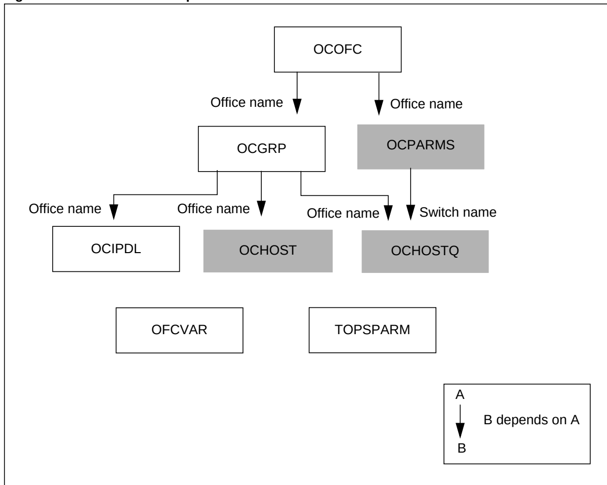
Figure 130 OC-IP datafill dependencies
