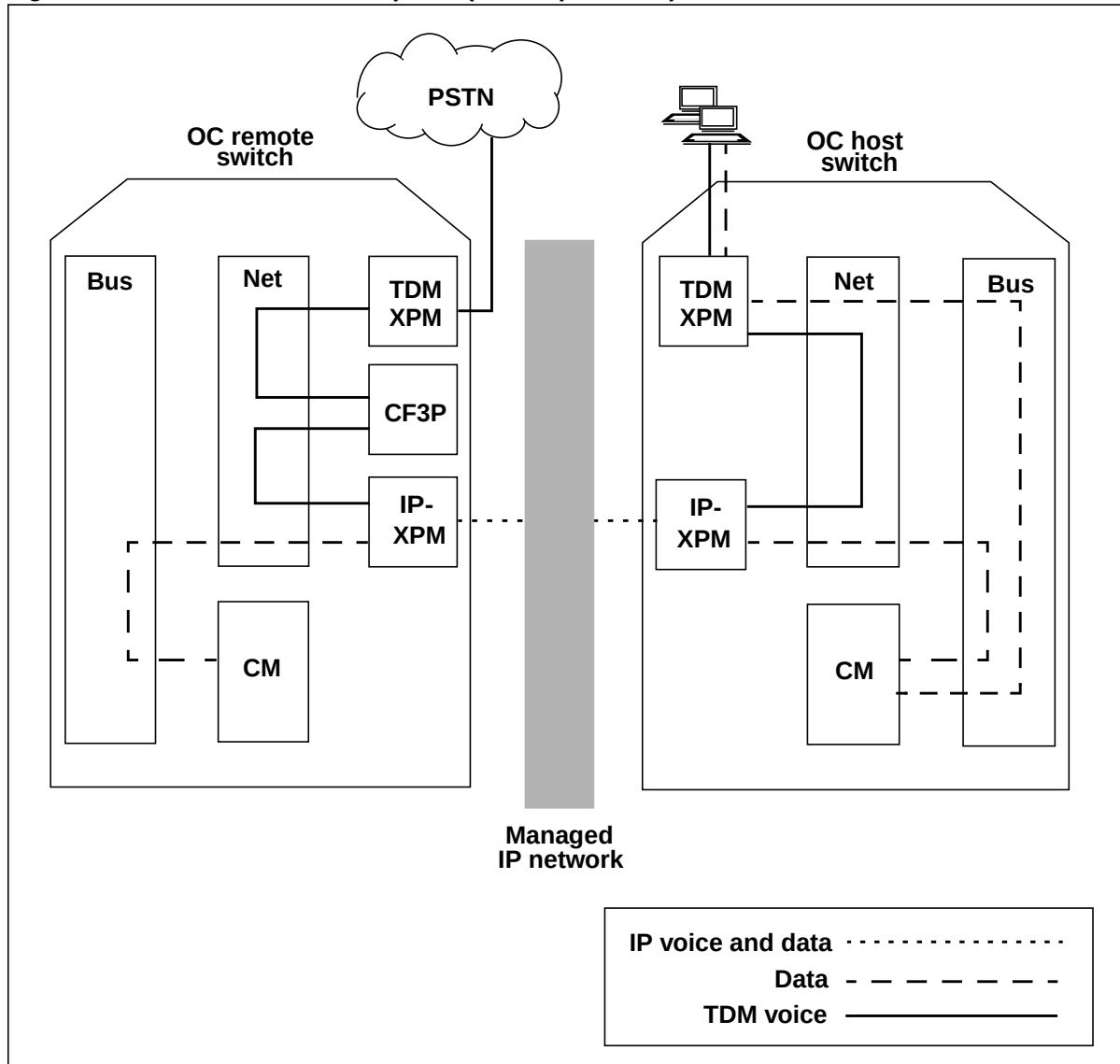
Figure 36 OC-IP voice and data paths (non-IP positions)
