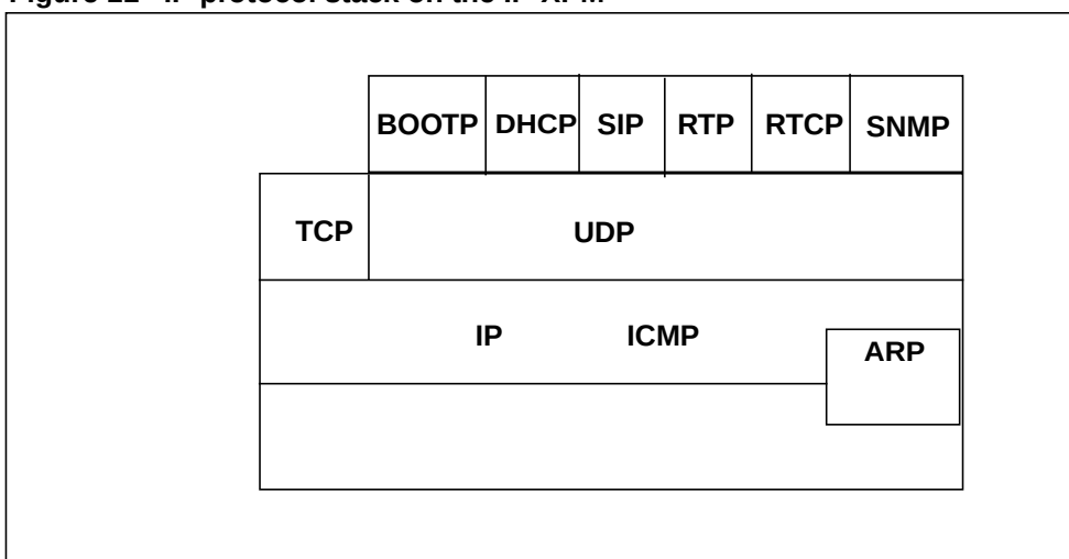
Figure 11 IP protocol stack on the IP-XPM
