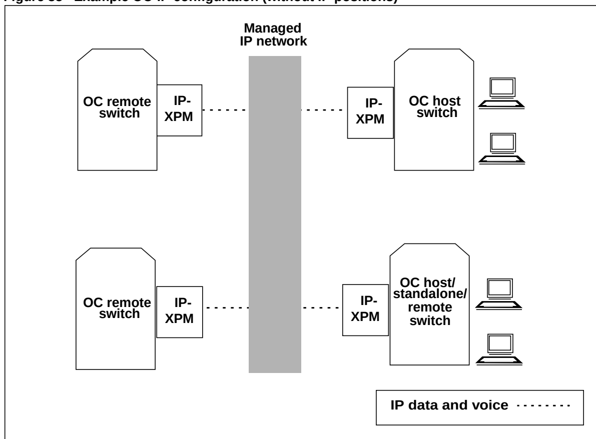
Figure 35 Example OC-IP configuration (without IP positions)
