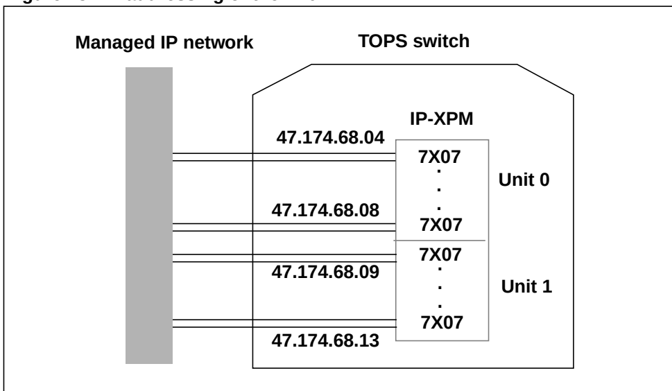
Figure 13 IP addressing of the 7X07AA
