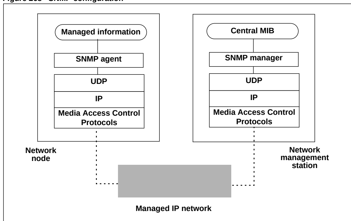
Figure 268 SNMP configuration
