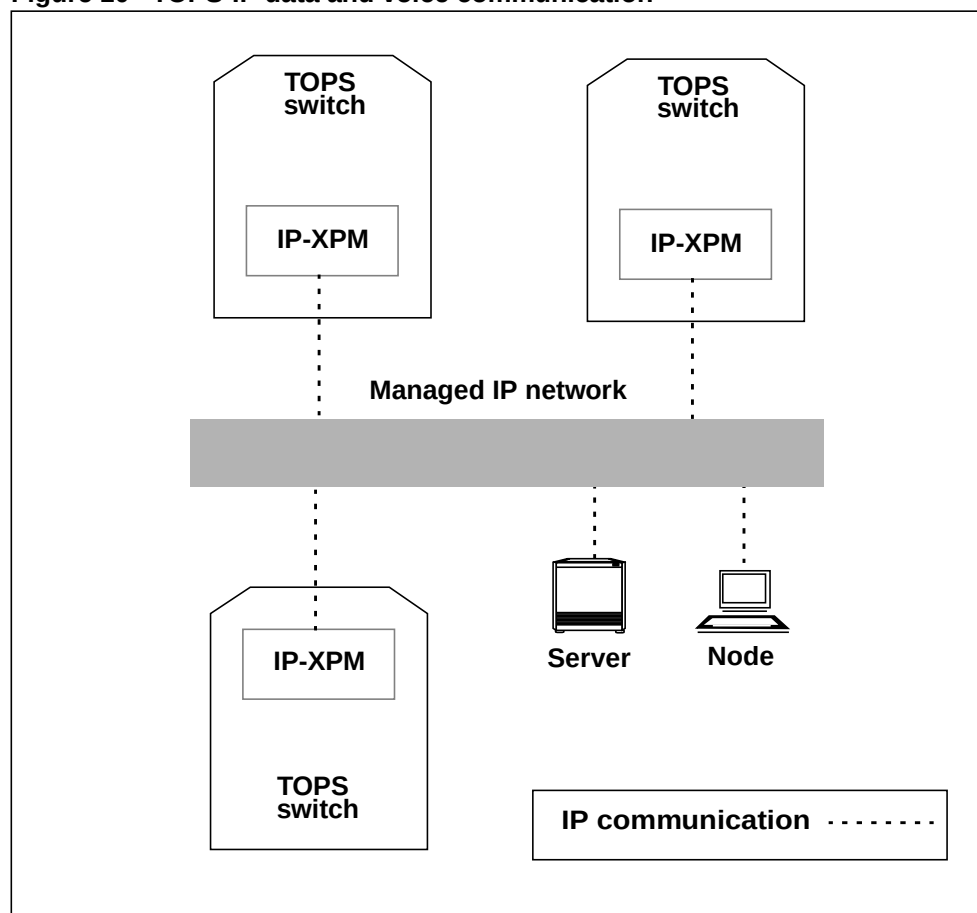
Figure 10 TOPS-IP data and voice communication
