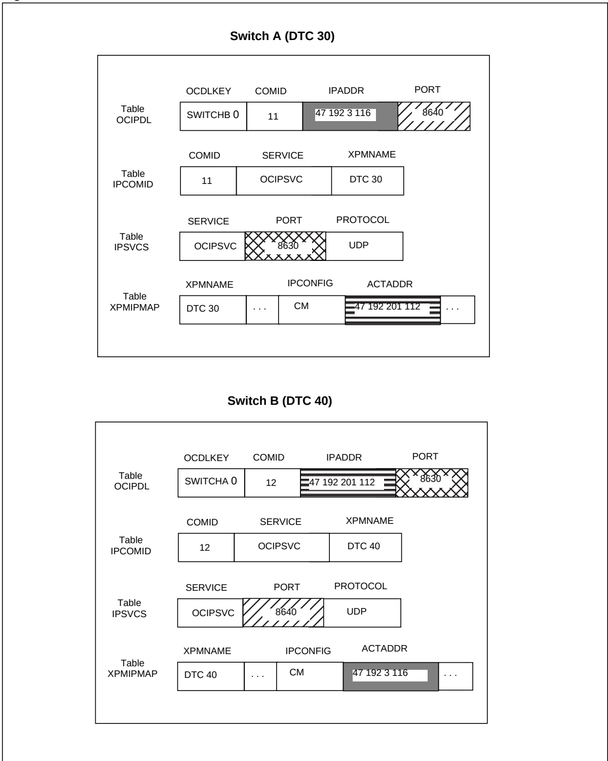
Figure 48 Parallel datafill for OC-IP data links—CM method
