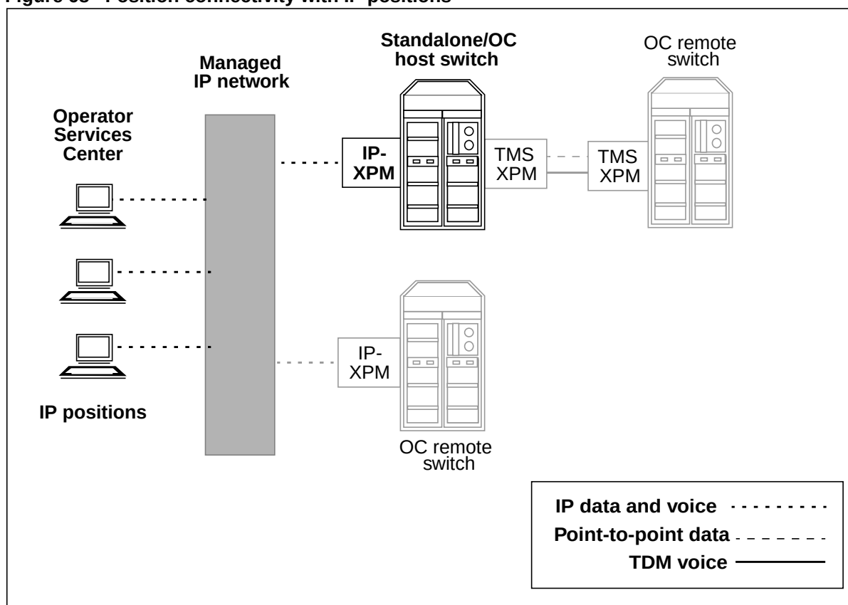
Figure 68 Position connectivity with IP positions
