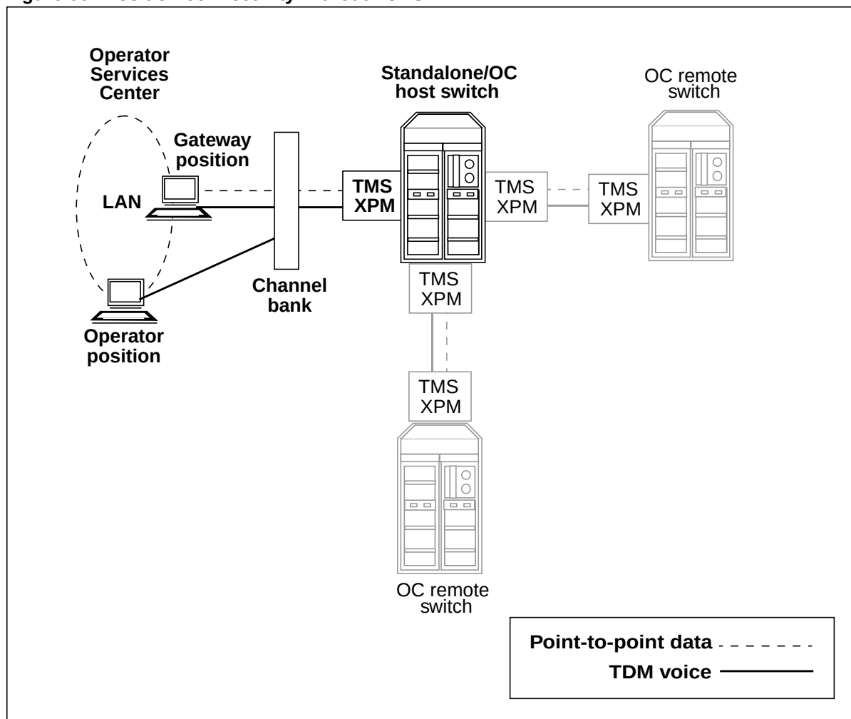
Figure 66 Position connectivity without TOPS-IP
