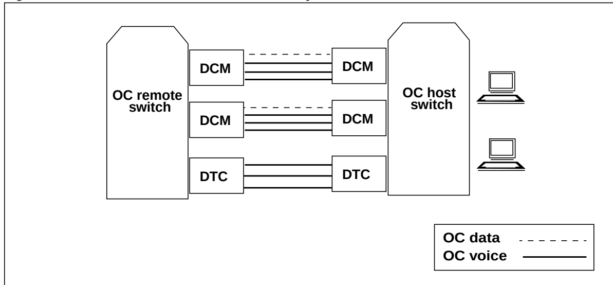
Figure 32 DCM OC data and voice connectivity
