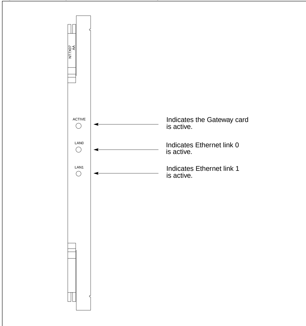
Figure 160 Gateway LED indicators on the faceplate
