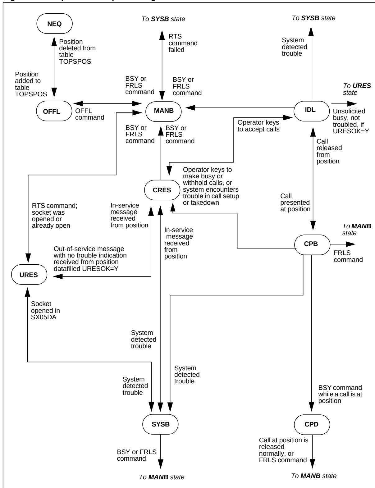
Figure 168 IP position call processing and maintenance states
