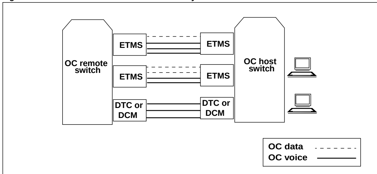
Figure 33 ETMS OC data and voice connectivity
