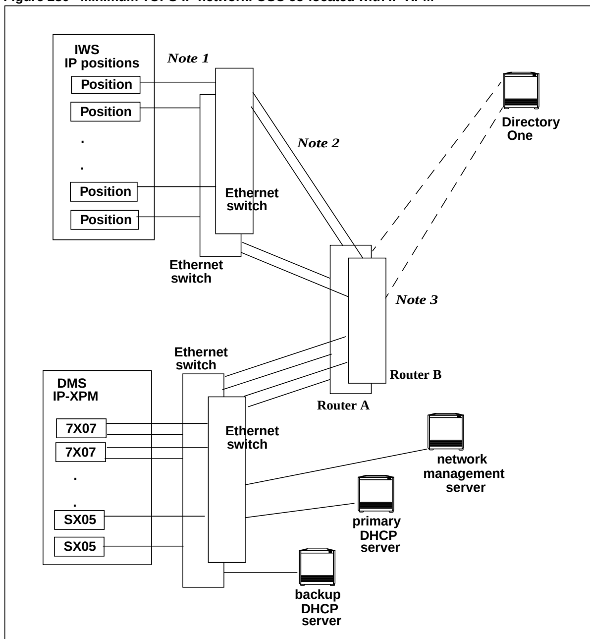
Figure 280 Minimum TOPS-IP network: OSC co-located with IP-XPM
