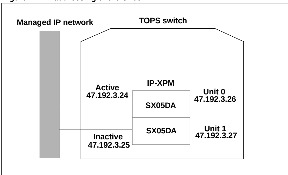
Figure 12 IP addressing of the SX05DA
