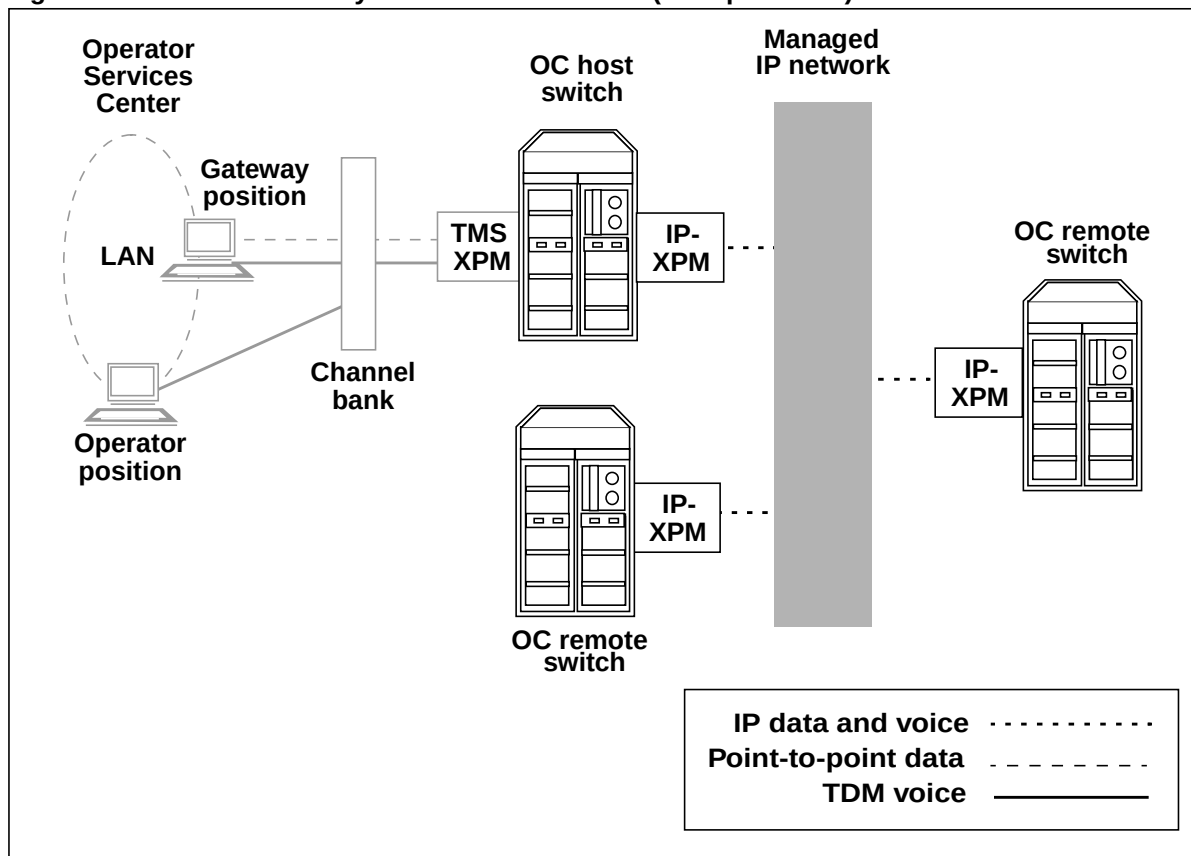
Figure 5 OC-IP connectivity in a TOPS-IP network (TDM positions)
