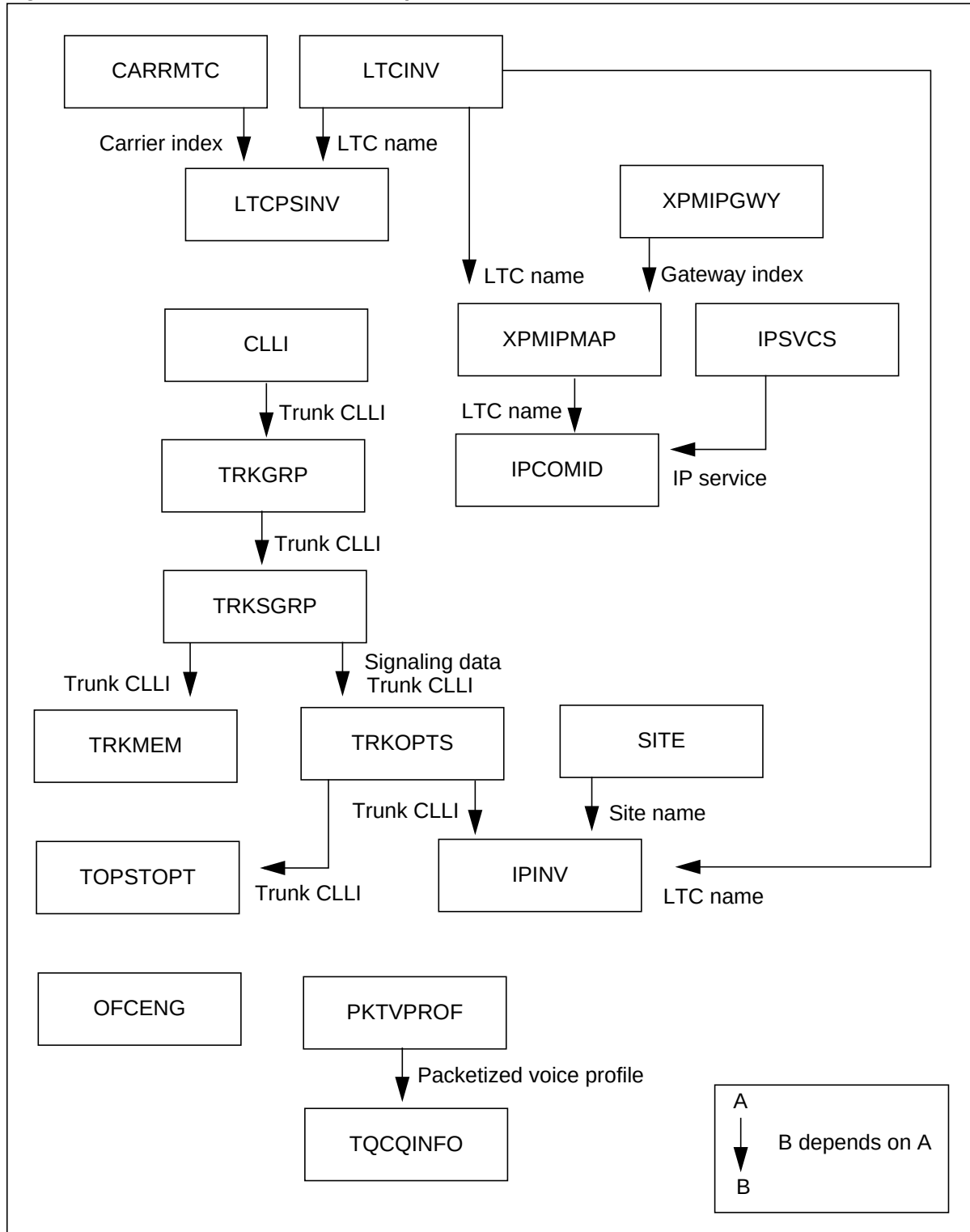
Figure 111 IP infrastructure datafill dependencies
