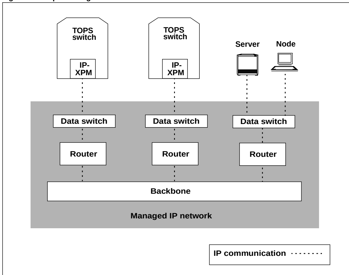
Figure 3 Simple managed IP network
