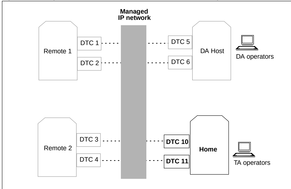
Figure 49 Configuration for OC-IP voice communication datafill examples
