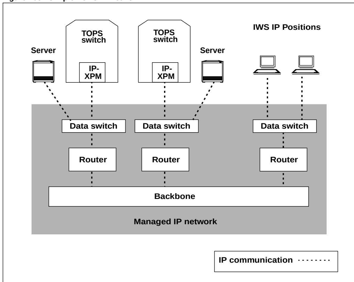
Figure 108 Simple TOPS-IP network
