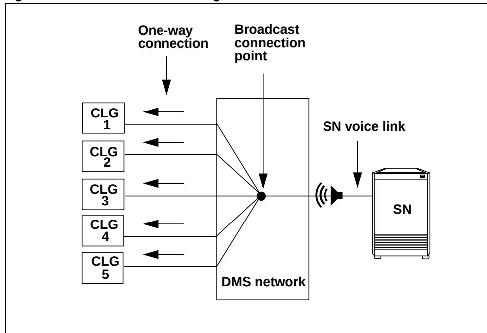
Figure 76 Voice link broadcasting to five calls
