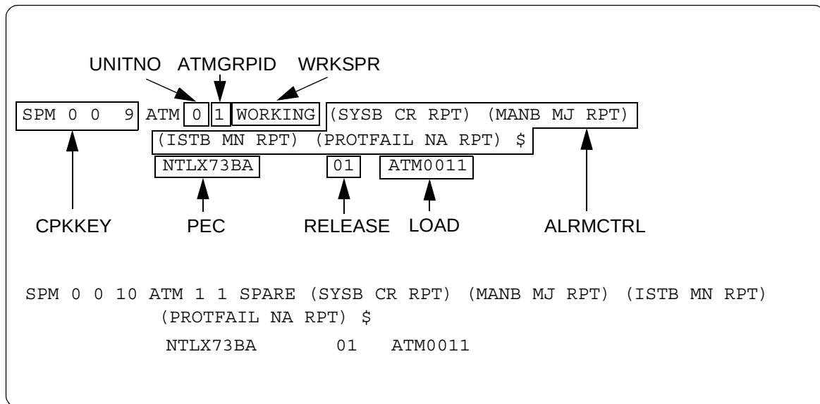
MAP display example for DLC card in table MNCKTPAK
