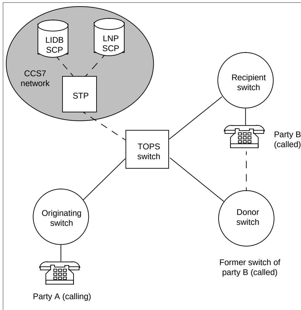
LNP network configuration
