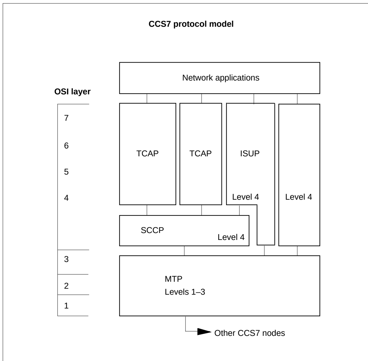
Figure 1-5 CCS7 architecture
