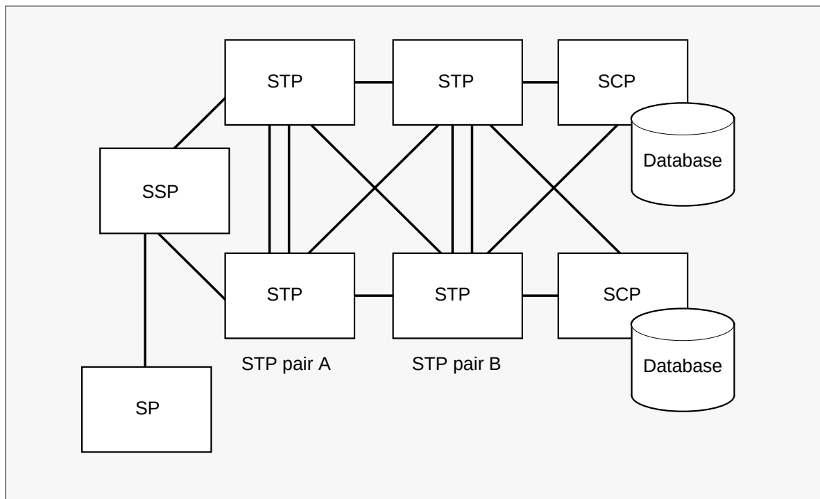
Figure 1-3 CCS7 nodes in a signaling network
