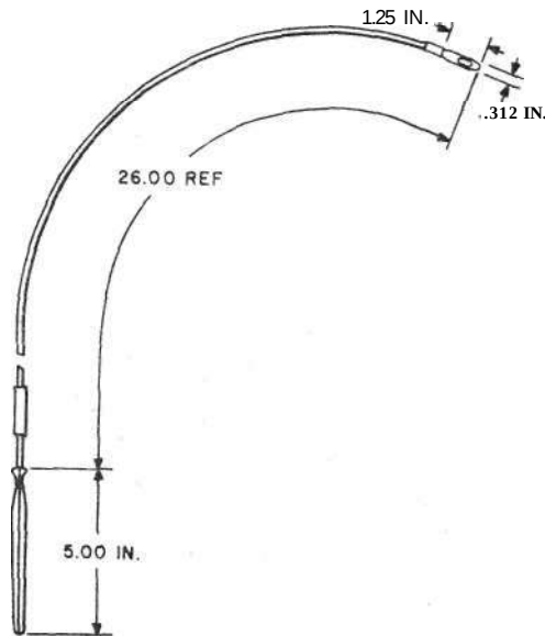
Fig. 5—&gt;KS-20096 L1 Needle&lt;
