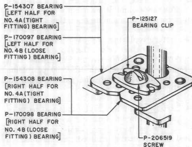
Fig. 9 - 4-type Bearing Parts
