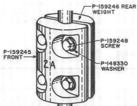
Fig. 4 - Compensator Used on District Finder Rods
