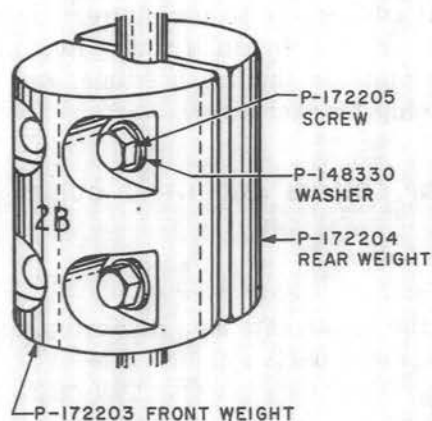
Fig. 5 - Compensator Used on Sender Selector Rods
