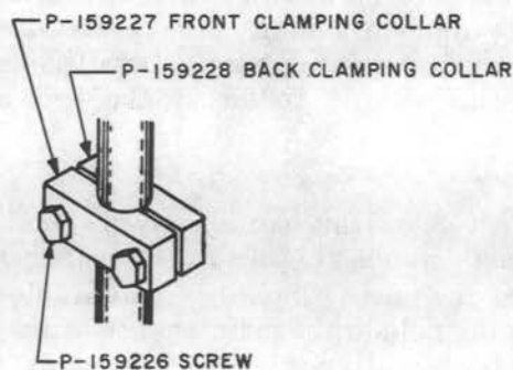
Fig. 2 - Upstop or Downstop Collar
