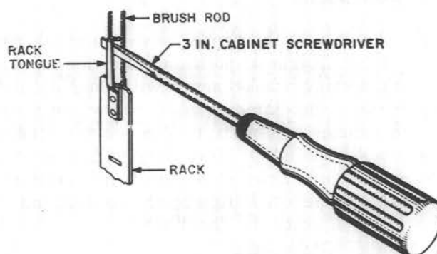
Fig. 10 — Method of Removing Rack From Brush Rod
