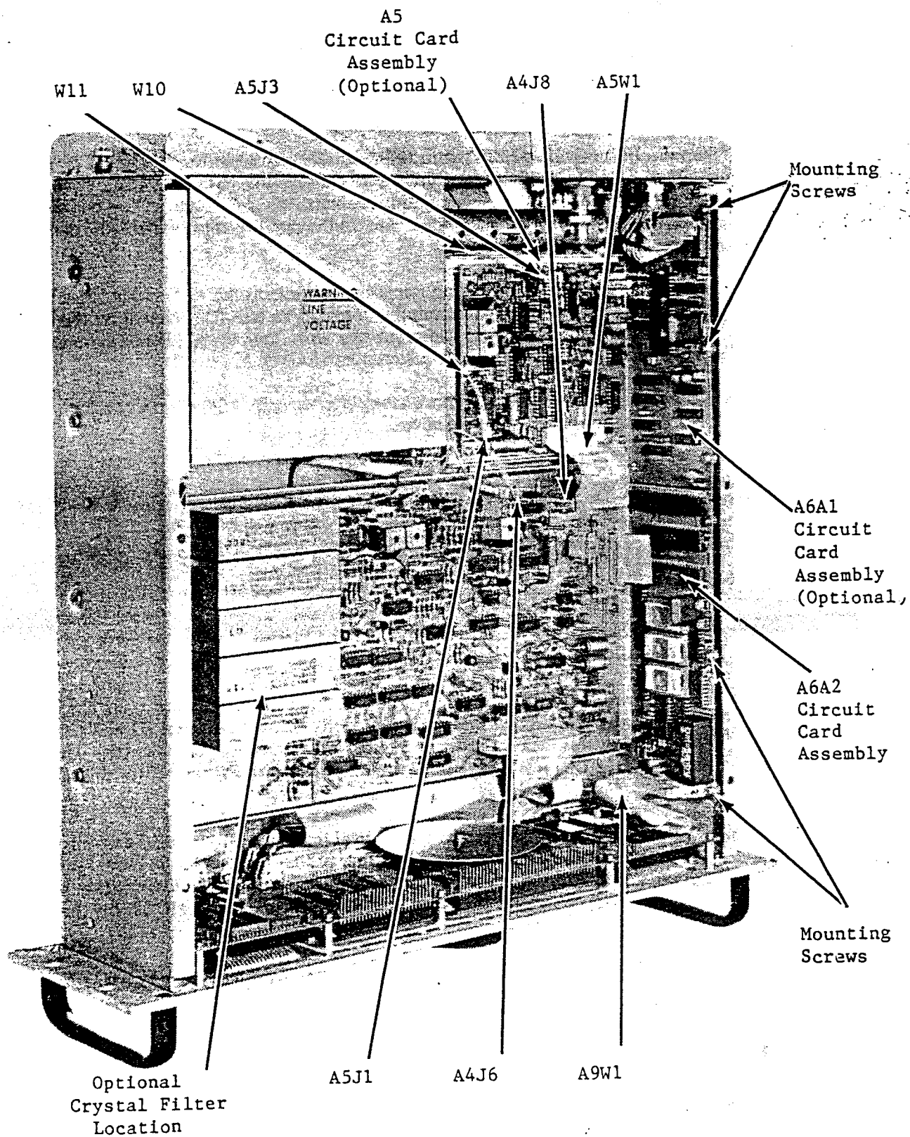
Figure 2-6. Receiver Options, Installation Detail
