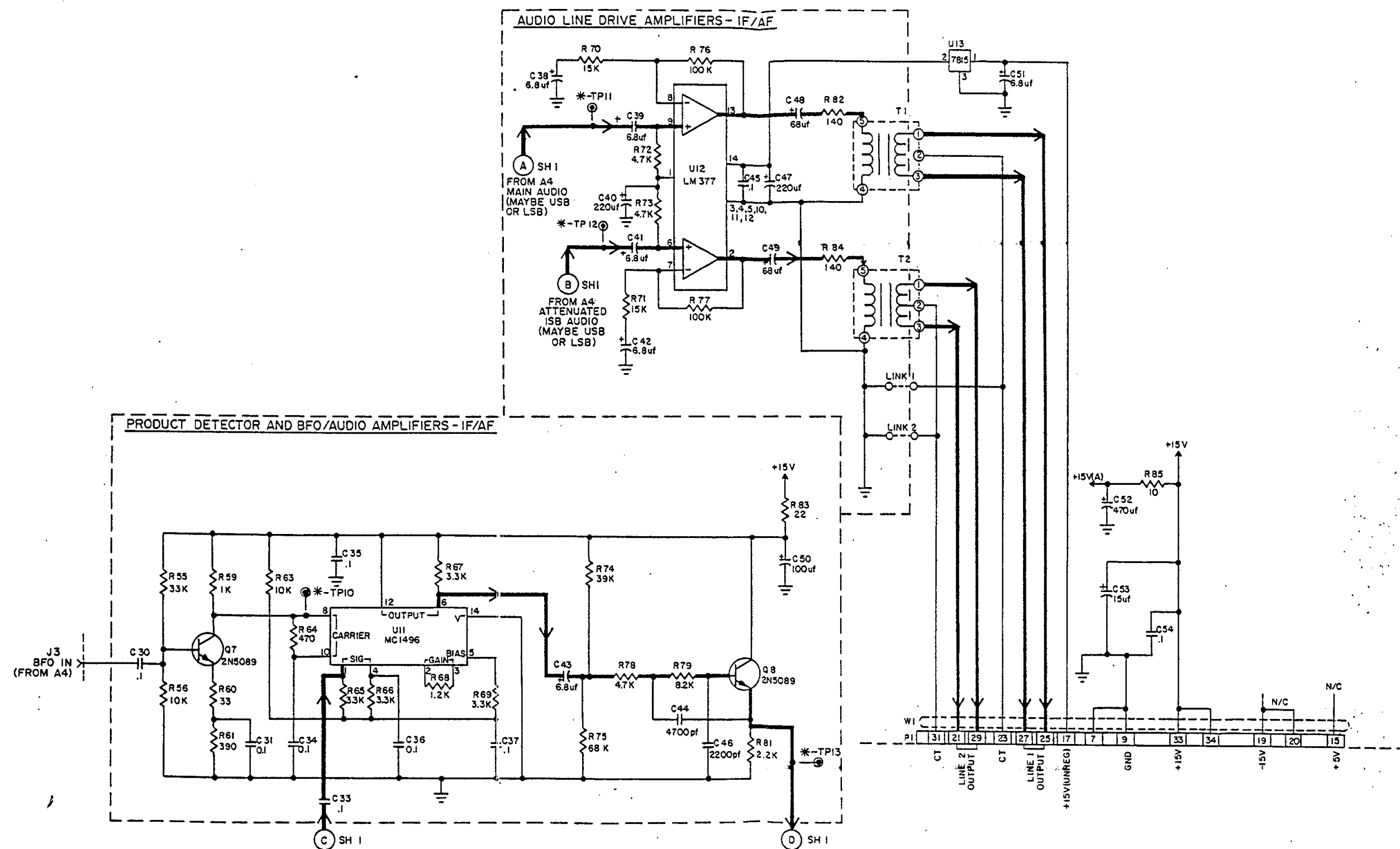
Figure 7-5. Schematic Diagram, ISB, A5 (Optional) (Sheet 2 of 2)
