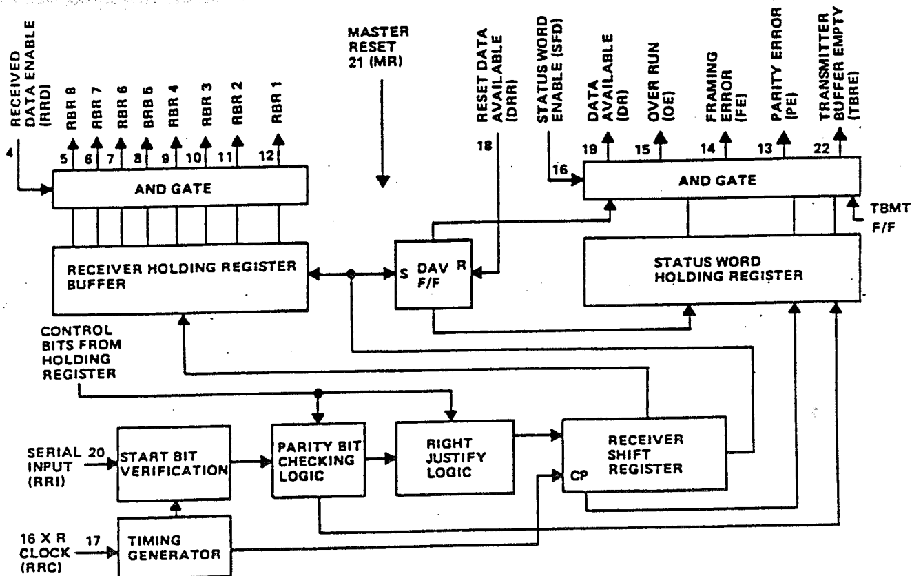
Figure 4-23. UART Receiver Functional Block Diagram
